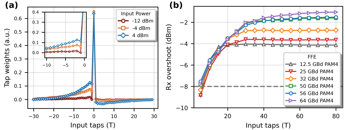
Figure 3.12: (a) Trained FFE taps showing the majority contribution of past symbols toward equalising the SOA patterning effect; (b) the strong dependence of linear FFE equalisation on the number of input taps for different baud rates.
