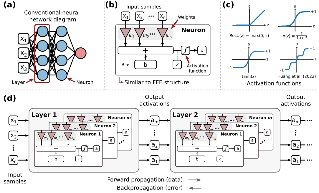
Figure 2.11: Schematics showing (a) conventional NN structure, (b) neuron operation, (c) popular activation functions, and (d) the composition of an NNE.
