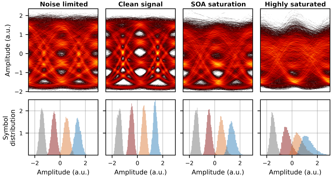
Figure 3.9: Increasing severity of SOA non-linear patterning on 100 Gbit/s PAM4 transmission as seen in eye diagrams and sampled symbol distributions.
