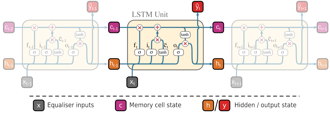
Figure 4.2: Schematic of an LSTM recurrent unit with memory cell c_t .
