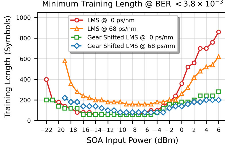
Figure 5.7: This graph shows the minimum number of training symbols required by SkipNet( K_1 + K_2 ) to achieve BER under the HD-FEC threshold with probability > 95\% across a range of SOA input powers. Rapid adaption can be achieved using the GS-LMS algorithm, comparable to that of existing FFE/DFE techniques [116].
