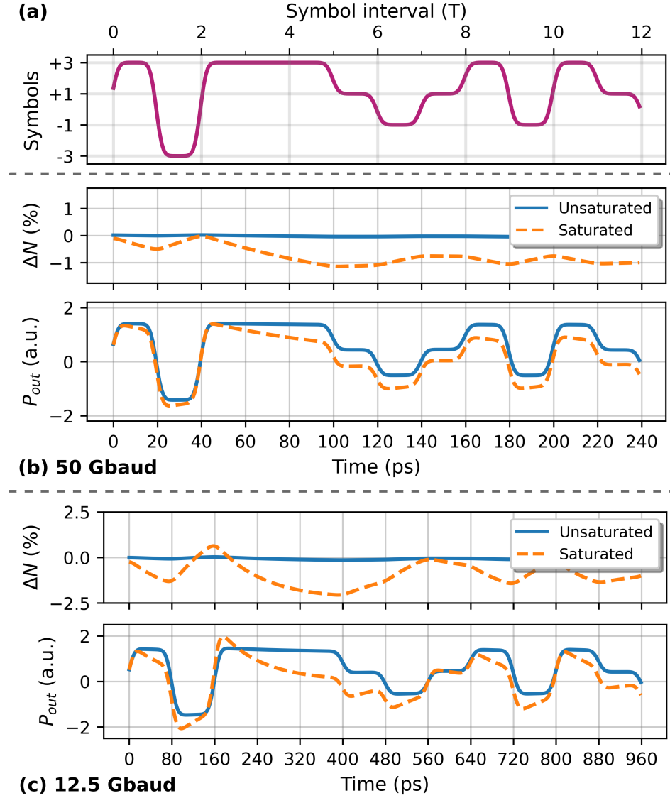
Figure 3.3: (a) The PAM4 sequence used as input to the simulated SOA device above and below the saturation input power. The percentage change in carrier density and resulting output power of the device in both scenarios are shown for (b) a 50 Gbaud and (c) 12.5 Gbaud signal, with both showing clear signs of patterning.
