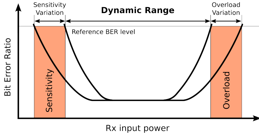
Figure 2.6: This graph illustrates how the operating dynamic range of a Rx is defined in terms of the Rx sensitivity and overload levels relative to a chosen BER threshold.
