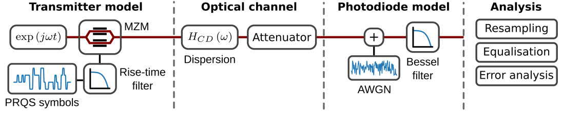
Figure 2.13: Simulation setup used for investigations into Rx bandwidth and chromatic dispersion impairments on 100 Gbit/s PAM4.
