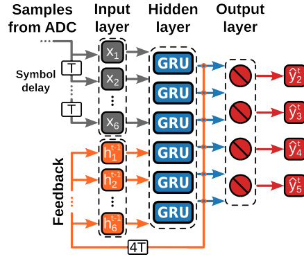
Figure 4.9: Multi-output GRU-based equaliser.
