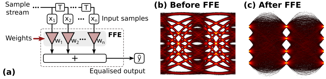
Figure 2.10: (a) The structure of an FFE; (b) shows a simulated 100 Gbit/s PAM4 eye after a 10 GHz 4 th order Bessel filter while (c) shows the same eye after equalisation using an FFE-11T.
