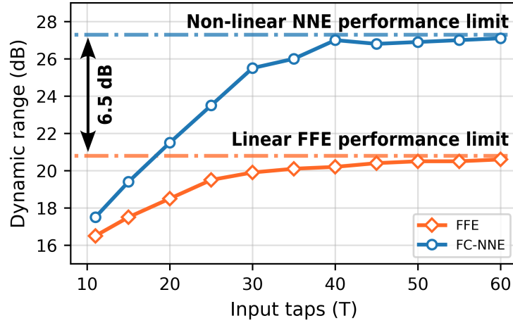
Figure 4.7: The strong dependence of BtB FC-NNE performance on the equaliser's number of input taps is shown, as well as the additional performance advantage a non-linear FC-NNE has over the linear FFE, resulting in an observed 6.5 dB dynamic range improvement.
