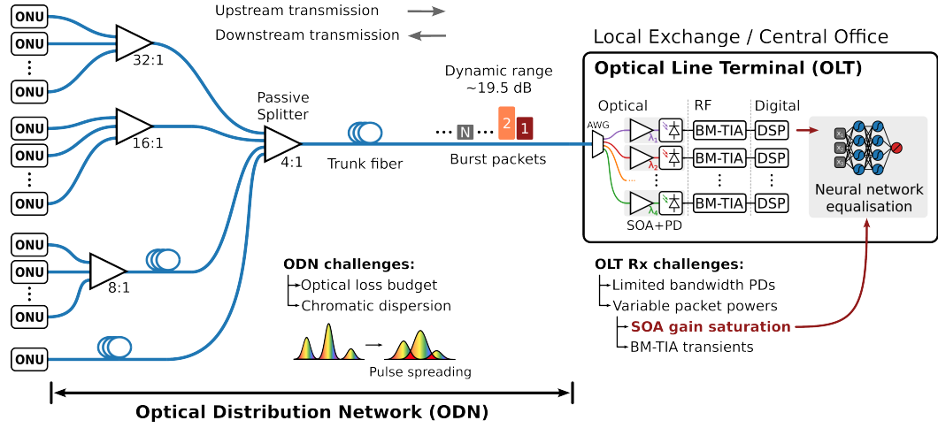
Figure 2.1: Schematic of PON system components.
