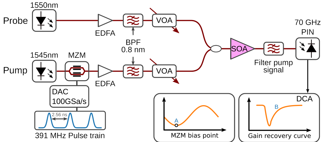
Figure 3.5: Experimental setup used to measure gain recovery time of SOA used.
