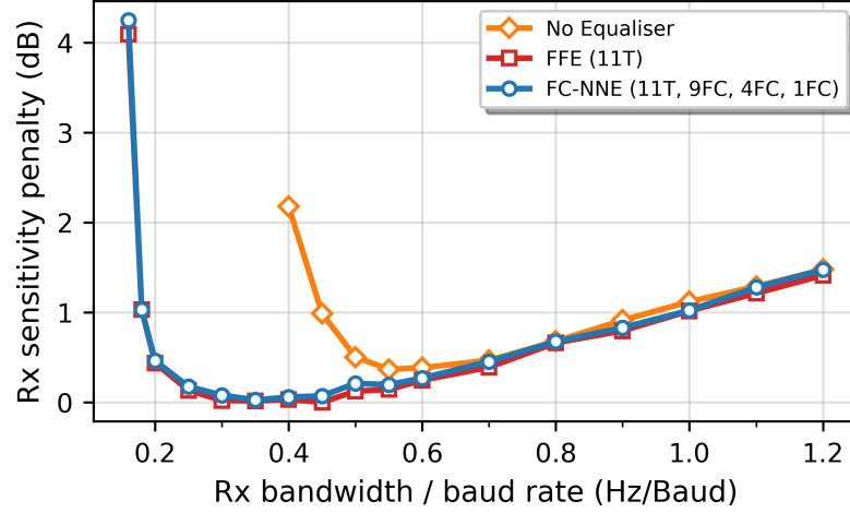
Figure 2.14: The sensitivity penalty of a bandwidth-limited receiver simulated using a 4th order digital Bessel filter.
