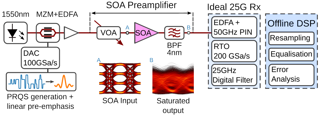
Figure 3.8: Experimental setup used to emulate multi-rate upstream PAM4 transmission.
