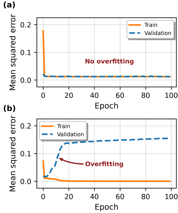
Figure 2.12: Example NNE learning curves showing (a) no overfitting, and (b) overfitting, where the model performance on the validation dataset diverges from that of the training dataset.
