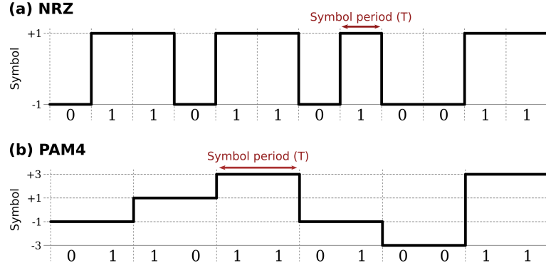
Figure 2.2: Comparison of (a) binary NRZ and (b) 4-level PAM4 modulation formats.
