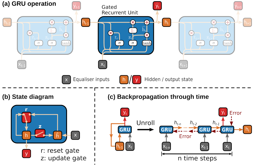
Figure 3.13: (a) Shows a schematic of a GRU neuron with a gated feedback mechanism, and (b) is the corresponding state diagram of a GRU; (c) shows the backpropagation through time algorithm for training RNNs.
