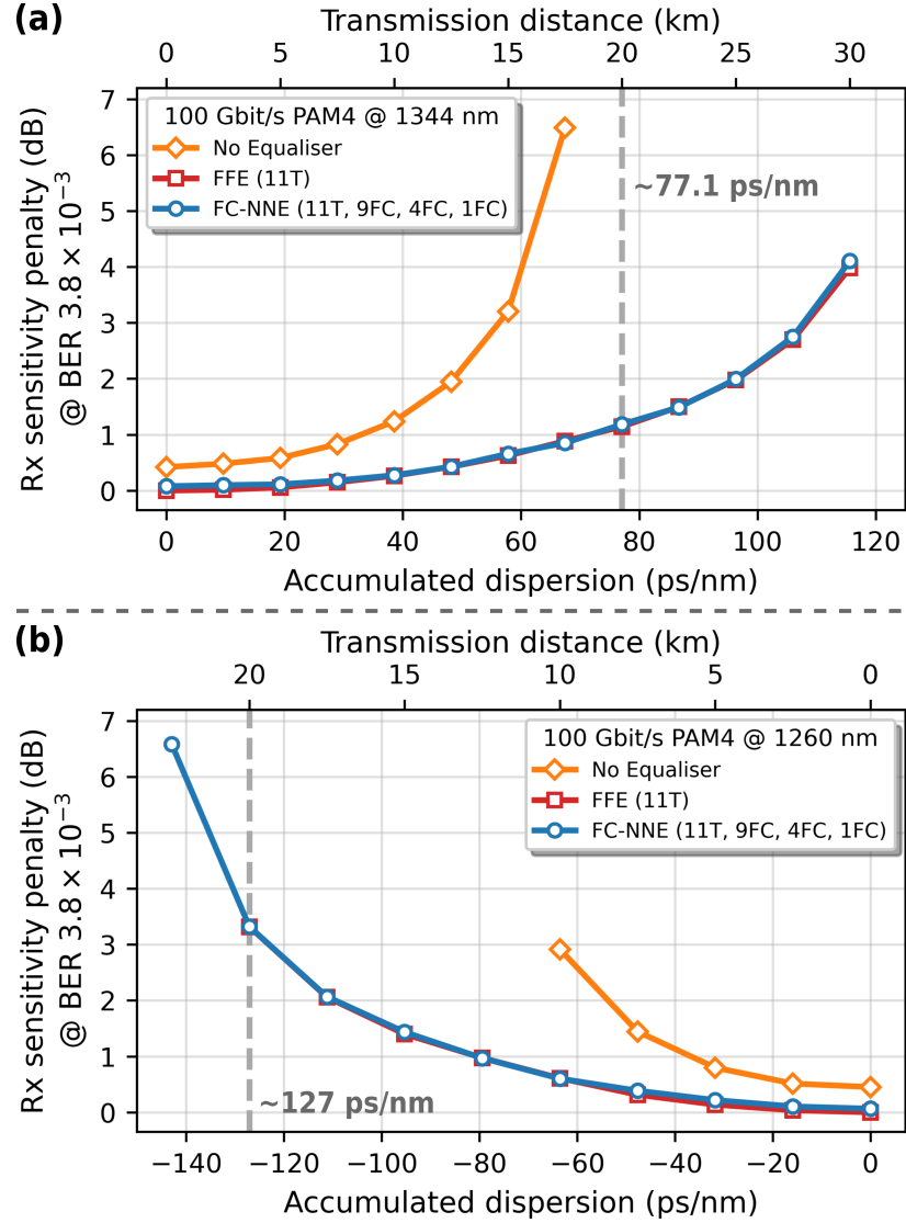
Figure 2.15: Simulated chromatic dispersion penalty at 3.8 \times 10^{-3} BER at (a) 1344 nm and (b) 1260 nm wavelengths.
