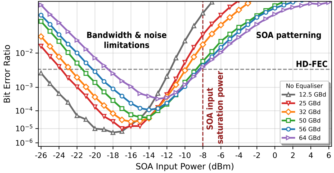
Figure 3.10: Performance of high-speed PAM4 signals for a range of SOA input powers. Clearly above -8 dBm the signals undergo saturated SOA non-linear patterning effect.
