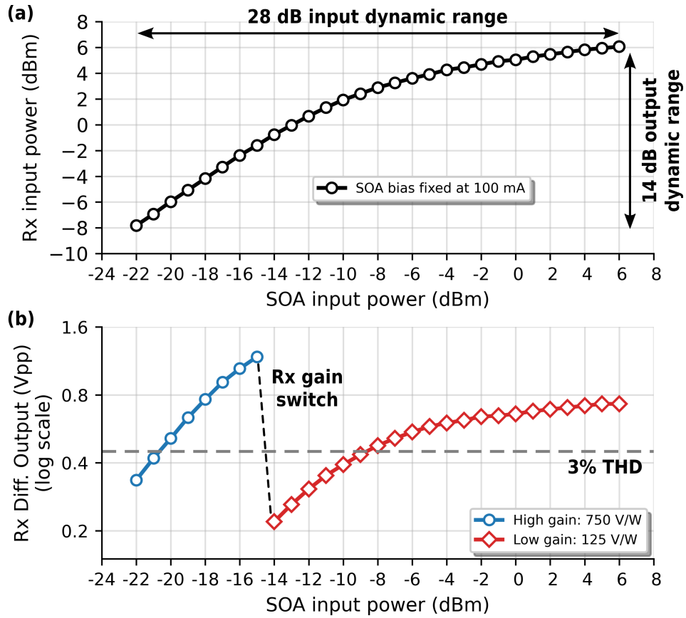
Figure 4.3: (a) The effect of SOA gain compression on input dynamic range to the SOA due to gain saturation; (b) graph showing the differential output swing from the photoreceiver amplifier with the gain-switch point indicated along with 3% Total Harmonic Distortion threshold.
