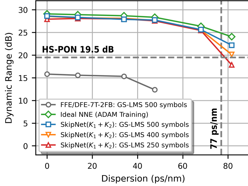
Figure 5.8: The SkipNet equaliser achieves > 25 dB DR for up to 68 ps/nm accumulated dispersion using just 250 symbols, clearly outperforming the adaptive FFE/DFE equaliser which cannot even support 19.5 dB PON DR requirement in the BtB scenario.
