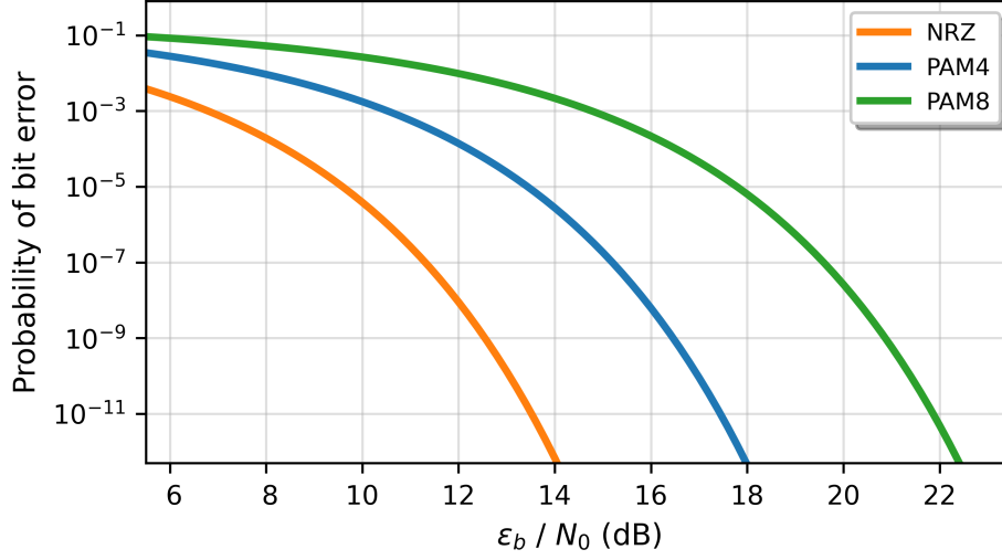
Figure 2.4: Plot of the error performances of NRZ, PAM4, and PAM8 for varying \epsilon_b/N_0 : clearly PAM4 requires more energy per bit to achieve the same error performance as NRZ.
