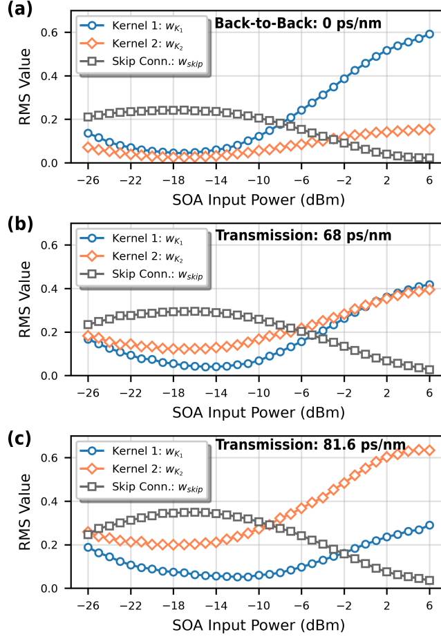
Figure 5.6: The RMS values of the converged weight parameters in the SkipNet output layer indicate kernel and skip connection relevance for (a) back-to-back (0 ps/nm), (b) 68 ps/nm, and (c) 81.6 ps/nm transmission scenarios. The LMS algorithm can clearly select between kernels and skip connections to target different packet impairments.
