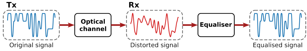
Figure 1.2: Equalisation allows distorted signals to be recovered at the Rx.
