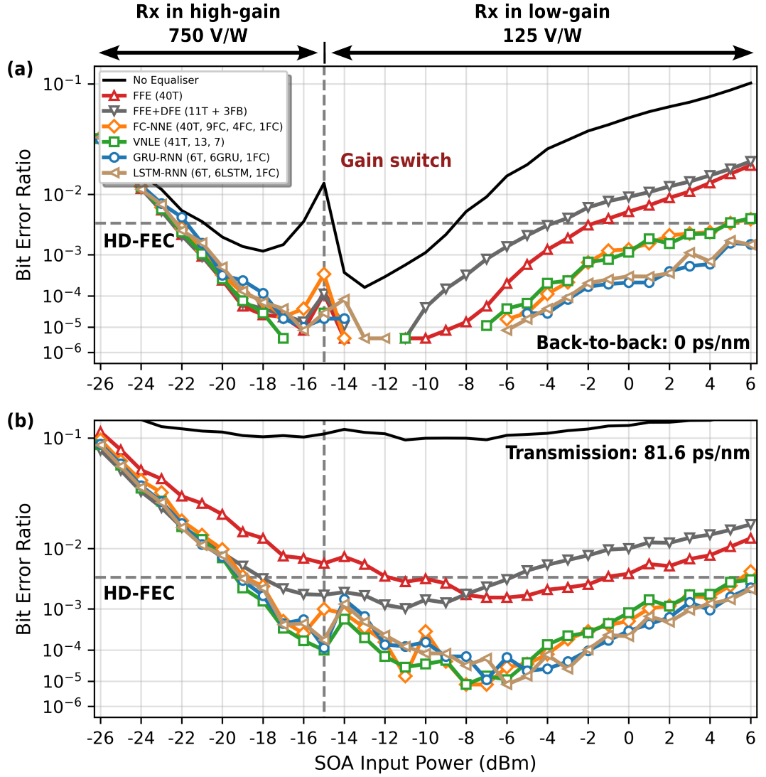
Figure 4.6: BER performance of feedforward (FFE, VNLE, FC-NNE), and feed-back (FFE/DFE, GRU-RNN, LSTM-RNN) equalisation applied to 100 Gbit/s PAM4 (a) back-to-back, and (b) transmission experiments.
