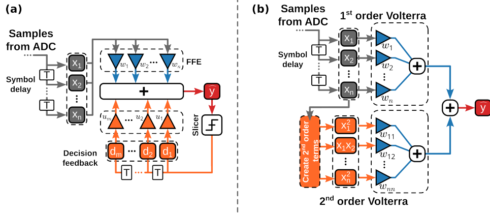
Figure 4.1: Schematics of (a) an FFE/DFE equaliser, and (b) a 2 nd -order non-linear Volterra equaliser.
