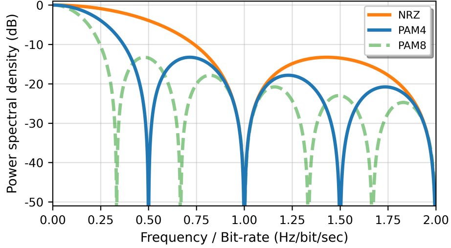
Figure 2.3: A comparison of the spectral efficiency of NRZ, PAM4, and PAM8.
