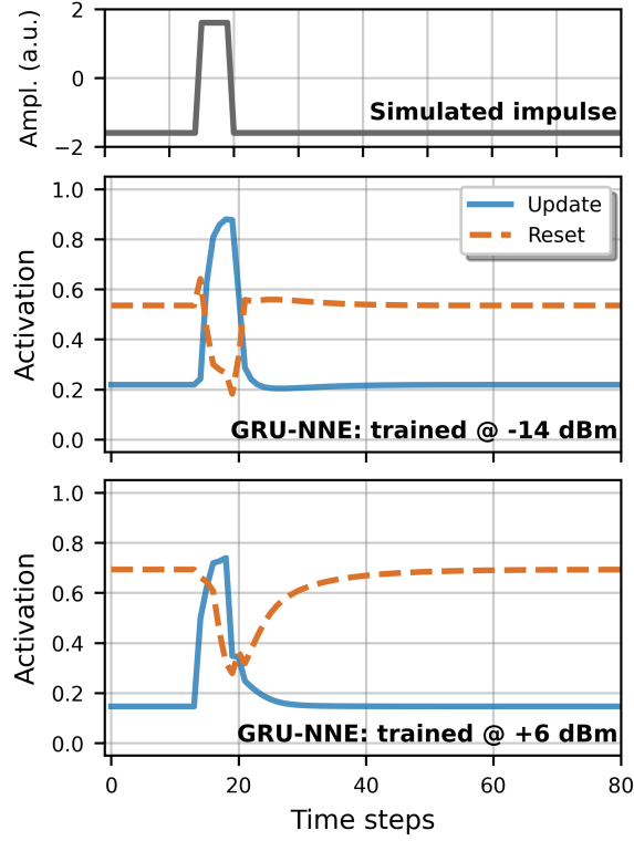
Figure 3.17: Shows the simulated pulse fed to trained GRU-NNE models on saturated and unsaturated SOA data, and the resulting output activation response of the most significant GRU neuron.
