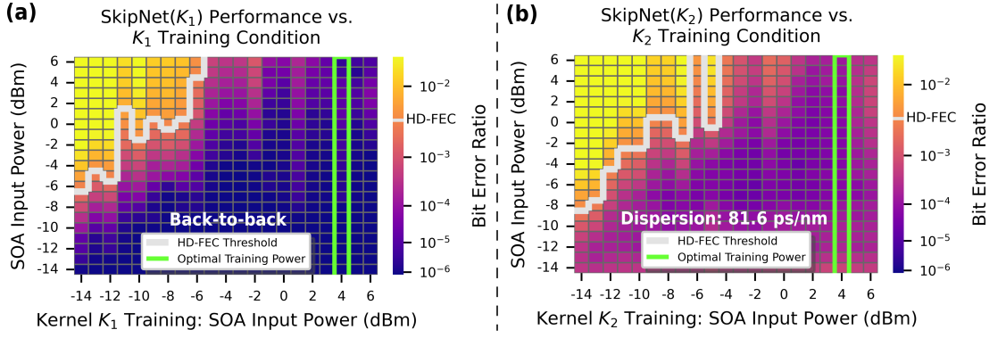
Figure 5.5: These heatmaps in (a) and (b) show how K_1 and K_2 's training conditions were chosen, by plotting kernel training power versus the BER performance of the resulting SkipNet equalisers.
