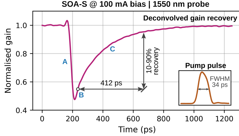
Figure 3.6: Results of pump-probe experiment to measure the SOA-S gain recovery for a constant bias of 100 mA and a 1550 nm probe wavelength
