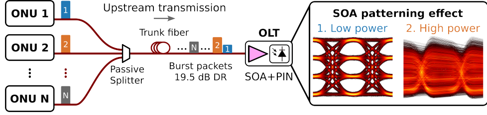
Figure 3.1: Challenges facing SOA preamplification due to burst-mode upstream transmission at the OLT.
