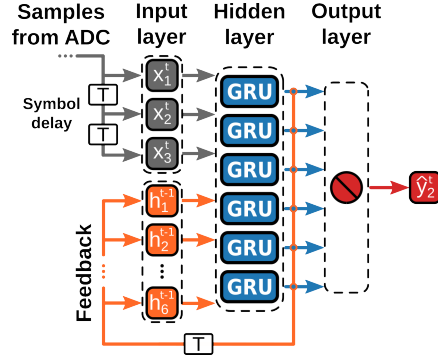
Figure 3.14: Schematic diagram of a GRU-based RNN equaliser.
