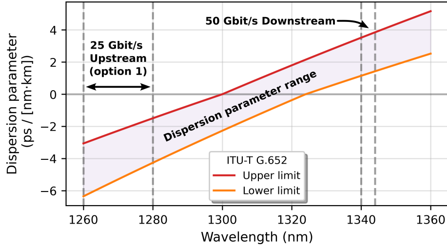
Figure 2.8: Typical dispersion profile of a commercially available fiber, generated using equation 6-1 in ITU-T G.652 [77], and parameters from Corning SMF-28+ product datasheet [78].
