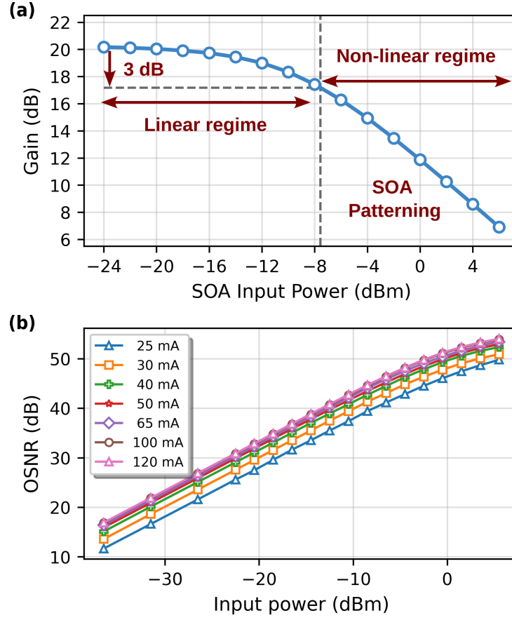
Figure 3.4: The gain curve of the CIP SOA-S at a constant bias of 100 mA is shown, with the linear and non-linear operating regimes delineated by the 3-dB gain saturation point.
