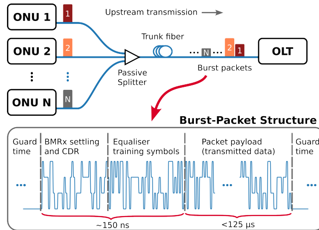
Figure 5.1: The burst-packet structure of upstream PON transmission according to the latest 50 Gbit/s HS-PON standards is shown. Only 150 ns preamble allocated for 25 Gbit/s upstream transmission, and 610 ns in a worst case scenario [12].
