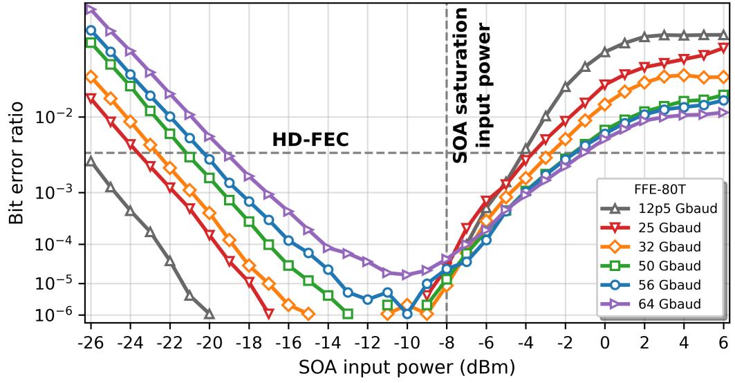
Figure 3.11: Transmission performance of various baud rate PAM4 signals using an SOA+PIN Rx configuration, and FFE-80T post-equalisation.
