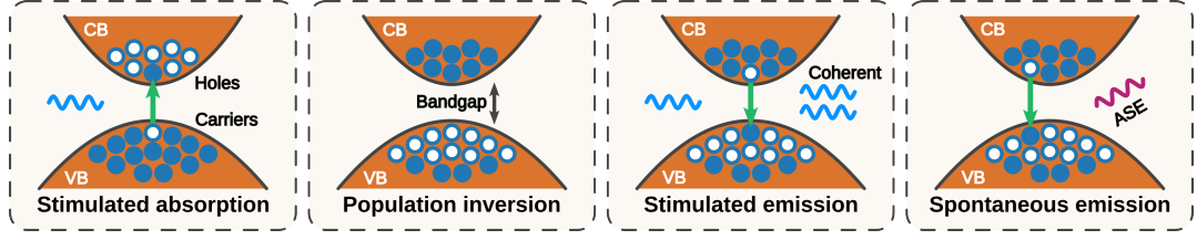
Figure 3.2: SOA structure, bandgap and optical amplification mechanism.
