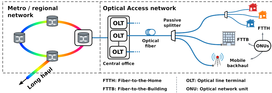
Figure 1.1: Optical access networks connect end users to the wider internet infrastructure using fiber optic cabling.
