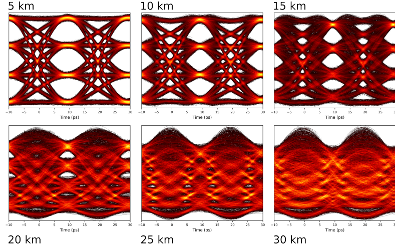
Figure 2.9: Eye diagrams show the effect of dispersion on a simulated 100 Gbit/s PAM4 signal at 1344 nm and using D and S parameters taken from Fig. 2.8.
