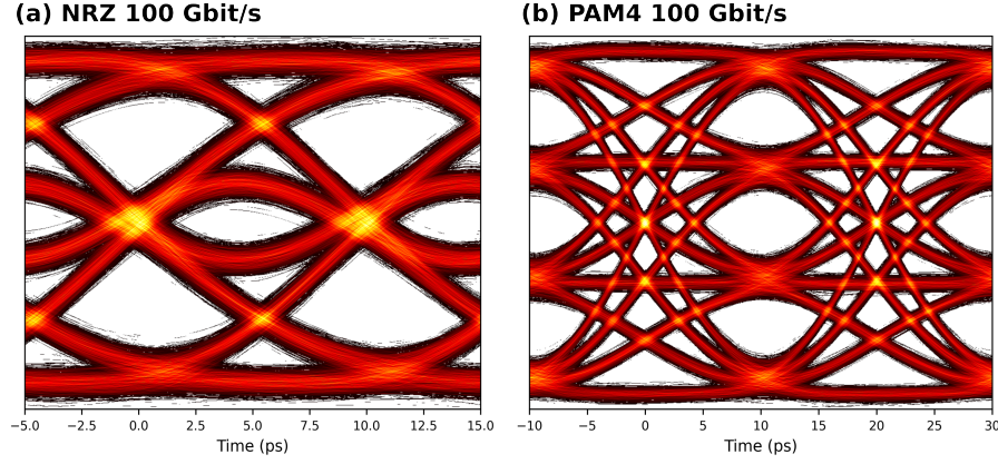
Figure 2.7: Simulated 100 Gbit/s (a) NRZ and (b) PAM4 eyes resulting from a bandwidth-limited 25 GHz Rx, implemented using a 4 th order Bessel filter.
