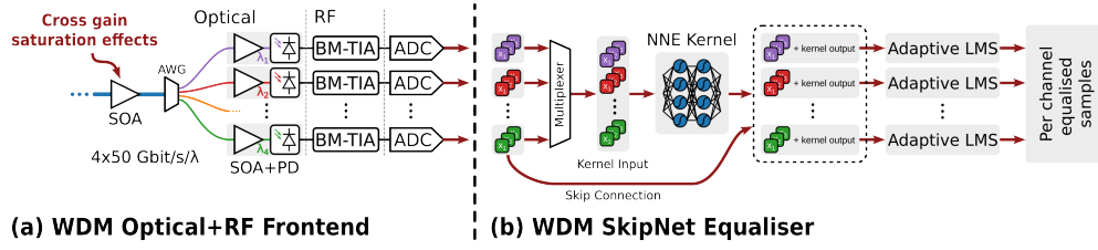
Figure 6.1: (a) Possible 400 Gbit/s PAM4 WDM PON scenario, with (b) adaptive SkipNet equaliser to mitigate SOA cross-channel patterning effects.
