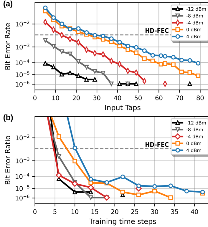
Figure 3.16: The performance dependence of (a) an FC-NNE on tap numbers is compared with that of a (b) GRU-NNE's performance dependence on training time steps, for varying SOA input powers.
