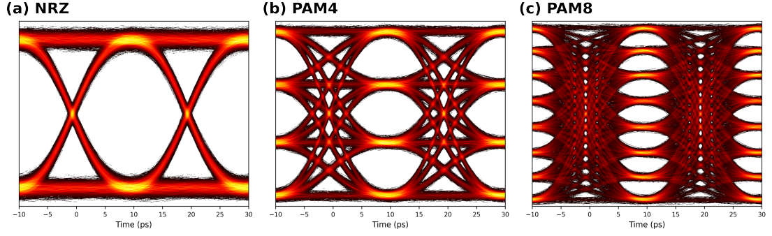
Figure 2.5: Example eye diagrams of (a) NRZ, (b) PAM4, and (c) PAM8.
