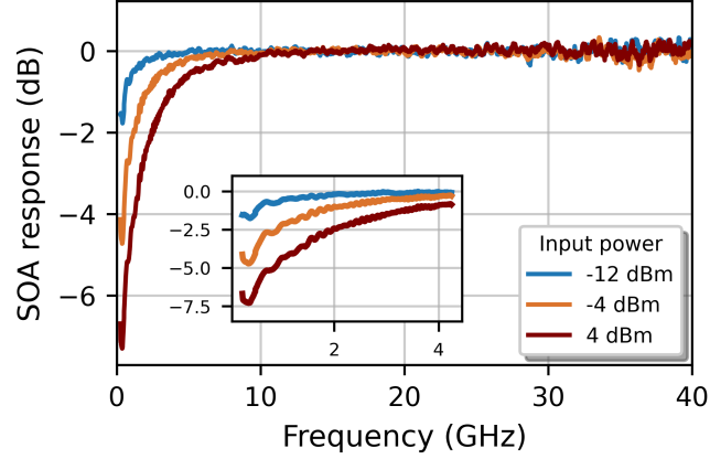
Figure 3.7: Frequency response of SOA for different input powers.
