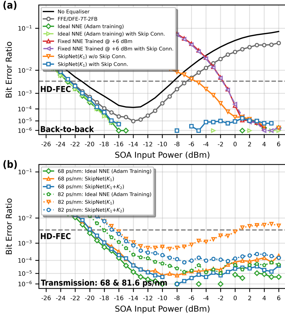
Figure 5.4: (a) Shows the BtB performance of the SkipNet( K_1 ) equaliser with and without skip connections, versus ideally trained and fixed (non-adaptive) NNEs. In (b), the transmission performance of single ( K_1 ) and double ( K_1 + K_2 ) kernel SkipNet equalisers underlines the flexibility of the scheme to accommodate additional low-complexity kernels for greater non-linear capability.
