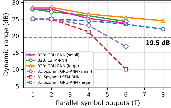
Figure 4.10: Graph showing GRU-RNN high dynamic range performance can be sustained when implementing multi-symbol output technique, at the cost of larger network size.
