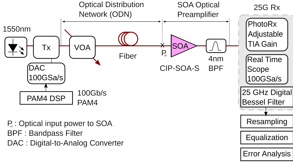
Figure 4.4: Experimental setup emulating 100 Gbit/s upstream PON transmission, using SOA gain saturation and neural network equalisation to enable > 28 dB dynamic range using only two electrical gain settings in the photoreceiver.
