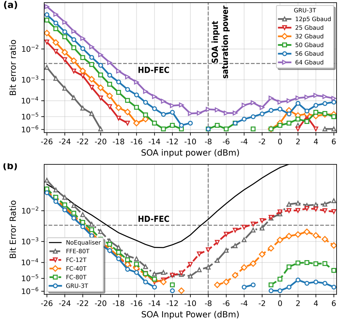
Figure 3.15: BER results for (a) GRU-NNE (3T) at different baud-rates, and (b) a comparison of results for GRU-, FC-NNE, and FFE equalisers for 100 Gbit/s PAM4.
