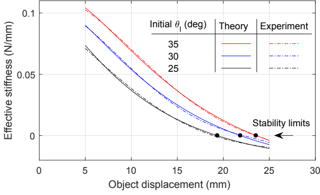
Fig. 7. Effective grasp stiffness dW_0/dX_a : Theory and experiment.
