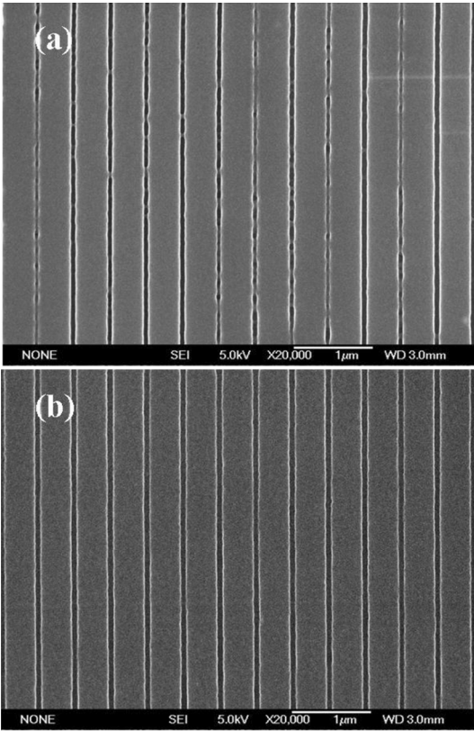
Figure 2. Scanning electron microscopy (SEM) images of semi-dense line arrays in PMMA resist with a 50 nm linewidth. The arrays are exposed with dose of (a) 180\text{ }\mu\text{C}/\text{cm}^2 and (b) 750\text{ }\mu\text{C}/\text{cm}^2 and developed with (a) a IPA:MIBK 3:1 mixture for 30 s and (b) IPA for 5 s.
