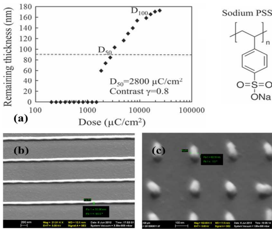
Figure 24. (a) Contrast curve of the water-soluble PSS resist, (b) SEM image showing a line array with a line width ~60 nm (narrower lines were found to have collapsed). (c) SEM images showing arrays of pillars with a mean diameter of 60 nm. 72
