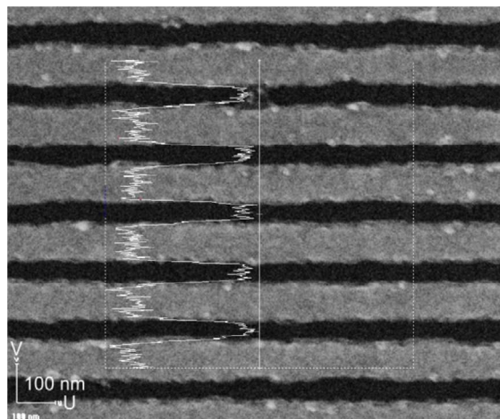
Figure 8. Line and space pattern: 90 nm wide gold lines on a SiO 2 substrate spaced 70 nm apart (80 nm half-pitch), structured with the after lift-off process with 40XT/PEDOT-PSS. The sample was developed for 60 s in a developer diluted with 40 % vol. DI water. 35
