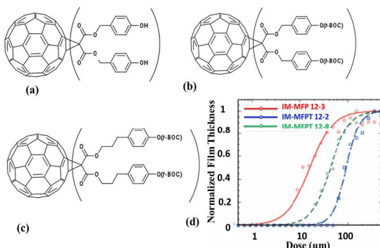
Figure 13. Chemical structures of (a) (3-phenol-1-propyl malonate)-methano-[60] fullerene, (b) (t-butoxycarbonyl malonate)-methano-[60] fullerene and (c) [3-(4-butoxycarbonyl) phenyl-1-propyl malonate]-methano-[60] fullerene and (d) contrast curves for the three resist derivatives. 49
