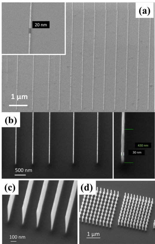
Figure 23: (a) Examples of lithography results achieved with optimized EBL parameters (3 keV acceleration voltage, 200–250 \mu\text{C cm}^{-2} exposure dose, 2 min at 120 ^{\circ}\text{C} PEB (b) Images of the same sample, with lines of 30 and 20 nm etched down to a depth of more than 400 nm; (c) and (d) images of the same sample, with 20 nm lines and 50 nm diameter pillars etched down to 350 nm. 69
