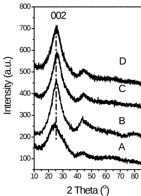
Figure 6 XRD patterns of carbon cages prepared on Co/Mo/MgO at (A) 650 °C, (B) 700 °C, (C) 750 °C and 10.34 MPa, respectively. (D) Carbons are prepared at 700 °C and 24.12 MPa.
