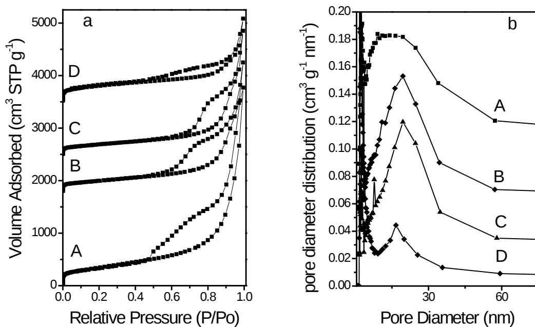
Figure 4 (a) N 2 sorption isotherms and (b) the corresponding pore-size distributions of CNCs prepared by sc-CO 2 on Co/Mo/MgO at (A) 650 °C, (B) 700 °C, (C) 750 °C and 10.34 MPa, (D) 700 °C and 24.12 MPa. The isotherms in figure 4a for B, C and D samples are offset vertically by 1800, 2500 and 3500 cm 3 STP g -1 .
