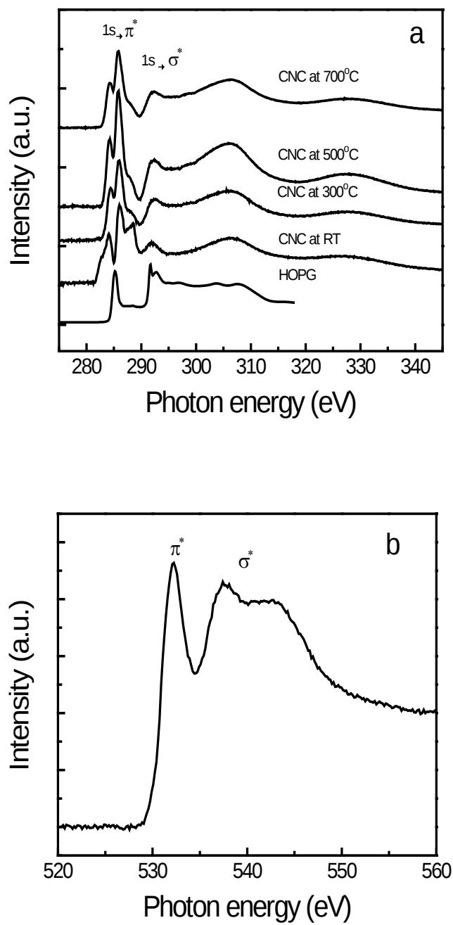
Figure 2 (a) Carbon K-edge NEXAFS spectra of HOPG and carbon nanocages as a function of annealing temperature, (b) Normalized NEXAFS spectra at the oxygen K-edge of a CNC sample.
