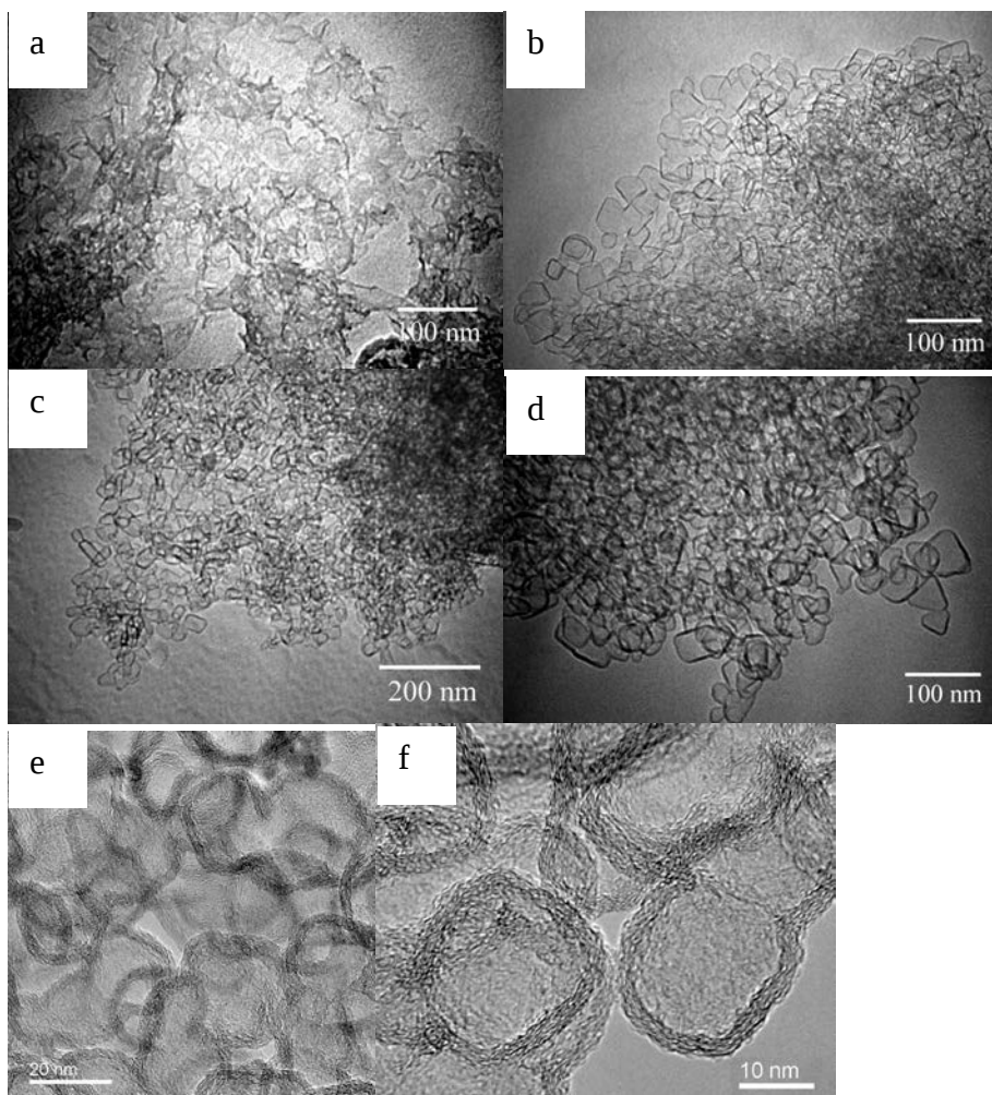
Figure 1 TEM images of carbon products prepared using sc-CO 2 on Co/Mo/MgO at (a) 600 °C, (b) 650 °C, (c) 700 °C, and (d) 750 °C. (e, f) HRTEM images of sample (c) reveal curved carbon layers. Molar ratio: p-xylene/CO 2 =0.4%, P CO 2 =10.34 MPa.
