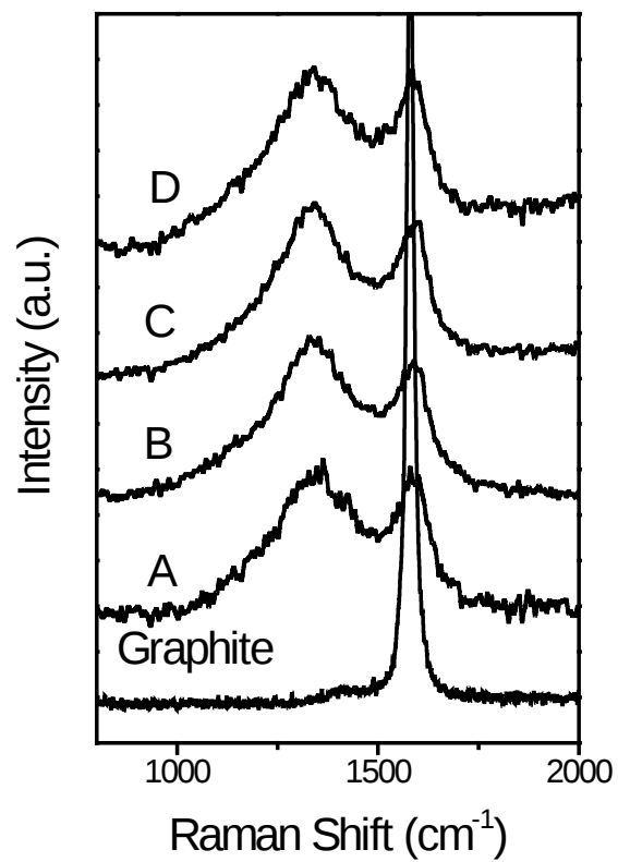
Figure 5 Raman spectra of graphite and carbon products over Co/Mo/MgO catalyst after decomposition of p-xylene at (A) 650 °C, (B) 700 °C, (C) 750 °C and 10.34 MPa, (D) 700 °C and 24.12 MPa.
