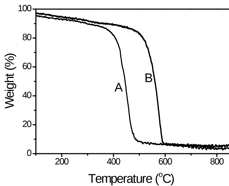
Figure 7 TG profiles of the synthesized CNCs on Co/Mo/MgO. (A) 650 °C, (B) 750 °C and 10.34 MPa.
