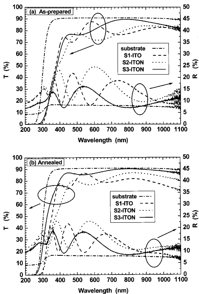
FIG. 7. UV-vis transmittance and reflectance of ITO and ITON films (a) just after deposition and (b) after annealing at 400 °C for 1 min. S1-ITO: 100%Ar plasma; S2-ITON: 50%Ar–50%N 2 plasma; S3-ITON: 100%N 2 plasma.
