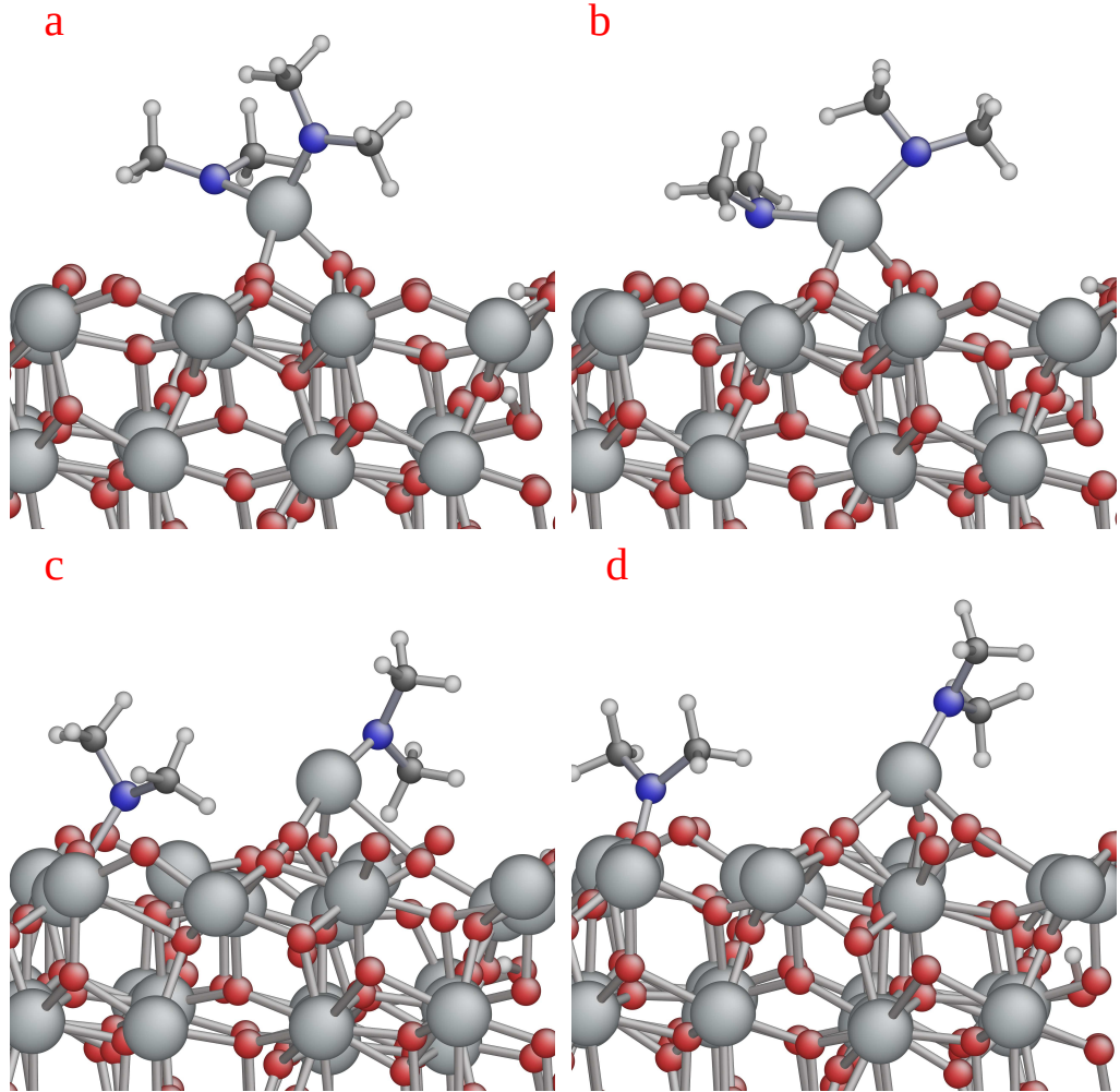
Figure 3.9: The amide group of the densified \text{HfX}_2 was transferred to under-coordinated hafnium at the surface; snapshots are from ab initio MD calculation, starting at T = 500 K and running for 0.4 ps.
