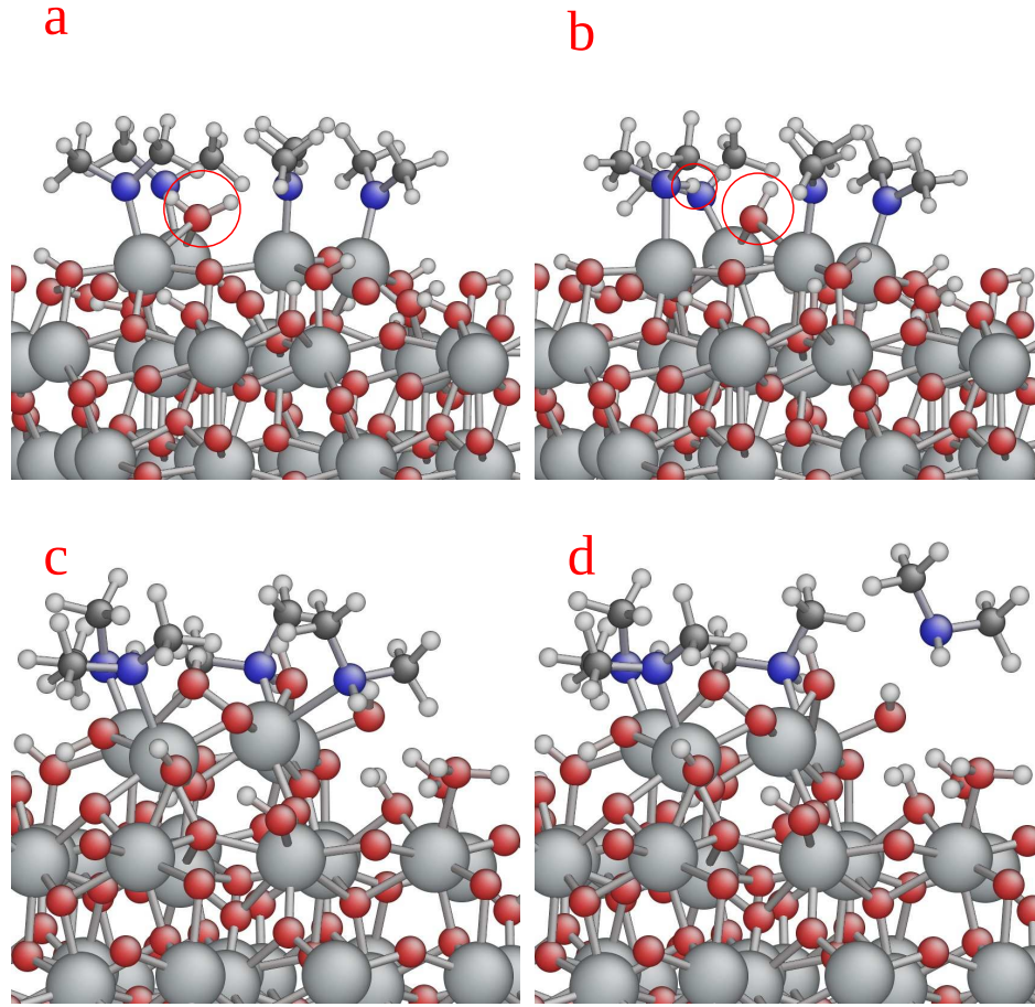
Figure 4.6: The incoming \text{H}_2\text{O} molecule is readily dissociated in the cluster of remaining precursor (here 4 \text{HfX} ). Due to multiple adsorptions of \text{H}_2\text{O} molecules, dissociation of the remaining ligands becomes energetically possible (Fig. 4.2). (a) Cluster of 4 \text{HfX} . Circle shows an incoming \text{H}_2\text{O} molecule. (b) The incoming \text{H}_2\text{O} molecule is barrierlessly dissociated. (c) Multiple adsorptions of \text{H}_2\text{O} molecules into the cluster. (d) Desorption of the remaining ligands is facilitated through multiple adsorptions of \text{H}_2\text{O} molecules.
