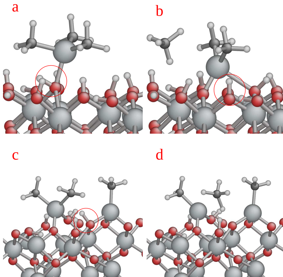
Figure 4.3: Through multiple adsorptions of AlX_3 , the surface oxygen becomes coordinatively saturated (Fig. 4.1). The rate of proton diffusion from the saturated oxygen increases and causes the desorption of HX and bonding of the metal of the precursor to the another surface oxygen. (a) Adsorption of AlX_3 . Circle shows the OH group to which AlX_3 is anchored. (b) Desorption of HX due to proton transfer from the anchor OH group. Circle shows a low coordinated OH group. (c) Co-existence of remaining precursors, resulting in coordinative saturation of the OH group (circle). (d) Desorption of second HX due to proton diffusion from coordinatively saturated OH group. (red = O, white = H, large gray = Al, small gray = C).
