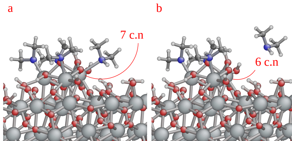
Figure 3.12: Dissociation of HX from seven coordinated hafnium during water pulse. Four oxygen (originally adsorbed as \text{H}_2\text{O} ) are coordinated to the cluster and dissociation of HX from the resulting 7-coordinate Hf is more favourable than the situation in Fig. 3.11.
