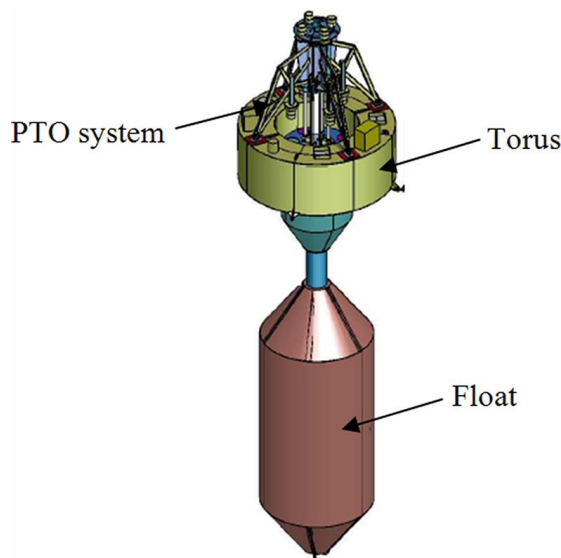
Fig. 1.1: Wavebob two-body heaving WEC [18].
