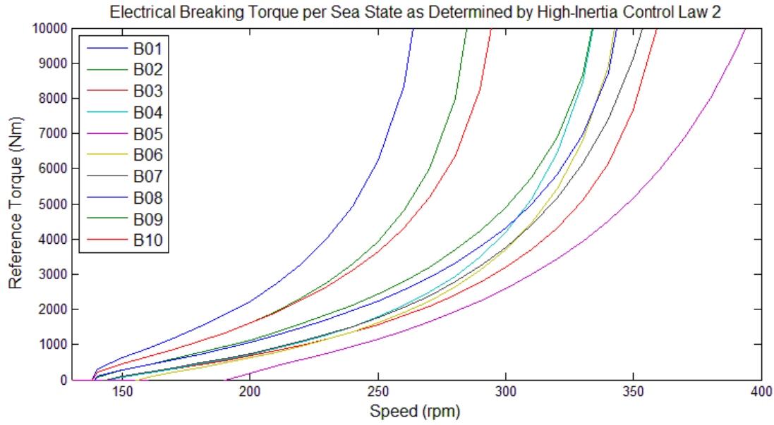
Fig. 5.7: Various torque-speed curves as determined using the high inertia control law equations.
