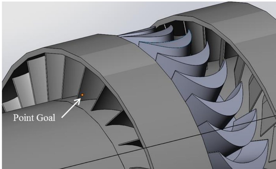
Fig. 4.8: Point goal selection for calculating air flow velocity, the orange point designates the location at which the calculations were performed.
