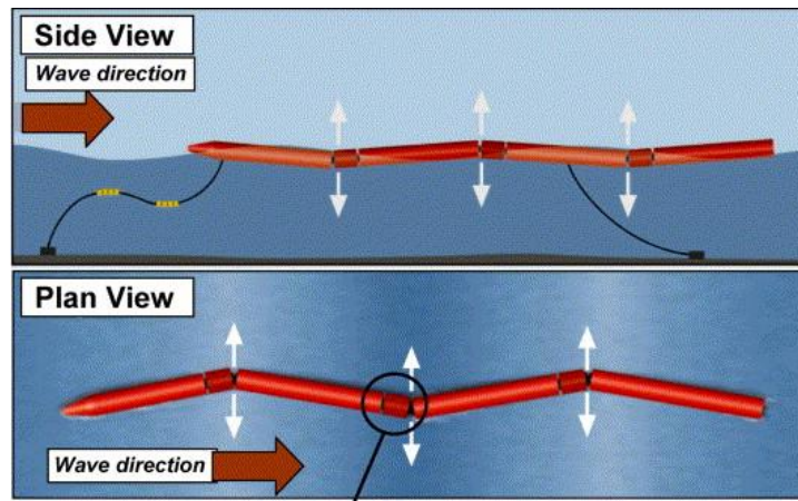
Fig. 1.4: Pelamis pitching WEC showing the two degrees of freedom between each cylinder [24].
