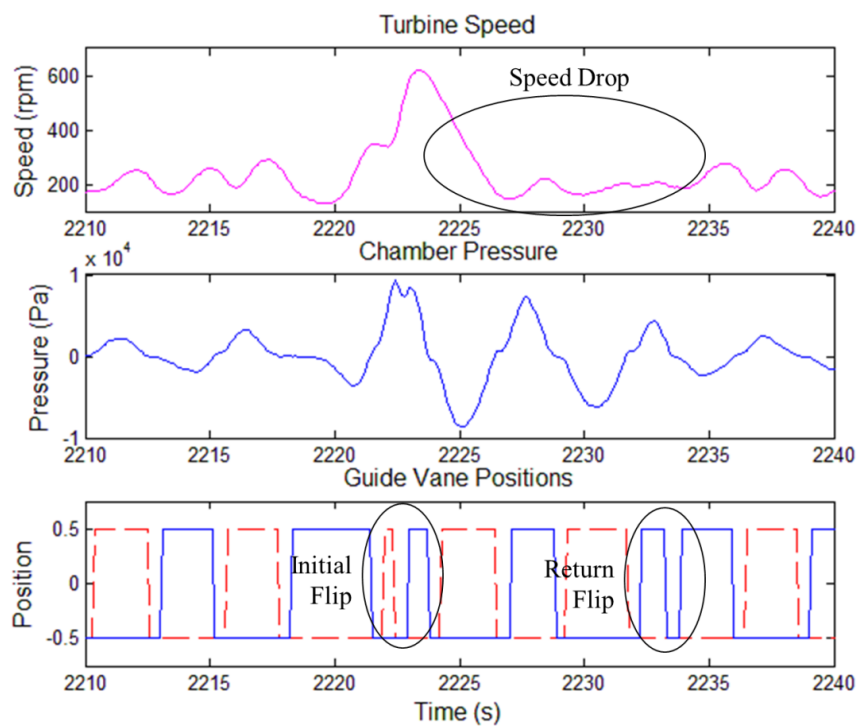
Fig. 3.19: Guide vane position relative to the plenum chamber pressure and the effect the guide vane position has on the rotational velocity of the turbine.
