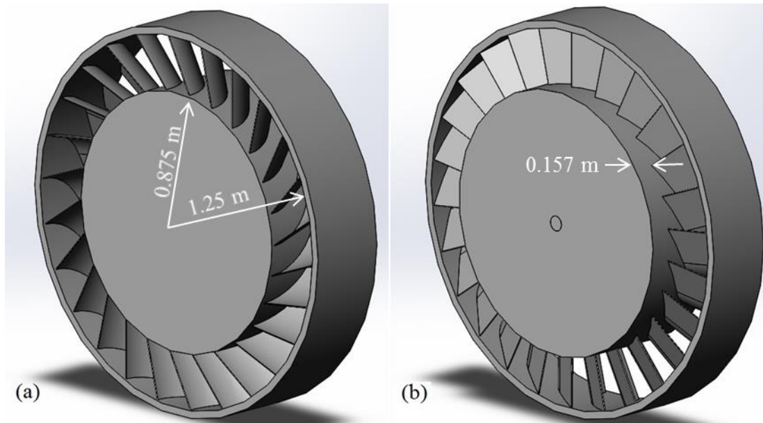
Fig. 4.5: (a) upstream and (b) downstream guide vanes for the 2.5 m diameter impulse turbine drafted using SolidWorks.
