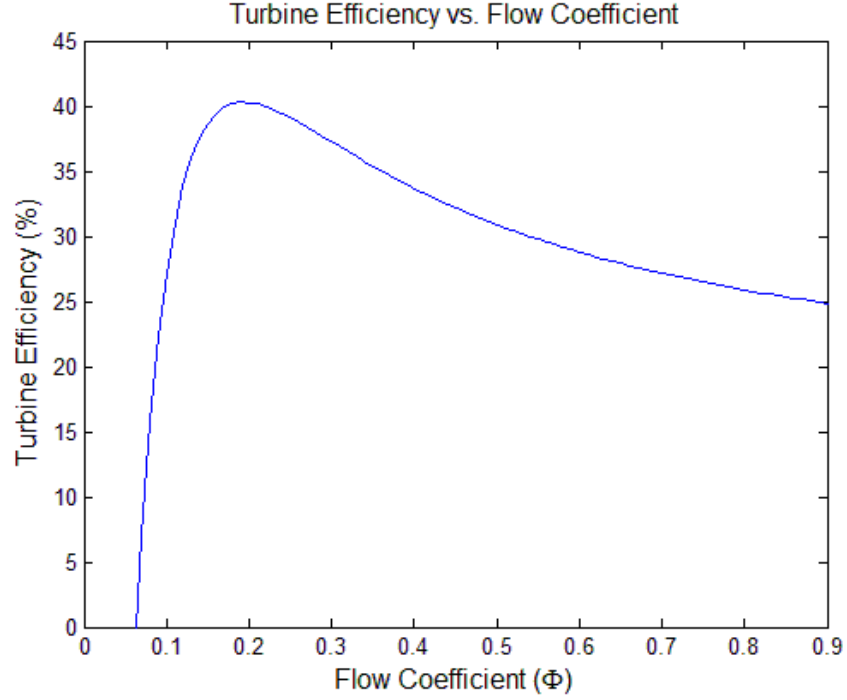
Fig. 5.3: Turbine efficiency vs. flow coefficient for the 2.5 m impulse turbine.
