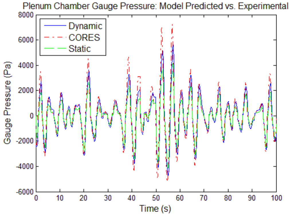
Fig. 3.8: Experimental, dynamically damped model, and statically damped model data for the plenum chamber pressure for the data set where H_s=1.09 m and T_z=3.57 s.
