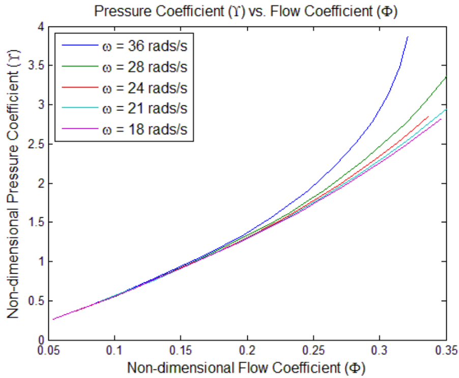
Fig. 4.20: Non-dimensional pressure vs. flow coefficient for 2.5 m impulse turbine based on the results of CFD simulations.
