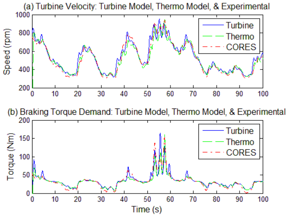
Fig. 3.13: Turbine model, thermodynamic model, and experimental data for the turbine rotational speed (a) and braking torque demand (b) for the data set where H_s=1.09 m and T_z=3.57 s.
