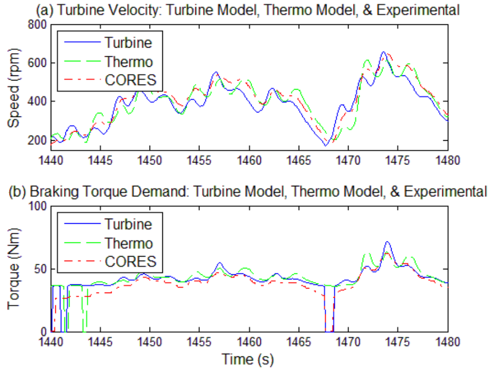
Fig. 3.11: Turbine model, thermodynamic model, and experimental data for the turbine rotational speed (a) and braking torque demand (b) for the data set where H_s=1.22 m and T_z=3.96 s.
