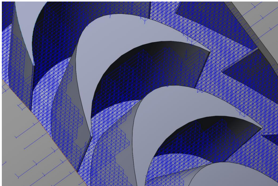
Fig. 4.9: Fluid mesh generated by Flow Simulation to calculate the flow across the turbine.
