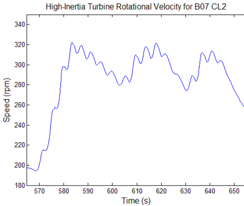
Fig. 5.17: Turbine rotational velocity from of the OWC model simulated with the high inertia turbine controlled using Control Law 2 and conditions created to match sea state B07.
