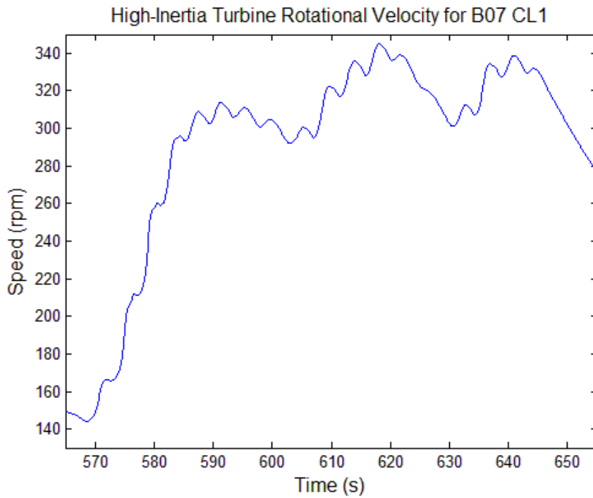
Fig. 5.13: Turbine rotational velocity from of the OWC model simulated with the high-inertia turbine controlled using Control Law 1 and conditions created to match sea state B07.
