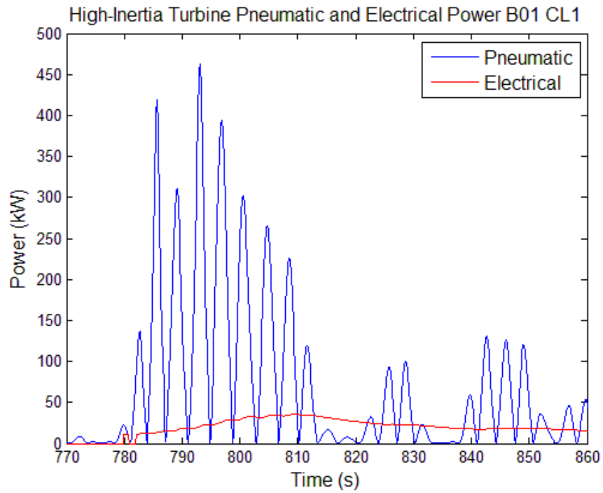
Fig. 5.14: Pneumatic and electrical power output of the OWC model with the high inertia turbine controlled using Control Law 1 as simulated and conditions created to match sea state B01.
