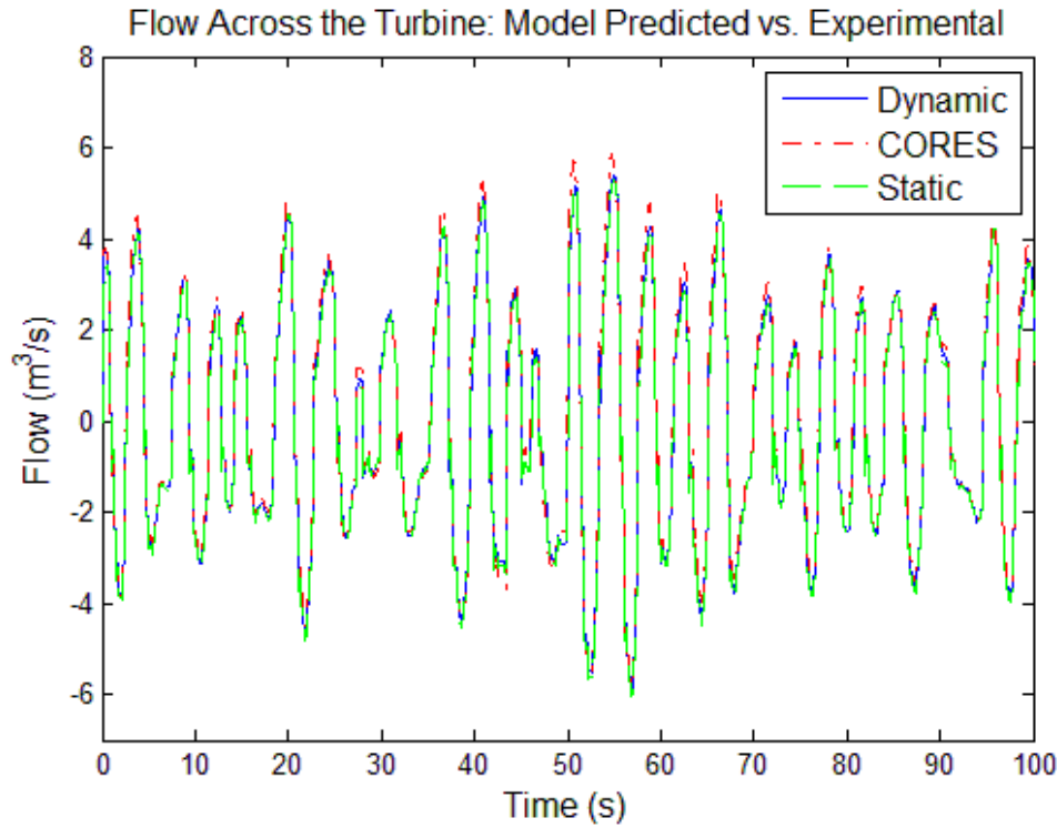
Fig. 3.9: Experimental, dynamically damped model, and statically damped model data for flow across the turbine for the data set where H_s=1.09 m and T_z=3.57 s.
