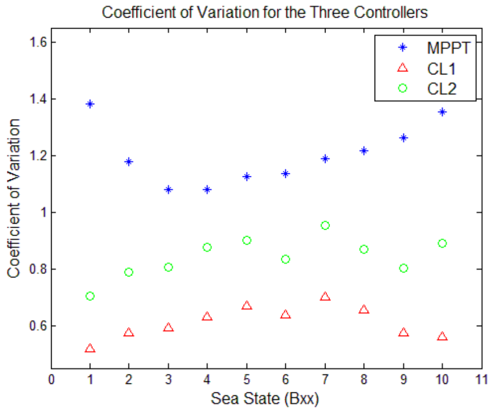
Fig. 5.22: Coefficient of Variation for the three controllers for each of the ten sea states tested during modelling.
