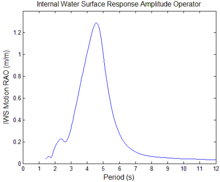
Fig. 2.2: Internal Water Surface Response Amplitude Operator of CORES buoy.
