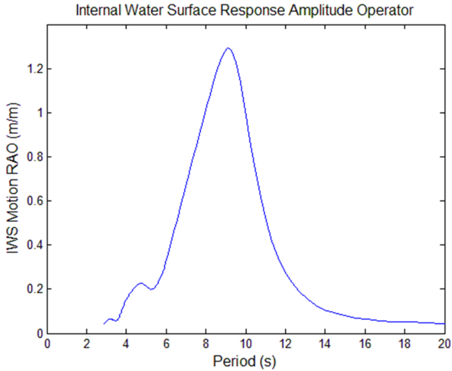
Fig. 4.2: RAO for the IWS of the OWC designed for the M1 site, derived from WAMIT [84].
