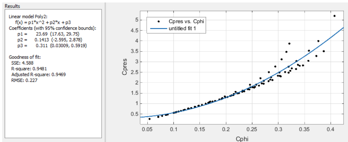
Fig. 4.21: MATLAB curve fitting application for the non-dimensional pressure drop across the turbine at a rotational velocity of 24 \text{ rads} \cdot \text{s}^{-1} .
