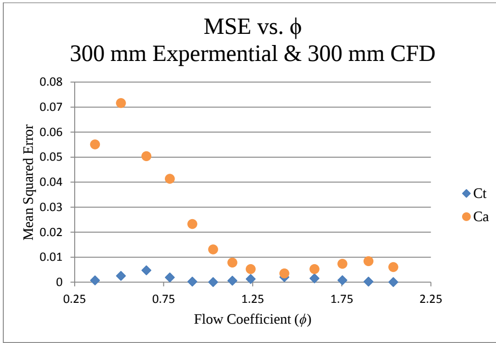
Fig. 4.14: Mean Squared Error vs \phi for 300 mm experimental results and 300 mm CFD generated results of C_t and C_a .
