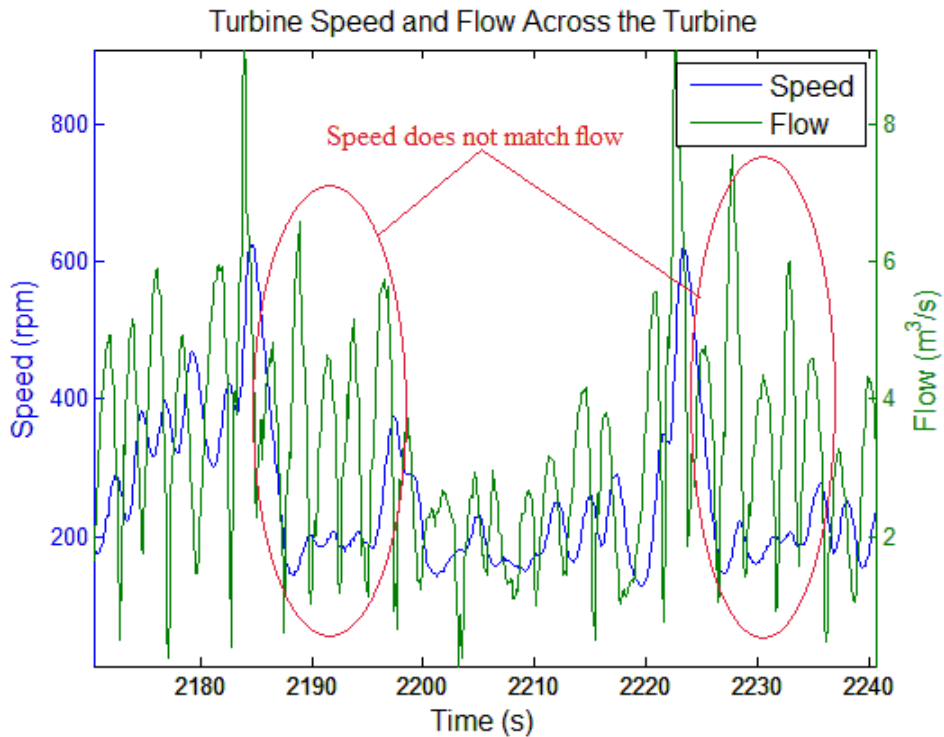
Fig. 3.17: Rotational velocity and flow across the turbine from the same data set as shown in Fig. 3.16. The red circles indicate areas where the turbine velocity did not increase despite the pressure of measured flow high enough to drive the turbine.
