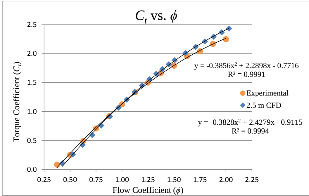
Fig. 4.15: C_t vs \phi , experimental results for 300 mm turbine [41, 102] against CFD results for 2.5 m turbine at 24 \text{ rad}\cdot\text{s}^{-1} .
