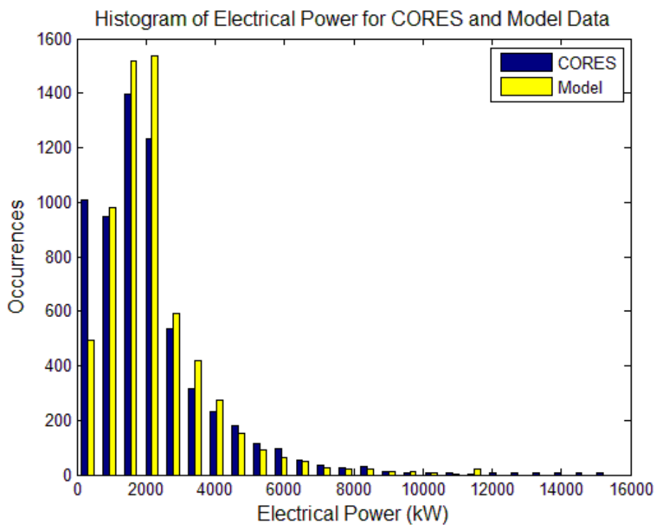
Fig. 3.7: Histogram of the electrical power output from the experimental and model data sets
