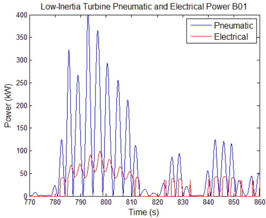
Fig. 5.10: Pneumatic and electrical power output of the OWC model simulated with conditions created to match sea state B01.
