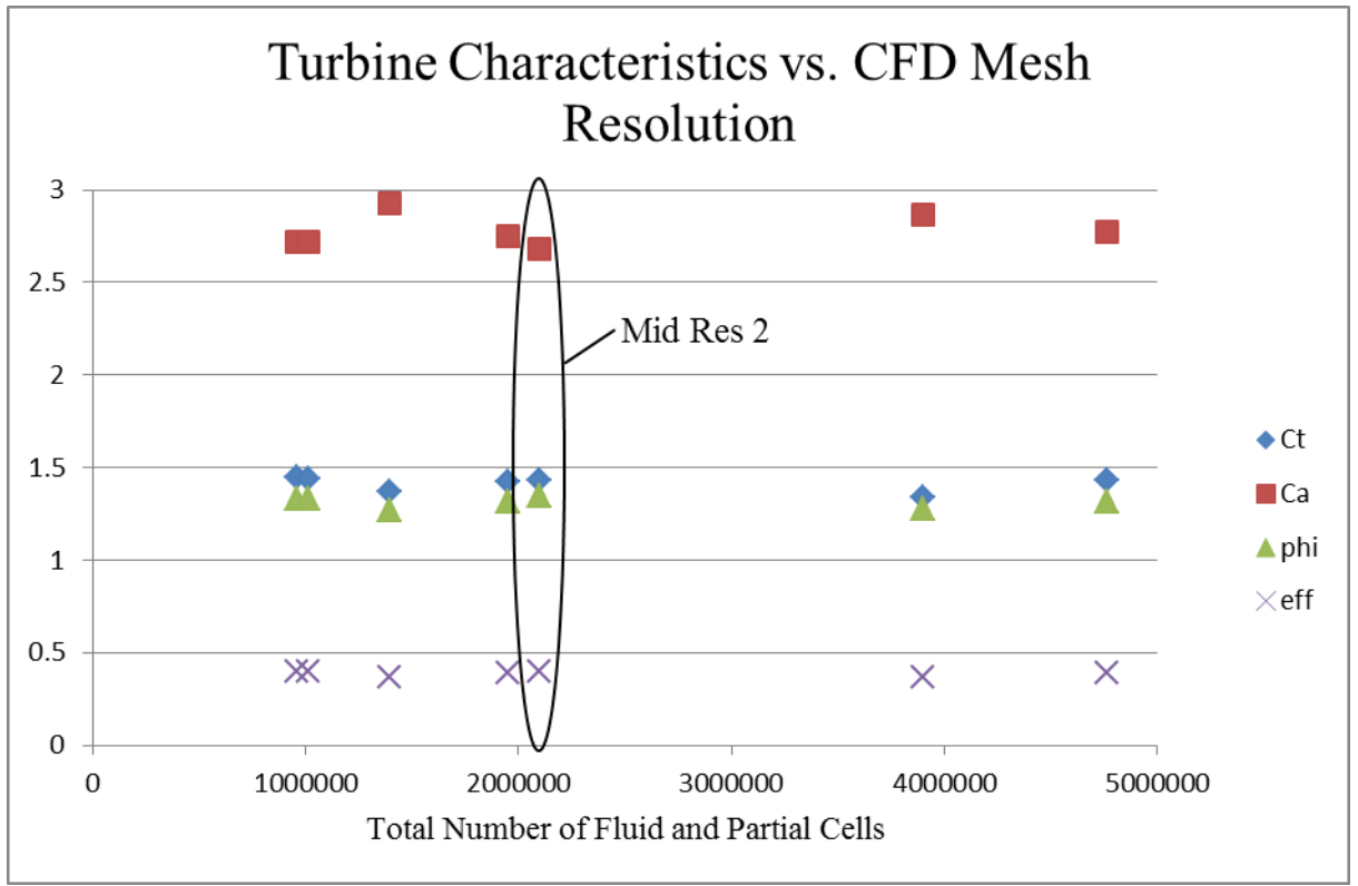
Fig. 4.11: Turbine characteristics determined by CFD simulations against mesh resolution.
