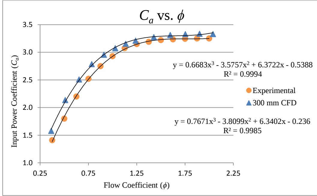
Fig. 4.13: C_a vs \phi , experimental results for 300mm turbine [41, 102] against CFD results for 300 mm turbine at 36 \text{ rads} \cdot \text{s}^{-1} .
