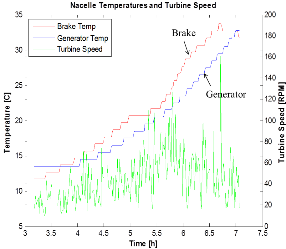
Fig. 3.18: Brake housing and generator stator temperatures and turbine rotational velocity during brake failure of the CORES OWC deployment.
