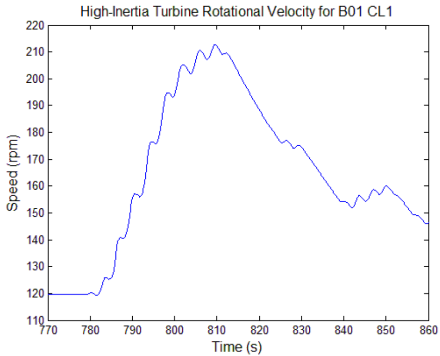
Fig. 5.15: Turbine rotational velocity from of the OWC model simulated with the high inertia turbine controlled using Control Law 1 and conditions created to match sea state B01.
