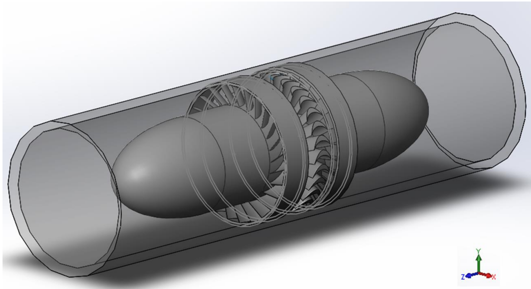
Fig. 4.6: Full turbine within duct as created for CFD simulations.
