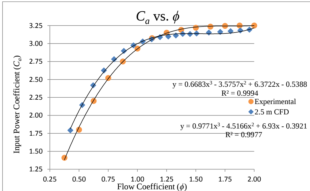
Fig. 4.16: C_a vs \phi , experimental results for 300mm turbine [41, 102] against CFD results for 2.5 m turbine at 24 \text{rads}\cdot\text{s}^{-1} .
