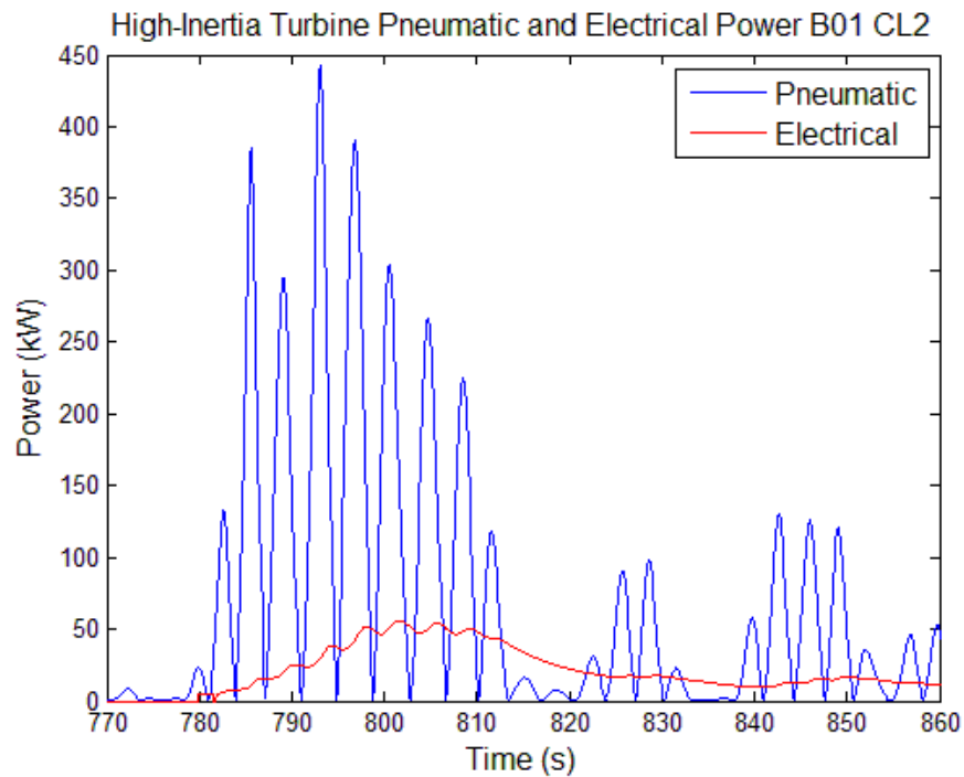
Fig. 5.18: Pneumatic and electrical power output of the OWC model with the high inertia turbine controlled using Control Law 2 as simulated and conditions created to match sea state B01.
