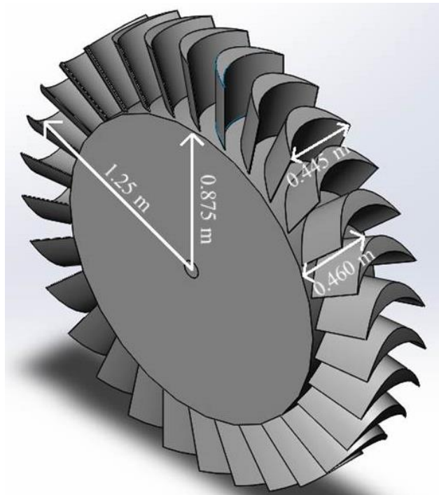
Fig. 4.4: 2.5 m diameter impulse turbine hub and blades drafted using SolidWorks.
