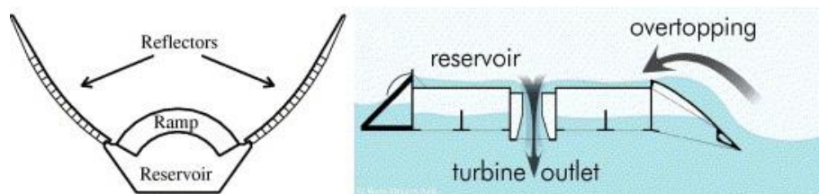
Fig. 1.6: Wave Dragon overtopping WEC plan and cross-sectional views [29].
