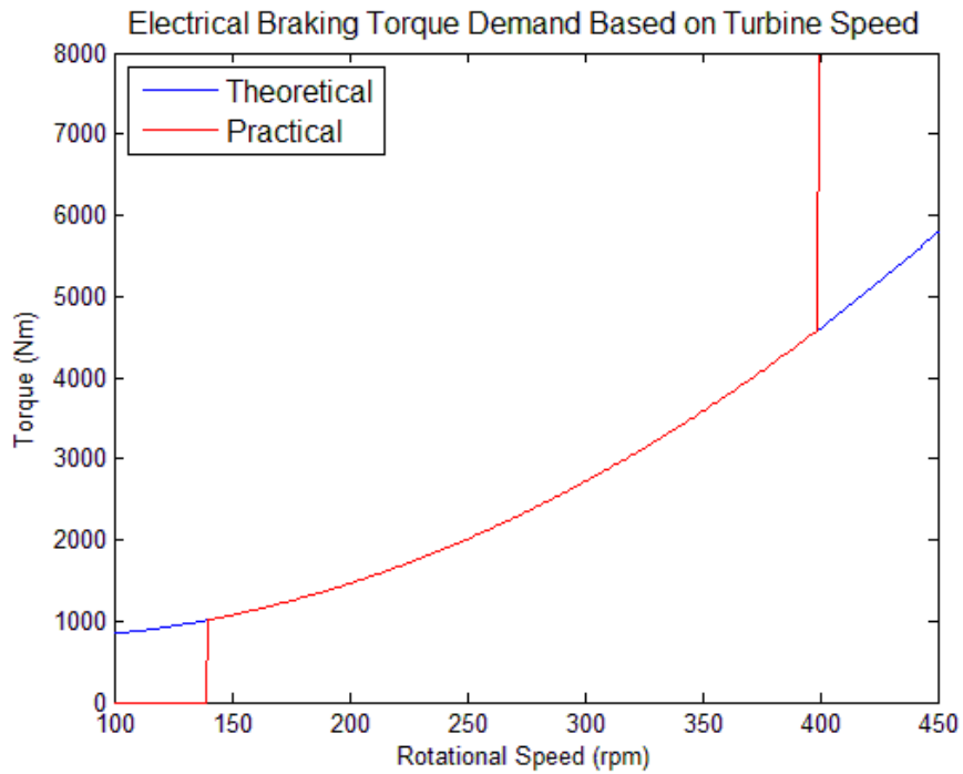
Fig. 5.6: Theoretical and practical values of the estimated electrical braking torque based on turbine speed produced by the high-inertia turbine control algorithm.
