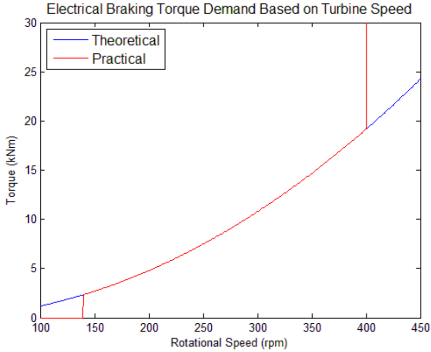
Fig. 5.5: Theoretical and practical values of the estimated electrical braking torque based on turbine speed produced by the low-inertia turbine control algorithm.
