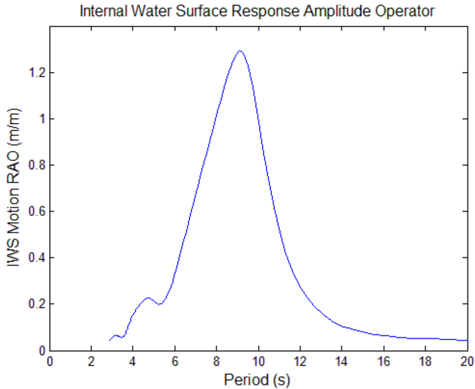
Fig. 5.2: RAO vs. wave frequency for the BBDB tested, as determined by WAMIT simulations.
