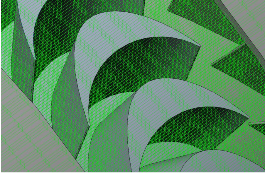
Fig. 4.10: Partial mesh generated by Flow Simulation to calculate the flow across the turbine.
