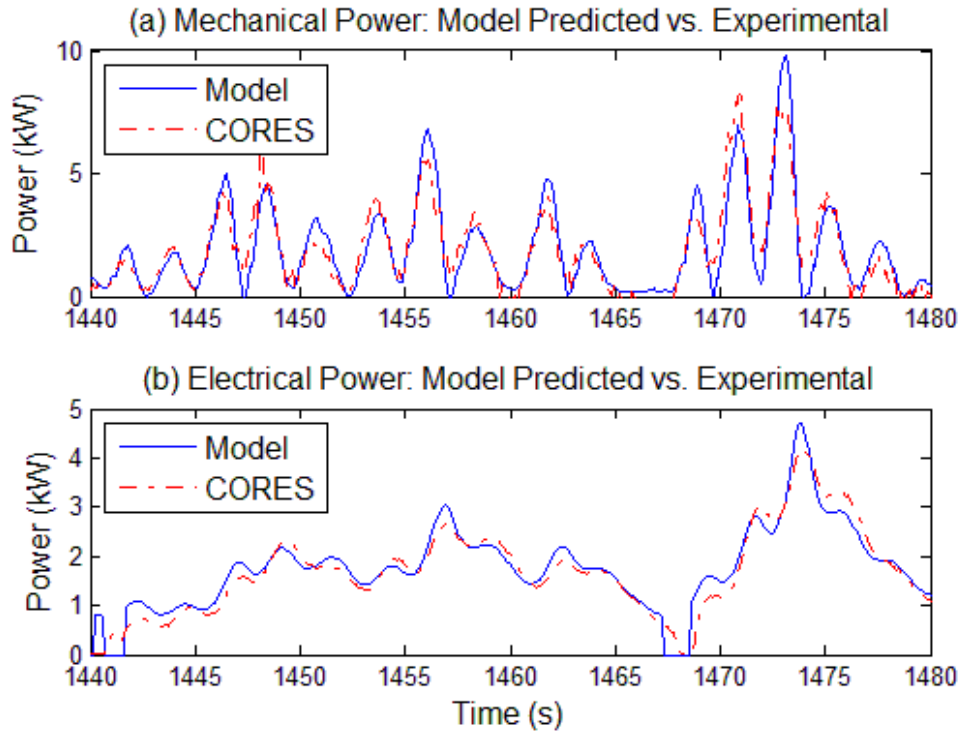
Fig. 3.5: Modelled and experimental data for mechanical power output (a) and electrical power output (b) for the data set where H_s=1.22 m and T_z=3.96 s.
