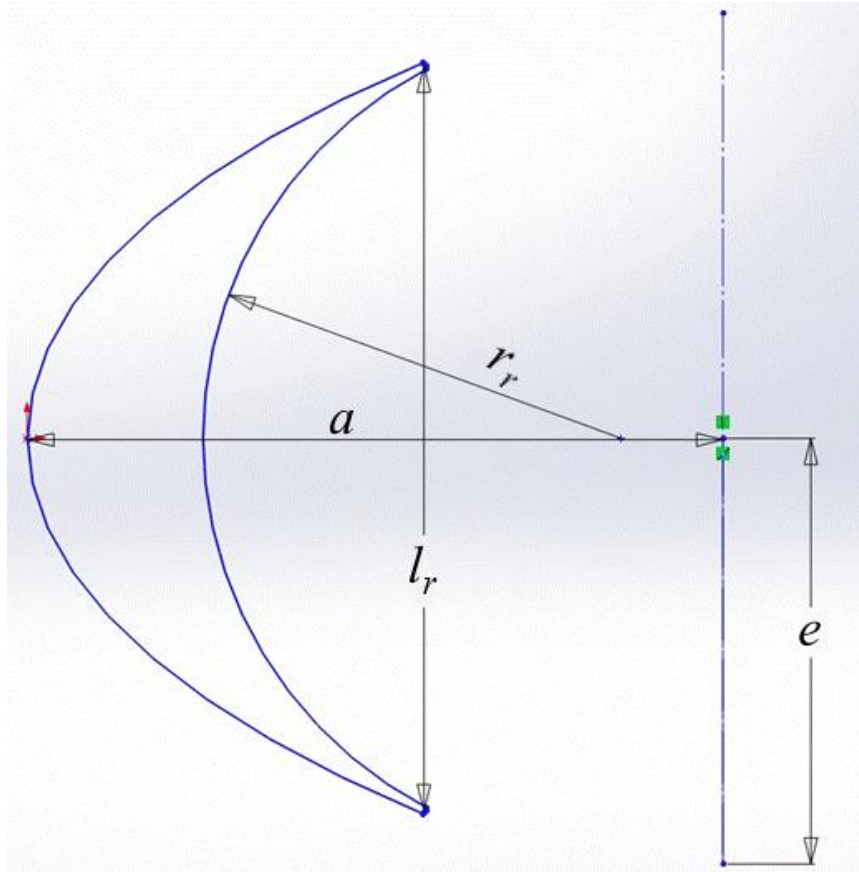
Fig. 2.8: Plan view of the turbine blade geometry with the main design parameters shown.
