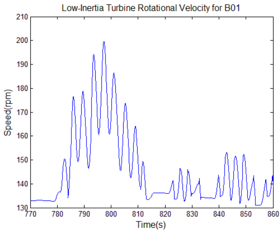
Fig. 5.11: Turbine rotational velocity from of the OWC model simulated with conditions created to match sea state B01.
