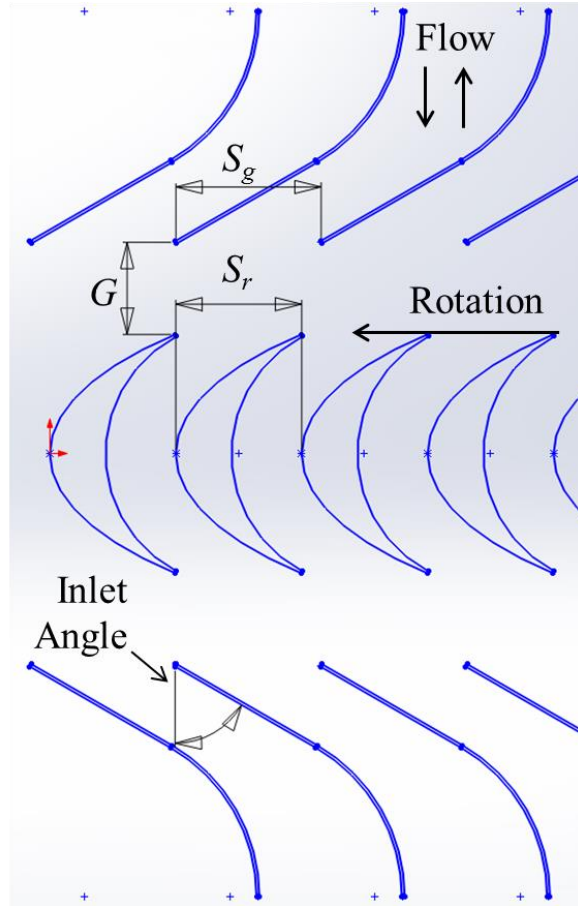
Fig. 2.10: The blade and guide vane profile in plan view along with the blade pitch, S_r , guide vane pitch, S_g , and the gap, G , between the guide vanes and rotor blades.
