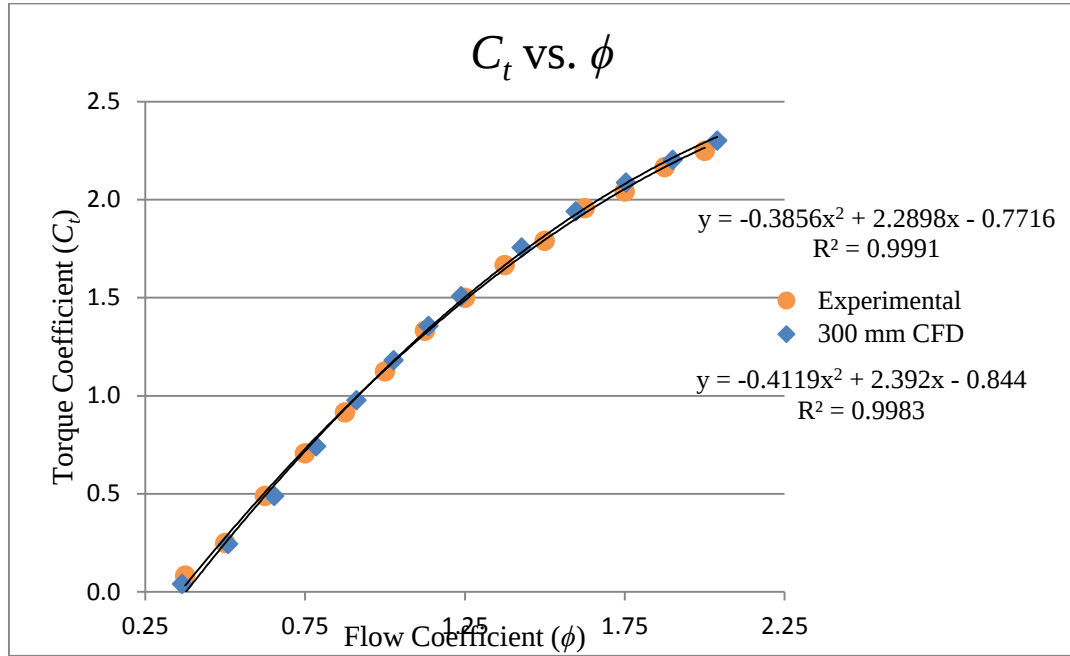
Fig. 4.12: C_t vs \phi , experimental results for 300mm turbine [41, 102] against CFD results for 300 mm turbine at 36 rads \cdot s ^{-1} .
