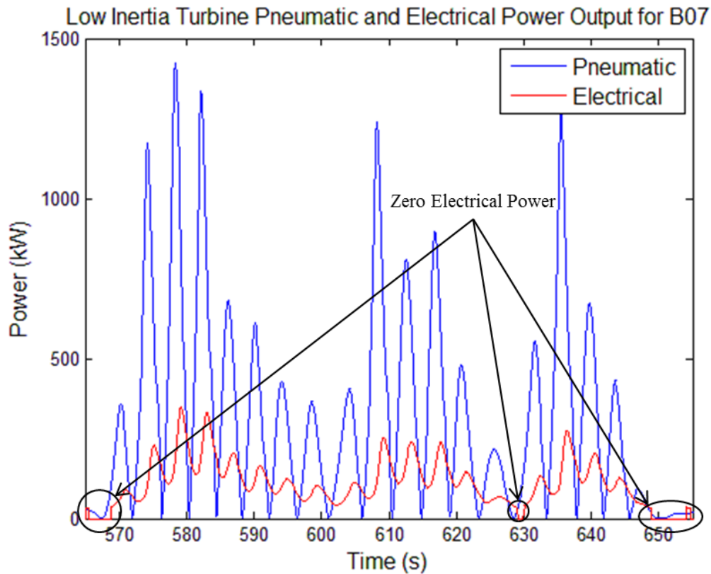
Fig. 5.8: Pneumatic and electrical power output of the OWC model simulated with conditions created to match sea state B07.
