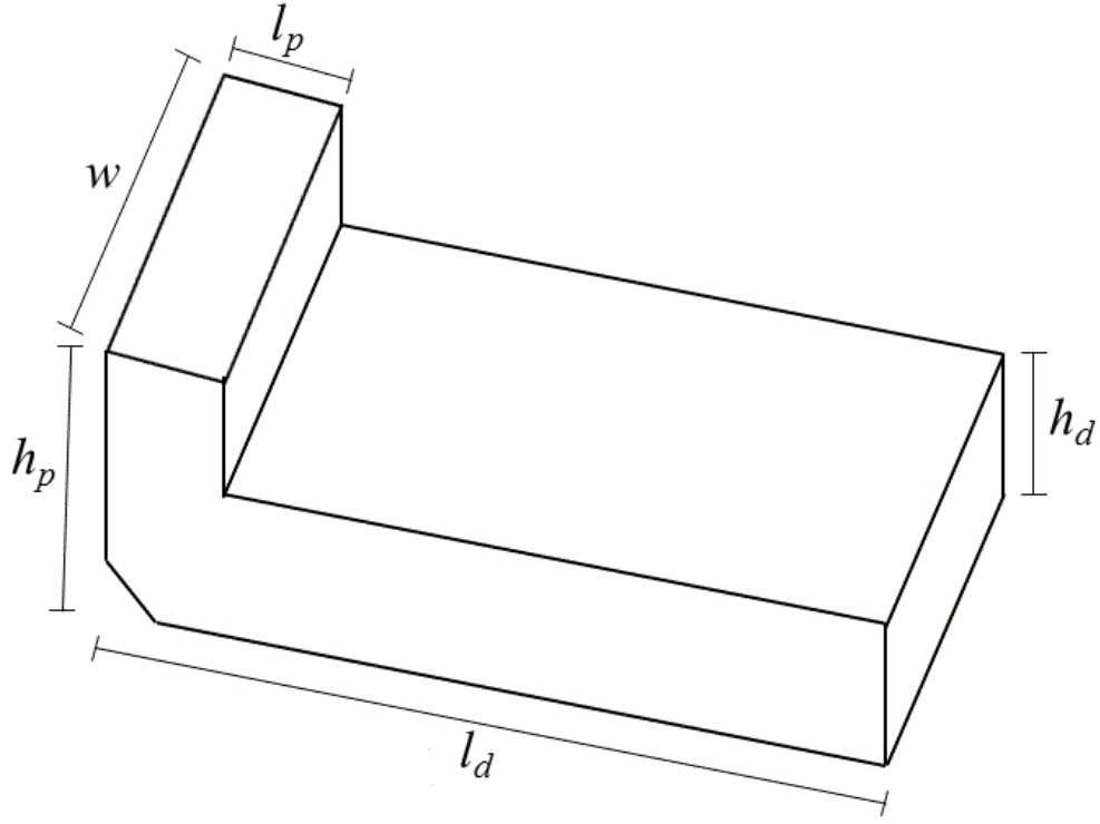
Fig. 4.1: BBDB design measurements: where width is w , draft length is l_d , draft height is h_d , plenum height is h_p and plenum length is l_p .
