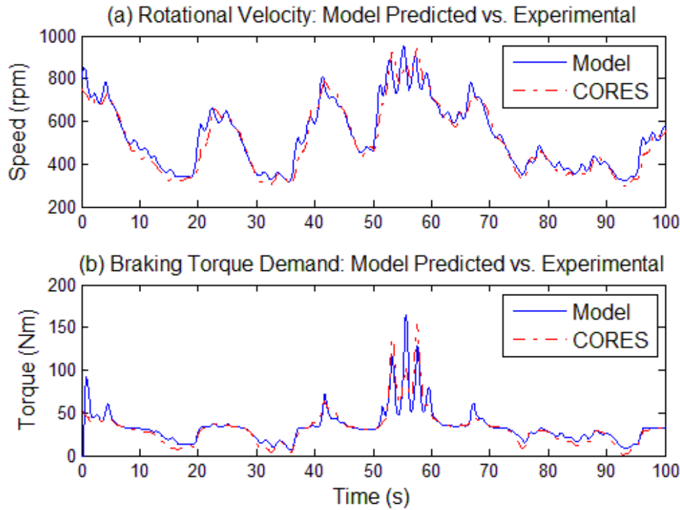
Fig. 3.3: Modelled and experimental data for the turbine rotational speed (a) and braking torque demand (b) for the data set where H_s=1.09 m and T_z=3.57 s.
