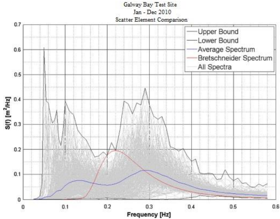
Fig. 3.15: Individual, averaged, and theoretical spectra within the ranges 0.625 \text{ m} < H_s < 0.75 \text{ m} and 3.0 \text{ s} < T_z < 3.5 \text{ s} for the Galway Bay test site [109].
