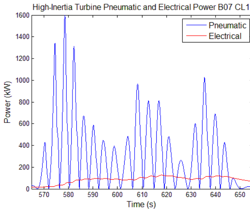
Fig. 5.12: Pneumatic and electrical power output of the OWC model with the high-inertia turbine controlled using Control Law 1 as simulated and conditions created to match sea state B07.
