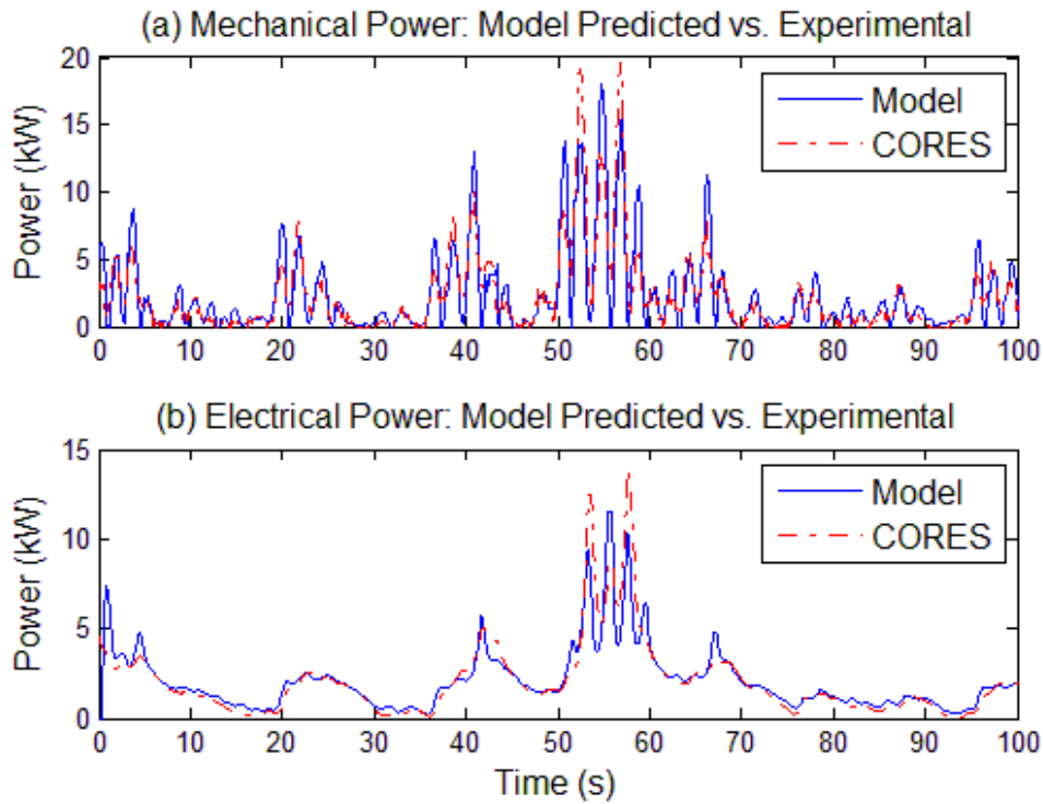
Fig. 3.6: Modelled and experimental data for mechanical power output (a) and electrical power output (b) for the data set where H_s=1.09 m and T_z=3.57 s.
