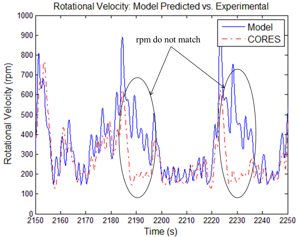
Fig. 3.16: Experimentally measured rotational velocity and model predicted velocity based on measured flow across the turbine.
