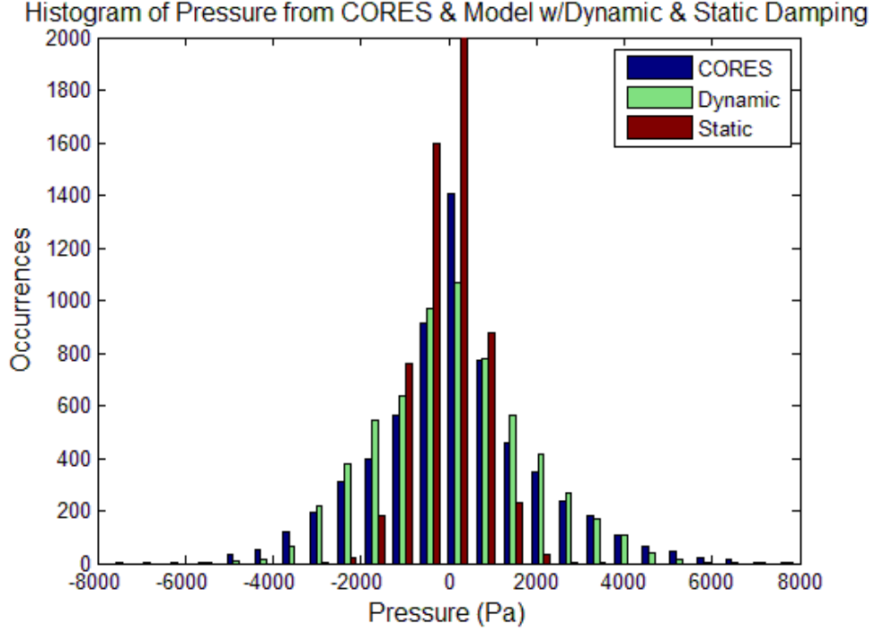
Fig. 3.10: Histogram of the experimental, dynamically damped model, and statically damped model data for chamber pressure for the data sets where H_s=1.09 m and T_z=3.57 s.
