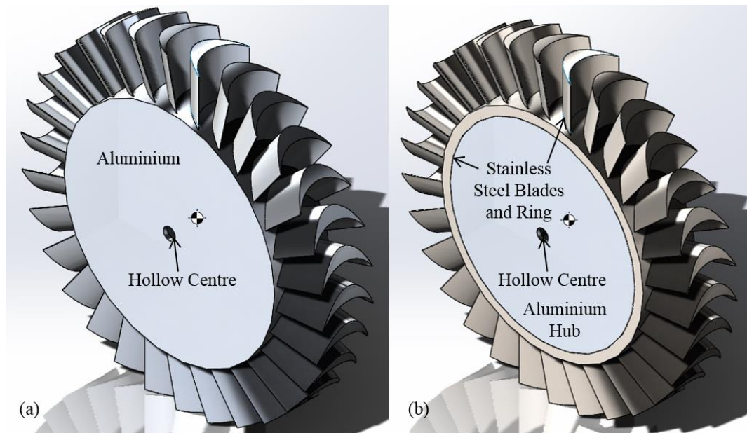
Fig. 5.1: Presents (a) the low-inertia aluminium alloy A356.0 impulse turbine minimises turbine mass and inertia and (b) the high-inertia impulse turbine composed of blades and outer ring of stainless steel with an inner hub hollow made of aluminium alloy A356.0 maximise inertia while minimising turbine mass.
