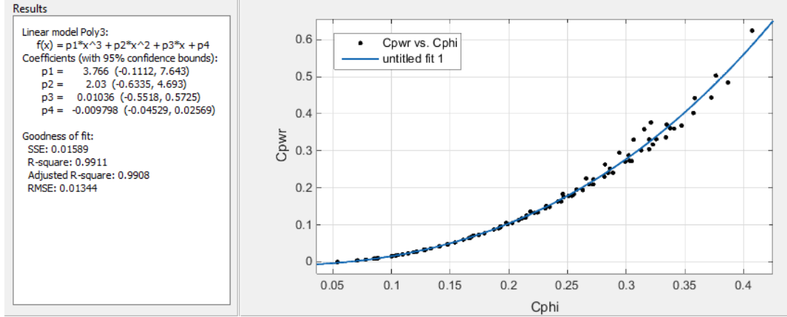
Fig. 4.19: MATLAB curve fitting application for the non-dimensional mechanical power data generated through CFD simulations.
