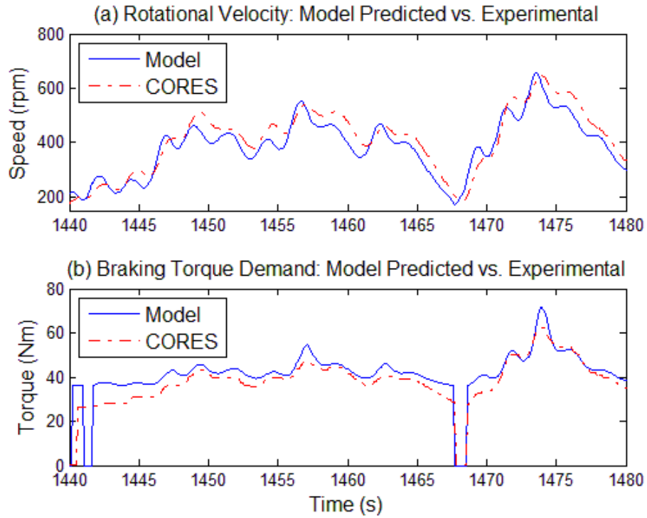
Fig. 3.2: Modelled and experimental data for the turbine rotational speed (a) and braking torque demand (b) for the data set where H_s=1.22 m and T_z=3.96 s.
