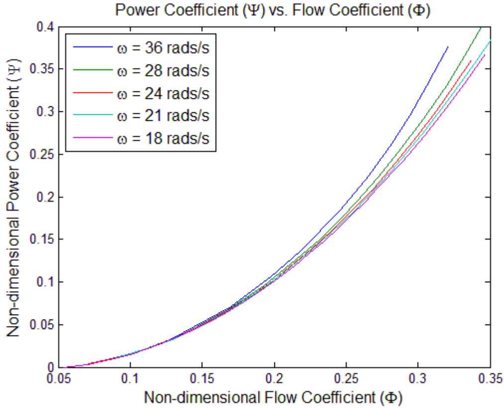
Fig. 4.18: Non-dimensional mechanical power, \Psi , vs. flow coefficient, \Phi , for 2.5 m impulse turbine based on the results of CFD simulations.
