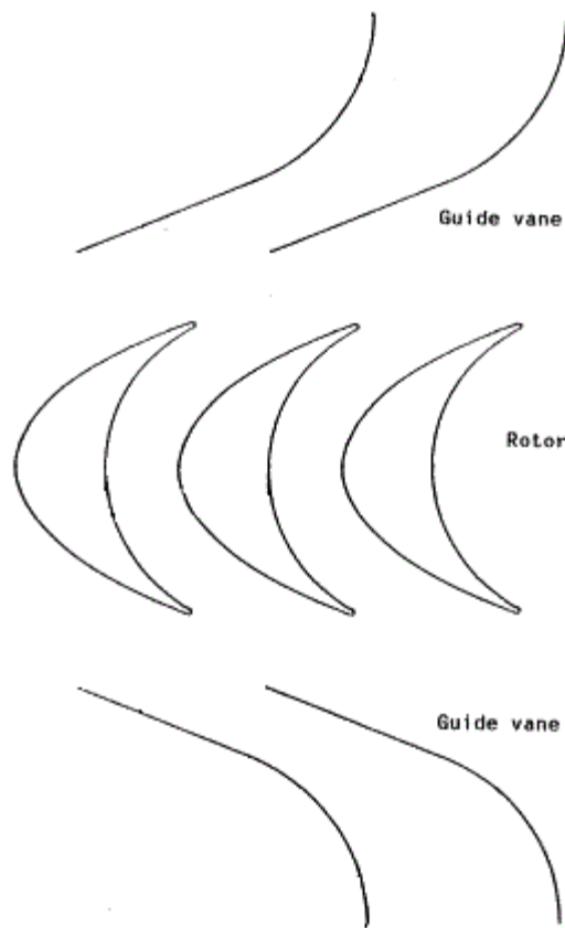
Fig. 1.11: Impulse turbine rotor blades and guide vanes [41].
