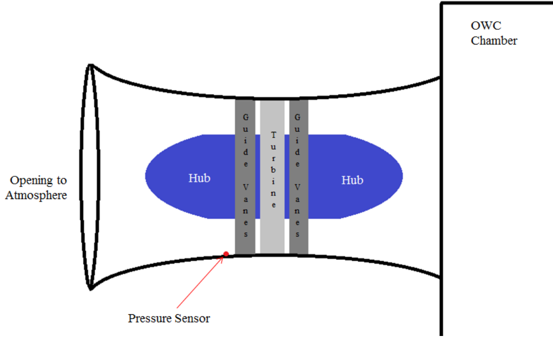
Fig. 3.1: The location of the pressure sensor used to calculate flow across the turbine using the Bernoulli method.
