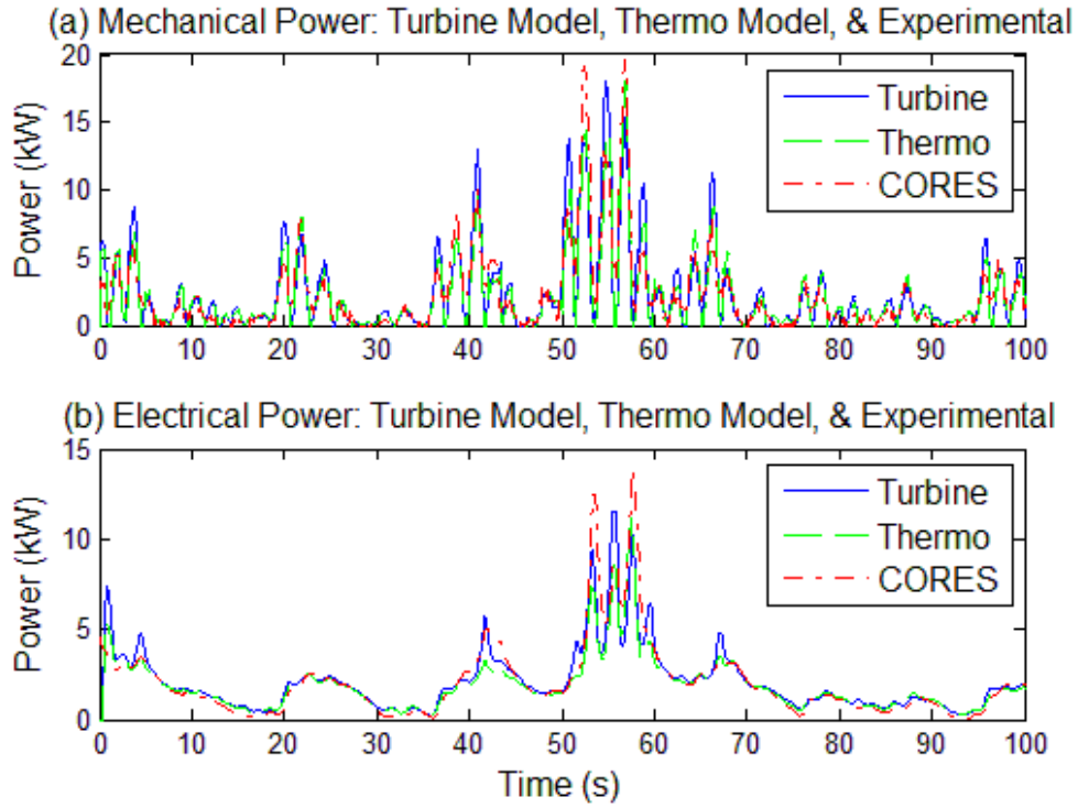
Fig. 3.14: Turbine model, thermodynamic model, and experimental data for the mechanical power output (a) and electrical power output (b) for the data set where H_s=1.09 m and T_z=3.57 s.
