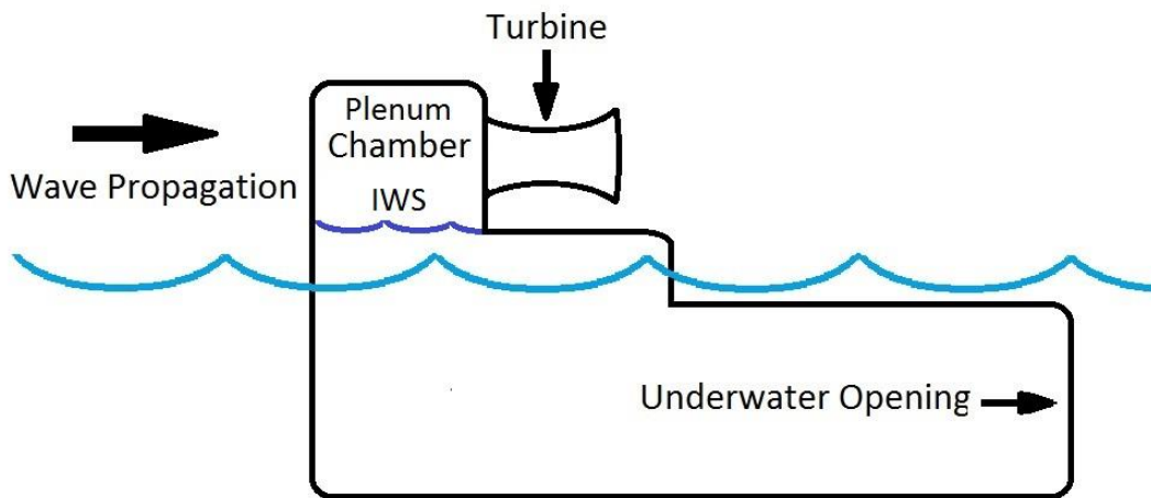
Fig. 2.1: Schematic diagram of a typical Bent Backwards Duct Buoy OWC.
