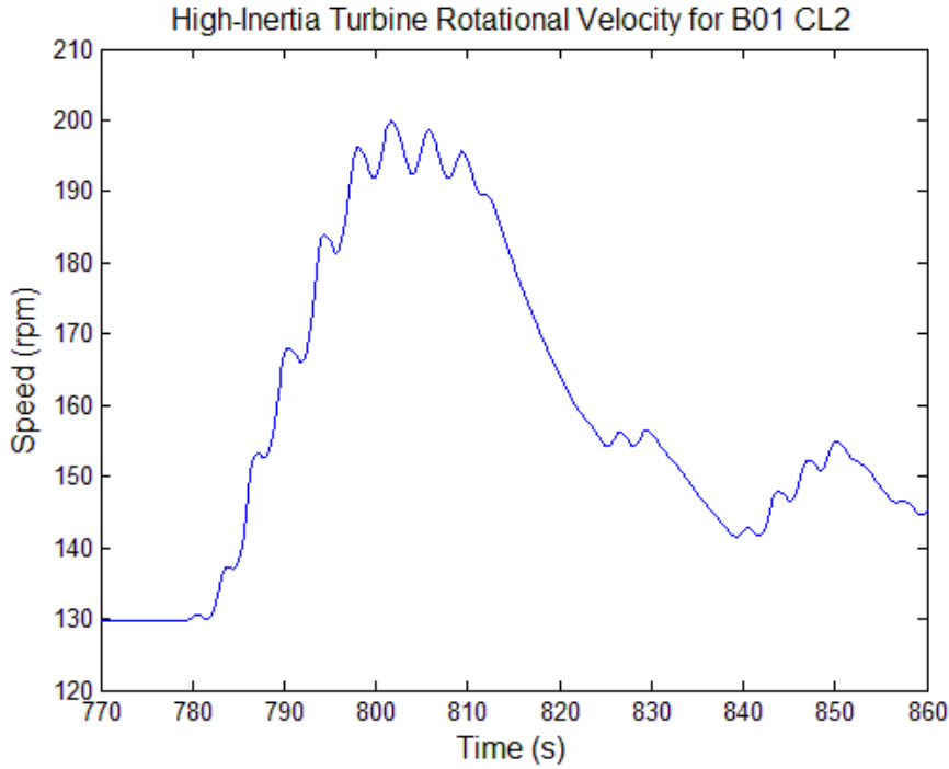
Fig. 5.19: Turbine rotational velocity from of the OWC model simulated with the high inertia turbine controlled using Control Law 2 and conditions created to match sea state B01.
