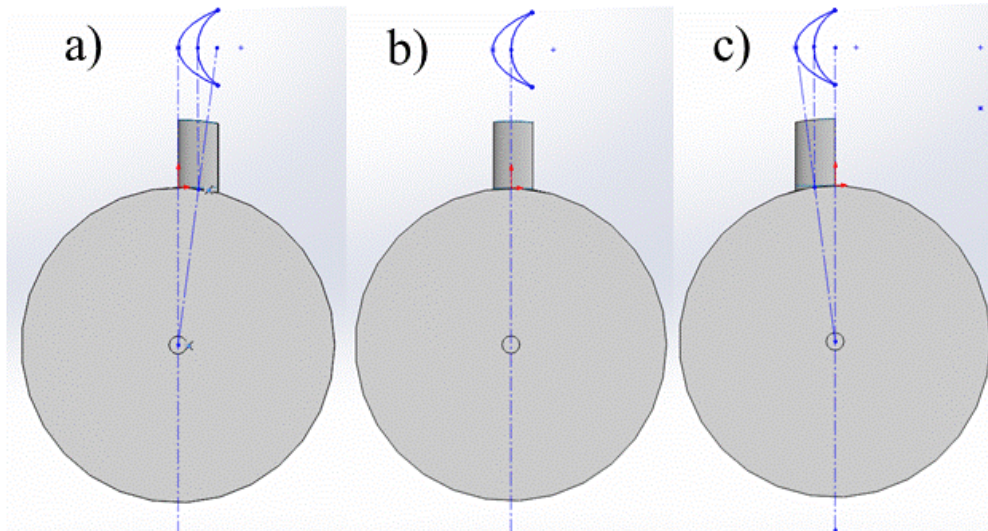
Fig. 2.11: How the blade sweep angles (a) -7.5^\circ , (b) 0^\circ , and (c) 7.5^\circ affect the position of the blade on the turbine hub.
