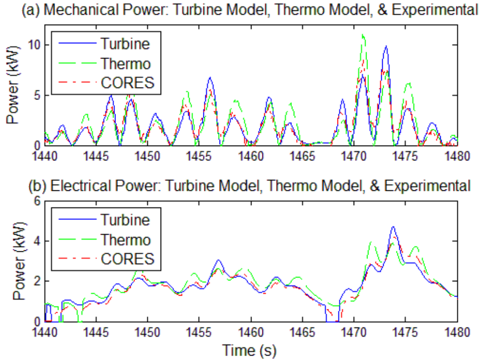
Fig. 3.12: Turbine model, thermodynamic model, and experimental data for the mechanical power output (a) and electrical power output (b) for the data set where H_s=1.22 m and T_z=3.96 s.
