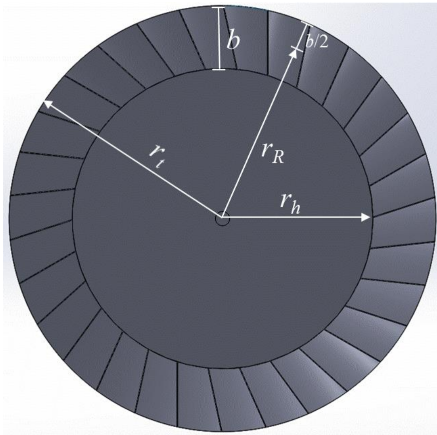
Fig. 2.7: An impulse turbine rotor with the values of the turbine radius, r_t , hub radius, r_h , mid-span radius, r_R , and the blade height, b .
