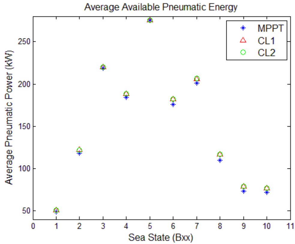
Fig. 5.20: Average available pneumatic energy per sea state for each of the three control laws tested.
