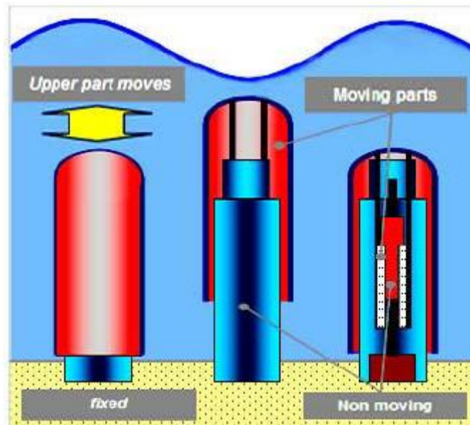
Fig. 1.3: Archimedes Wave Swing submerged heaving WEC [23].
