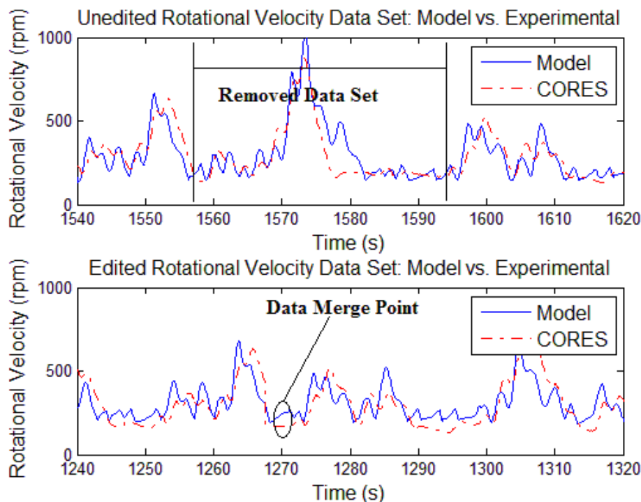
Fig. 3.20: Example of the edits performed on the experimentally collected data to remove the data compromised by the malfunctioning guide vanes.
