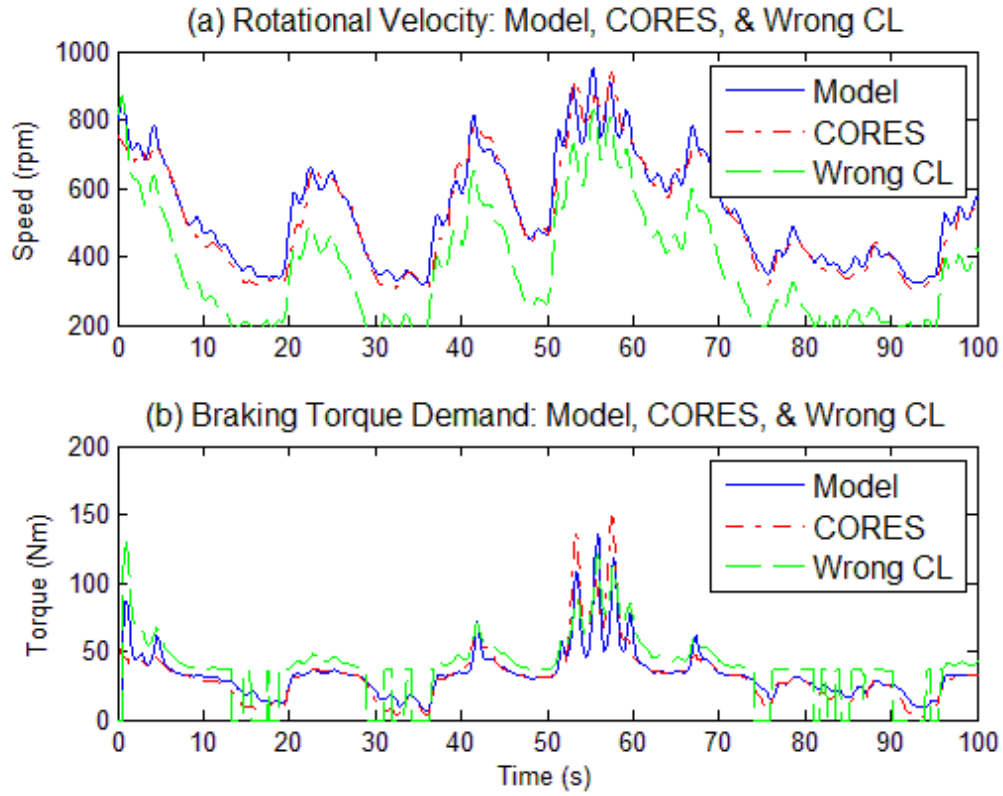
Fig. 3.4: Modelled, experimental and the modelled wrong control law coefficients data for the turbine rotational speed (a) and braking torque demand (b) for the data set where H_s=1.09 m and T_z=3.57 s.
