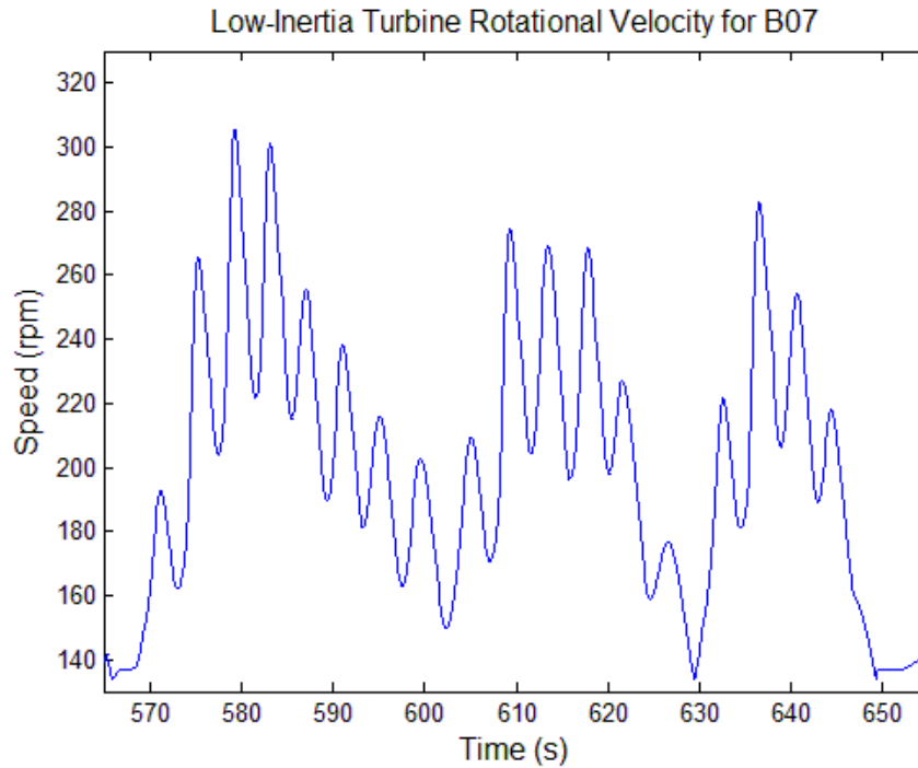
Fig. 5.9: Turbine rotational velocity from of the OWC model simulated with conditions created to match sea state B07.
