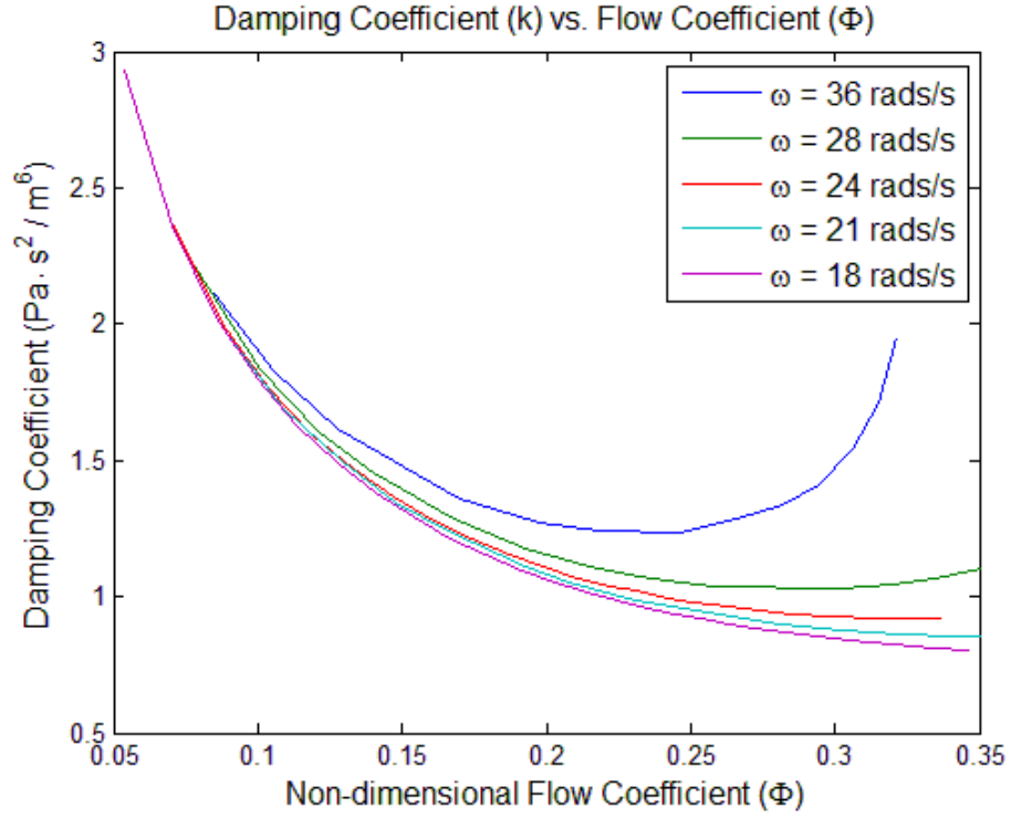
Fig. 4.22: Damping coefficient vs. flow coefficient for 2.5 m impulse turbine based on the results of CFD simulations.
