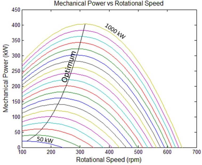
Fig. 5.4: Mechanical power output of the impulse turbine at different rotational speeds for pneumatic power from 50 kW to 1,000 kW in 50 kW steps and is represented by the various coloured curves. The optimal mechanical power based on rotational speed is represented by the black curve.
