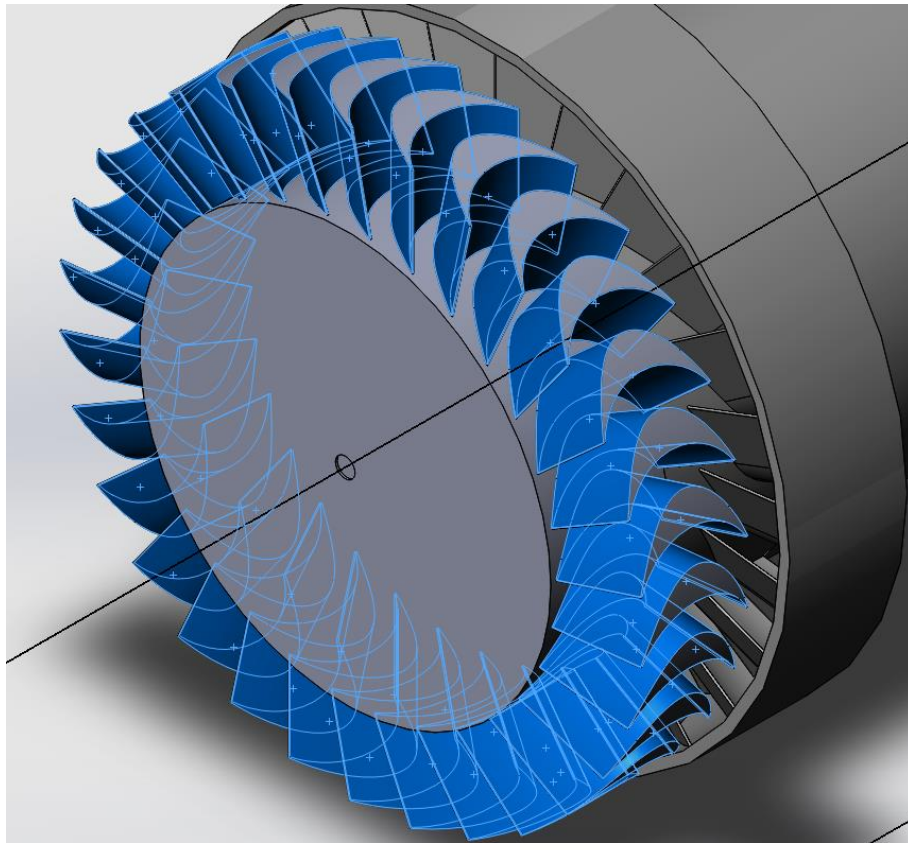
Fig. 4.7: Surface goal selection for turbine torque calculation.
