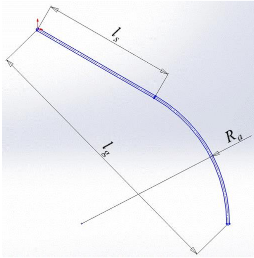
Fig. 2.9: Plan view of the guide vane geometry with the main design parameters shown.
