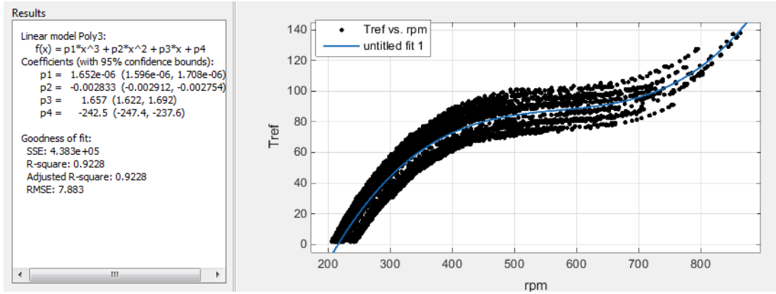
Fig. 2.4: Application of the MATLAB Curve Fitting App [98] to determine the control law coefficients for a single data set from the CORES output.
