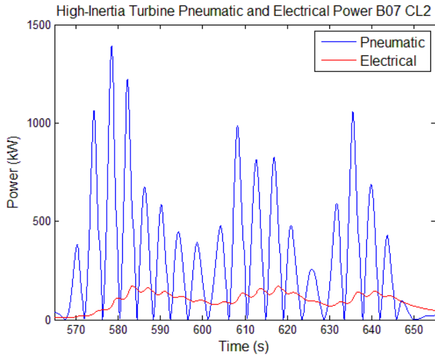
Fig. 5.16: Pneumatic and electrical power output of the OWC model with the high inertia turbine controlled using Control Law 2 as simulated and conditions created to match sea state B07.
