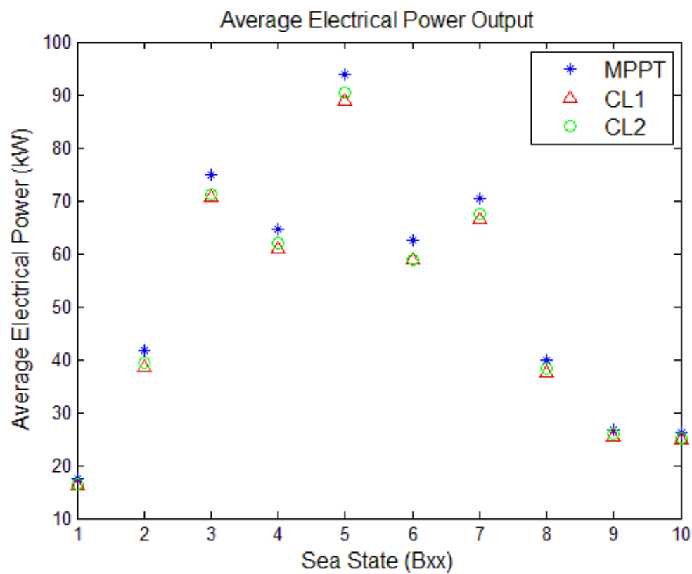
Fig. 5.21: Average electrical power output per sea state for each of the three control laws tested.
