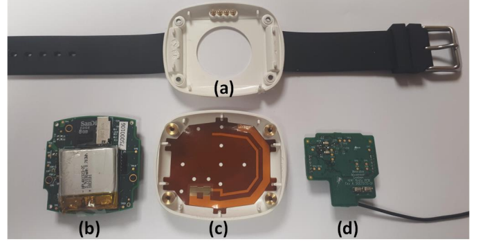
Fig. 6. Wristwatch model assembly: (a) Wristwatch enclosure, (b) Sensor assembly with battery, (c) Antenna prototype, and (d) Radio PCB.
