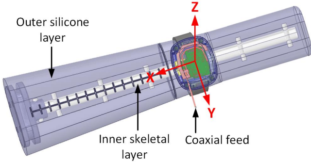
Fig. 2. Wristwatch model placed on a Speag phantom arm [14].
