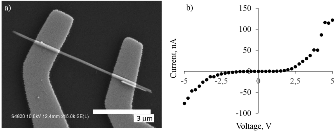
FIG. 2. (a) SEM image of a \text{SiO}_2 -coated Si substrate showing deposited \text{Bi}_2\text{S}_3 nanowires (diameters around 200 nm) and Ti/Au electrodes. (b) Typical current-voltage characteristics of an individual \text{Bi}_2\text{S}_3 nanowire released from the AAO membrane.
