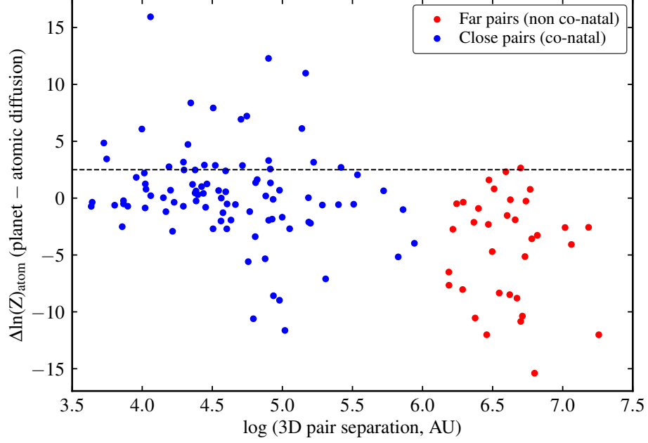
Extended Fig. 4: Differences in Bayesian evidence \Delta \ln(Z)_{\text{atom}} between the planetary ingestion and the atomic diffusion models as a function of spatial separations \Delta s . The red and blue circles represent the far and close co-moving pairs, respectively. The dashed line marks out our selection criterion for \Delta \ln(Z)_{\text{atom}} . It demonstrates that the far co-moving pairs (non co-natal sample) are distinctively affected by atomic diffusion (possibly due to larger differences in the relative stellar parameters such as \Delta T_{\text{eff}} ), when compared to the close, co-natal co-moving pairs.
