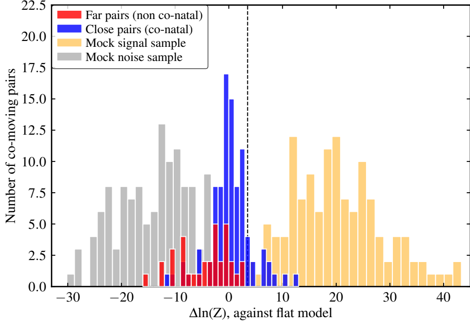
Extended Fig. 3: The distributions of differences in Bayesian evidence \Delta\ln(Z) between the planetary ingestion and the flat models. Red: the control sample of far co-moving pairs ( \Delta s \geq 10^6 AU); blue: the target sample of close, co-natal co-moving pairs ( \Delta s < 10^6 AU); grey: the mock noise sample; orange: the mock signal sample. The distributions, unlike that of T_{\text{cond}} trends, are distinguishable between different samples, indicating that we can effectively disentangle the potential planet signatures in the 91 co-natal pairs from the control sample of far pairs, as well as from the mock sample representing realistic noise and pure signal.
