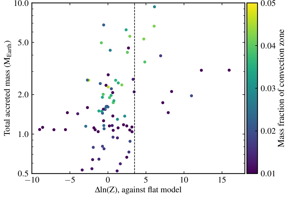
Extended Fig. 5: Total accreted mass of Earth material (from the best-fitting model) as a function of \Delta \ln(Z) between the planetary ingestion and the flat models for the 91 close, co-natal co-moving pairs. The dashed line marks out our selection criterion for \Delta \ln(Z) . The data are colour-coded with the mass fraction of convection zone ( f_{\text{CZ}} ), indicating that stars with larger \Delta \ln(Z) tend to have larger accreted mass, while the exact amount of accretion is determined by f_{\text{CZ}} .
