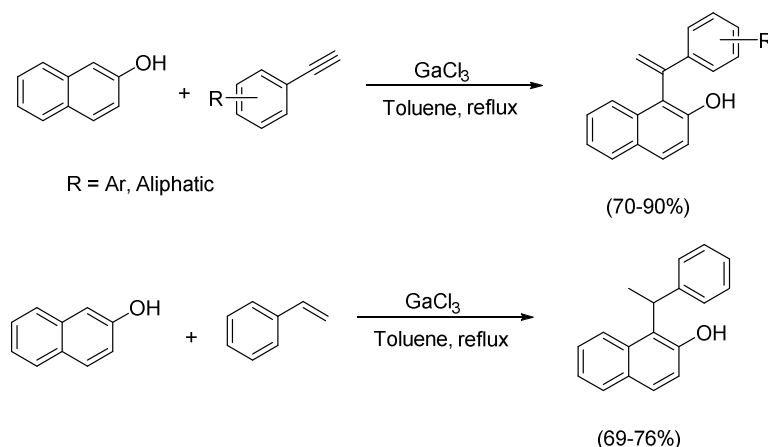
Scheme 45
