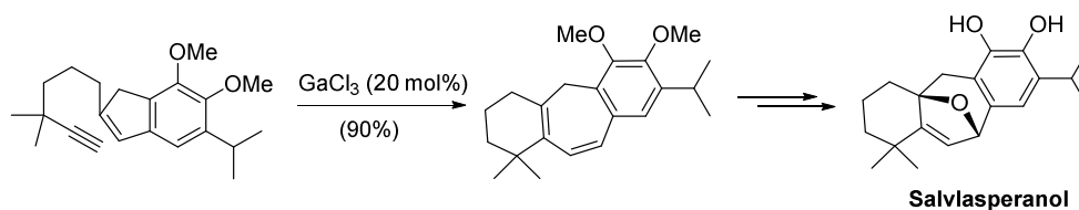
Scheme 30
