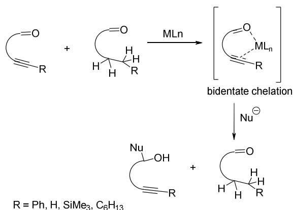
Scheme 24
