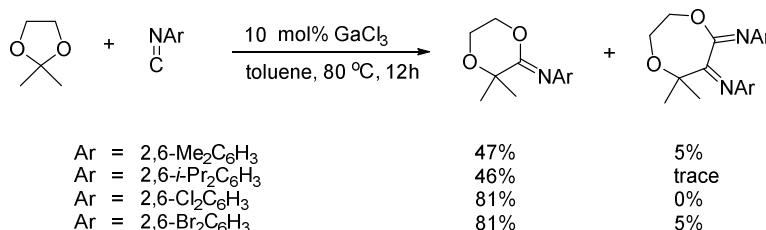
Scheme 35
