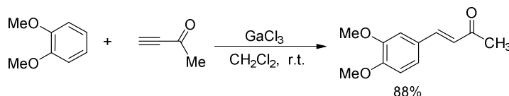
Scheme 46
