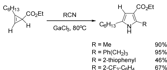
Scheme 39
