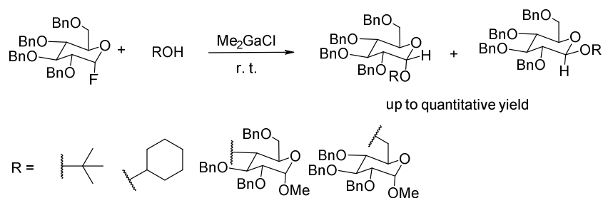
Scheme 36
