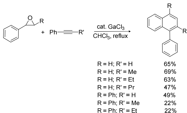
Scheme 18
