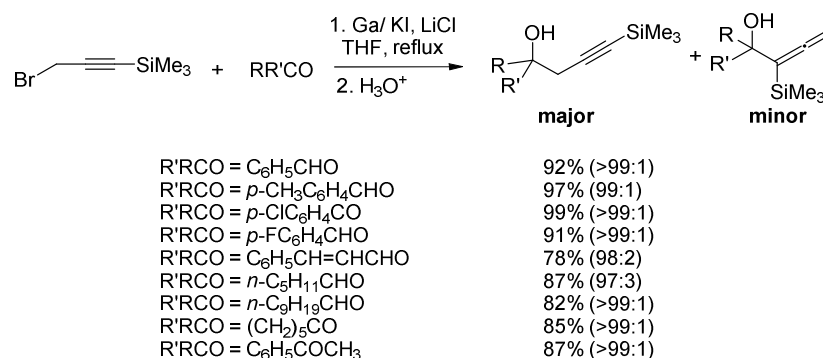
Scheme 13
