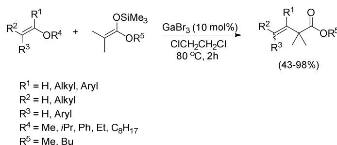
Scheme 21
