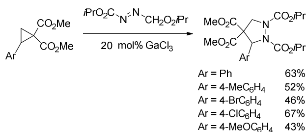
Scheme 33
