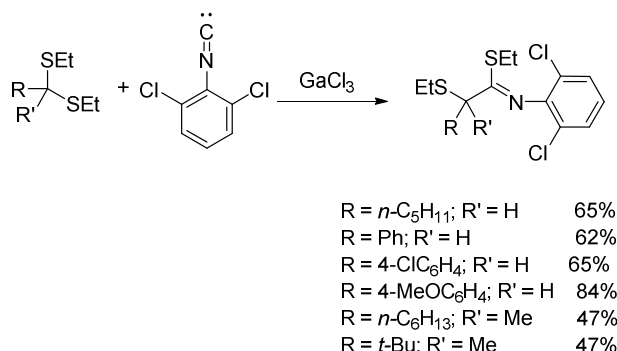
Scheme 34
