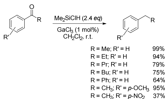
Scheme 48
