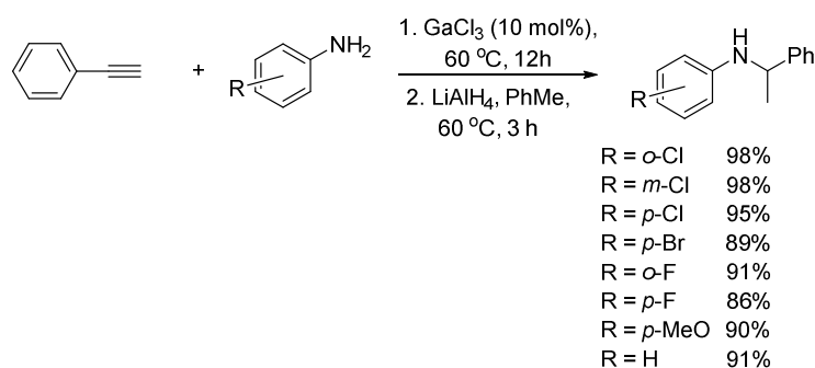
Scheme 49
