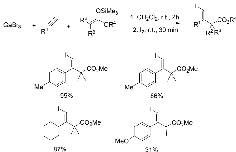
Scheme 23
