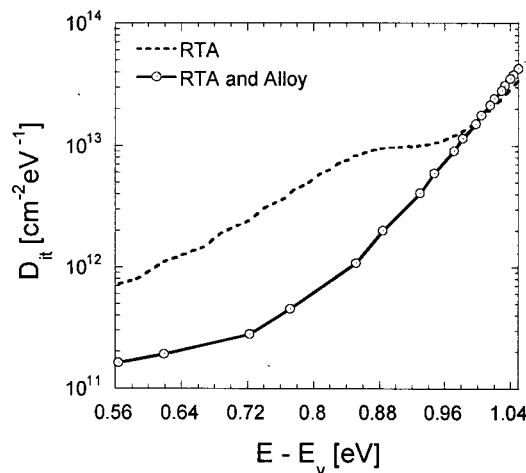
FIG. 7. Density of interface states ( D_{it} ) across the energy gap at the Si(100)–SiO 2 interface, extracted from the measured HFCV characteristics in Fig. 6 for process 2. The interface state densities are plotted with reference to the highest energy in the valence band ( E_v ). The figure shows the data for the 1050 °C RTA only sample, and for the sample subjected to RTA and alloy. The D_{it} values from E_v to mid-gap are not plotted as the extraction was performed using HFCV data.
