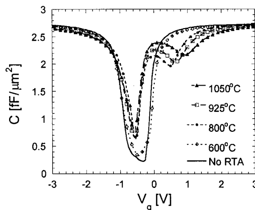
FIG. 3. Measured quasi-static CV characteristics of polysilicon/oxide(120 Å)/p-silicon(100) capacitor structures (process 1) subjected to RTA at a range of temperatures as the final processing step. All RTA processes were 10 s duration in N 2 . The control sample exposed to no RTA is also shown.
