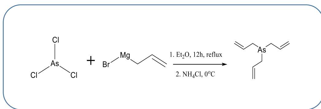
Figure 2.1. Synthetic reaction scheme for the triallylarsine molecule. Arsenic trichloride was reacted with an excess of allylmagnesium bromide in refluxing diethyl ether for 12 h. After the 12 h had elapsed the reaction was quenched with saturated ammonium chloride solution at 0 °C and stirred for a further 2 h after which the oily residue was twice distilled and stored under argon.
