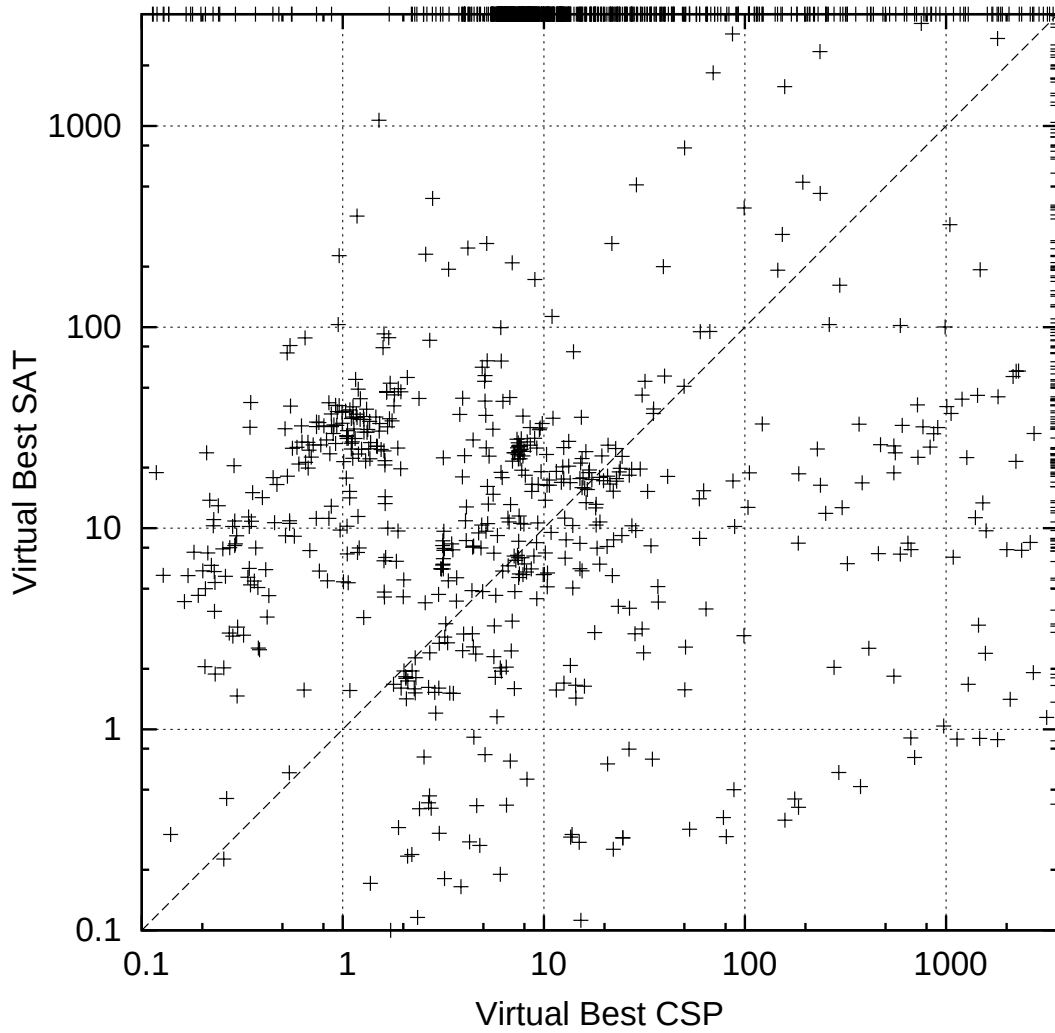
Figure 4.2: Performance of the virtual best CSP portfolio and the virtual best SAT-based portfolio.
