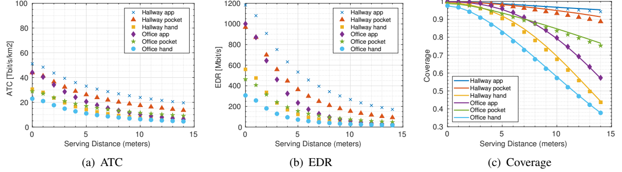
Fig. 8. Impact of the serving distance. Other network settings n_{TX} = 11 , \omega_{TX} = 30^\circ , and p_{LOS} = .5 .
