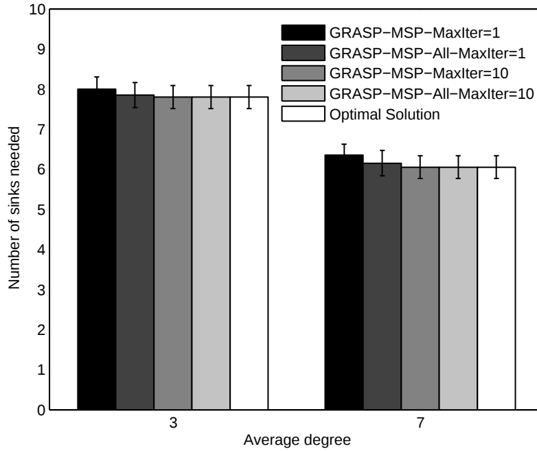
Figure 84: Number of sinks needed for GRASP-MSP and the optimal solution versus average degree
