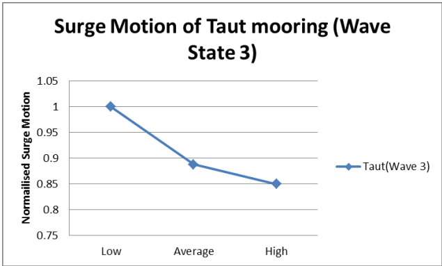
Fig. 26: Maximum surge displacement from CoG at varying depths
