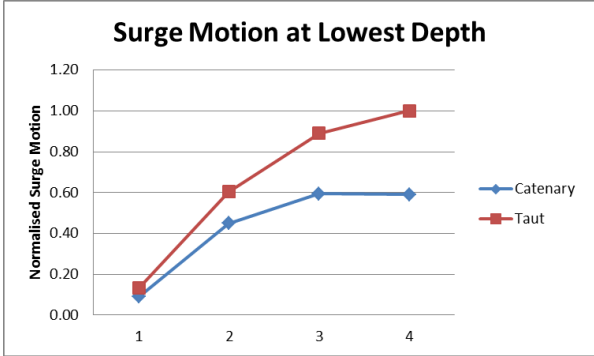
Fig.25: Maximum Surge motion from CoG at lowest depth
