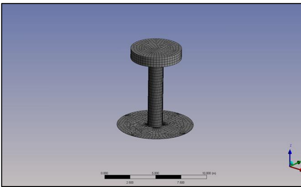
Fig. 8: Mesh of the RM3 device in ANSYS AQWA
