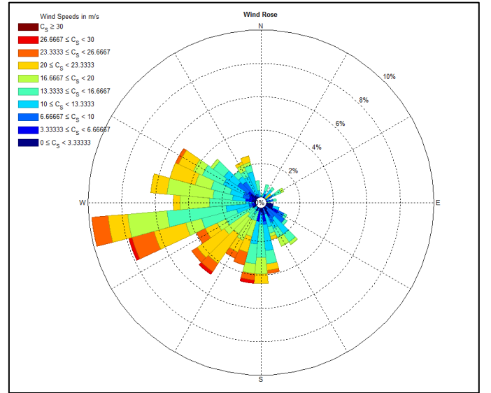
Fig. 6: Wind rose diagram for Galway bay
