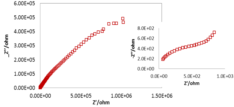
Figure 4.28: Nyquist plot of EIS for B6 microband array ( N=5 , d=50\ \mu\text{m} ) in 1 mM FCA in PBS. E_{1/2} at 0.29 V, frequency 0.01-1MHz (Inset: EIS at higher frequency of 28,400 Hz -1MHz).
