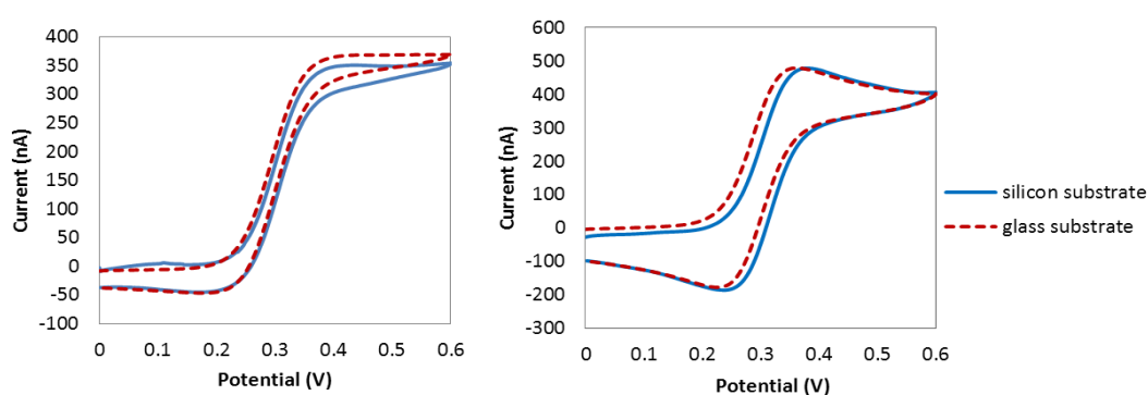
Figure 3.16: CV comparison for glass-based (red dotted line) and silicon-based microelectrode array (blue line) for 10 \text{ }\mu\text{m} microdisc (right) and 10 \text{ }\mu\text{m} microband (left) at 200 nm recess depth. Scan rate 100 \text{ mV s}^{-1} in 1 mM FCA in PBS.
