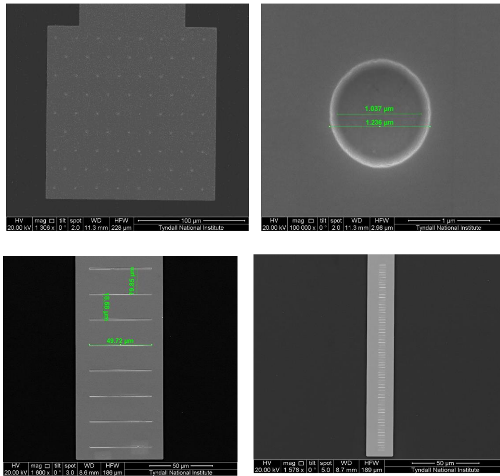
Figure 3.5: Top row: SEM images of 1 μm microdisc array, d2 (300 nm recess depth). Bottom row: SEM images of 1 μm microband, b2 (left) and 100 nm microband, b3 (right); both with 200 nm recess depth.
