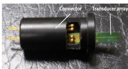
Figure 3.8: Picture of the custom made connector with the fabricated microelectrode array
