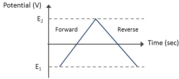
Figure 1.6: The potential waveform applied to the working electrode in the cyclic voltammetry experiment.
