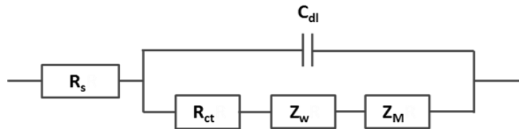
Figure 4.29: Equivalent circuit suggested for microelectrode.
