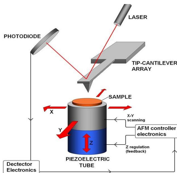
Figure 5.4: Schematic representation of the atomic force microscopy*.
