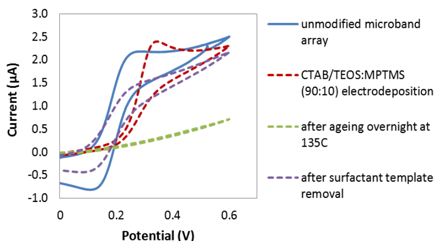
Figure 3.45: CVs of the unmodified microband array (solid blue line), electrodeposition of CTAB/TEOS:MPTMS precursors on the surface (red dashed line), after ageing overnight at 135°C (green dashed line) and after surfactant removal (purple dashed line). CV recorded in 5 mM FcMeOH in 0.1M NaCl (scan rate 50 mV s -1 ). Potential achieved after deposition time of 8 secs was -1.41 V, current density -7.4 mA cm -2 .
