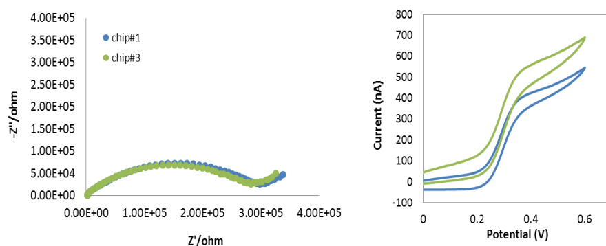
Figure 6.6: EIS (frequency 0.01- 100,000 Hz) and CV (scan rate of 100 mV s -1 ) performed in 1 mM FCA in PBS for unmodified electrodes.
