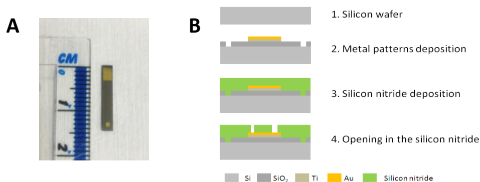
Figure 5.7: (A) Picture of gold electrode with 1mm disc used in this study; and (B) simplified fabrication process for the electrode.
