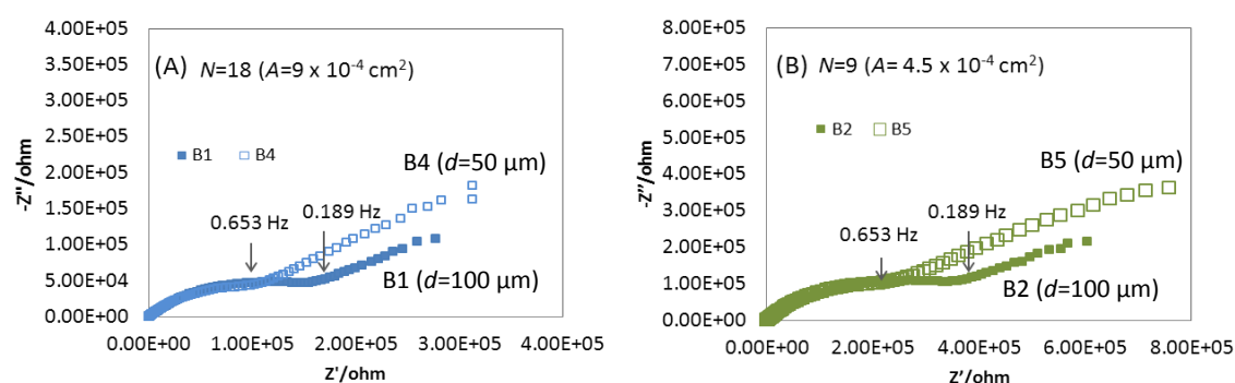
Figure 4.27: EIS spectrum in 1 mM FCA in PBS (frequency 0.01-1MHz, E_{1/2} at 0.29 V) for the band arrays of same surface area (A) A=9 \times 10^{-4}\ \text{cm}^2 ( N=18 ); and (B) A=4.5 \times 10^{-4}\ \text{cm}^2 ( N=9 ). Filled marker indicate d=100\ \mu\text{m} while non-filled marker indicate d=50\ \mu\text{m} .
