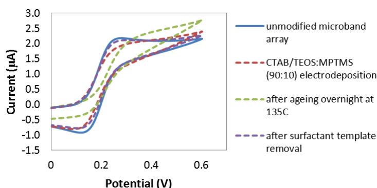
Figure 3.42: CVs of the unmodified microband array (solid blue line), electrodeposition of CTAB/TEOS:MPTMS precursors on the surface (red dashed line), after aging overnight at 135°C (green dashed line) and after surfactant removal (purple dashed line). CV recorded in 5 mM FcMeOH in 0.1M NaCl (scan rate 50 mVs -1 ). Potential achieved after deposition time of 16 secs was -0.84 V, current density -0.74 mA cm -2 .
