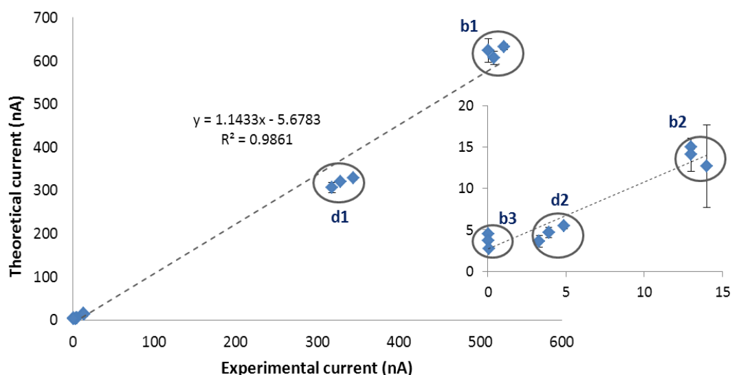
Figure 3.17: Correlation between experimental current and theoretical current for all the microelectrode designs and recess depth thicknesses. Inset: Correlation graph for 1 \mu m microdisc (d2), 1 \mu m microband (b2) and 100 nm microband (b3) arrays.
