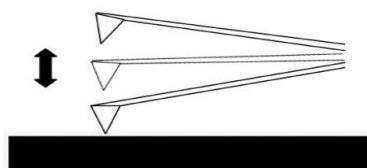
Figure 5.5 : Diagram of probe and surface interaction in tapping mode.
