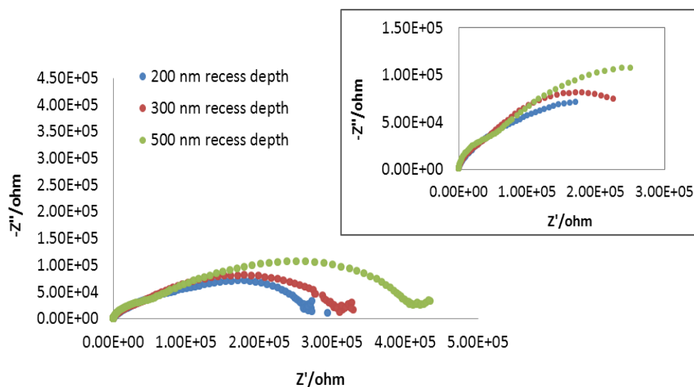
Figure 3.23: Impedance spectra for d1 microdisc arrays with different passivation layers in 1mM FCA in PBS. Frequency range 0.01 Hz -1 MHz and applied amplitude 0.01 V for all arrays. Inset: EIS at frequency 200-200,000 Hz.
