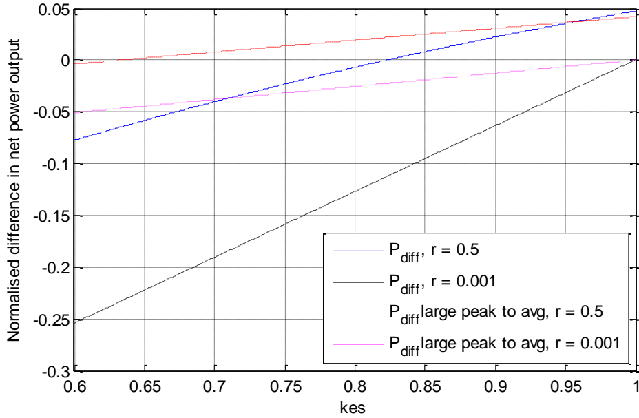
Figure A.7: Normalised difference in net power output for cases where energy storage is and isn't used. Also taking into account the resultant power loss due to I^2R in the transmitted power, and comparing with large peak to average input power
