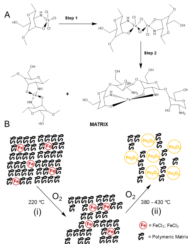
Fig. 7. Schematic representation of the possible mechanism in the formation of \text{Fe}_2\text{O}_3 nanoparticles from the decomposition of the various precursors. (A) Coordination model of \text{FeCl}_2 to Chitosan. (B) Representation of pyrolytic decomposition including chain scission, oxidation and crystallization of \text{Fe}_2\text{O}_3 from the macromolecular complexes.
