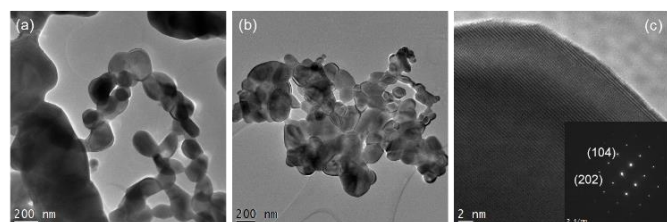
Fig. 4. (a,b) TEM images of the pyrolytic fused nanocrystal product from the PS-co-4-PVP•(FeCl 3 ) y precursor (c) HRTEM image of the single crystalline structure of Fe 2 O 3 nanoparticles.
