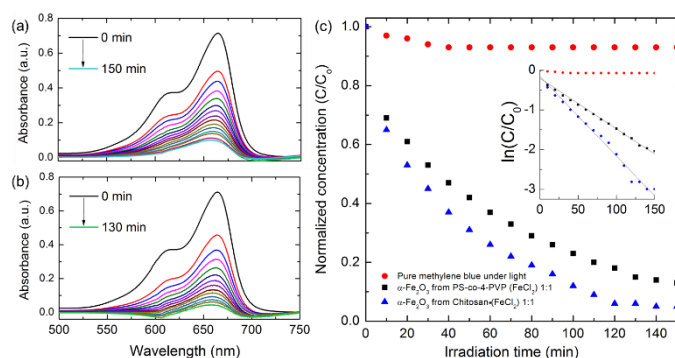
Fig. 8. (a) Degradation curves of MB in presence of (a) \alpha\text{-Fe}_2\text{O}_3 /PS-co-4-PVP, (b) \alpha\text{-Fe}_2\text{O}_3 /Chitosan. (c) Normalized concentration changing of MB without catalyst, in presence of \alpha\text{-Fe}_2\text{O}_3 /PS-co-4-PVP and in presence of \alpha\text{-Fe}_2\text{O}_3 /Chitosan.
