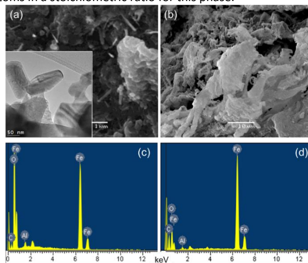
Fig. 2. (a) SEM image of the product from pyrolysis of the Chitosan•(FeCl 3 ) y precursors in 1:1 ratio and (b) from the Chitosan•(FeCl 3 ) n precursor in a 1:5 ratio. (c,d) The EDS spectra confirm Fe and O presence and successful elimination of Cl from both precursors during hematite formation. The Al signal is from the sample stub.
