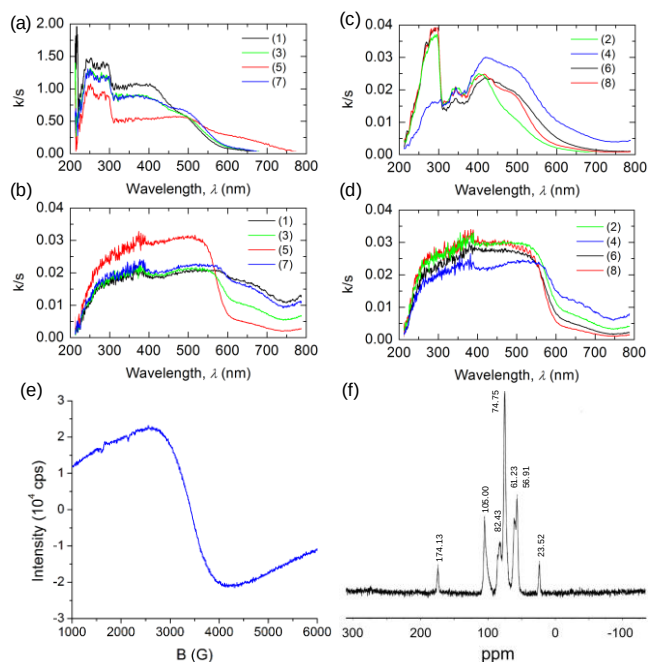
Fig. 1. UV-visible Kubelka-Munk diffuse reflectance spectra of macromolecular complexes 1,3,5,7 (a) before and (b) after pyrolysis. (c) UV-visible spectra from macromolecular complexes 2,4,6,8 (c) before and (d) after pyrolytic treatment. Spectra were acquired from samples in powder form after pyrolysis. (e) EPR spectra of macromolecular complex 1 and (f) ^{13}C MAS NMR spectrum of Chitosan•(FeCl 3 ) y . Reference diffuse reflectance spectra from the Chitosan and PS-co-4-PVP shown in Supporting Information, Fig. S 2 .
