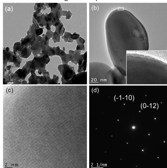
Fig. 3. (a) TEM image of the fused nanoparticulate structure of the pyrolyzed hematite from the 1:1 Chitosan•(FeCl 3 ) y precursor. HRTEM examination in (b) and (c) confirms single crystal structure indexed to trigonal hematite (Space Group R-3c) in the electron diffraction pattern in (d).
