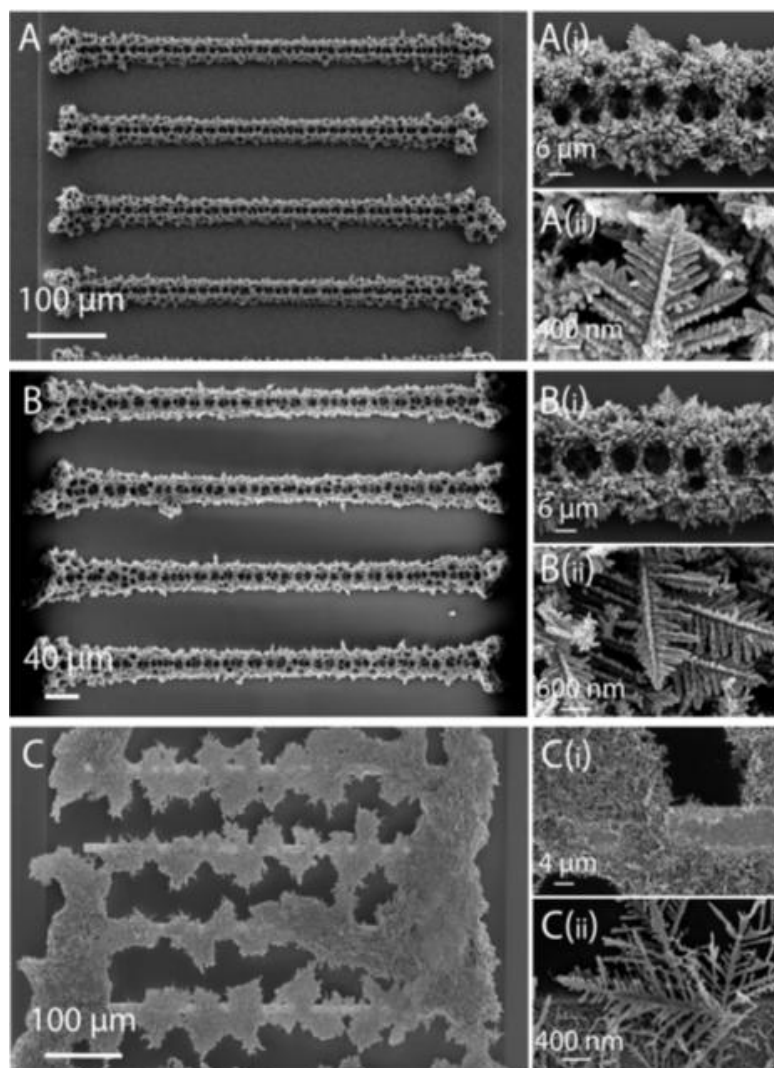
Figure 2.2. SEM images of BA10-CuFoam electrodes prepared at different \text{H}_2\text{SO}_4 concentrations; (A, A-i and A-ii; increased magnification), 1M \text{H}_2\text{SO}_4 , (B, B-i and B-ii; increased magnifications) 0.5M \text{H}_2\text{SO}_4 , (C, C-i and C-ii; increased magnifications) 0.05M \text{H}_2\text{SO}_4 at a applied voltage of -6 V vs. Ag/AgCl in the solution containing 0.87 mg \text{Cu}^{2+}
