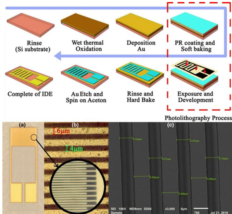
Figure 1.27 Fabrication of the electrode. LPM, HPM and SEM images for Au IDE electrode; (a) LPM image under 4.5 \times magnification, (b) 15 \times and 50 \times magnification was used to scan the Au IDE surface using HPM under ambient temperature (c) SEM image for 3000 \times magnification 114
