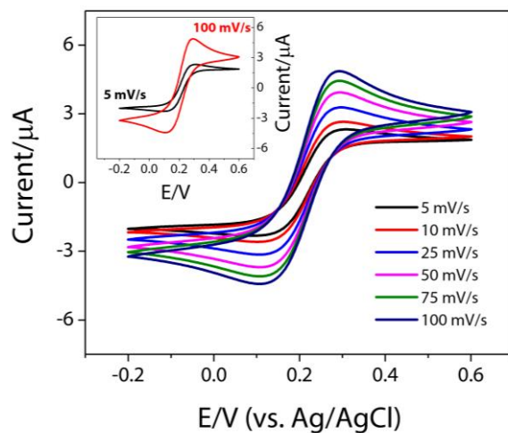
Fig 5.S2. CVs of bare band array electrode recorded at different scan rates; 5, 10, 25, 50, 75 and 100 mV s -1 , (inset: CVs recorded at scan rates of 5 and 100 mV s -1 ) in a solution of 5 mM Fe(CN) 6 3-/4- as a redox probe in 0.01 M PBS (pH 7.4), containing 0.1 M KCl
