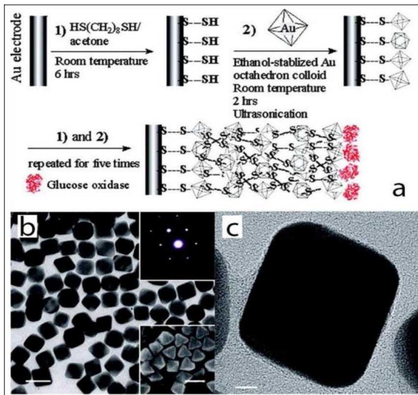
Figure 1.9 (a) Schematic representation of the stepwise construction of the gold nananoctahedra and glucose oxidase base biosensor, TEM images of gold nananoctahedra particles at (b) low and (c) high magnifications 62
