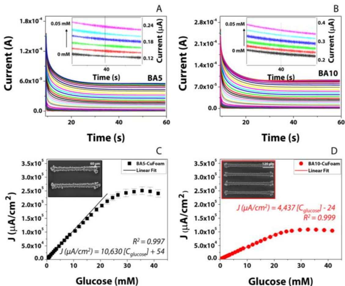
Figure 2.7. Chronoamperograms of the BA5-CuFoam (A) and BA10-CuFoam (B) sensors obtained in 0.1 \text{ M NaOH} solution as a function of increasing concentration of glucose at an applied potential of +0.45 \text{ V} (inset graphs show the magnified image of first six chronoamperograms at 40 th second), and corresponding calibration curves for the BA5-CuFoam (C) and BA10-CuFoam (D) sensors.
