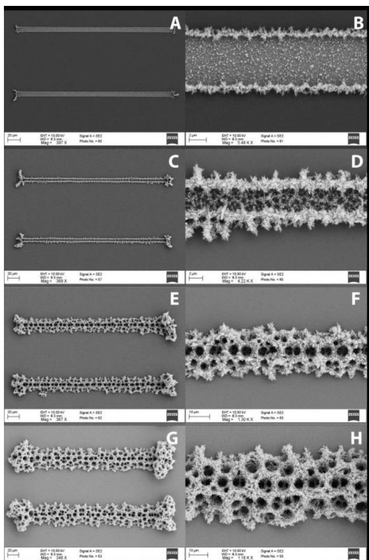
Figure 2.S2. SEM images of BA5-CuFoam electrodes prepared at different \text{Cu}^{2+} concentrations; (A,B) 0.05 mg \text{Cu}^{2+} /2.5 M \text{H}_2\text{SO}_4 , (C,D) 0.20 mg \text{Cu}^{2+} /2.5 M \text{H}_2\text{SO}_4 , (E,F) 0.50 mg \text{Cu}^{2+} /2.5 M \text{H}_2\text{SO}_4 and (G, H) 1.5 mg \text{Cu}^{2+} /2.5 M \text{H}_2\text{SO}_4 at a applied voltage of -5 V vs Ag/AgCl, deposition time is 20 seconds.
