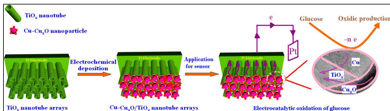
Figure 1.20 Schematic illustration of the preparation of the \text{Cu-Cu}_2\text{O}/\text{TiO}_2 NTA/Ti electrode and the electron transfer through the \text{Cu-Cu}_2\text{O}/\text{TiO}_2 TNA interface for the electrocatalytic oxidation of glucose 100
