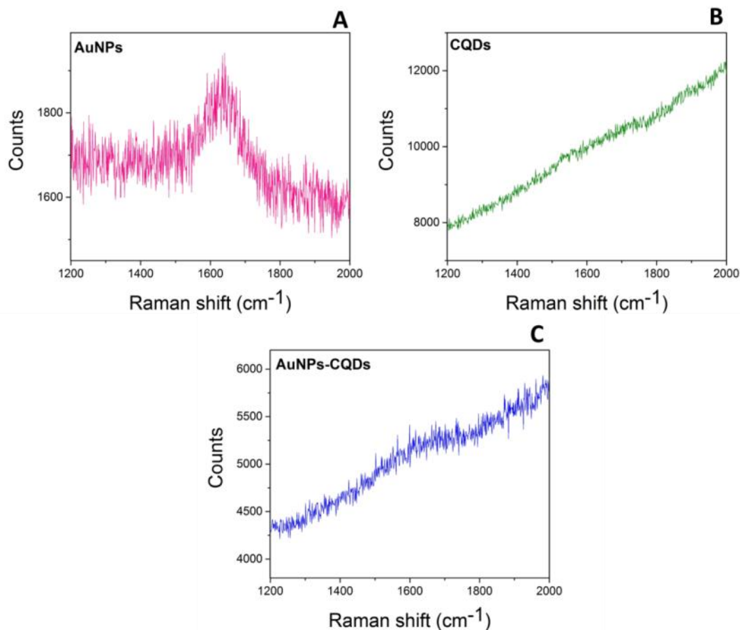
Figure 4.S1. Raman Spectrum of AuNPs (A), CQDs (B) and AuNPs-CQDs nanohybrid material (C)
