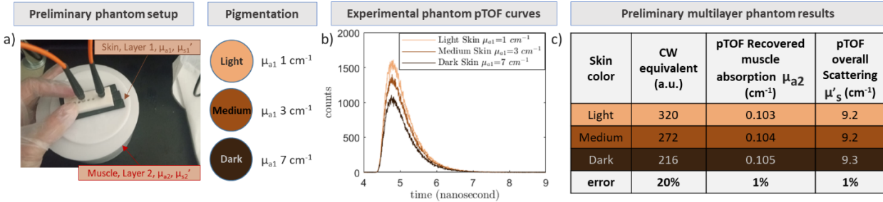
Fig. 2. Bias-free feasibility results on phantoms a) experimental setup of two-layer phantom and TDDOS probe b) pTOF curves of the two-layer phantom with changing skin color (light, medium, dark) layer c) preliminary bias-free extraction of deep layer absorption with varying skin pigmentation, changing the pigment of skin layer does not affect the estimated deep layer (muscle) absorption ( \mu_{a2} )
