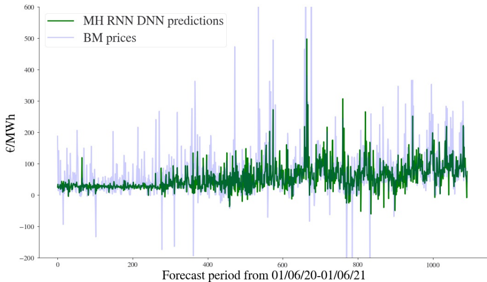
Figure 4.4: MH RNN DNN Forecasts for BM
