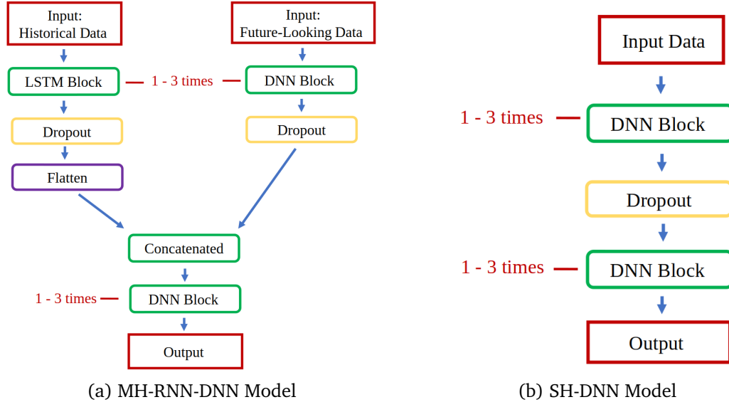
Figure 4.2: Comparison of the MH-RNN-DNN Model and SH-DNN Model.
