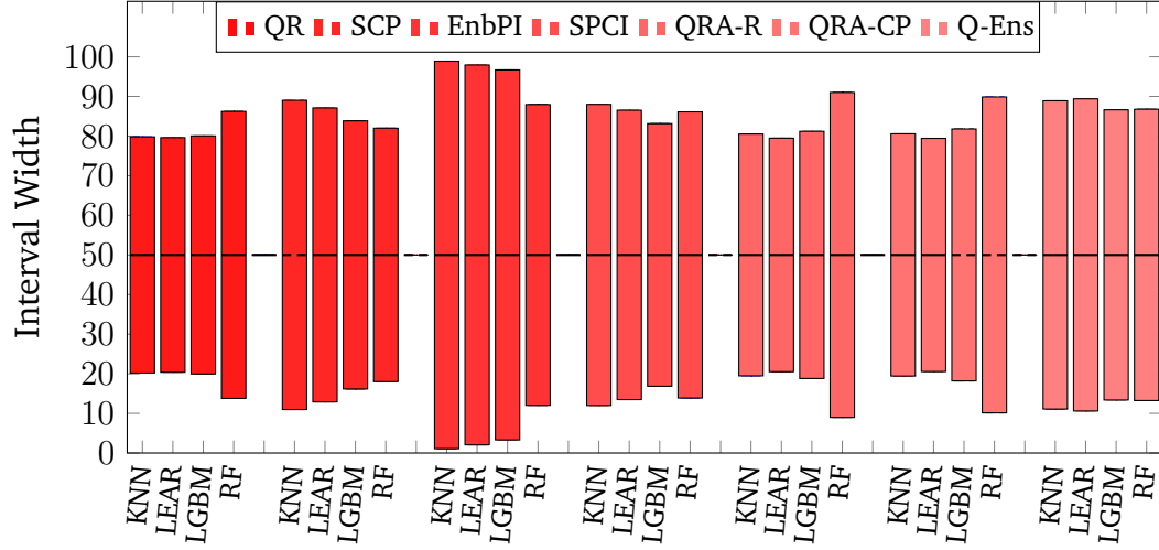
Figure 6.6: Interval Width for each model in the BM
