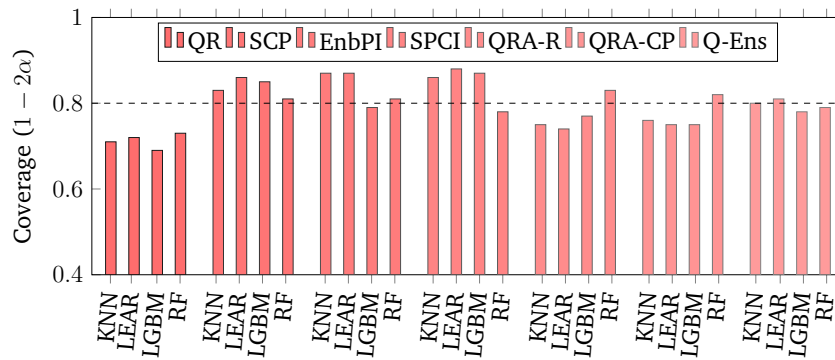
Figure 6.7: BM Coverage for 0.1-0.9 quantile pair
