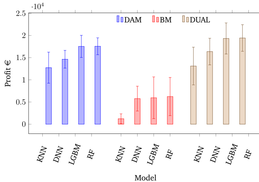
Figure 5.6: TS3 Profit for Models in the DAM, BM & Dual with Range in Quantile Pair Performance for each Model
