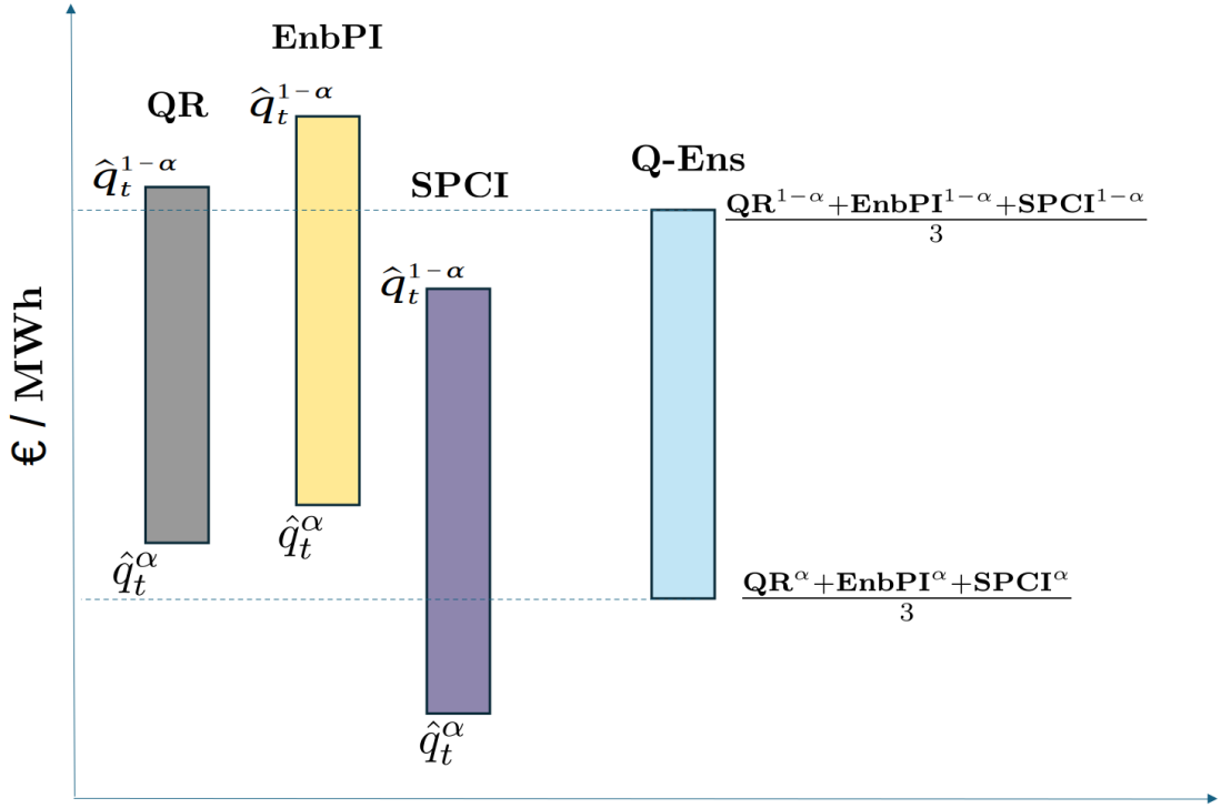
Figure 6.2: Construction of the Ensemble, Q-Ens.
