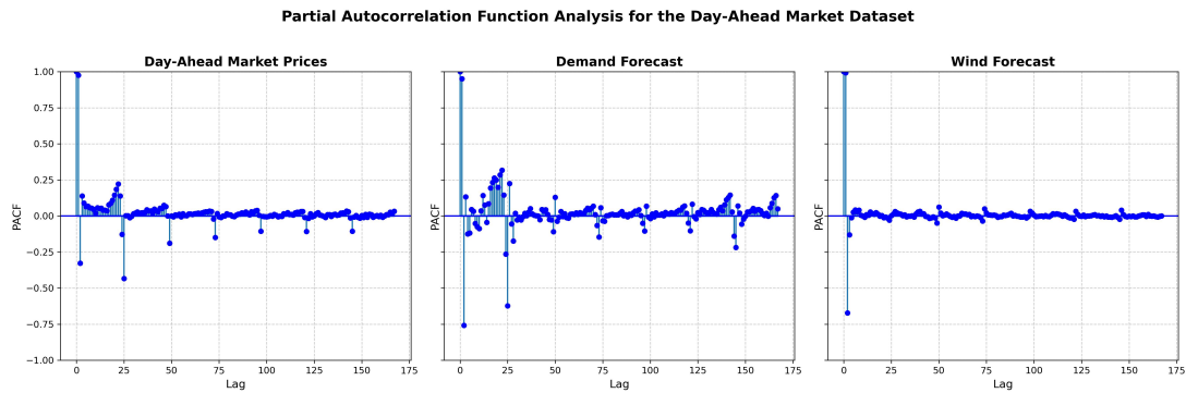
Figure 3.5: Partial Autocorrelation Plots for the DAM Prices and predictors
