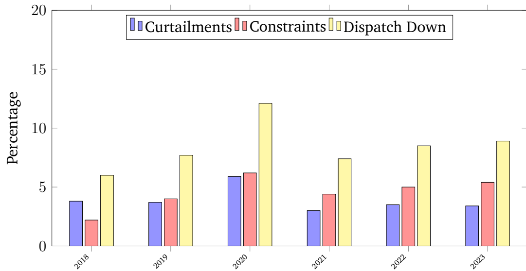
Figure 5.1: Annual percentages of curtailments, constraints, and dispatch down incidents, illustrating the impact of renewable energy challenges on wind output ([Eir23]).
