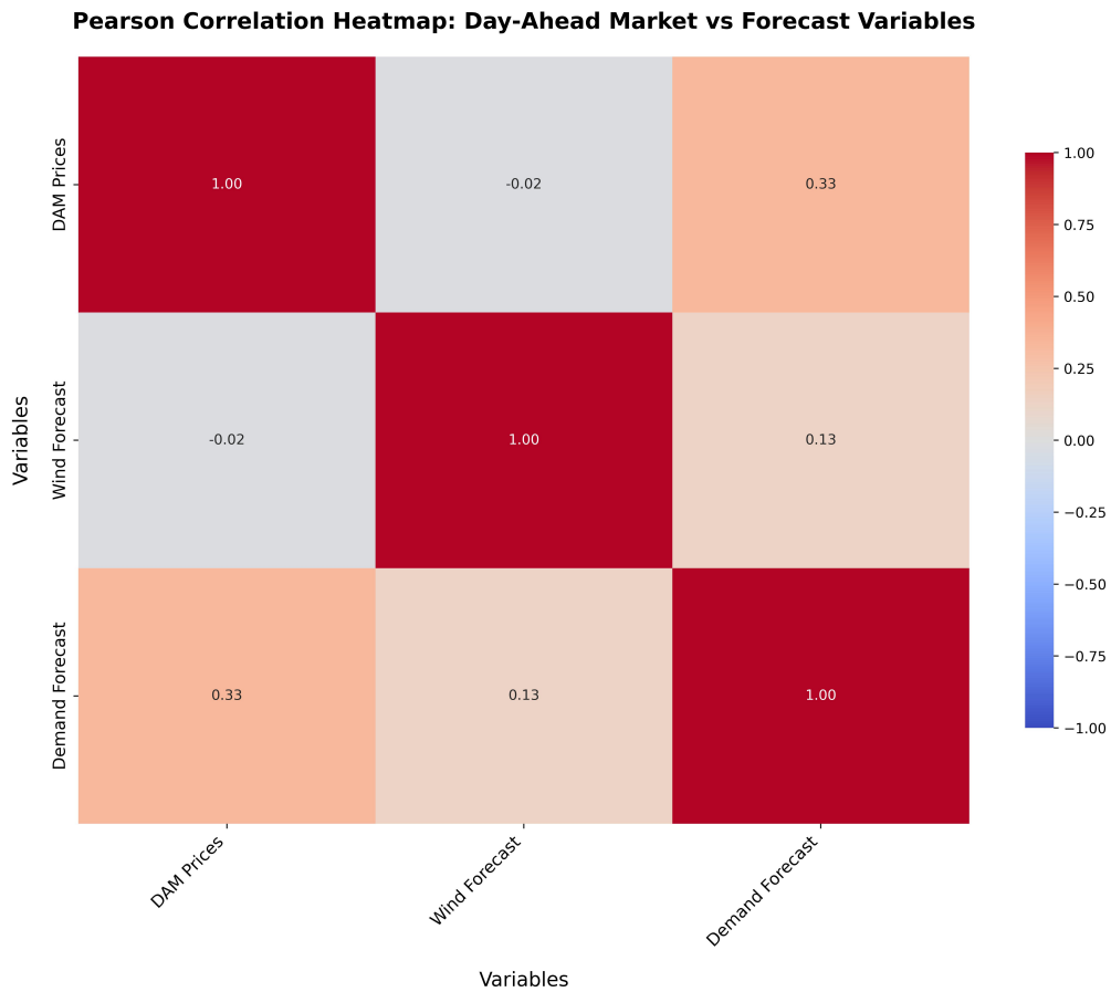
Figure 3.7: Pearson Correlation Plots for the DAM Prices and predictors
