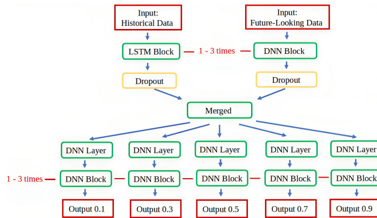
Figure 5.2: MH-RNN-DNN Model
