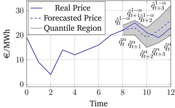
Figure 2.5: Quantile forecast of electricity prices
