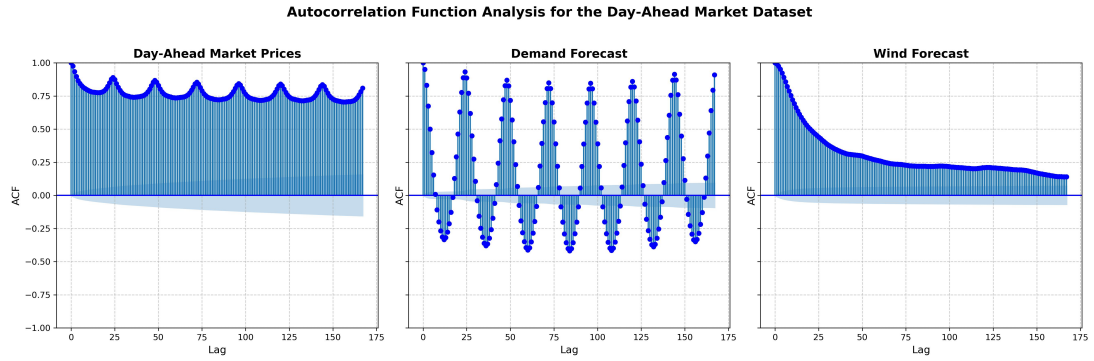
Figure 3.3: Autocorrelation Plots for the DAM Prices and predictors
