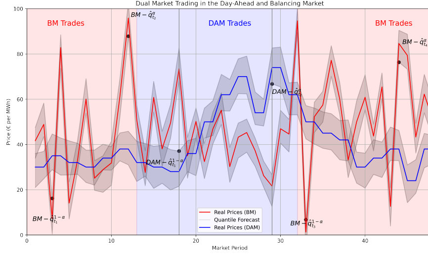
Figure 5.3: TS3-Dual Strategy
