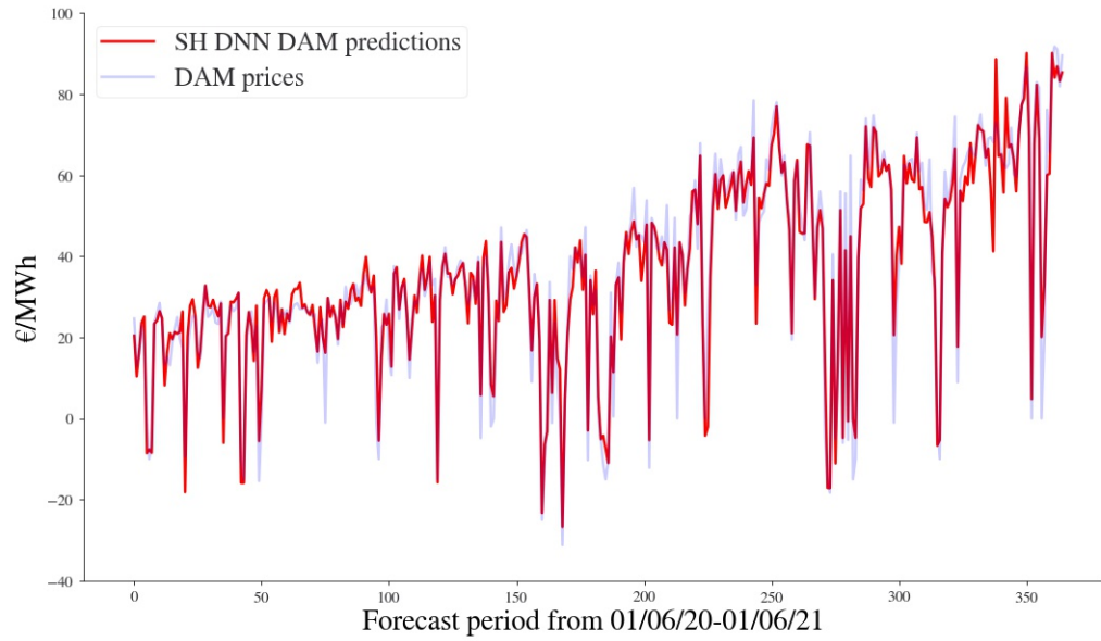
Figure 4.7: SH DNN Forecast for DAM
