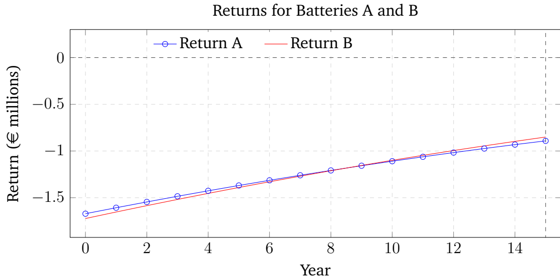
Figure 5.8: 15-year cost breakdown for the 3 MWh Scottish Power and 3.9 MWh Tesla capacity
