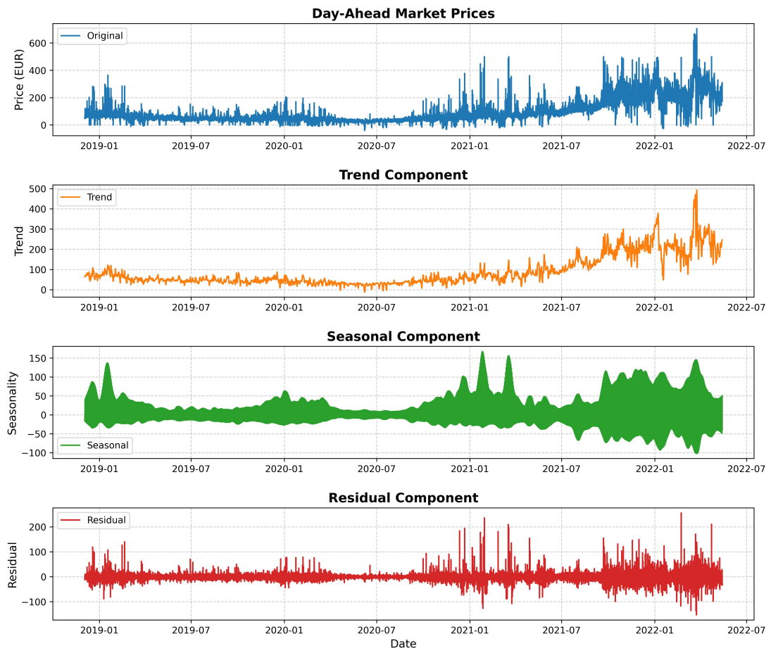
Figure 3.11: Seasonal and Trend Decomposition for DAM Prices
