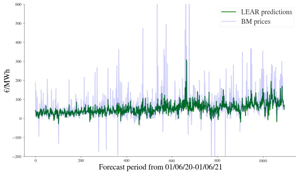
Figure 4.3: LEAR Forecast for BM
