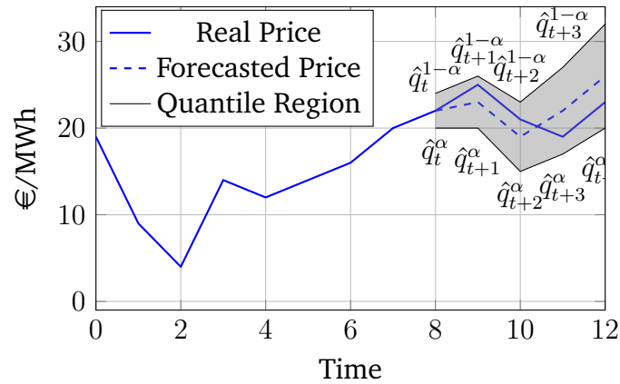
Figure 6.1: Quantile forecast of electricity prices
