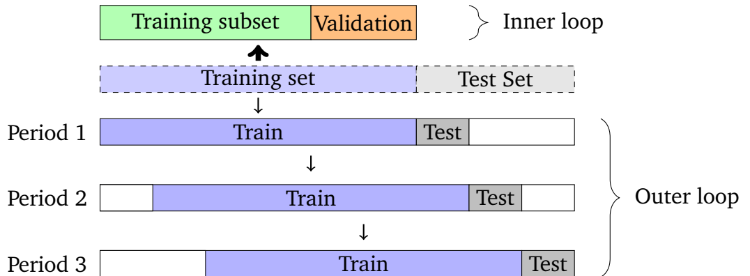
Figure 4.1: Rolling Walk-Forward Validation process for the first three periods in our experimental configuration.
