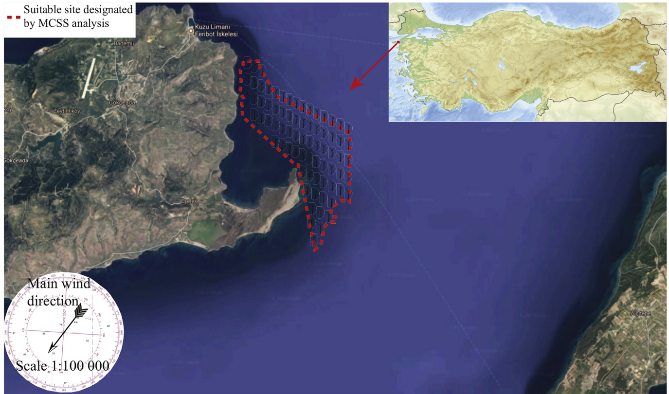
Fig. 10. The selected site and sitting of wind turbines at Gokceada shores (The map is adapted from Google Maps).
