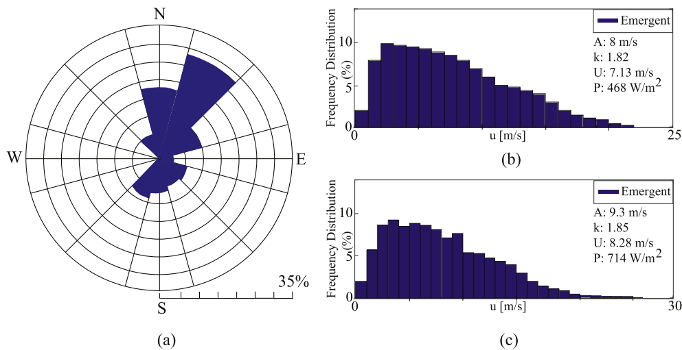
Fig. 5. WAsP analysis for Bozcaada a) frequencies (%) of wind direction b) frequency distribution of wind speed at 50 m c) frequency distribution of wind speed at 150 m.
