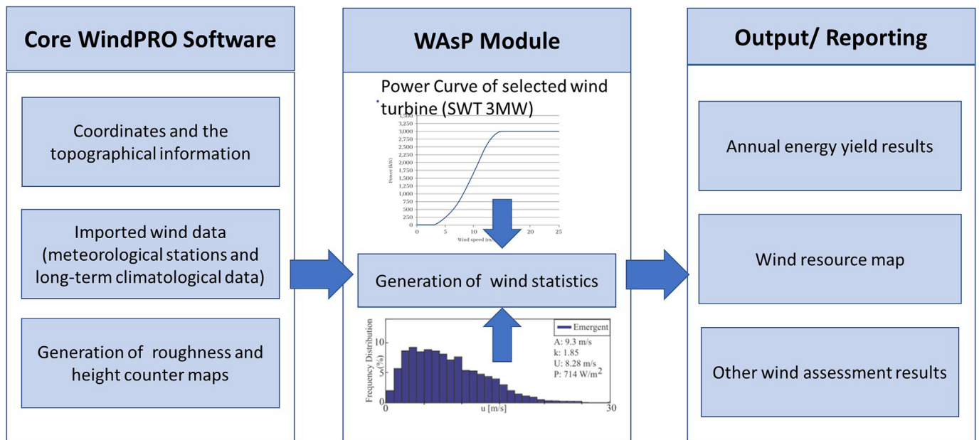
Fig. 2. Wind resource assessment using windPRO and WAsP.
