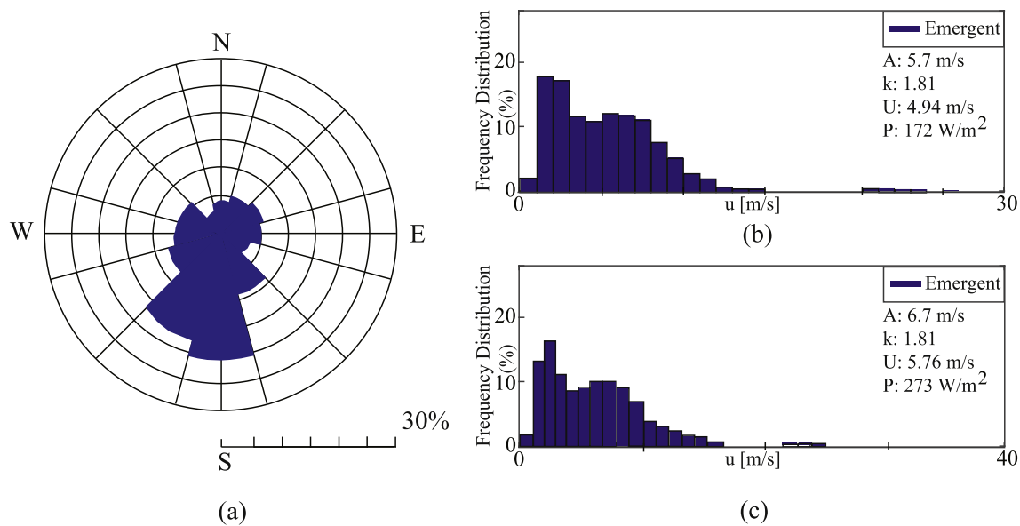
Fig. 11. (a) WASP analysis for Inebolu a) frequencies (%) of wind direction b) frequency distribution of wind speed at 50 m c) frequency distribution of wind speed at 150 m.
