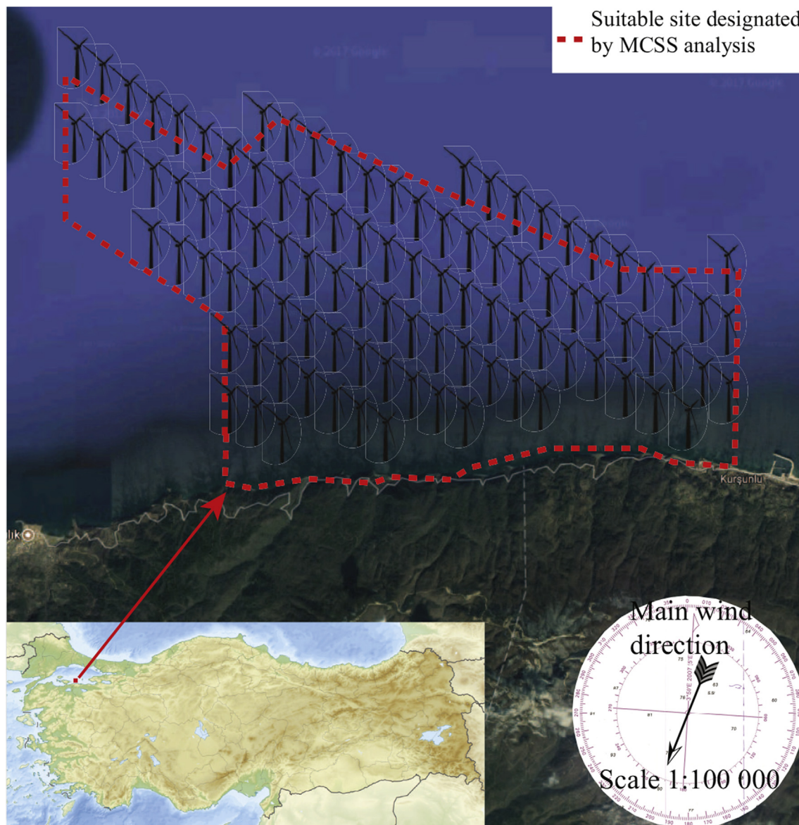
Fig. 8. The selected site and sitting of wind turbines at Bandirma shores (The map is adapted from Google Maps).
