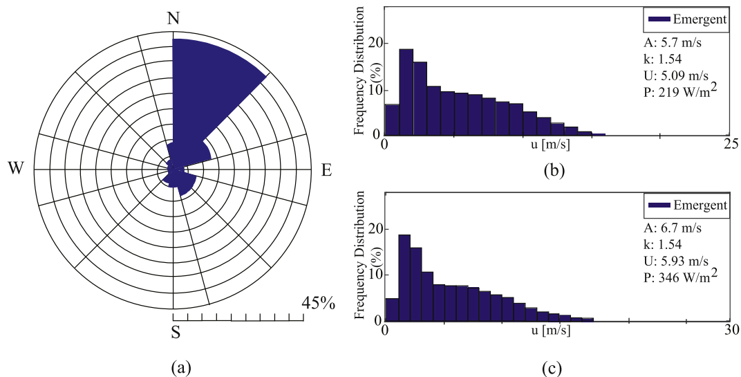
Fig. 7. WAsP analysis for Bandirma a) frequencies (%) of wind direction b) frequency distribution of wind speed at 50 m c) frequency distribution of wind speed at 150 m.
