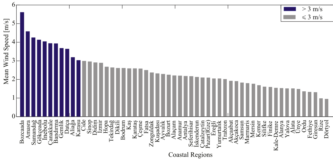
Fig. 3. Hourly mean wind speed of coastal regions at 10 m.
