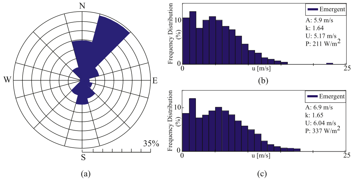
Fig. 9. WAsP analysis for Gokceada a) frequencies (%) of wind direction b) frequency distribution of wind speed at 50 m c) frequency distribution of wind speed at 150 m.
