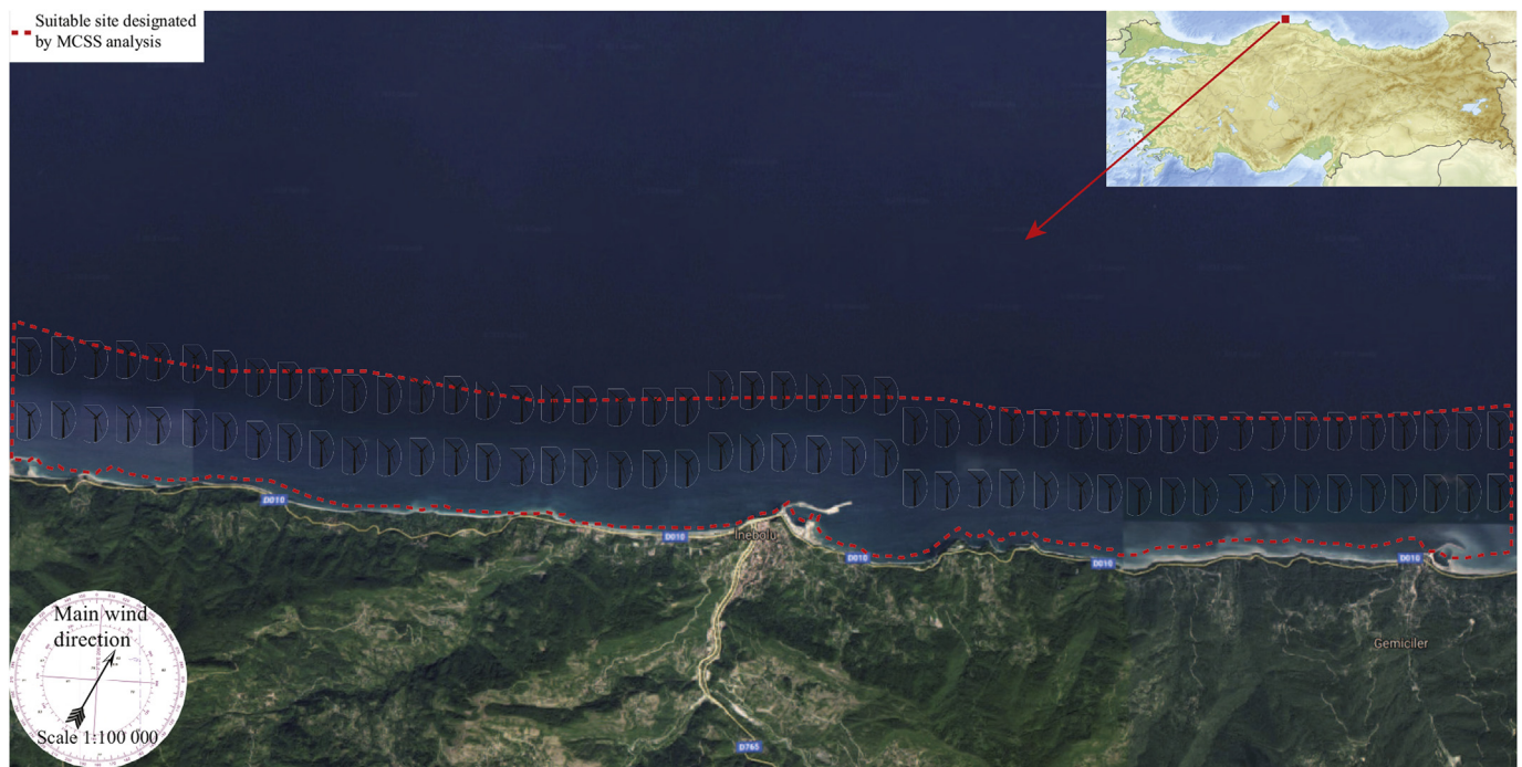
Fig. 12. The selected site and sitting of wind turbines at Inebolu shores (The map is adapted from Google Maps).
