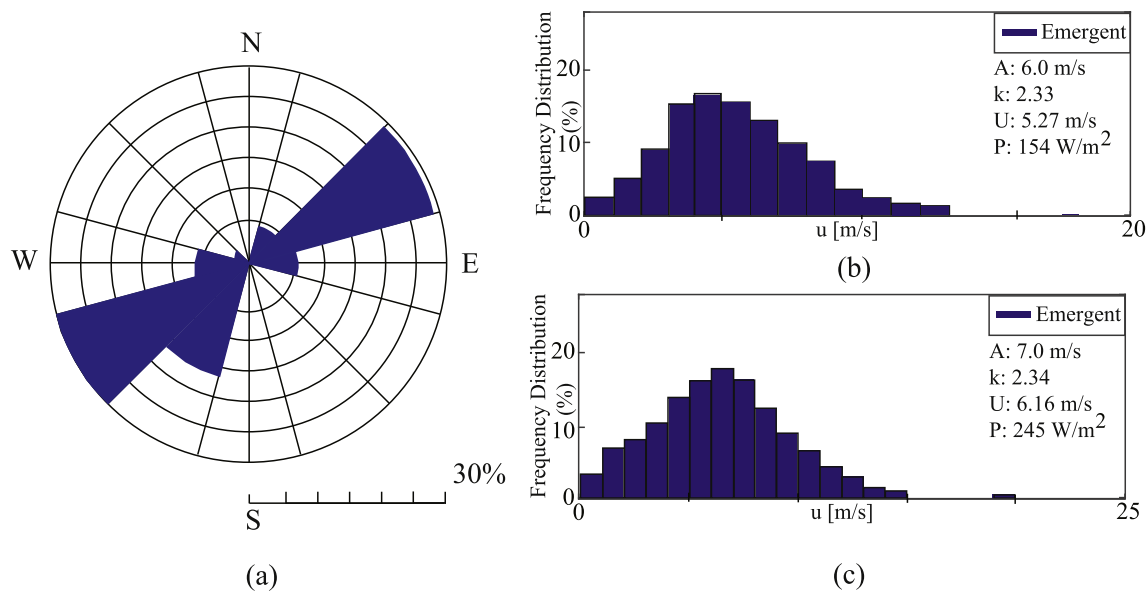
Fig. 13. WAsP analysis for Samandag a) frequencies (%) of wind direction b) frequency distribution of wind speed at 50 m c) frequency distribution of wind speed at 150 m.
