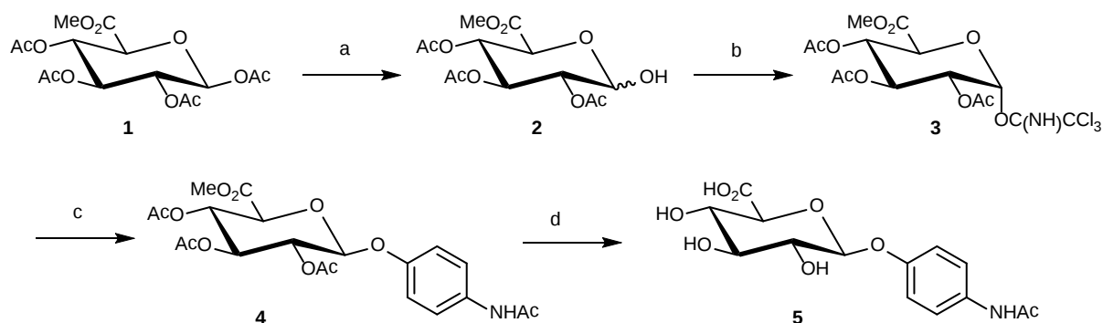
Scheme 1. (a) \text{Bu}_3\text{SnOMe} , \text{CH}_2\text{Cl}_2 , 87%; (b) \text{CCl}_3\text{CN} , DBU, \text{CH}_2\text{Cl}_2 , 65%; (c) paracetamol, \text{BF}_3\cdot\text{Et}_2\text{O} , \text{CH}_2\text{Cl}_2 , 76%; (d) 2 eq. \text{K}_2\text{CO}_3 in 5:5:1 \text{MeOH}:\text{THF}:\text{H}_2\text{O} , followed by Amberlyst ® 15 \text{H}^+ ion exchange resin, 47% (for sodium salt, Amberlyst ® 15 \text{H}^+ resin, then aq. \text{NaHCO}_3 soln, \text{MeOH} , 85%).
