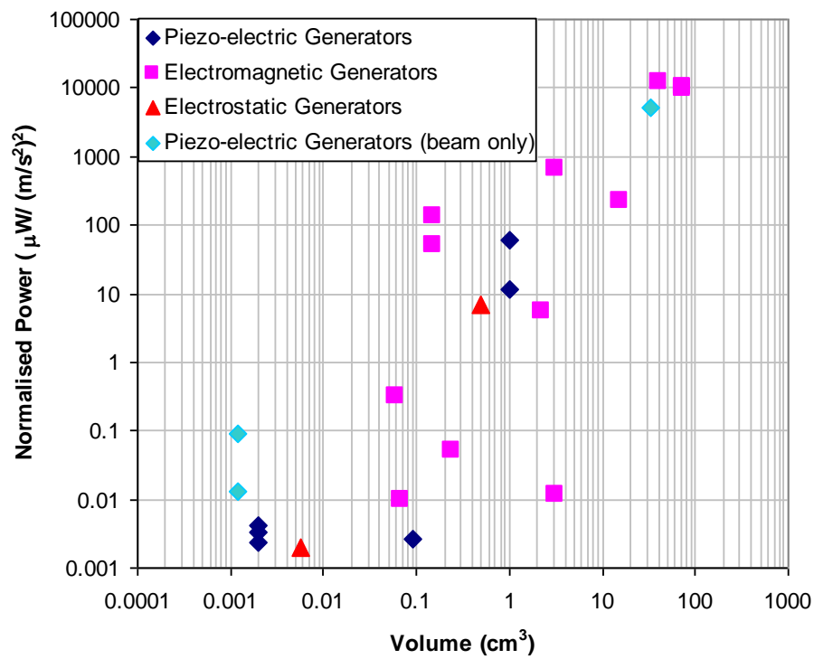
Figure 2(a): Power density of reported vibrational generators normalised to (1 m/s^2)^2 .
