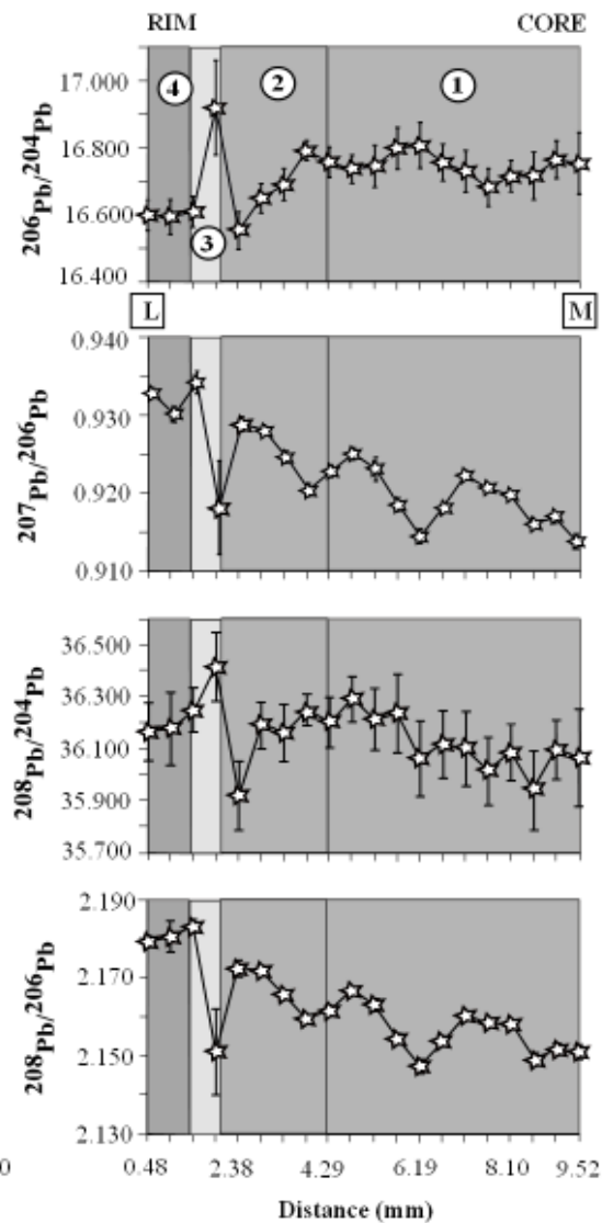
D - Pb-Pb MC-ICP-MS Laser traverse (L-M) 1-20
