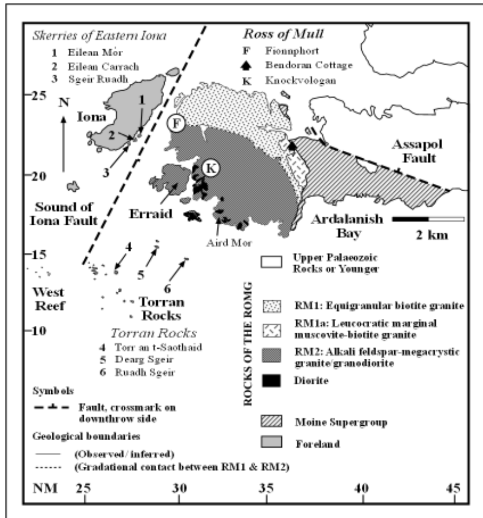
Fig. 3.1 Location and facies map of the ROMG (adapted from Zaniewski et al. 2006); place names are given for ease of use as when cited in the text.
