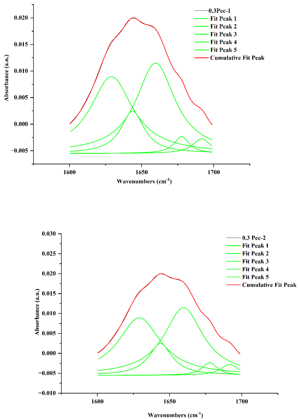
Fig. S3-1 and S3-2. Peak fitting of FTIR spectrum (Lorentz function) in the region of Amide I (1700–1600 cm -1 ) of mixture of 0.3 % HMP (w/w) and MFGs/MFGM
