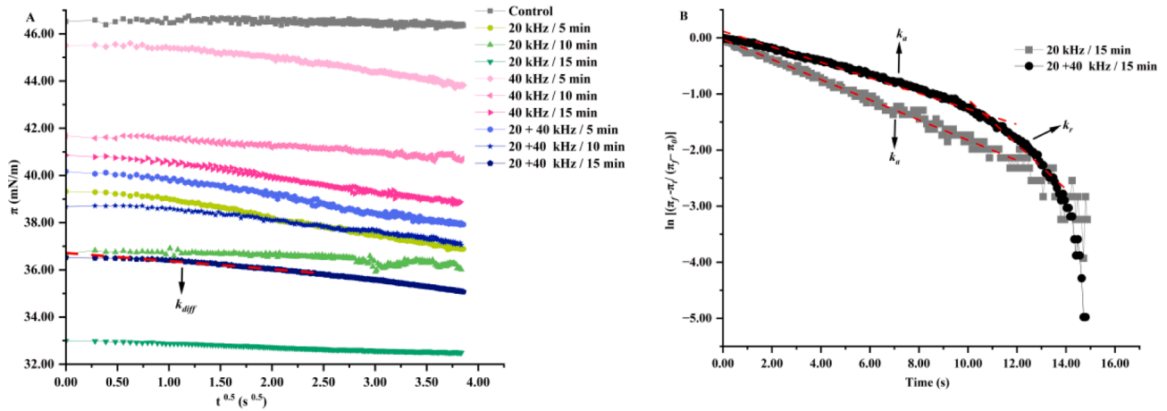
Fig. 5. (A) Interfacial tension ( \pi ) as a function of time ( t^{0.5} ) at the surface of sample droplets (control and samples treated at different ultrasonic intensities), k_{diff} is the diffusion rate. (B) The profile rate of protein adsorption and rearrangement for 20 kHz/ 15 min and 20 + 40 kHz/ 15 min samples, k_a and k_r are the first-order rate of adsorption (penetration) and rearrangement, respectively.
