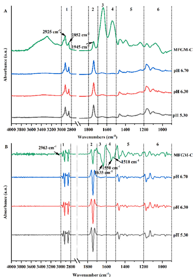
Fig. 2. Original (A) and representative second derivation (B) FTIR spectra of MFGs/MFGM from acidified bovine milk and sweet whey (MFGM-C) (Spectra between 2700 and 1900 \text{cm}^{-1} did not be shown because there was no peak was detected for all samples, and all the spectra exhibited the similar flat plots).
