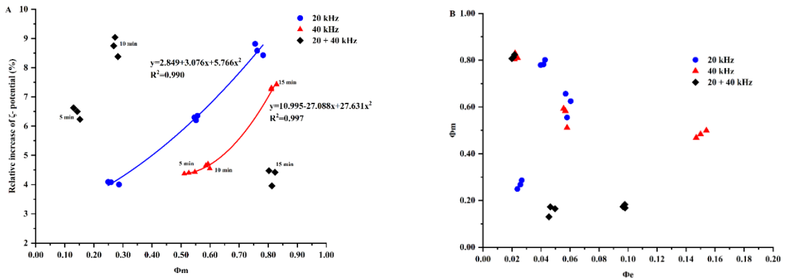
Figure 4-3. The relative increase of \zeta - potential ( \zeta_R ) for control and ultrasonicated samples as a function of measured surface fraction ( \Phi_m ) of MFGs/MFGM samples (A). Scatters of \Phi values by Mastersizer measurement ( \Phi_m ) and the predictive model estimated ( \Phi_e ) (Eq. (4)) (B).
