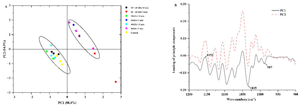
Fig. S9. PCA scores (A) and loading plots (B) of FTIR spectra in the region of 1200–900 \text{cm}^{-1} of MFGs/MFGM prepared from bovine raw milk treated by different ultrasonic intensities.
