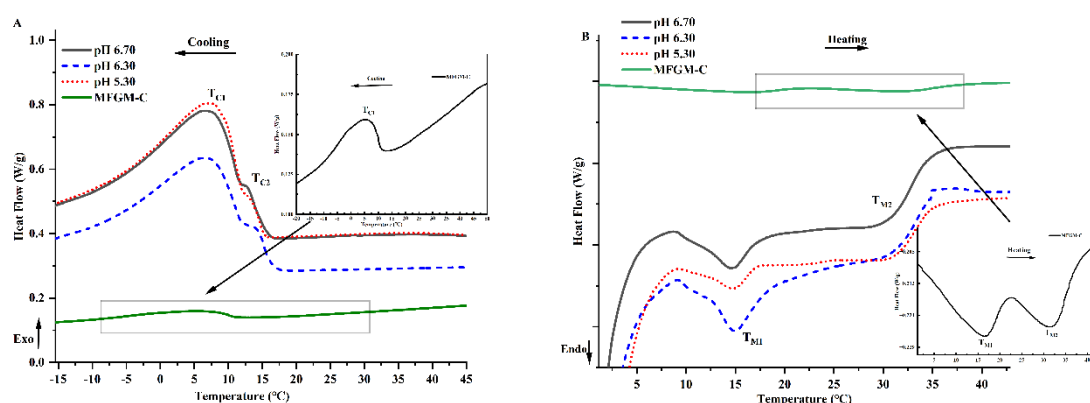
Figure 3-6. Crystallization (A) and melting (B) thermograms of MFGs/MFGM prepared from different pH bovine milk and sweet whey.
