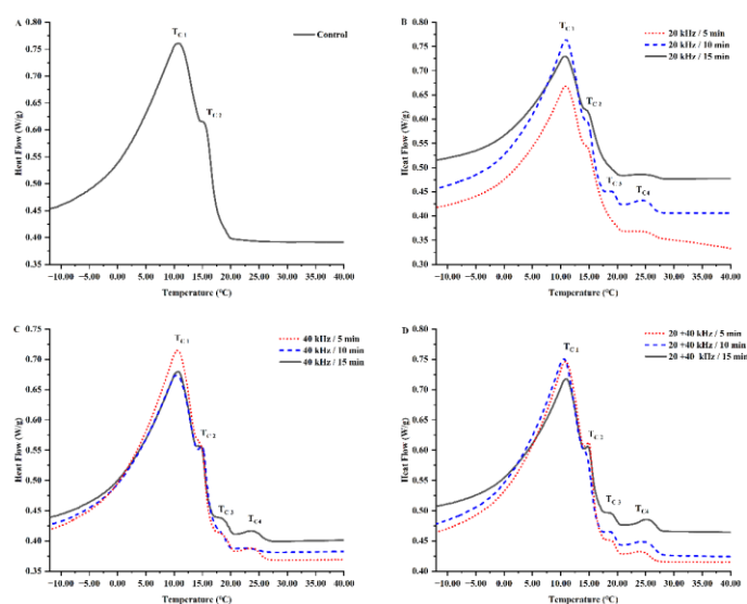
Figure 4-7. DSC crystallization thermograms of MFGs/MFGM samples separated from the control and ultrasonicated bovine milk, T_{C1} - T_{C4} are crystallization temperatures
