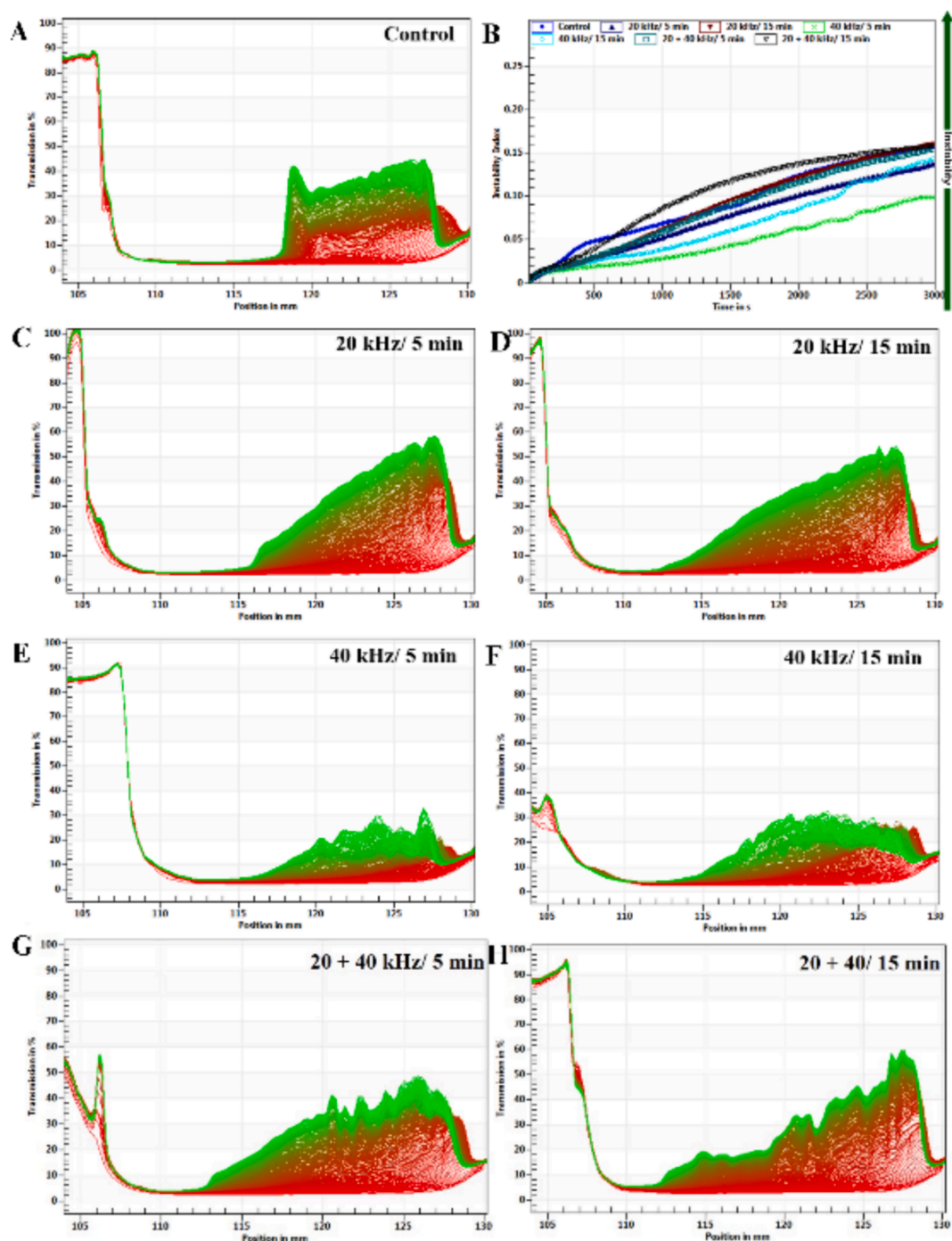
Fig. 4. Lumisizer phase separation near infrared (NIR) transmission profiles and instability index of MFGs/MFGM prepared from bovine raw milk treated by different ultrasonic intensities: A, control; B, instability index; C-D, 20 kHz treated for 5 min and 15 min; E-F, 40 kHz treated for 5 min and 15 min; G-H, Combined treatment using 20 kHz and 40 kHz for 5 min and 15 min.
