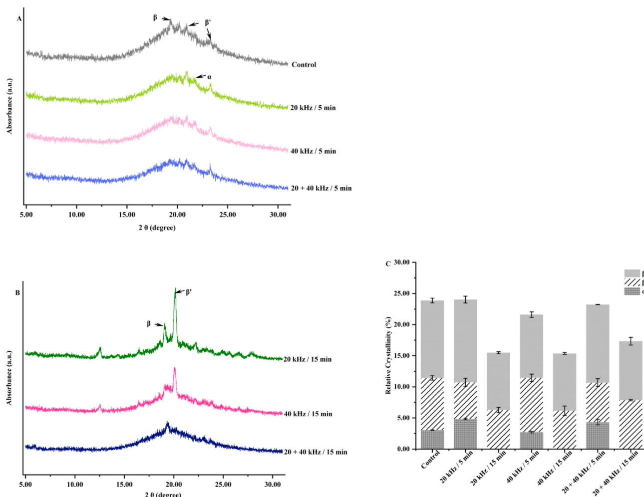
Fig. 6. X-ray spectra of control and ultrasonic-treated 5 min samples (A) and 15 min duration MFGs/MFGM samples (B); (C) relative crystallinity of \alpha , \beta , and \beta' crystals in MFGs/MFGM samples.
