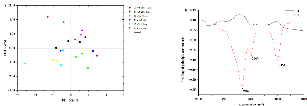
ig. S2. PCA scores (A) and loading plots (B) of FTIR spectra in the region of 3000–2800 \text{cm}^{-1} of MFGs/MFGM prepared from bovine raw milk treated by different ultrasonic intensities.
