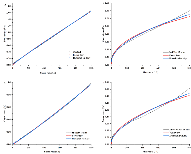
Fig. 5-4 Rheogram of MFGs/MFGM isolated from control (A), 20 kHz/ 15 min (B), 40 kHz/ 15 min (C), and 20 + 40 kHz/ 15 min (D) treated bovine milk showing the fitting by power law and Herschel-Bulkley models.
