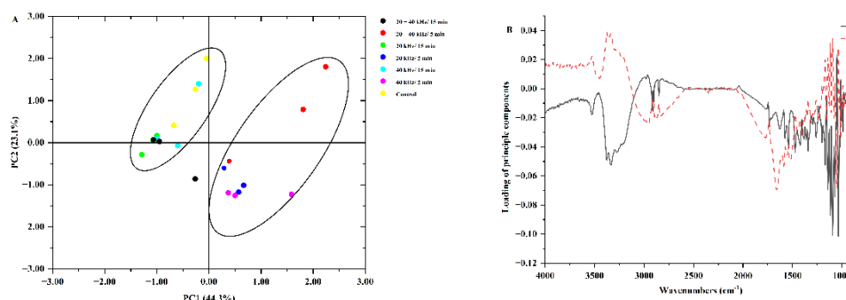
Fig. S1. PCA scores (A) and loading plots (B) of FTIR spectra in the region of 4000–900 \text{cm}^{-1} of MFGs/MFGM prepared from bovine raw milk treated by different ultrasonic intensities.
