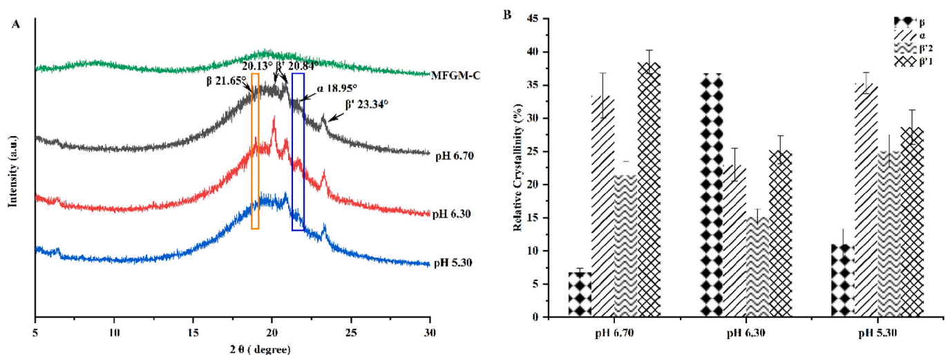
Fig. 5. XRD patterns (A) and the relative crystallinity (B) of \beta , \alpha , \beta'_2 , and \beta'_1 crystals in MFGs/MFGM isolated from different pH bovine milk or sweet whey. Relative crystallinity in MFGM-C was not shown because no crystal peaks were detected during the integration process.
