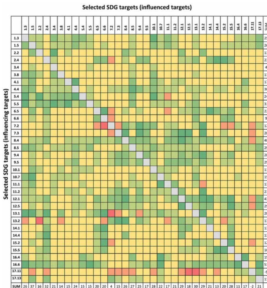
Figure 5.4. Example of a cross-impact matrix of 34 targets and their interaction in Sweden. Colour according to the scale in Figure 5.3 from dark red (−3/cancelling) to dark green (+3/indivisible). The net influence from a target on all other targets is shown by the row-sum and the column-sum shows how much a target is influenced by all other targets in total. Source: Weitz et al. (2018); licensed under CC BY 4.0 ( https://creativecommons.org/licenses/by/4.0/ ).
