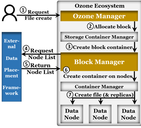
Fig. 4. Ozone Internal Working and Calling Placement Framework.
