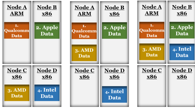
Fig. 2. Three possible solutions for the simplified data placement problem.
