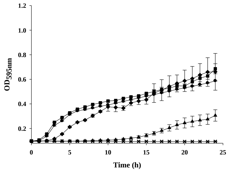
Fig. 7 Growth curve of lux -tagged E. coli in LB broth (●), plus 2% salt (■), 4% (◆), 6% (▲) and 10% (x) over 24 h of growth. Data are represented as OD 595nm millilitre \pm standard deviations.
