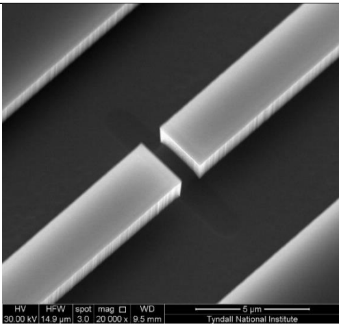
Fig 3: SEM images of the slotted ridge waveguide and a single slot.
