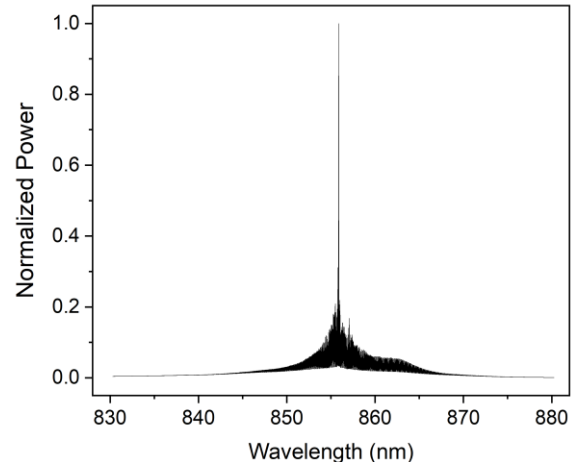
Fig 4: Output laser spectrum for a fixed gain, phase and mirror currents
