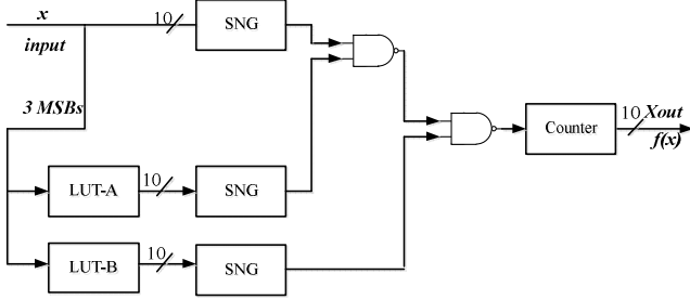
Fig. 3: The architecture of stochastic implementation of the functions \ln(1+x) , \tanh(x) , \text{sigmoid}(x) , \sin(x)
