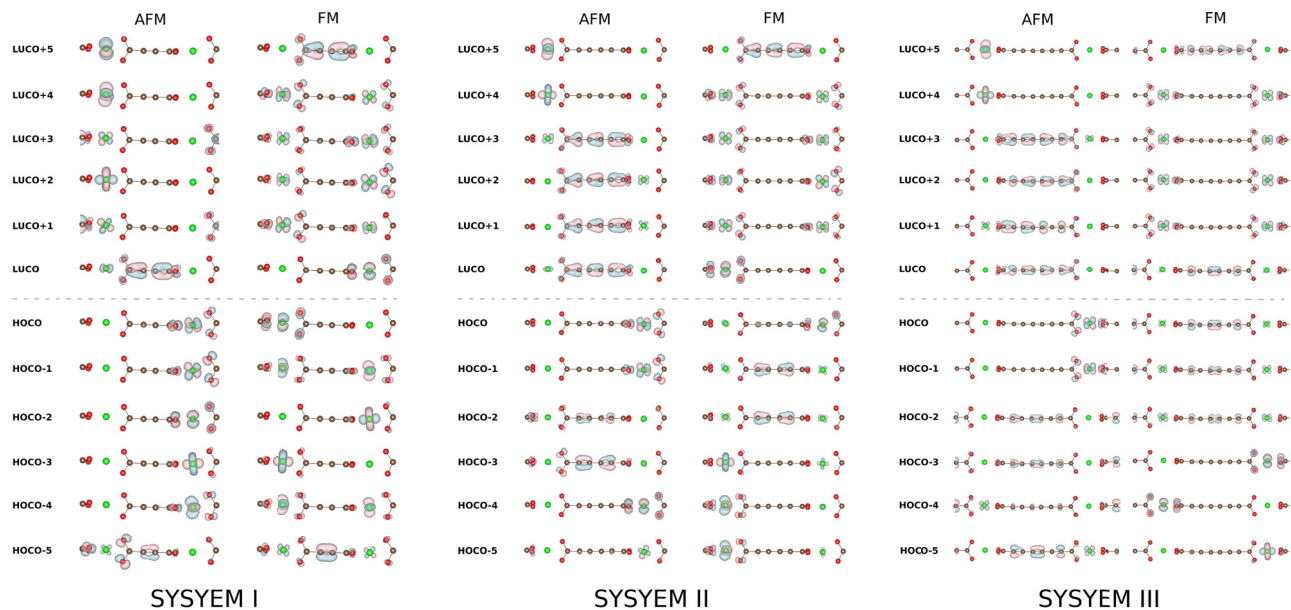
Figure S4: Frontier orbitals for the AFM and FM states for systems I (left), II (middle) and III (right). Isovalue = 5 \times 10^{-3} a.u. O = red, C = brown, Mn = green.
