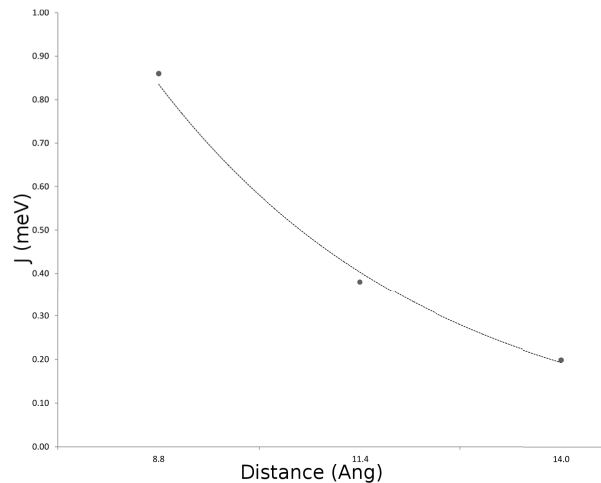
Figure S3: Exponential decay of the exchange energy vs d(\text{M-M}) . R^2 = 0.998 .
