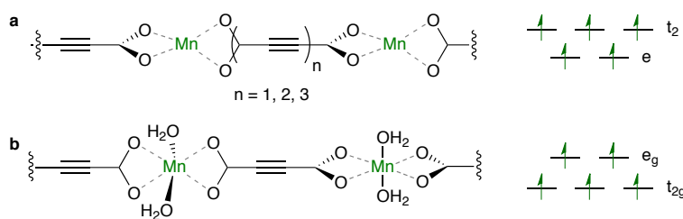
Figure S1: Schematic structures and ligand field splitting for Mn polymers with (a) tetrahedral and (b) octahedral coordination. The associated relaxed structure parameters are given in the tables below.
