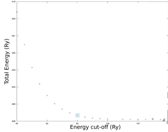
Figure S2: Plane-wave cut-off convergence for the norm-conserving pseudopotential with the PBEsol exchange correlation functional. A value of 80 Ry has been used in our production runs.
