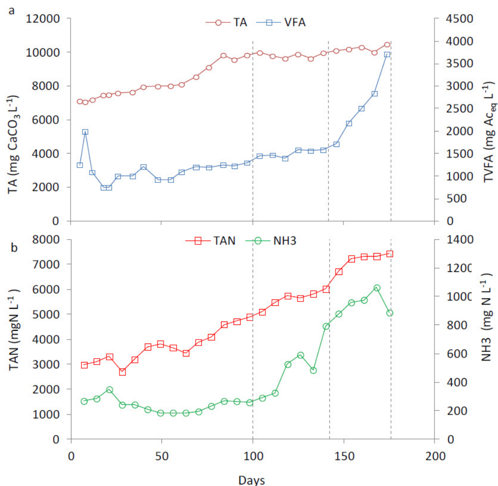
Figure 5 (a) Monitoring of total alkalinity (TA) and total volatile fatty acids. (TVFA) (b) total ammonia nitrogen (TAN) and free ammonia ( \text{NH}_3 ) in the semi-continuous trial.
