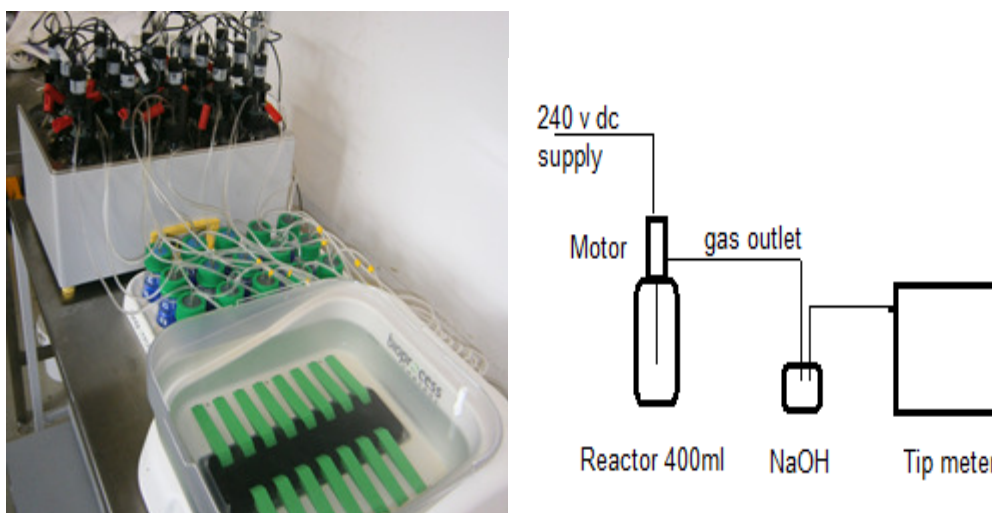
Figure 6.3 Biomethane potential test system.
