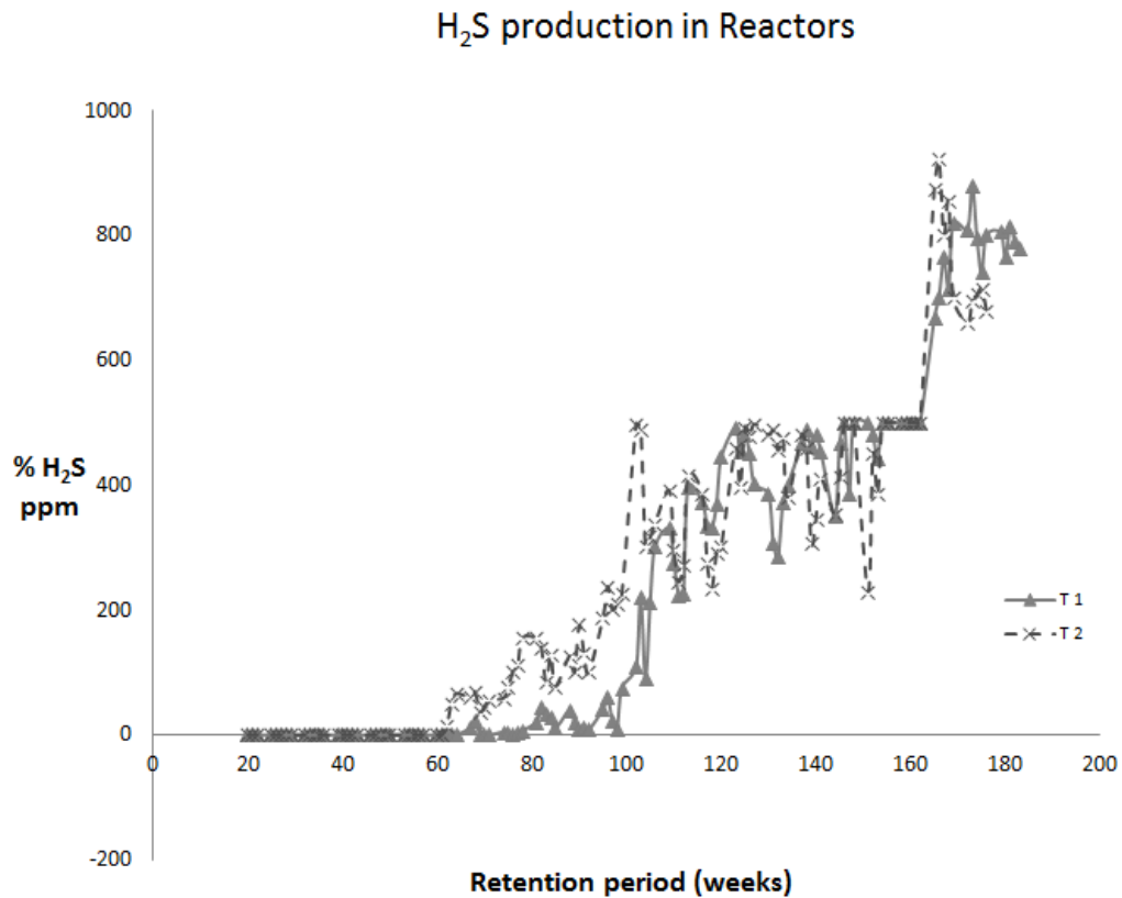
Figure 4.3 Levels of \text{H}_2\text{S} (ppm) in biogas from T1 and T2.
