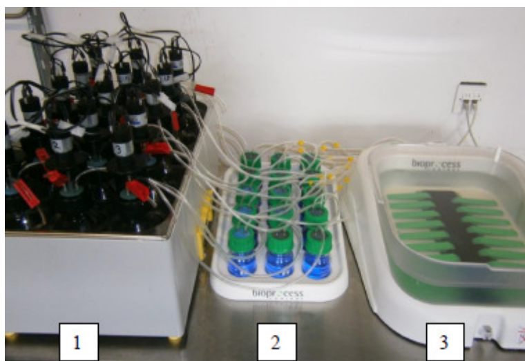
Figure 2 BMP apparatus used in the paper: Automatic Methane Potential Test
