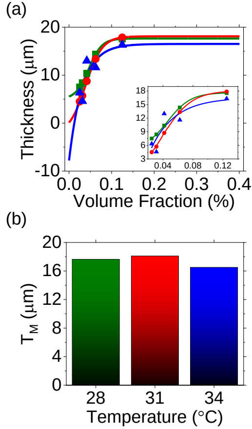
Figure 4.2. (a) Thickness volume fraction relationship for each evaporation temperature with sigmoidal Boltzmann fit function applied to an extended volume fraction range of 0 – 0.4%. Inset: Boltzmann function applied to volume fraction range of 0.025 – 0.125% as per experimental measurements. (b) Maximum thickness T_M for opals grown at each evaporation temperature based on the Boltzmann function.
