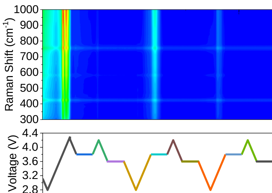
Figure S7.2. Full operando Raman spectroscopy colormap from chronoamperometric cycling of commercial NMC cathode in Li-ion half-cell from which the stages in Figure 7.6 of the main text were extracted. Synchronised voltage profile below.
