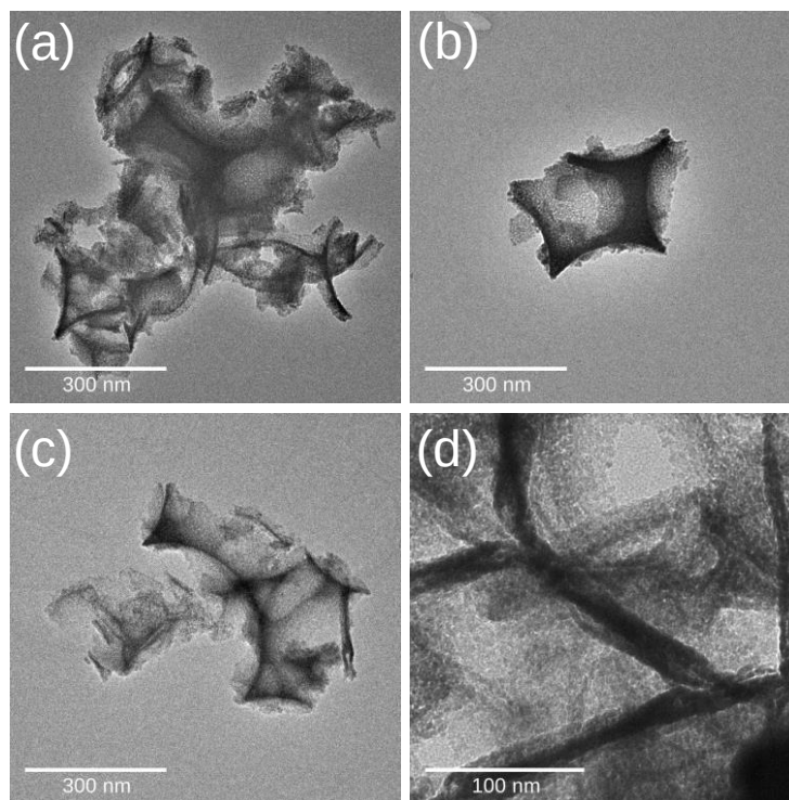
Figure S6.2: Additional TEM images of the \text{SnO}_2 shown in the main text. (a)-(c) Various IO fragments at 300 nm resolution. (d) Magnification of thin pore wall at 100 nm resolution.
