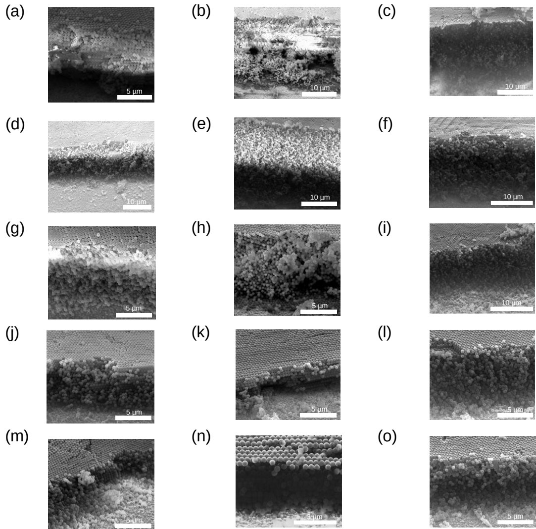
Figure S4.2. Cross-sectional SEM images of opals as examples used for thickness measurements provided to establish relationship with volume fraction. Evaporation temperatures are 28 °C, 31 °C, 34 °C, increasing from columns 1-3. Sphere solution volume fractions: (a)-(c) 0.025 %, (d)-(f) 0.0625 %, (g)-(i) 0.042 %, (j)-(l) 0.031 %, (m)-(o) 0.025 %.
