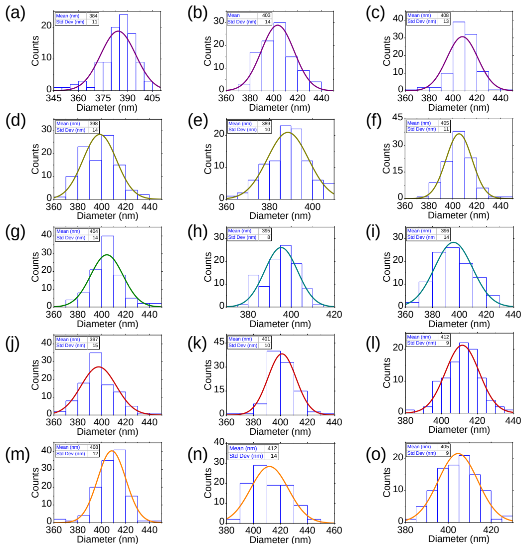
Figure S4.5. Size distributions for opals grown from sphere solutions with a nominal sphere diameter of 370 nm. Evaporation temperatures are 28 °C, 31 °C, 34 °C, increasing from columns 1-3. Sphere solution volume fractions: (a)-(c) 0.125%, (d)-(f) 0.063% (g)-(i) 0.042%, (j)-(l) 0.031%, (m)-(o) 0.025%.
