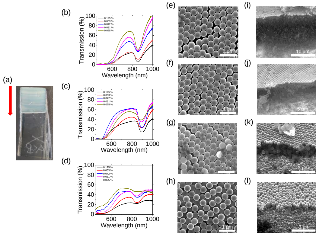
Figure 5.1. Optical and structural characterisation of opals grown by EISA at an evaporation temperature of 34 °C. (a) Photograph of opal sample. Opal thickness decreases in the direction of the red arrow. Optical transmission spectra for five opals, denoted by their volume fractions from 0.025 % to 0.125 %. (b) Spectra obtained at an angle of -25°, corresponding to a location near the tail of the red arrow. (c) Spectra obtained at normal incidence, near the centre of the sample. (d) Spectra obtained at an angle of 25°, at a location near the head of the red arrow. (e)-(g) SEM images obtained normal to the stacking direction at four positions along the direction of the red arrow shown in (a). (i)-(l) Corresponding cross-sectional SEM images obtained at four positions along the direction of the red arrow in (a) captured at an angle of 45° to the stacking direction.
