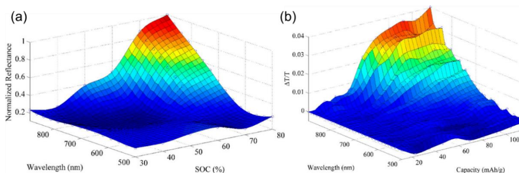
Figure 2.15. (a) In-situ optical reflectance measurements of lithiated commercial graphite electrodes at various states of charge. (b) Operando optical transmission measurements of graphite electrodes during lithiation. Adapted from ref. (168). Copyright ACS 2016.
