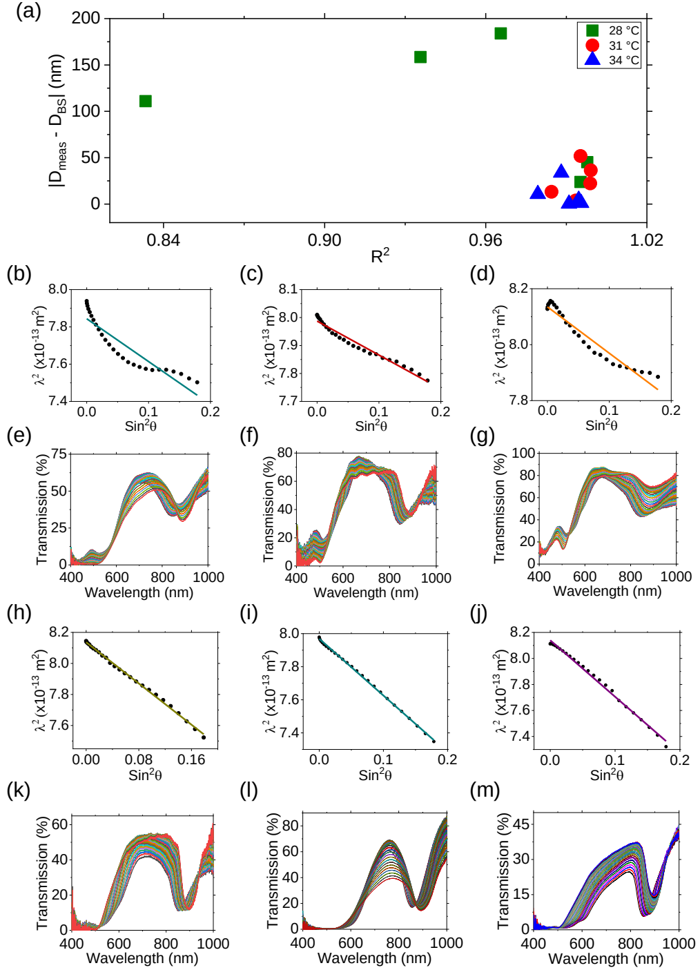
Figure 4.3. (a) Agreement between experimentally measured sphere diameters and those calculated according to Eq. 4.3 as a function of the R^2 value of the corresponding linear fits for opals grown from all five volume fractions at each of the three evaporation rates. (b)-(d) Bragg-Snell plots based on the central frequencies of the primary transmission dips observed in the transmission spectra for opals grown by EISA at an evaporation temperature of 28 °C from sphere solution volume fractions of 0.063%, 0.042%, and 0.025% respectively, the three outlier cases for which the Bragg-Snell relationship breakdown occurs.
