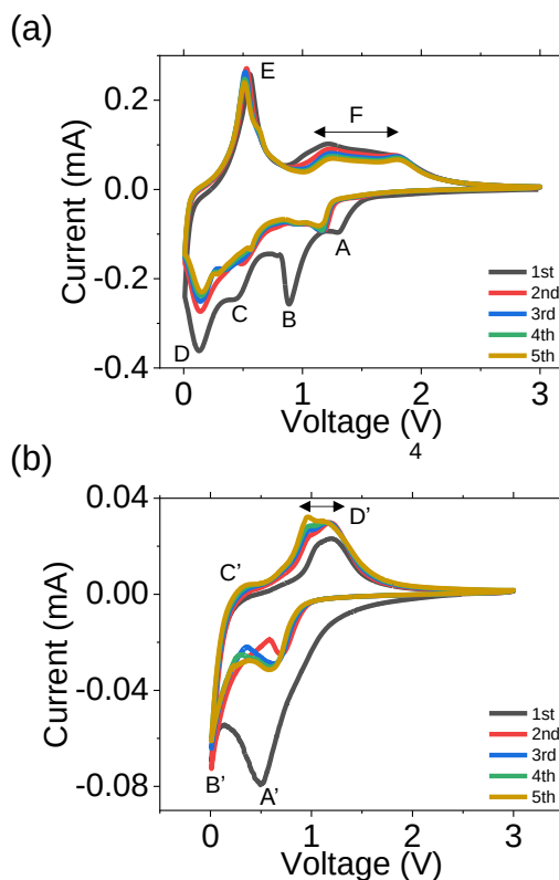
Figure 6.4. Cyclic voltammetry curves obtained over 5 cycles for SnO 2 IO in (a) Li-ion system and (b) a Na-ion system in a potential window of 0.01 V to 3.0 V at a scan rate of 0.1 mV s -1 . The electrode was initially swept from 3.0 V to 0.01 V in each case.
