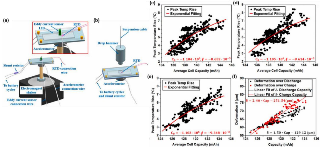
Figure 2.26. Operando testing platform for LIBs: (a) setup for operando vibration test, and (b) setup for operando impact test analysis. Relation between maximum temperature increase and capacity of (c) cell 1, (d) cell 2 and (e) cell 3. Relation between maximum deformation and capacity of cell 3. Adapted from ref. (246). Copyright Elsevier B.V. 2020.
