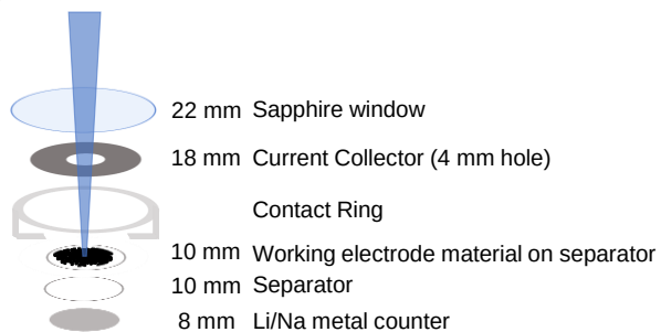
Figure 7.1: (a) Photograph of assembled EL-Cell-Opto-10 under Raman microscope. (b) Schematic of 'ring system' electrode stack. (c) Schematic of mesh electrode stack. (d) Schematic of coated separator electrode stack.
