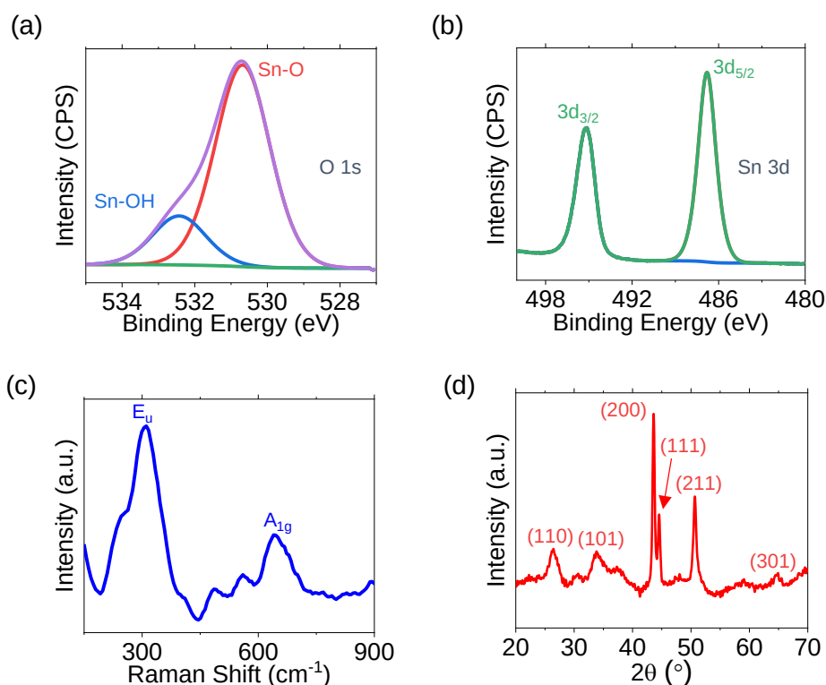
Figure 6.3. XPS core-level photoemission spectra of the (a) O 1s region and (b) Sn 3d region for a SnO 2 IO. (c) Raman scattering spectrum of SnO 2 IO. (d) XRD spectrum of SnO 2 IO showing reflections associated with tetragonal SnO 2 .
