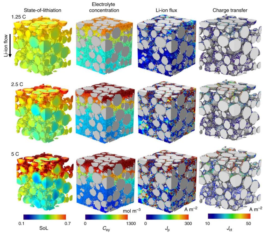
Figure 2.4. Simulated discharge of the reconstructed cathode and an ideal Li anode (half-cell) at 1.25, 2.5 and 5 C. The ionic current flows from the top (separator side) to the bottom (current collector side). Field variables at 50% depth-of-discharge (DoD) are shown here. Reproduced from ref. (46). Copyright Nature Publishing Group 2020.
