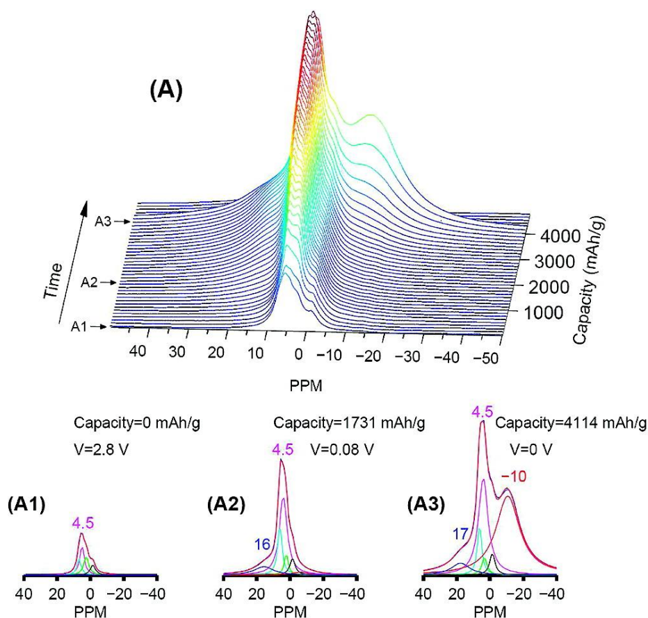
Figure 2.20. (A) Stacked plots of in-situ ^7\text{Li} static NMR spectra of the first discharge of an actual crystalline Si vs Li/Li ^+ battery (the colour bar shows the relative intensity scale for the spectra). (A1-A3) Deconvoluted spectra at various discharge capacity values of interest. Adapted from ref. (15). Copyright ACS 2009.
