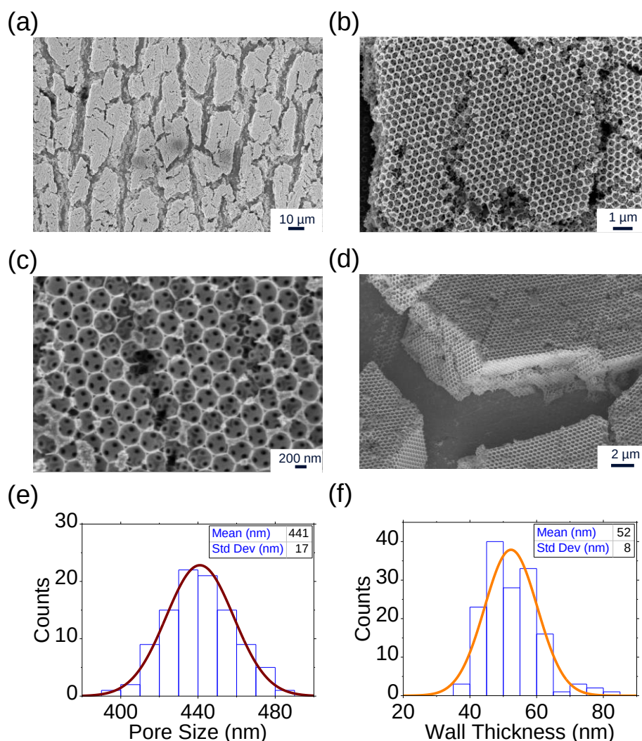
Figure 6.1. (a)-(c) Planview SEM images of SnO 2 IO at various levels of magnification. (d) Cross-sectional SEM image at a tilt angle of 30°. (e) Pore size distribution of SnO 2 IO obtained from SEM images. (f) Pore wall thickness distribution obtained from SEM images.
