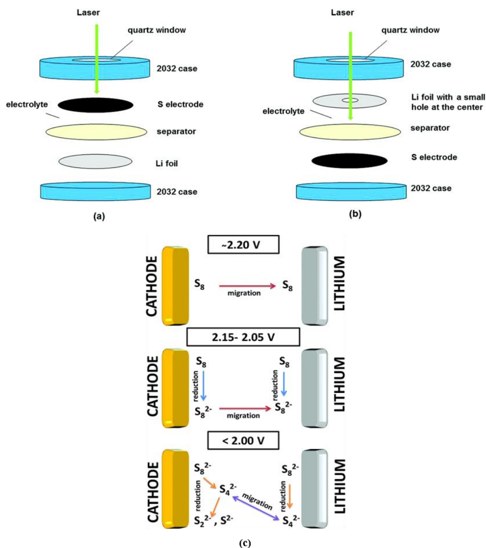
Figure 2.11. In-situ Raman cell designs for monitoring changes in (a) the cathode and (b) electrolyte near Li metal. (c) Schematic of the reduction process from in-situ Raman measurements at both the cathode and Li metal sides depicting the evolution of polysulfide species in a Li-S battery. Adapted with permission from ref. (98). Copyright RSC 2017.
