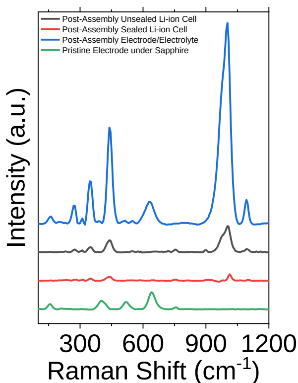
Figure S7.3. Ex-situ Raman spectra acquired from anatase TiO 2 slurry to show the effects of cell components and sealing on Raman signals: Pristine electrode under sapphire window (green), electrode post-assembly in sealed cell (red), electrode in unsealed cell post-assembly (grey), bare electrode with decomposed electrolyte species post-assembly.
