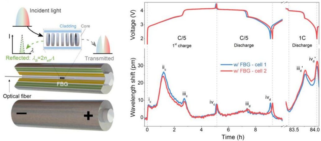
Figure 2.17. (Left) Schematic representation of the integration of optical fiber into a 18650 battery cell. (Right) The time-resolved voltage of the cell and spectral shift from the FBG for two separate cells over a single C/5 charge-discharge cycle and also after a discharge at 1 C. Spectral reflectance maxima 1 st charge at C/5. The wavelength shift is relative to the wavelength at time = 0 h on the 1 st charge at C/5. Adapted from ref. (192). Copyright Nature Publishing Group 2022.
