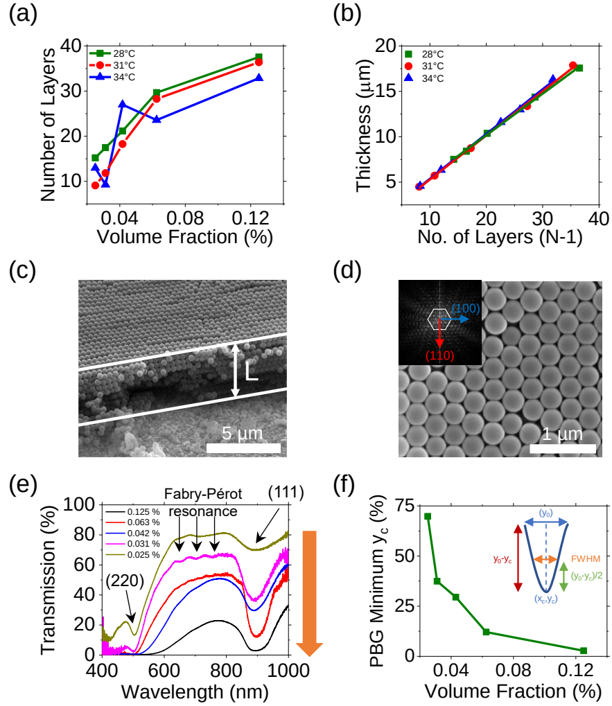
Figure 4.1. (a) Volume fraction-thickness relationship for opals grown from PS sphere solutions of five volume fractions at three evaporation temperatures. (b) Number of opal layers calculated using Eq. 4.1 as a function of measured sample thickness for samples formed under all investigated conditions. (c) Cross-sectional SEM image of representative opal demonstrating thickness measurement. (d) Plan view SEM image of surface of an opal grown from a volume fraction of 0.125 % at 28 °C. Inset: FFT with 2D hexagonal symmetry, the (100) and (110) directions labelled corresponding to the \Gamma -X and \Gamma -L directions of a 2D hexagonal lattice. (e) Transmission spectra obtained at normal incidence for opals grown from all five volume fractions at 28 °C. (f) Transmission intensity at the PBG centre as a function of volume fraction for all opals grown at 28 °C. Inset: Schematic illustrating the defining parameters of spectral transmission dips.
