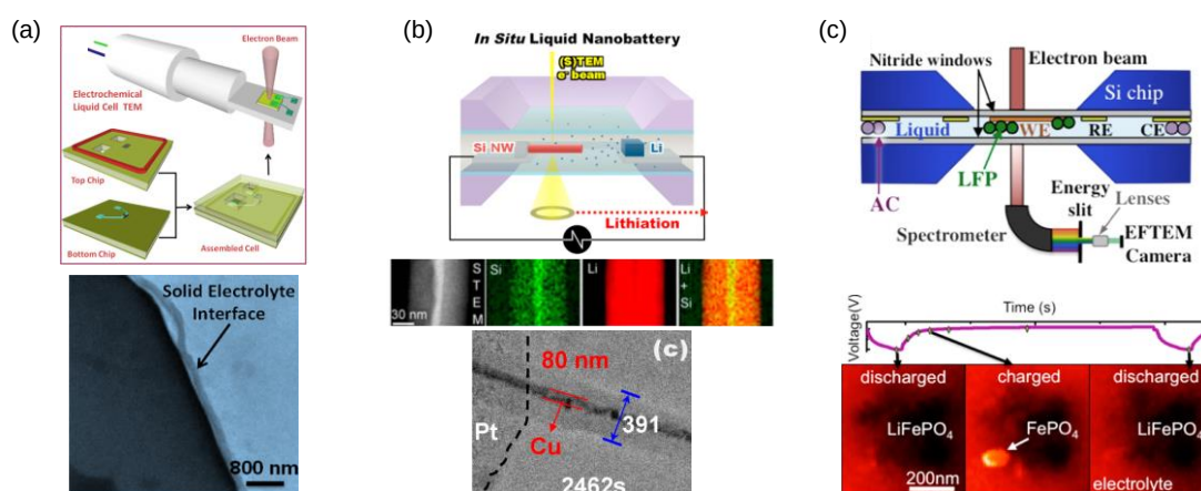
Figure 2.6. (a) Setup for in-situ liquid electrochemical cell to examine electrode-electrolyte interfaces. Adapted with permission from Nano Lett. 14, 1745 (2014). Copyright 2014 American Chemical Society. (b) A liquid electrochemical operando cell (Si NW electrode) using \text{SiN}_x membranes of \sim 50 nm in thickness to seal the liquid, while still allowing transmission of the high energy electrons for imaging. This liquid cell allowed elemental analysis and imaging of \text{Li}_x\text{Si} around a Si NW electrode. Adapted with permission from Nano Lett. 13, 6106 (2013). Copyright 2013 American Chemical Society. (c) \text{SiN}_x membraned liquid cell holder to allow operando EFTEM of \text{LiFePO}_4 cathodes. Adapted with permission from Nano Lett. 14, 1453 (2014). Copyright 2014 American Chemical Society.
