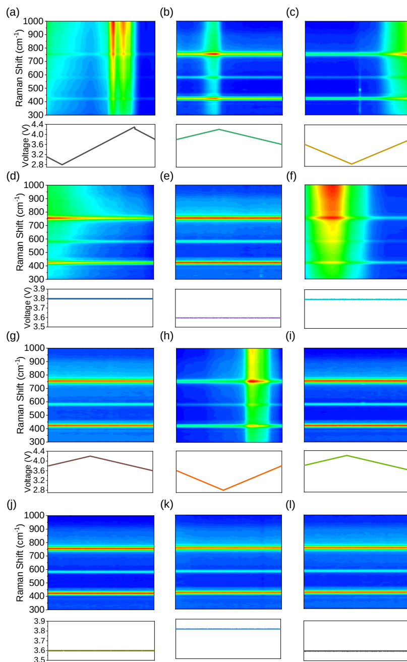
Figure 7.6: Operando Raman spectroscopy from chronoamperometric cycling of commercial NMC cathode in Li-ion half-cell at a specific power of 20 mW. For each stage, colormaps are presented with the associated time-voltage profiles below. For the colormaps, the x and y axes represent time versus Raman shift, while the colour represents Raman intensity. Spectra were acquired every 5 mins. Chronoamperometry was performed over six stages, each consisting of a potential sweep step shown in (a)-(f), followed by a fixed potential step (g)-(l). Note 1: Background subtraction has not been performed. Note 2: A colour scale is applied to the colormaps from each individual stage of the chronoamperometric experiment based on the maximum and minimum intensities during that stage to enhance visualisation of detected changes.
