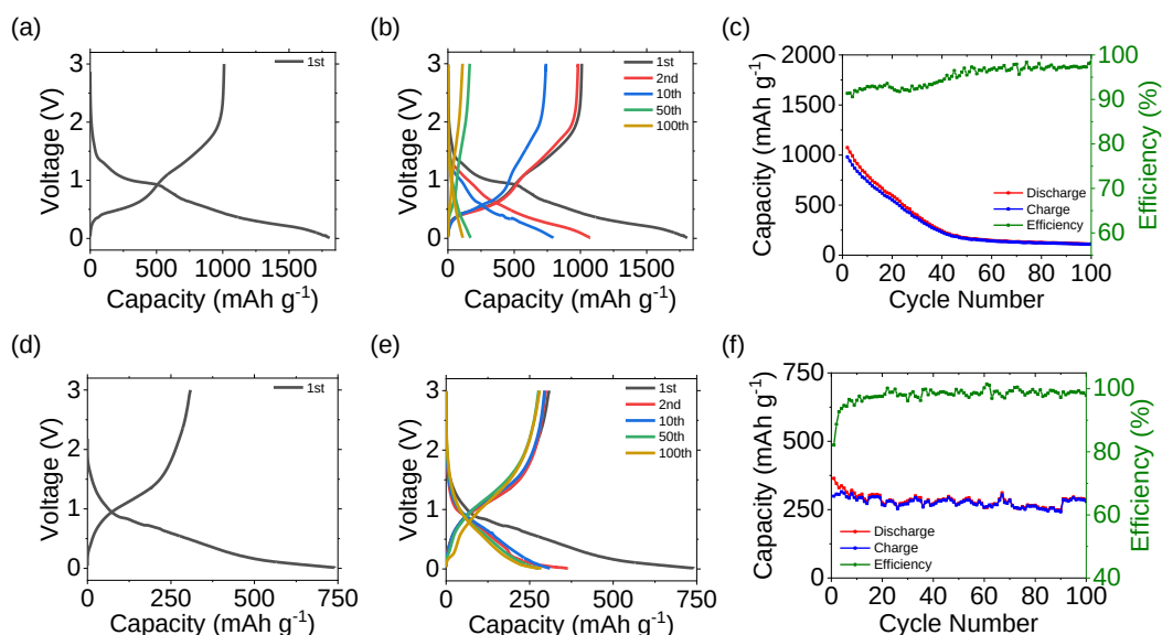
Figure 6.5. Galvanostatic cycling for a SnO 2 IO in a Li-ion half-cell at a specific current of 50 \text{ mA g}^{-1} showing (a) charge and discharge voltage profiles for first cycle, (b) a range of select charge discharge profiles up to the 100 th cycle and (c) specific capacity and coulombic efficiency (CE) as a function of cycle number. Galvanostatic cycling results for a SnO 2 IO in a Na-ion half-cell at a specific current of 50 \text{ mA g}^{-1} showing (d) charge and discharge voltage profiles for first cycle, (e) a range of select charge discharge profiles like the Li-ion half-cell and (f) specific capacity and coulombic efficiency as a function of cycle number.
