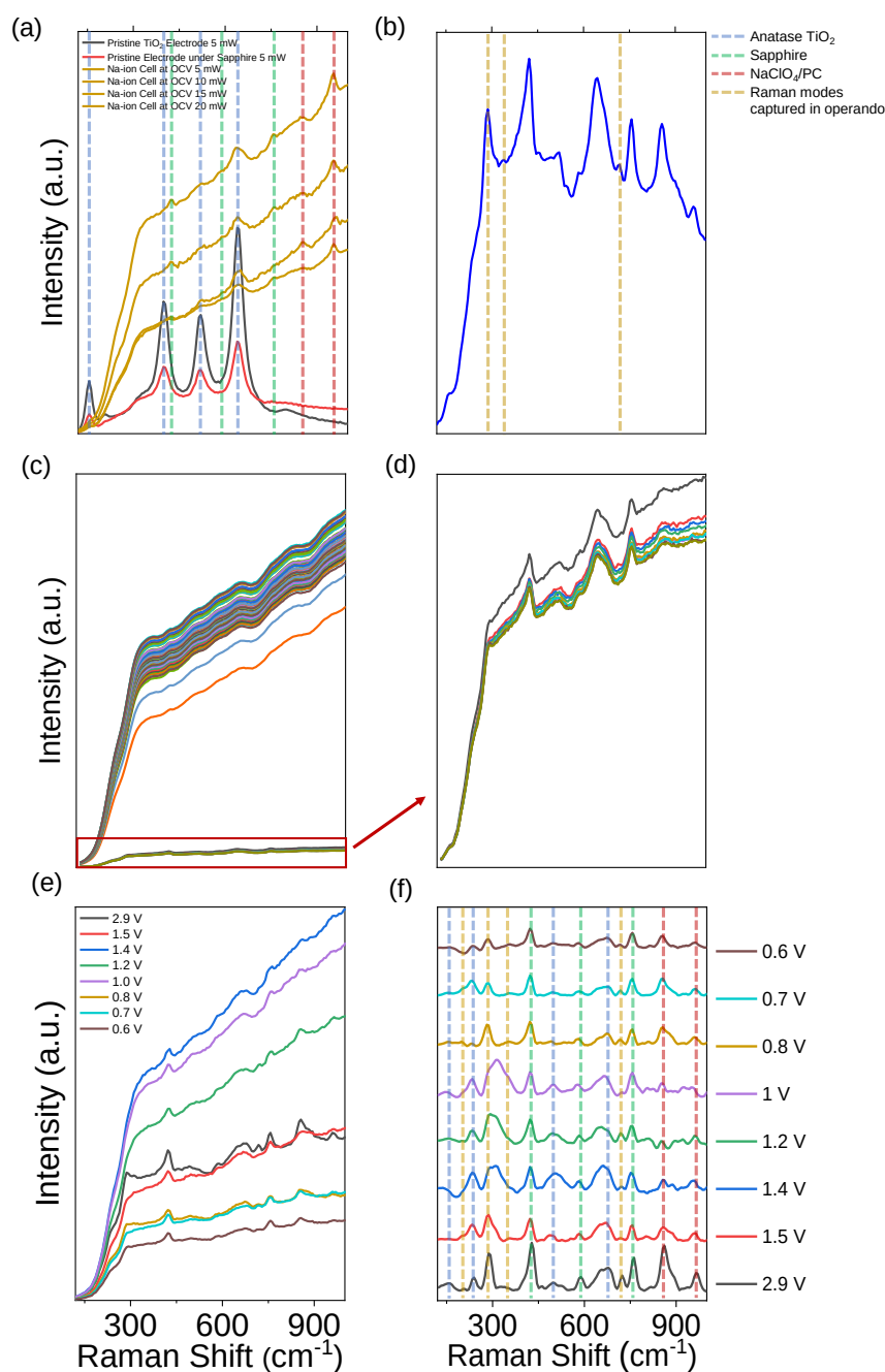
Figure 7.9. (a) Raw Raman spectra of the TiO 2 slurry electrode demonstrating the changes caused by the sapphire window and the cell components compared to the pristine electrode. Characteristic Raman modes are highlighted by dashed lines. (b) Raw Raman spectrum obtained from Na-ion half-cell during discharge, upon instantaneous laser emission with the appearance of new Raman modes highlighted by dashed lines, the colour scheme for the dashed lines throughout this figure is provided by the legend in the upper right hand corner. (c) Raw operando Raman spectra collected during electrochemical discharge with continuous laser emission, demonstrating the formation of the fluorescence mask which hides previously observed Raman modes. The red rectangle highlights spectra for which Raman modes could be distinguished prior to the formation of the mask.
