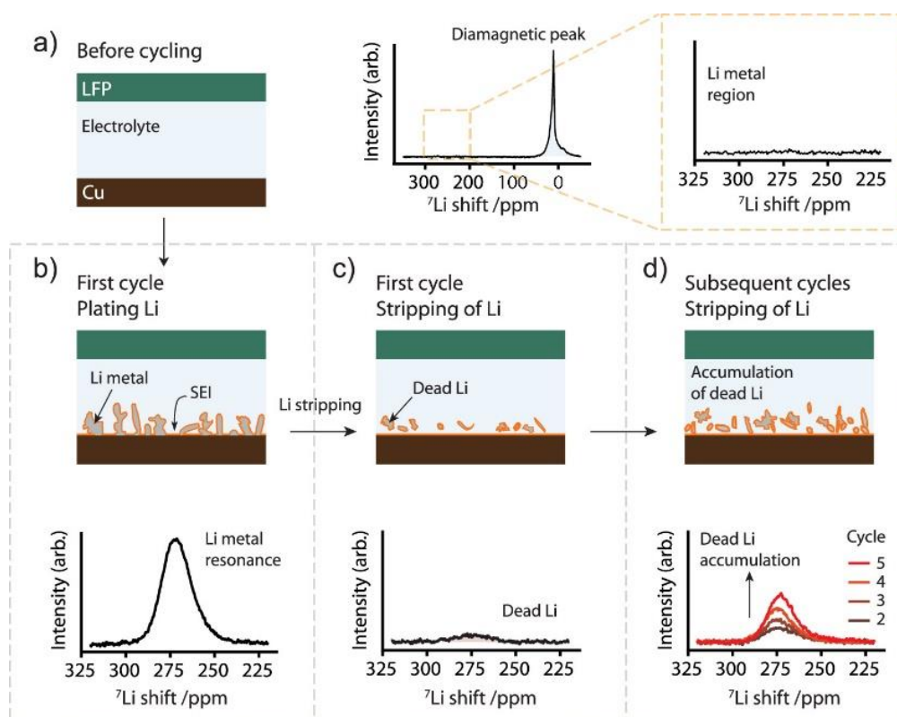
Figure 2.22. Schematic of the ^7\text{Li} in-situ NMR technique used to study dead Li formation and the resulting ^7\text{Li} NMR spectra. (a) The Cu-LiFePO 4 (LFP) cell before cycling and the corresponding ^7\text{Li} NMR spectrum showing the resonance of the diamagnetic Li (the SEI and Li + ions) and the absence of the Li metal peak. (b) Charging the cell results in Li deposition, as shown in the ^7\text{Li} NMR spectrum of the Li metal region. (c) At the end of discharge, the Li metal signal can still be observed, which is attributed to dead Li. (d) Further cycling of the Cu-LFP cell results in an accumulation of dead Li over the next cycles (cycle 2–5), the intensity of the Li metal signal increasing at the end of stripping in each cycle. Adapted from ref. (220). Copyright ACS 2020.
