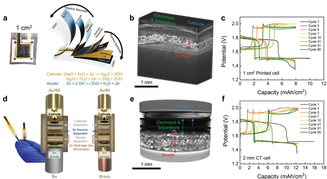
Figure 2.5. Cell design and performance of a Zn-AgO printed cell (a) and in-situ CT cell (d). 3D X-ray CT tomographic reconstructions (b, e), and electrochemical performance (c, f) for Zn-AgO printed cell (top row) and in-situ CT cell (bottom row). Adapted from Ref. (49). Copyright Wiley VCH 2017.
