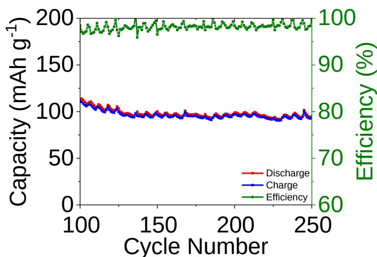
Figure S6.3: Specific capacity of and Coulombic efficiency as a function of cycle number for the same SnO 2 IO Li-ion half-cell from the main text.
