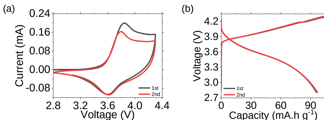
Figure 7.4: (a) CV curves obtained at a scan rate of 0.05 \text{ mV s}^{-1} and (b) galvanostatic cycling curves obtained at a specific current of 25 \text{ mA g}^{-1} for the commercial NMC-622 electrode using the ‘ring system’ electrode stack configuration during which operando Raman measurements were obtained.
