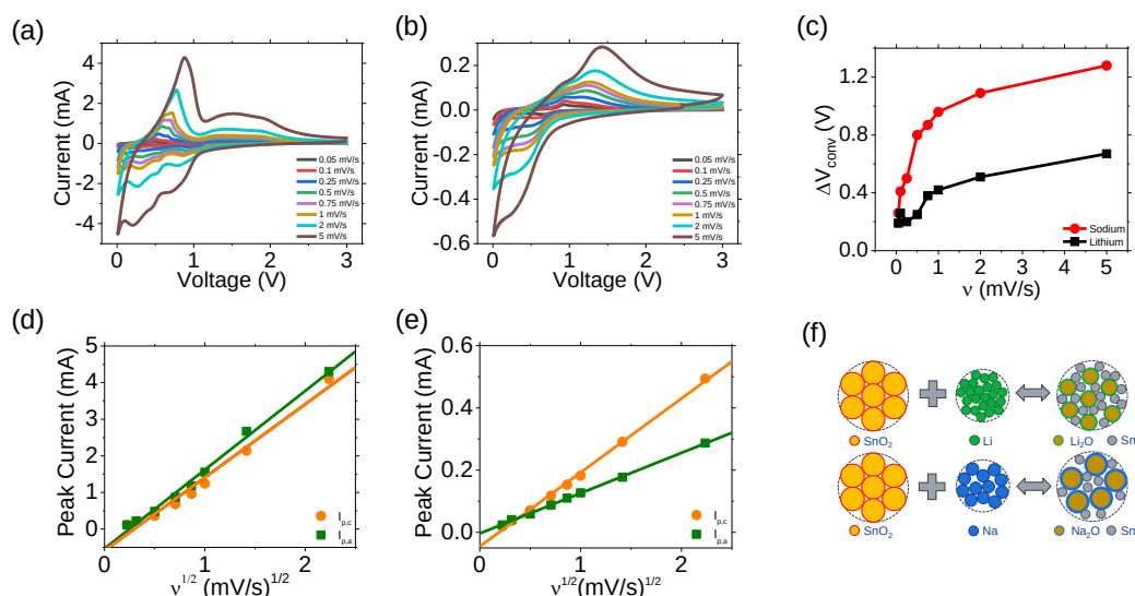
Figure 6.8. Cyclic voltammetry for a range of scan rates from 0.05 \text{ mVs}^{-1} to 5 \text{ mVs}^{-1} for a \text{SnO}_2 IO (a) vs \text{Li/Li}^+ and (b) vs \text{Na/Na}^+ . (c) Potential separation between oxidation and reduction peaks as a function of scan rate for the Li-ion and Na-ion systems. (d) Peak current response as a function of the square root of scan rate for the anodic oxidation ( I_{p,a} ) and cathodic reduction ( I_{p,c} ) reactions in the (d) Li-ion system and (e) Na-ion system. The lines are linear fits to each data set. (f) Visual representation of the conversion reactions between \text{SnO}_2 and metallic Sn in both the Li-ion and Na-ion systems.
