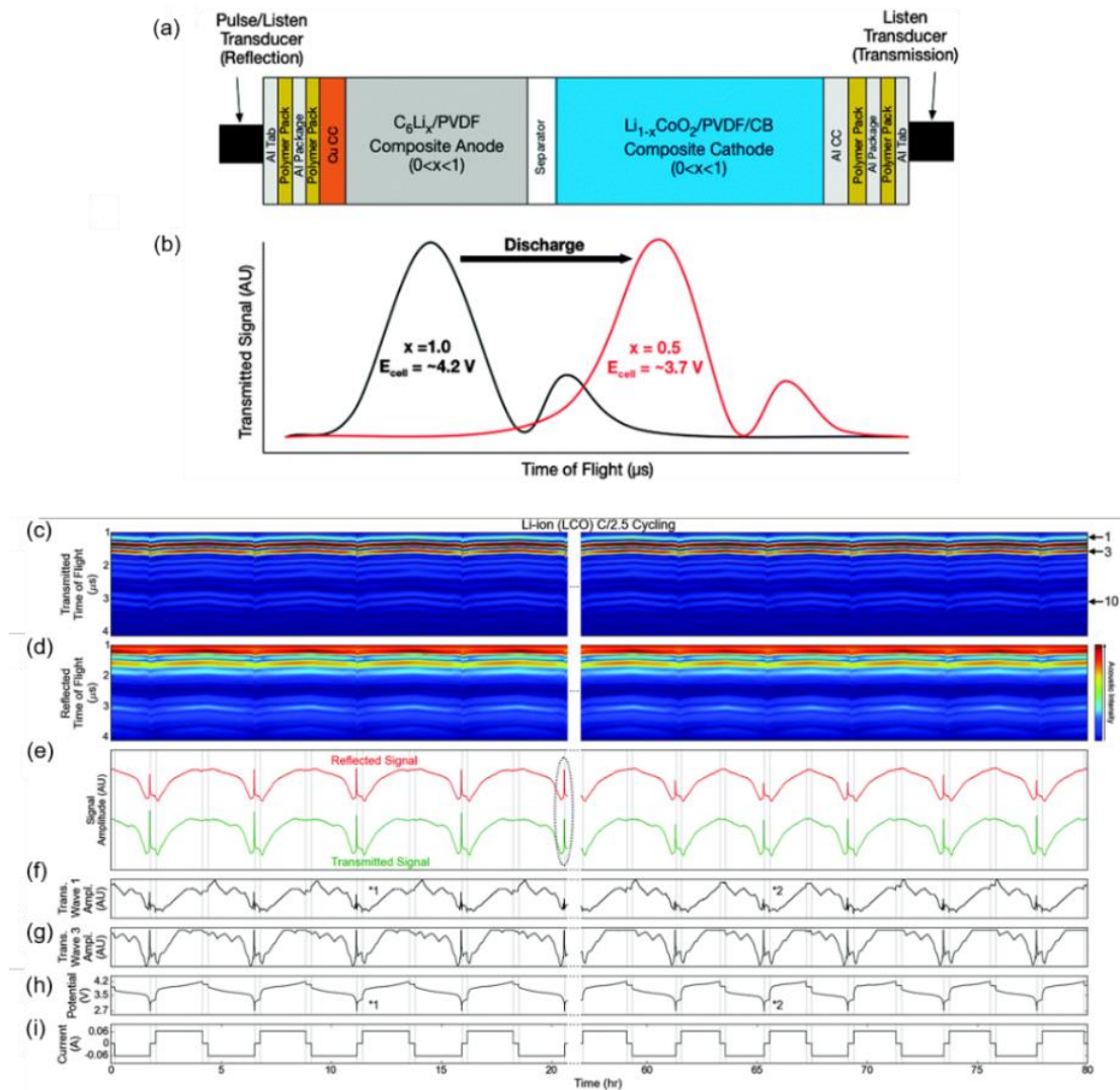
Figure 2.24. Ultrasonic probe of a representative battery. (a) Schematic representation of the battery stack used for acoustic modelling and experimental measurements, shown with packaging, current collector, electrode, separator layers and two acoustic transducers (b) Example illustration of the increase in time of flight (ToF) of the transmitted signal as a
