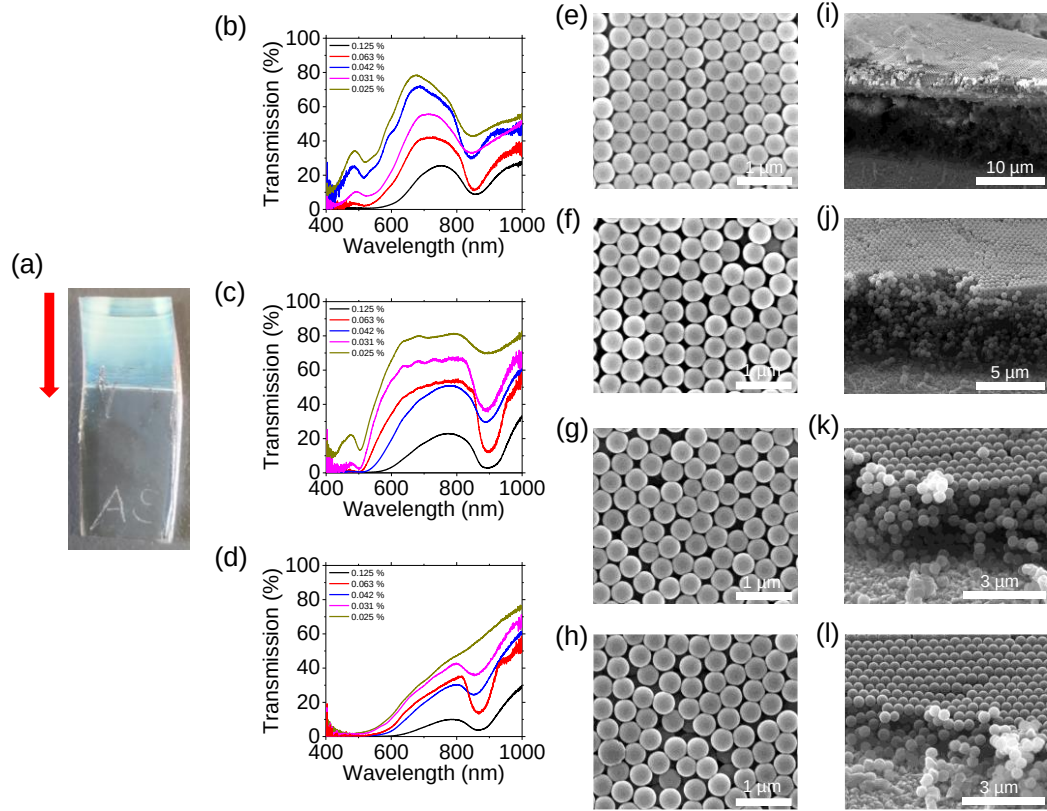
Figure 5.3. Optical and structural characterisation of opals grown by EISA at an evaporation temperature of 28 °C. (a) Photograph of opal sample. Opal thickness decreases in the direction of the red arrow. Optical transmission spectra for five opals, denoted by their volume fractions from 0.025 % to 0.125 %. (b) Spectra obtained at a sample angle of -25°, corresponding to a location near the tail of the arrow. (c) Spectra obtained at normal incidence, near the centre of the sample. (d) Spectra obtained at an angle of 25°, at a location near the head of the arrow. (e)-(g) SEM images obtained normal to the stacking direction at four positions along the direction of the red arrow shown in (a). (i)-(l) Cross-sectional SEM images obtained at four positions along the direction of the red arrow in (a) captured at an angle of 45° to the stacking direction.
