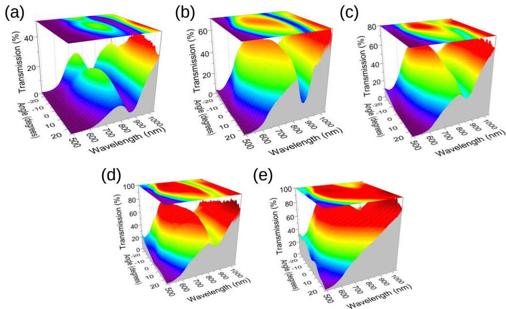
Figure 5.4. Angle-resolved transmission spectra of opals grown by EISA at 28^\circ\text{C} for a range of concentrations of (a) 0.125 %, (b) 0.063 %, (c) 0.042 %, (d) 0.031 %, and (e) 0.025 % at a range of incident angles from -25^\circ to 25^\circ with corresponding 2D color maps of transmission intensity overhead.
