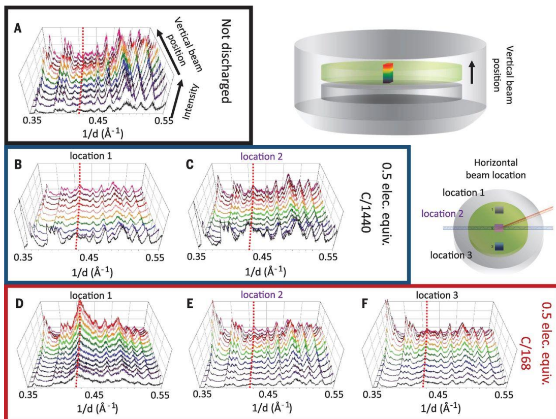
Figure 2.2. Spectra resulting from spatially resolved in-situ EDXRD measurements within three coin cells: (A) A non-discharged cell, (B and C) two different locations within a cell discharged to 0.5 elec. equiv. at a rate of C/1440, and (D to F) three different locations within a cell discharged to 0.5 elec. equiv. at a rate of C/168. Spectra were obtained every 20 mm through the cathode; for clarity, only half of the scans are presented in the figure. Spectra toward the top of the figure (red hues) were obtained within the side of the cathode closer to the stainless-steel coil cell top, and spectra toward the bottom of the figure (black hues) were obtained closer to the Li anode. Adapted from ref. (42). Copyright AAAS 2015.
