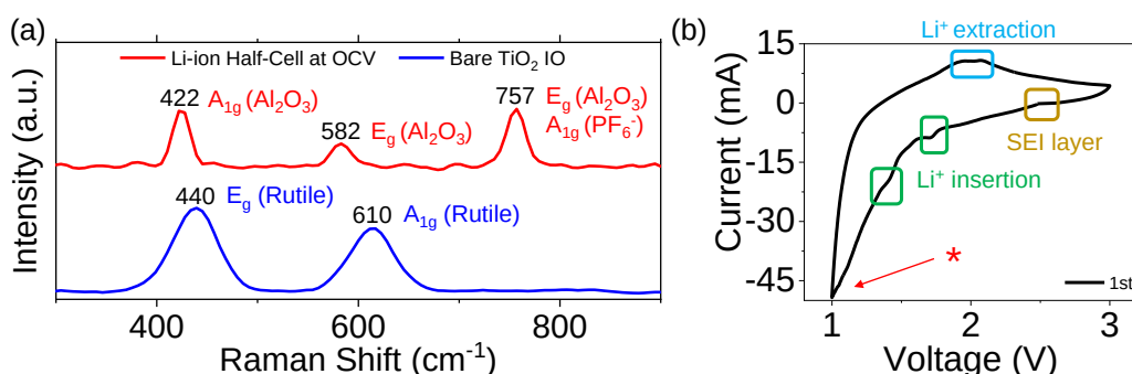
Figure 7.2: (a) Raman spectrum of bare TiO 2 IO (blue) and Raman spectrum with beam focused on TiO 2 IO as a component of assembled Li-ion half-cell at open circuit voltage (OCV) (red). (b) Cyclic voltammogram corresponding to the Li-ion half-cell with TiO 2 IO working electrode.
