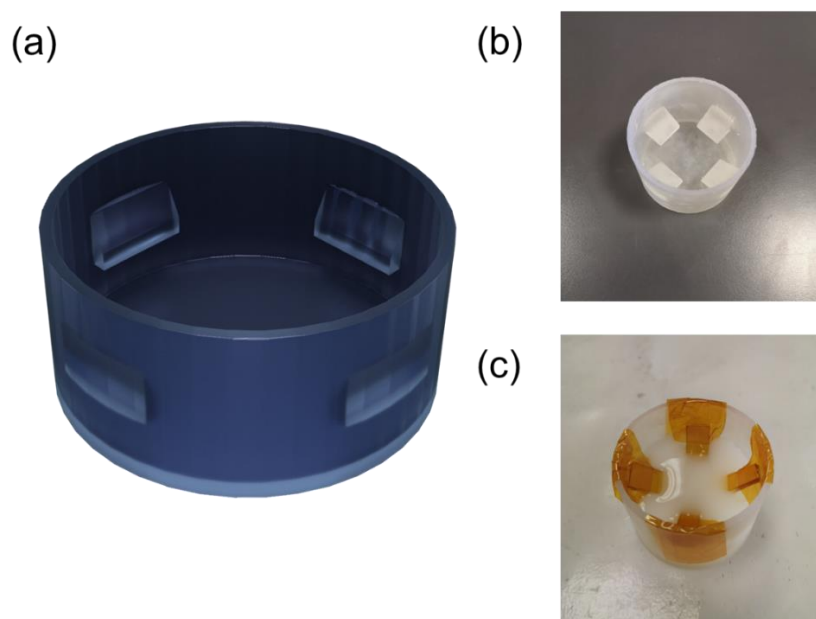
Figure 3.1. (a) Schematic and (b) photograph of the 3D printed beaker used during the EISA process. (c) Photograph of the 3D printed beaker prepared with samples fixed in position and sphere solution added.
