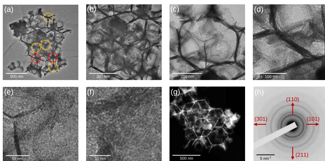
Figure 6.2. (a)-(d) TEM images of \text{SnO}_2 IO at various levels of magnification. Red circles: Octahedral sites. Orange circles: Tetrahedral sites. (e)-(f) HRTEM images showing configuration of nanoparticles within the pore walls and the fringes of the \text{SnO}_2 lattice. (g) STEM image of \text{SnO}_2 IO. (h) Electron diffraction pattern of \text{SnO}_2 IO with indexed lattice planes.
