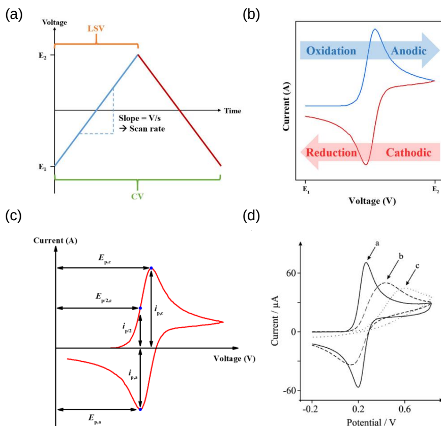
Figure 3.7. Schematics showing basic principles of cyclic voltammetry. (a) Voltage-time profile for linear sweep (LSV) and cyclic voltammetry (CV). (b) Typical CV curve indicating oxidation and reduction directions. (c) CV curve highlighting the most informative points quantities, peak currents, and potentials. (d) Contrast of CV curves for different types of electron transfer: a – reversible, b – quasi-reversible and c – irreversible.(19)
