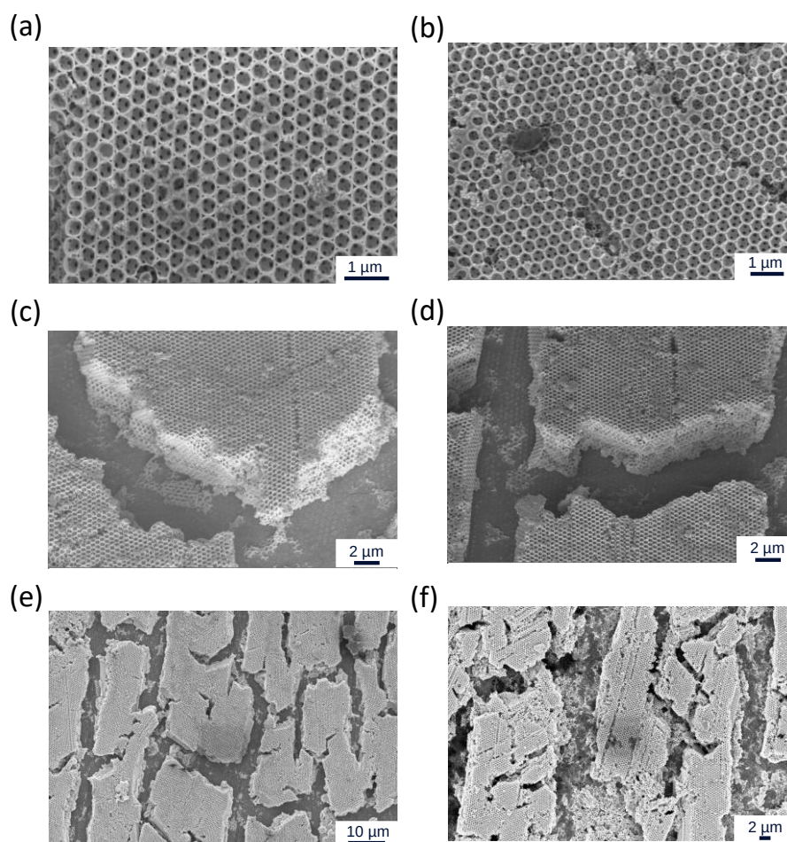
Figure S6.1: Additional SEM images of an \text{SnO}_2 IO to those shown in the main text. (a), (b) Planview, provides overview of porous network with honeycomb pattern. (c), (d) Cross-sectional, obtained at a stage tilt angle of 30^\circ . (e), (f) Planview, provides overview of island of IO material.
