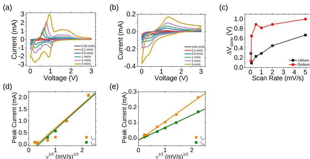
Figure S6.4. CV scan rate testing without prior fixed rate CV scans, which was performed for the results shown in the main text. Cyclic voltammetry for a range of scan rates from 0.05 \text{ mVs}^{-1} to 5 \text{ mVs}^{-1} for a \text{SnO}_2 IO (a) vs \text{Li/Li}^+ and (b) vs \text{Na/Na}^+ . (c) Potential separation between oxidation and reduction peaks as a function of scan rate for the Li-ion and Na-ion systems. (d) Peak current response as a function of the square root of scan rate for the anodic oxidation ( I_{p,a} ) and cathodic reduction ( I_{p,c} ) reactions in the (d) Li-ion system and (e) Na-ion system.
