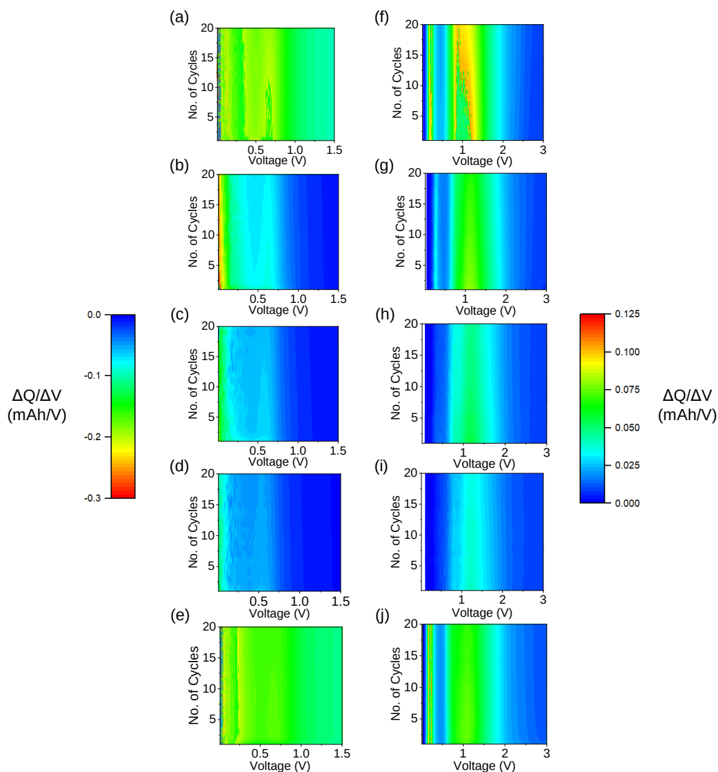
Figure 6.10. Differential capacity colour maps obtained from rate capability testing of the SnO 2 IO in the Na-ion system at current densities presented in the following order from top to bottom: 50 mA g -1 , 150 mA g -1 , 300 mA g -1 , 450 mA g -1 , 50 mA g -1 , generated from discharges (a)-(e) and charges (f)-(j). Colour bars associated with discharges and charges positioned left and right, respectively.
