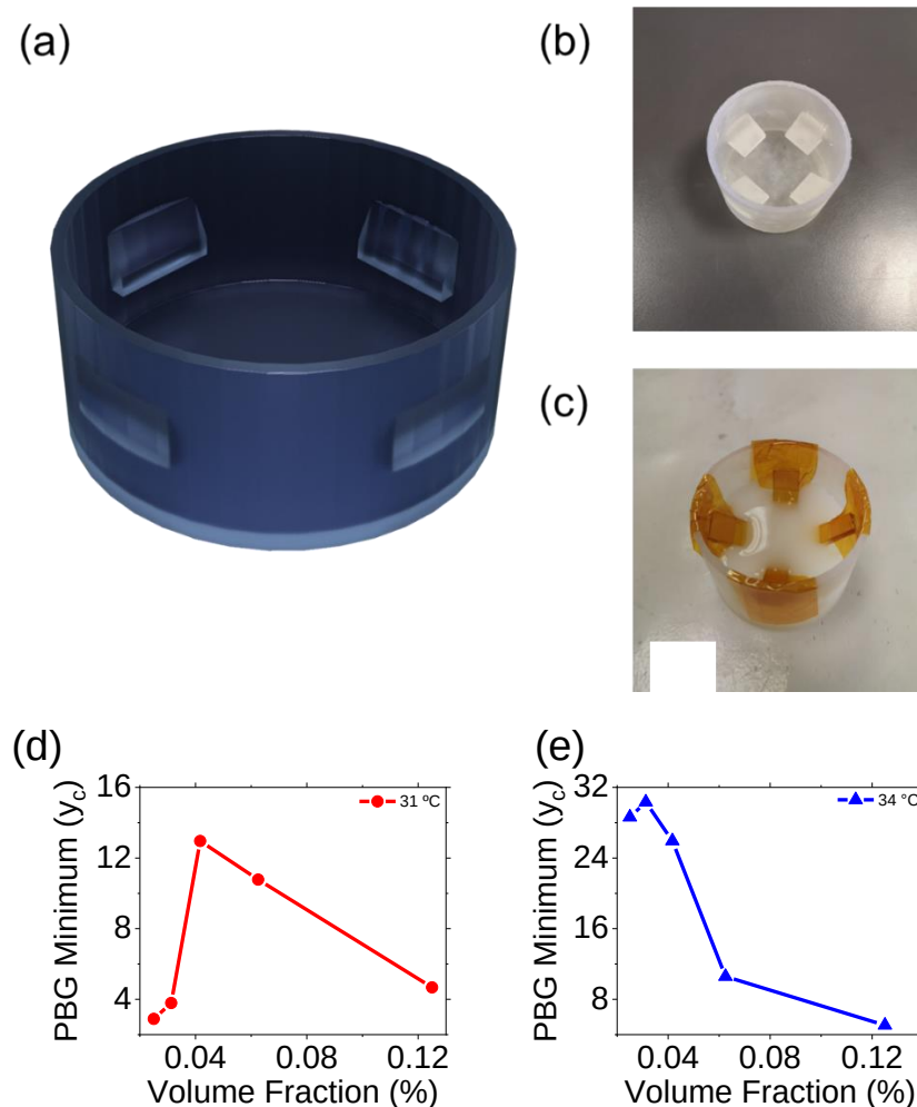
Figure S4.1. SLA 3D printed beaker designed with substrate rests at an angle of 30 ° to the vertical used for opal growth by EISA. (a) 3D rendered image of beaker. (b) Photograph of beaker. (c) Photograph depicting FTO substrates immersed in PS sphere solution inside beaker. (d) Intensity of central PBG frequency as a function of sphere solution volume fraction for opals grown using EISA at evaporation temperatures of 31 °C and 34 °C.
