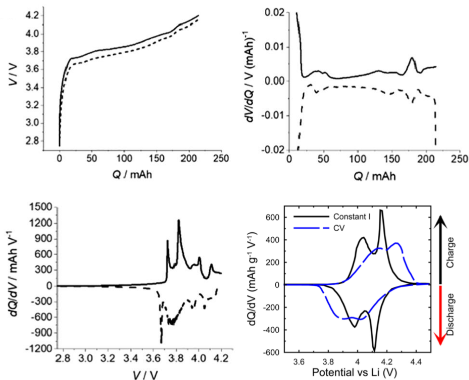
Figure 3.9. (a) Typical charge-discharge curve from galvanostatic cycling. (b) Differential voltage calculated as the first derivative of (a). (c) Differential capacity, calculated as the reciprocal of (b). (d) Comparison of typical differential capacity and cyclic voltammetry curves.(23)
