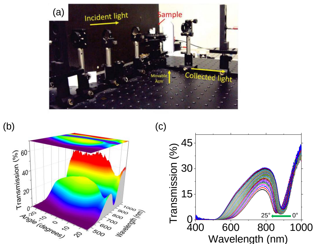
Figure 3.5. (a) Photograph of spectroscopy setup. (b) 3D angle-resolved transmission spectrum of an opal PhC. (c) Typical angle-resolved transmission spectra of opal PhC. Green arrow indicates blue shift of PBG as incident angle is increased from 0° to 25°.
