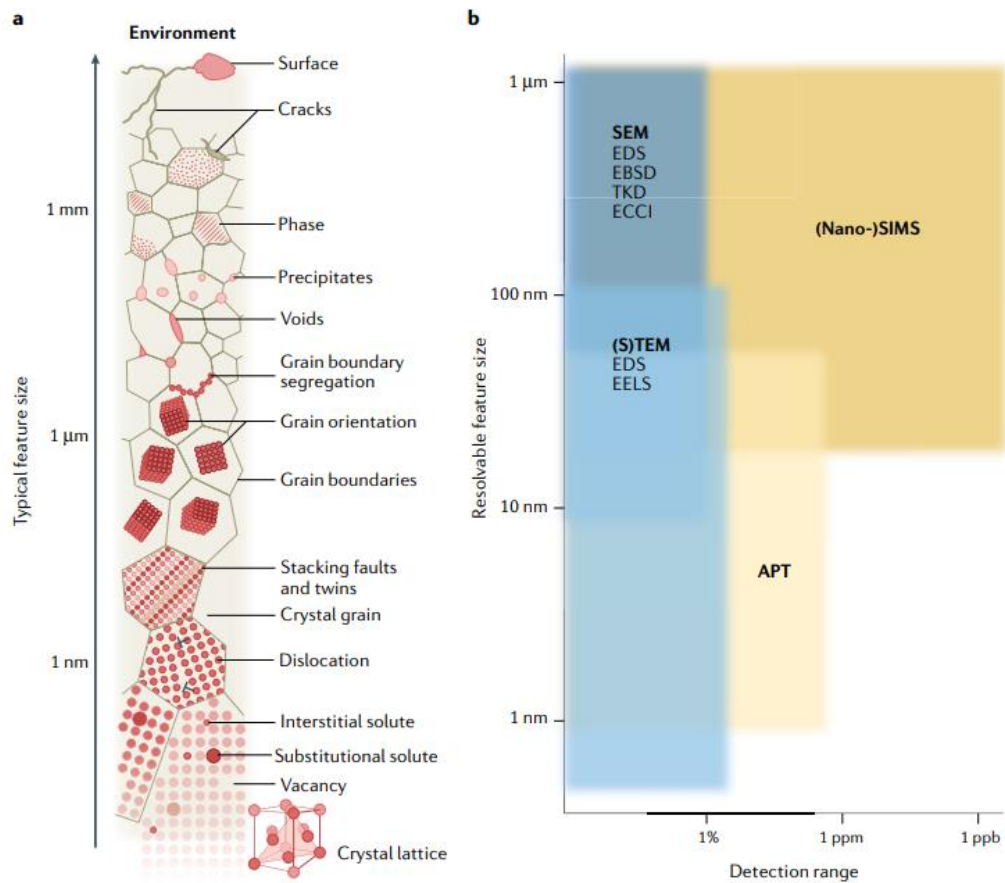
Figure 2.8. Features of microstructured materials with their relative sizes and some analytical techniques used to resolve them. (a) A range of common structural features of interest, from the atomic arrangement of a crystal lattice, through a range of crystalline defects, phases, and grains, to imperfections at the surface. (b) Sensitivity and analysable feature size for some structural analysis techniques. Atom probe tomography (APT); Electron backscattered diffraction (EBSD); Electron-channelling contrast imaging (ECCI); Energy-dispersive X-ray spectroscopy (EDS); Electron energy loss spectroscopy (EELS); Scanning electron microscopy (SEM); Secondary ion mass spectrometry (SIMS); (Scanning) transmission electron microscopy ((S)TEM); Transmission Kikuchi diffraction (TKD). Adapted with permission from ref. (71). Copyright Springer Nature Limited 2021.
