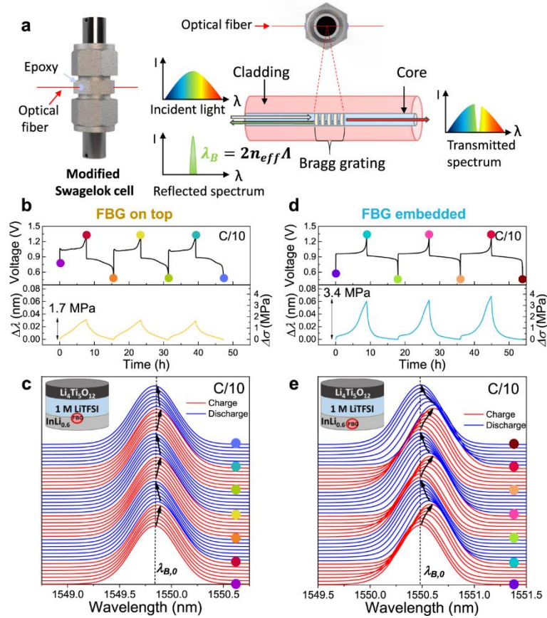
Figure 2.19. (a) Integration of an FBG into an in-house-modified Swagelok cell with a graphical summary of the working principle of an FBG optical sensor. (b) Time-resolved voltage (top) and \Delta\lambda_B and \Delta\sigma (bottom) evolution from the FBG sensor of an \text{InLi}_{0.6} – LTO cell in a 1 M LiTFSI in DOL:DME electrolyte. The FBG was put at the anode/electrolyte interface. (c) Reflectance spectra from the FBG sensor located at the anode/electrolyte interface for the cycles shown in (b). (d, e) Analogous plots to (b, c), for a cell with the FBG sensor embedded within the \text{InLi}_x electrode. Adapted from Ref. (192). Copyright Nature Publishing Group 2022.
