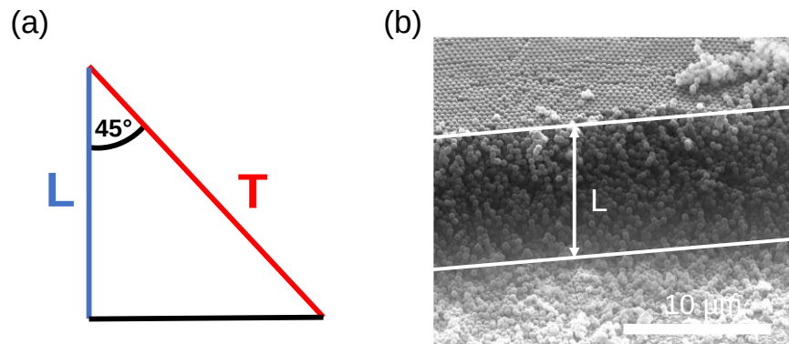
Figure S4.6. (a) Schematic of the determination of opal thickness. (b) Sample cross-sectional SEM image illustrating the method used to acquire thickness measurements.
