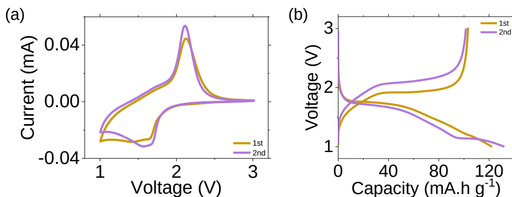
Figure 7.7: (a) CV curves obtained at a scan rate of 0.05 \text{ mV s}^{-1} and (b) galvanostatic cycling curves obtained at a specific current of 10 \text{ mA g}^{-1} for the \text{TiO}_2 slurry electrode using the ‘ring system’ electrode stack configuration from which operando Raman measurements were obtained.
