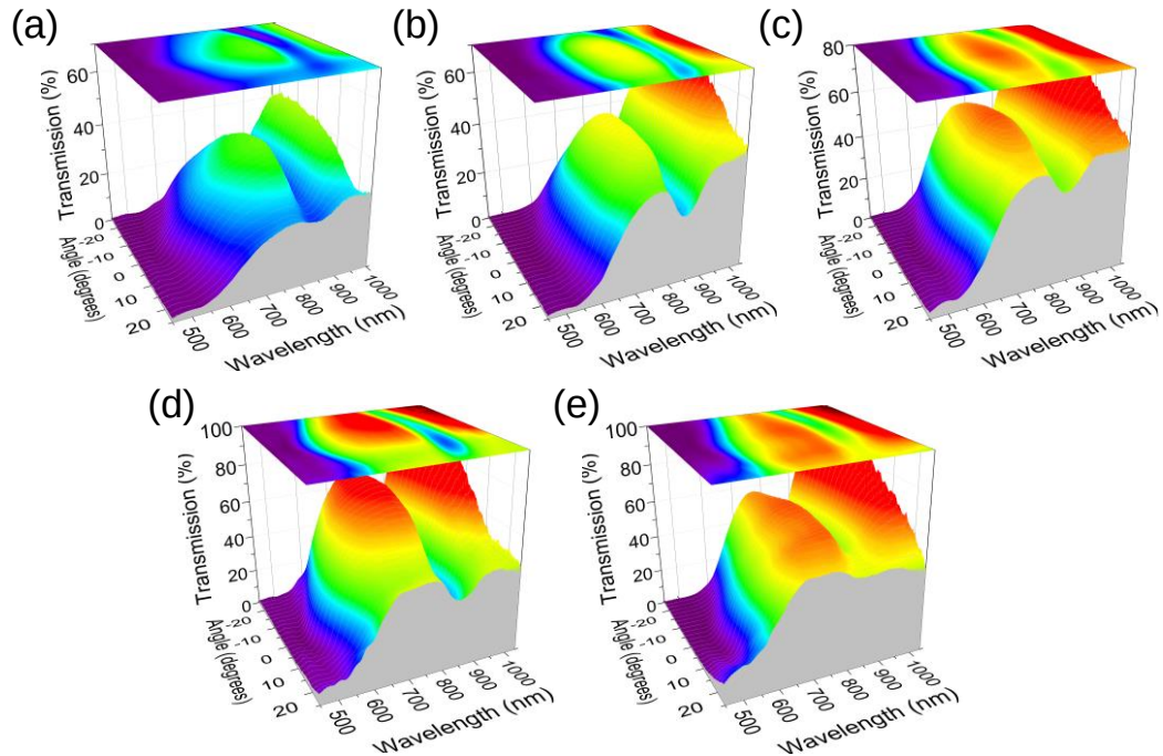
Figure 5.2. Angle-resolved transmission spectra showing the variation of optical transmission as a function of angle of incidence and wavelength, for opals grown by EISA at 34 °C. The spectra correspond to transmission intensity for a range of volume fractions of (a) 0.125 %, (b) 0.063 %, (c) 0.042 %, (d) 0.031 %, and (e) 0.025 % at a range of incident angles from -25° to 25°. Corresponding 2D color maps overhead show the degree of symmetry in the angle-resolved response of EISA grown opals. The colors are linked to transmission intensity.
