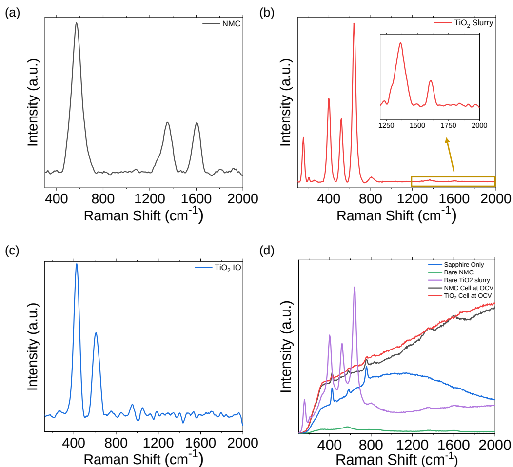
Figure S7.1. Ex-situ Raman spectra after background subtraction for (a) commercial NMC electrode at a laser specific power of 20 mW, (b) TiO 2 slurry (inset highlights region where carbon peaks occur) with at 2 mW, and (c) TiO 2 IO at 20 mW. (d) Raw Raman spectra comparing two of the bare electrodes, sapphire window, and the same electrodes as components of Li-ion half-cells to highlight the appearance of the fluorescence mask.
