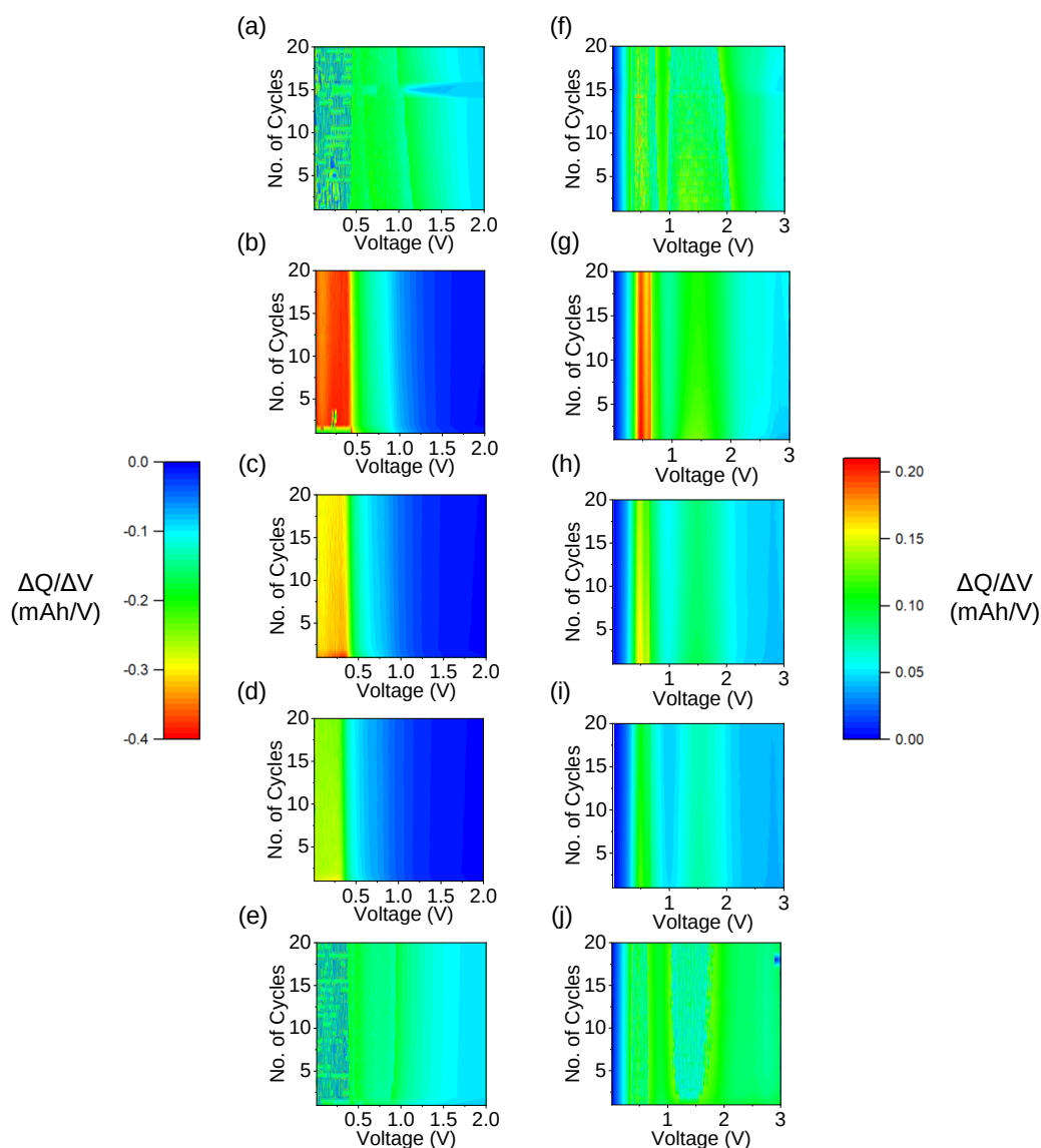
Figure 6.9. Differential capacity colour maps obtained from rate capability testing of the \text{SnO}_2 IO in the Li-ion system at current densities presented in the following order from top to bottom: 50 \text{ mA g}^{-1} , 150 \text{ mA g}^{-1} , 300 \text{ mA g}^{-1} , 450 \text{ mA g}^{-1} , 50 \text{ mA g}^{-1} , generated from discharges (a)-(e) and charges (f)-(j). Colour bars associated with discharges and charges positioned left and right, respectively.
