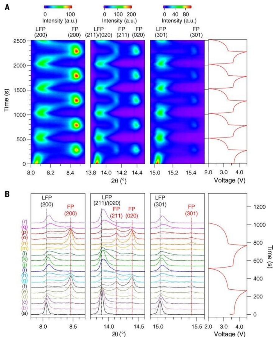
Figure 2.3. In-situ XRD patterns during galvanostatic charge and discharge at a rate of 10 C. (A) Diffraction patterns for (200), (211), (020), and (301) reflections during the first five charge-discharge cycles. The horizontal axis represents the selected 2\theta regions, and time is on the vertical axis. Diffraction intensity is colour coded with the scale bar shown on top. The corresponding voltage curve is plotted to the right. LFP, \text{LiFePO}_4 ; FP, \text{FePO}_4 . (B) Selected individual diffraction patterns during the first two cycles and voltage profile. The baseline is represented by horizontal dashed grey lines. Black vertical lines mark the positions of \text{LiFePO}_4 peaks at the start of reaction; red vertical lines mark the position of \text{FePO}_4 peaks formed during the first cycle. Adapted from ref. (44). Copyright AAAS 2014.
