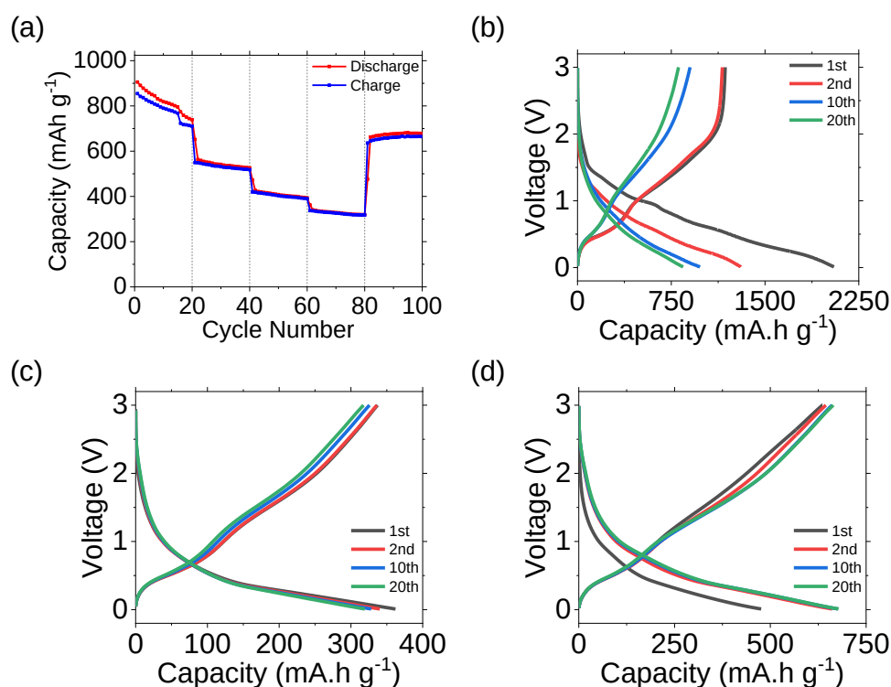
Figure 6.6. (a) Rate capability testing of \text{SnO}_2 IO in Li-ion system. Galvanostatic cycling curves (b) for initial specific settling current of 50 \text{ mA g}^{-1} prior to the rate test, (c) maximum specific current applied during rate test of 450 \text{ mA g}^{-1} , and (d) charging and discharging at a final current of 50 \text{ mA g}^{-1} .
