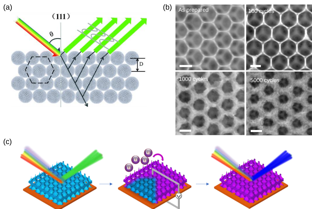
Figure 2.14. (a) Schematic of the PBG in a PhC, selectively reflecting a narrow band of photon energy. Light within the PBG is reflected from the crystal, determined by the lattice constant D . Reproduced from ref. (175). Copyright RSC 2019. (b) \text{TiO}_2 IO materials used as an anode in a Li-ion battery showing interconnected volumetric swelling as lithiated titanate over 100, 1000 and 5000 cycles. Scale bar = 200 nm. Adapted from Ref. (176). Copyright Wiley 2017. (c) Schematic representation of operando angle-resolved reflectance measurement of a PBG during reversible lithiation.
