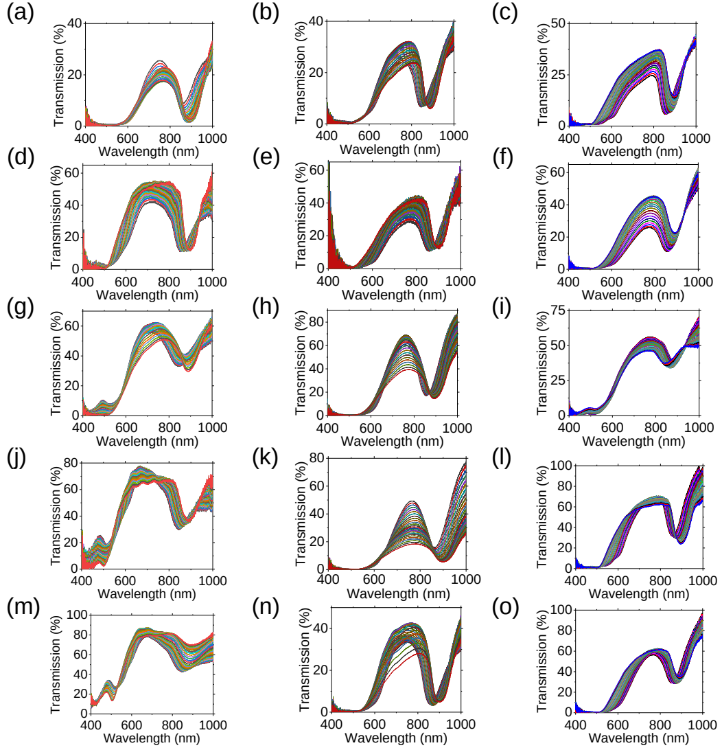
Figure S4.4. Transmission spectra of opals obtained in the incident angle range of 0-25 ° relative to the normal to the (111) plane of an FCC lattice. Evaporation temperatures are 28 °C, 31 °C, 34 °C, increasing from columns 1-3. Sphere solution volume fractions: (a)-(c) 0.125%, (d)-(f) 0.063% (g)-(i) 0.042%, (j)-(l) 0.031%, (m)-(o) 0.025%.
