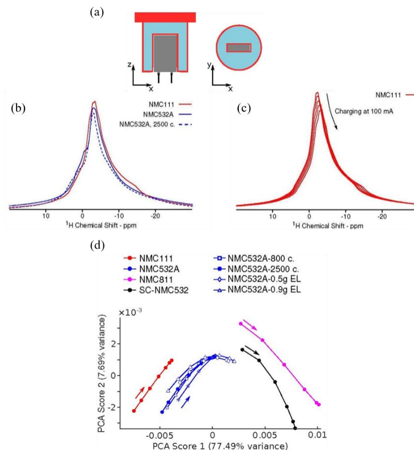
Figure 2.23. (a) Schematic of 3D-printed holder (red) used for ioMRI and NMR. The holder contains the cell (grey), which is surrounded by water compartment (light blue). The system is placed inside an NMR probe with the z-axis aligned with the static magnetic field. The vertical and horizontal cross sections are shown left and right, respectively. (b) ^1\text{H} NMR spectra taken at 2.5 V for cells containing, as cathode: NMC111 (red), NMC532A (solid blue) and NMC532A already undergone 2500 cycles prior to the MRI (dashed blue). (c) ^1\text{H} NMR spectra taken at intervals during charging of the cell containing NMC111 as cathode. The black arrow shows the direction of shift of the spectra as the cell undergoes charging. (d) Principal component analysis (PCA) performed on the ^1\text{H} NMR spectra of all the cells. Each arrow indicates the direction of the trend(s) of the corresponding colour as the cell is charged. Adapted with permission from ref. (221). Copyright Wiley 2020.
