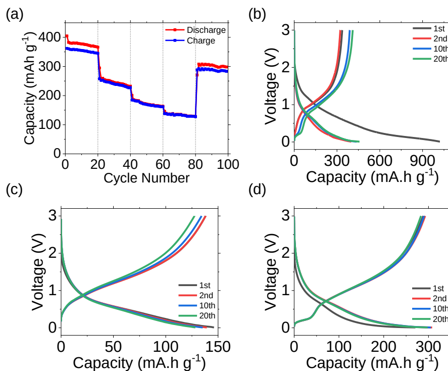
Figure 6.7. (a) Rate capability testing of SnO 2 IO in Na-ion system. Galvanostatic cycling curves (b) for initial specific settling current of 25 mA g -1 prior to rate test, (c) maximum specific current applied during rate test of 450 mA g -1 , and (d) final current of 50 mA g -1 .
