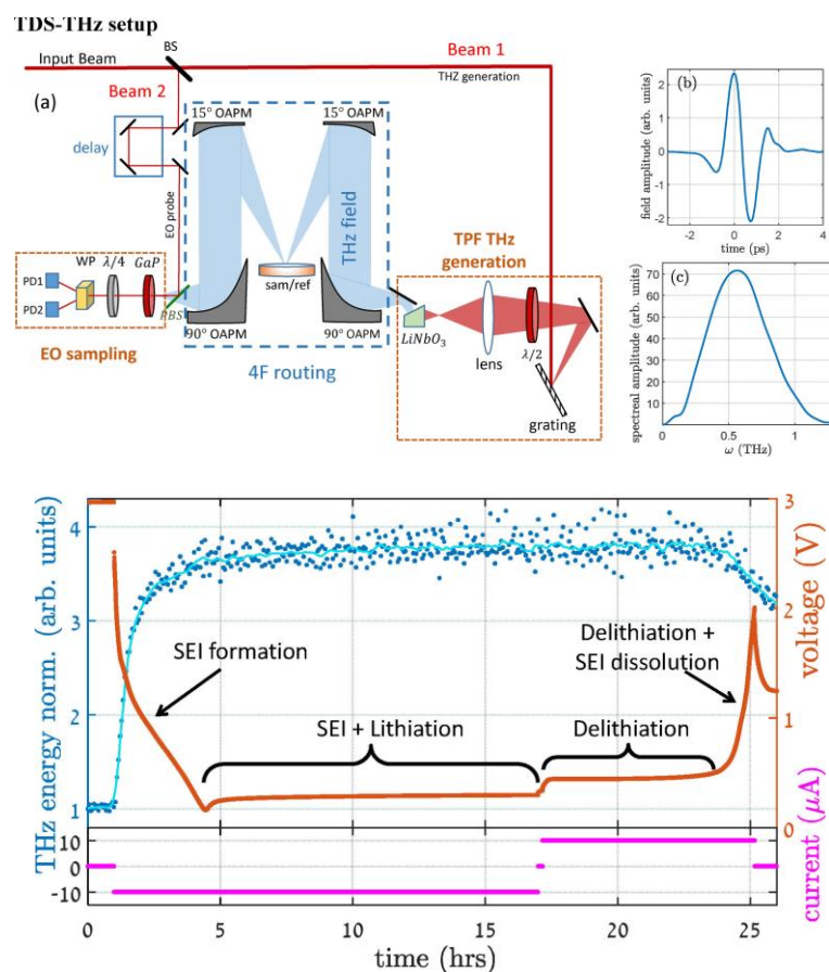
Figure 2.16. (Top) (a) Schematic of the time-domain THz spectrometer setup in reflection mode with the battery cell placed at prime focus. (b) An example of a THz signal in the time domain together with its associated amplitude spectrum. Electrooptic sampling module includes a pellicle beam splitter (PBS), a Gallium Phosphate crystal (GaP), quarter-wave plate, a Wollaston prism (WP) and two photodiodes. (Bottom) The THz signal (blue dots) in the time domain during a single full cycle. The cycle comprised the discharge (1–17 hours) followed by charging (18–26 hours). The cell voltage is shown in orange and the current in magenta. Reproduced from ref. (189). Copyright Wiley VCH 2022.
