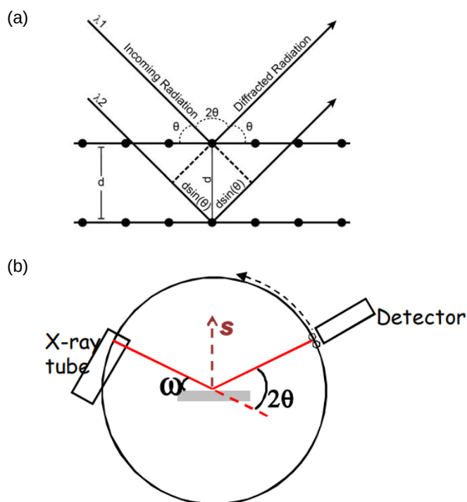
Figure 3.6. (a) Schematic depicting the concept of XRD which demonstrates the origin of Bragg's Law. (b) Schematic of typical XRD instrument setup that illustrates the geometry of the goniometer, highlighting the sample tilt direction over angle \omega and detector rotation direction over 2\theta . s is the diffraction vector.
