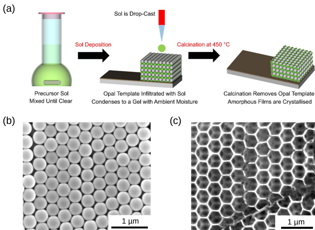
Figure 3.2. (a) Schematic of sol-gel process depicting the infiltration of opal template with metal alkoxide precursor and calcination to form IO. (b) SEM image of opal template prior to infiltration. (c) SEM image of IO after infiltration and calcination.
