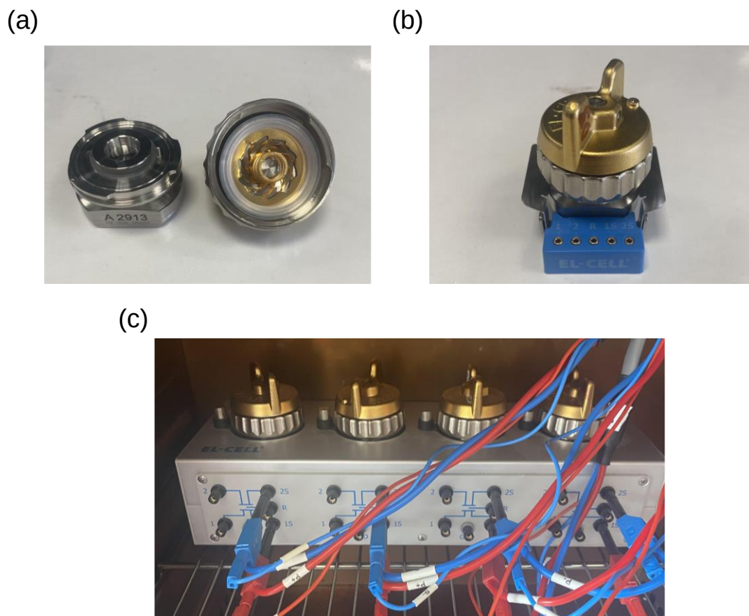
Figure 3.3. Photographs of EL Cell PAT cells used for battery performance testing (a) Opened PAT cell (b) PAT Cell clipped into PAT-Clamp for connection to potentiostat. (c) PAT cells clipped into docking station inside temperature-controlled oven connected to potentiostat.
