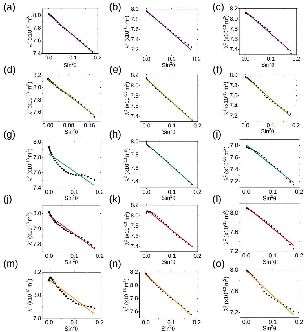
Figure S4.3. Bragg-Snell plots based on the central frequency of the primary transmission dip observed in the optical spectra of opals obtained in the incident angle range of 0-25 °. Evaporation temperatures are 28 °C, 31 °C, 34 °C, increasing from columns 1-3. Sphere solution volume fractions: (a)-(c) 0.125%, (d)-(f) 0.063% (g)-(i) 0.042%, (j)-(l) 0.031%, (m)-(o) 0.025%.
