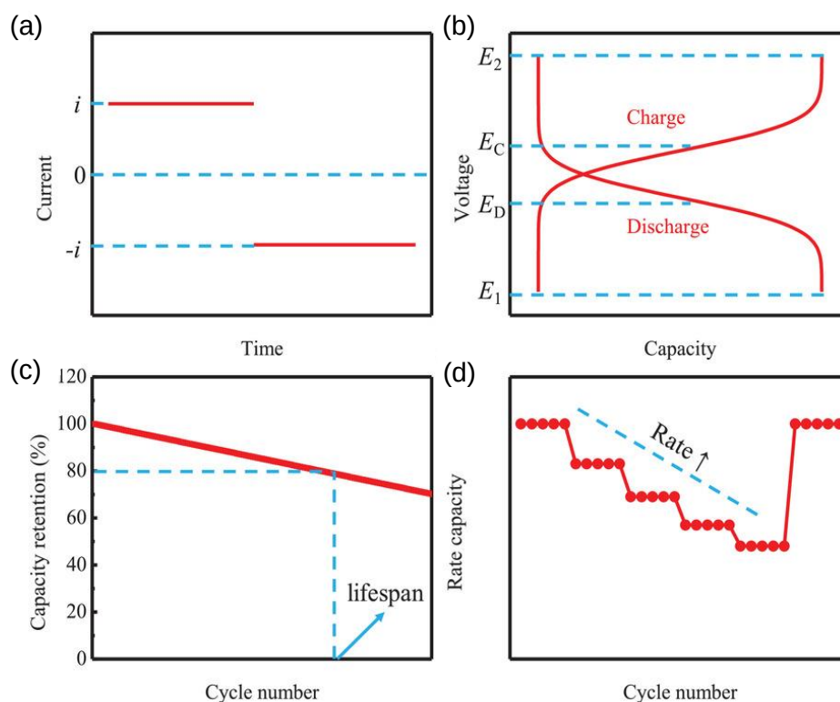
Figure 3.8. Schematics depicting results generated from typical galvanostatic cycling of batteries. (a) Applied current profile. (b) Charge-discharge curve showing voltage response vs capacity. (c) Cycling stability, capacity retention over battery lifetime. (d) Typical rate test showing change in capacity at each rate as a function of cycle number.(22)
