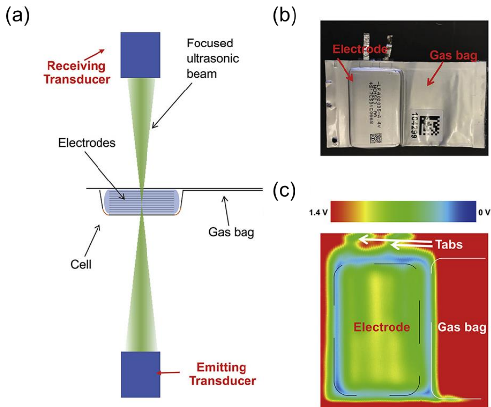
Figure 2.25. (a) Schematic of ultrasonic transmission setup showing path of focused beam. (b) Photograph of pouch cell and its main components. (c) Ultrasonic transmission image of the pouch cell overlapped on the optical photo. Adapted from ref. (45). Copyright Joule 2020.
