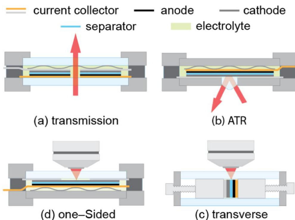
Figure 2.10. Operando spectrochemical cell designs for optical spectroscopic methods grouped into the 4 primary configurations which appear in the literature. Reprinted from ref. (91). Copyright 2022 IOP Publishing.
