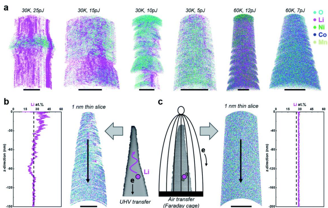
Figure 2.9. (a) 3D atom maps of NMC811 samples obtained under a range of pulse energies and cryogenic specimen temperatures after UHV transferring. Scale bars are all 10 nm. APT results from (b) UHV and (c) air transferred samples. The nominal Li composition of NMC811 in each of the 1D composition profiles are indicated by the black dashed lines. Both APT measurements were performed at a base temperature of 60 K and a pulsed laser energy of 5 pJ. Scale bars in the atom maps are (b) 20 and (c) 50 nm. Reproduced with permission from ref. (32). Copyright RSC 2022.
