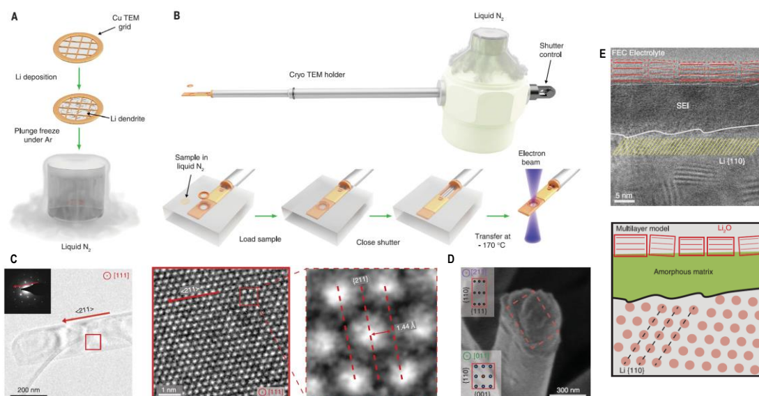
Figure 2.7. (a) Setup where Li metal dendrites are electrochemically deposited directly onto a Cu TEM grid and then plunged into liquid nitrogen after battery disassembly. (b) The specimen is then placed onto the cryo-TEM holder in liquid nitrogen, kept isolated at -170^{\circ}\text{C} . (c) TEM of Li metal dendrites growing along the \langle 211 \rangle directions with corresponding SAED pattern (electron dose rate < 1 \text{ e } \text{\AA}^{-2} \text{ s}^{-1} for \sim 30 \text{ s} ). (e) Atomic-resolution image and schematic of the multilayered SEI structure on Li dendrites in FEC-containing electrolyte. Electron dose rate \sim 1000 \text{ e } \text{\AA}^{-2} \text{ s}^{-1} for \sim 30 \text{ s} . Adapted with permission from Science 358, 506 (2017). Copyright 2017 American Association for the Advancement of Science.
