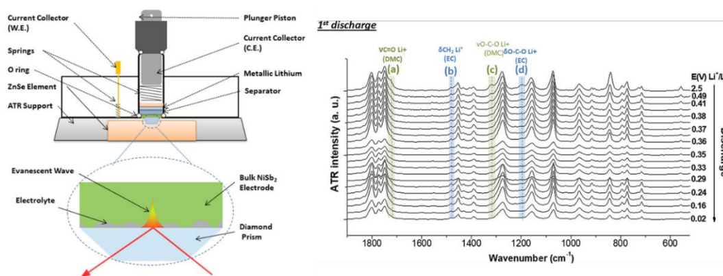
Figure 2.13. (a) Schematic of the electrochemical cell used for the operando ATR-FTIR experiment. (b) Operando IR spectra obtained during the 1 st discharge of NiSb 2 electrode at a rate of 1 C with 1 M LiPF 6 in EC: DMC (1:1) + 2 % vol VC electrolyte. Adapted from ref. (116). Copyright ACS 2017.
