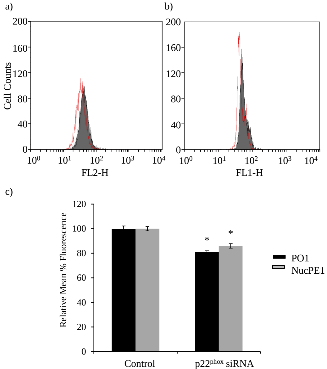
Figure 2. 14. Quantification of cellular and nuclear H_2O_2 following the p22 phox siRNA knockdown. MV4-11 cells were stained with either PO1 (a) or NucPE1 (b) for 1 h, 24 h after the siRNA transfection. a) FACS analysis of relative mean PO1 fluorescence of control (scrambled siRNA; grey) and p22 phox siRNA treated (Control; red) MV4-11 cells. b) FACS analysis of relative mean NucPE1 fluorescence of control (scrambled siRNA; grey) and p22 phox siRNA treated (Control; red) MV4-11 cells. c) Bar chart represents flow cytometry analysis of mean relative %PO1 and % NucPE1 fluorescence of control treated and p22 phox siRNA treated MV4-11 cells. Results are shown as relative geometric mean \pm SD. Results are representative of at least 3 biological replicates. The asterisk indicates statistically significant difference ( p < 0.05 ) as analysed by Student t-test. The error bars represent \pm SD.
