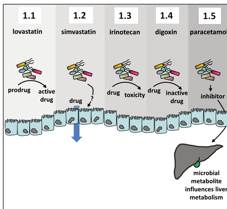
Figure 1. A summary of selected mechanisms by which the microbiota influences drug pharmacokinetics. Individual panels correspond to the article text. 1.1 Agents including lovastatin or sulfasalazine are directly activated by the gut microbiota. 1.2 The availability and uptake of drugs including simvastatin and amiodarone is influenced by the microbiota or by co-administration of probiotics through unknown mechanisms. 1.3 Toxicity of irinotecan is elevated by microbial \beta -glucuronidase activity and can be selectively inhibited by antibiotics or specific microbial \beta -glucuronidase inhibitors. 1.4 Digoxin is inactivated in the gut by specific enzymatic activity associated with specific strains of Eggerthella lenta ( cgr+ ). 1.5 Paracetamol detoxification in the liver is competitively inhibited by the gut microbial metabolite p -Cresol.
