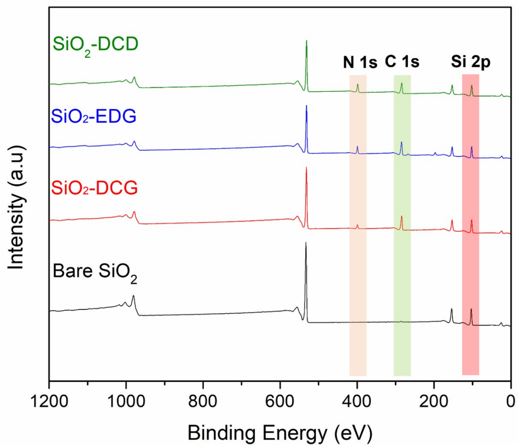
Figure S2: XPS Survey scan for bare \text{SiO}_2 , \text{SiO}_2\text{-DCG} , \text{SiO}_2\text{-EDG} and \text{SiO}_2\text{-DCD} catalysts.
