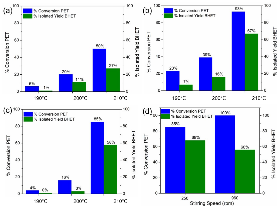
Figure S5: Microwave assisted glycolysis of PET under different reaction temperatures for (a) \text{SiO}_2 -DCG, (b) \text{SiO}_2 -EDG and (c) \text{SiO}_2 -DCD and catalysts (d) Stir speed optimization.
