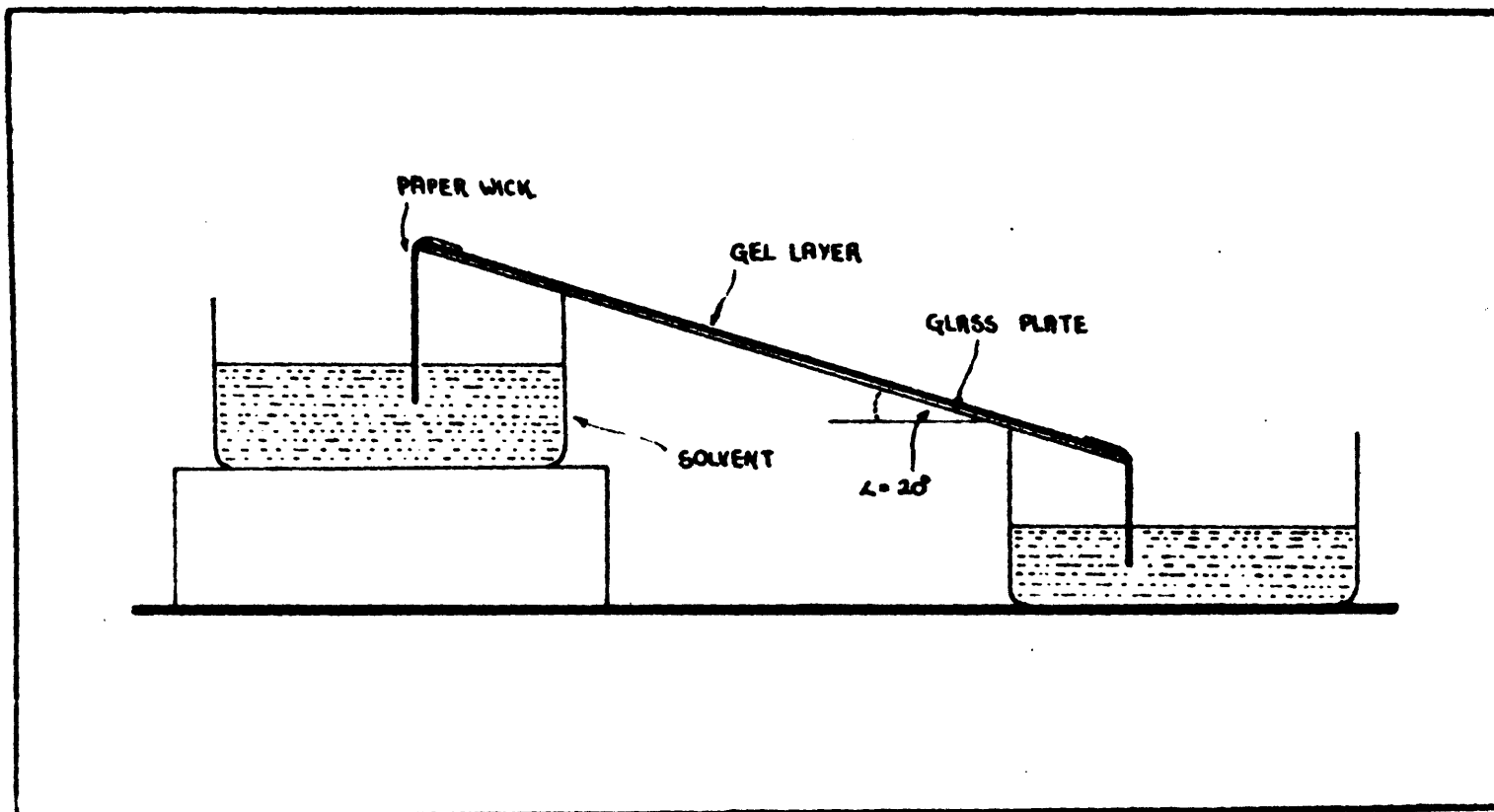
FIG. 3. Schematic representation of thin-layer gel filtration apparatus.
