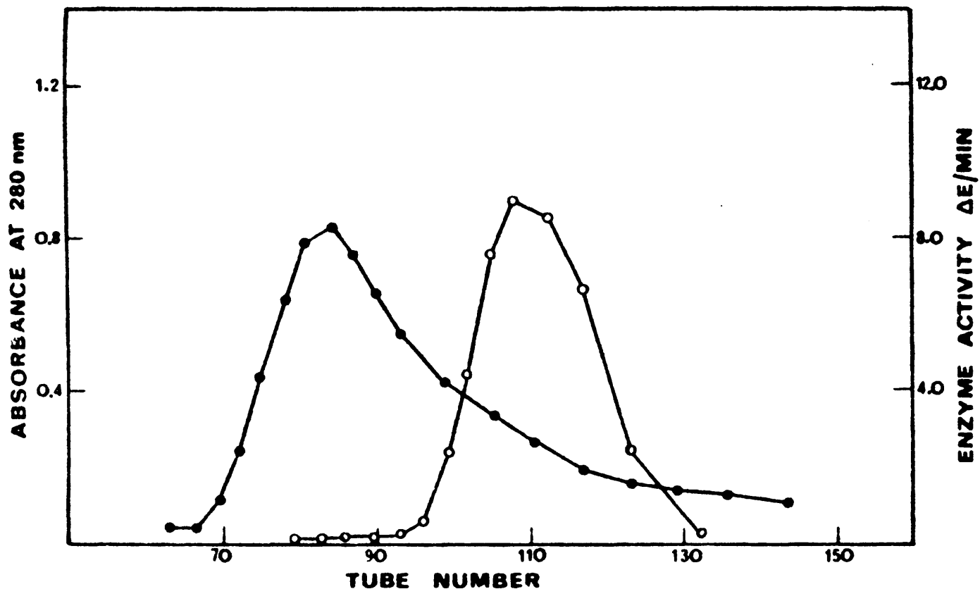
FIG. 14. Gel filtration of adenosine on Sephadex G-75 (coarse). 5 ml. of concentrated enzyme solution after the DEAE chromatography step ( sp. act. 16.2 e.u.) was applied to the column which was equilibrated with 0.04 M Tris buffer pH 7.4 containing 0.24 M KCl. 3 ml. fractions were collected. Protein concentration was measured by absorbance at 280 nm and enzyme activity estimated spectrophotometrically at 265 nm (pH 7.0). ●—●, protein; ○—○, adenosine deaminase activity.
