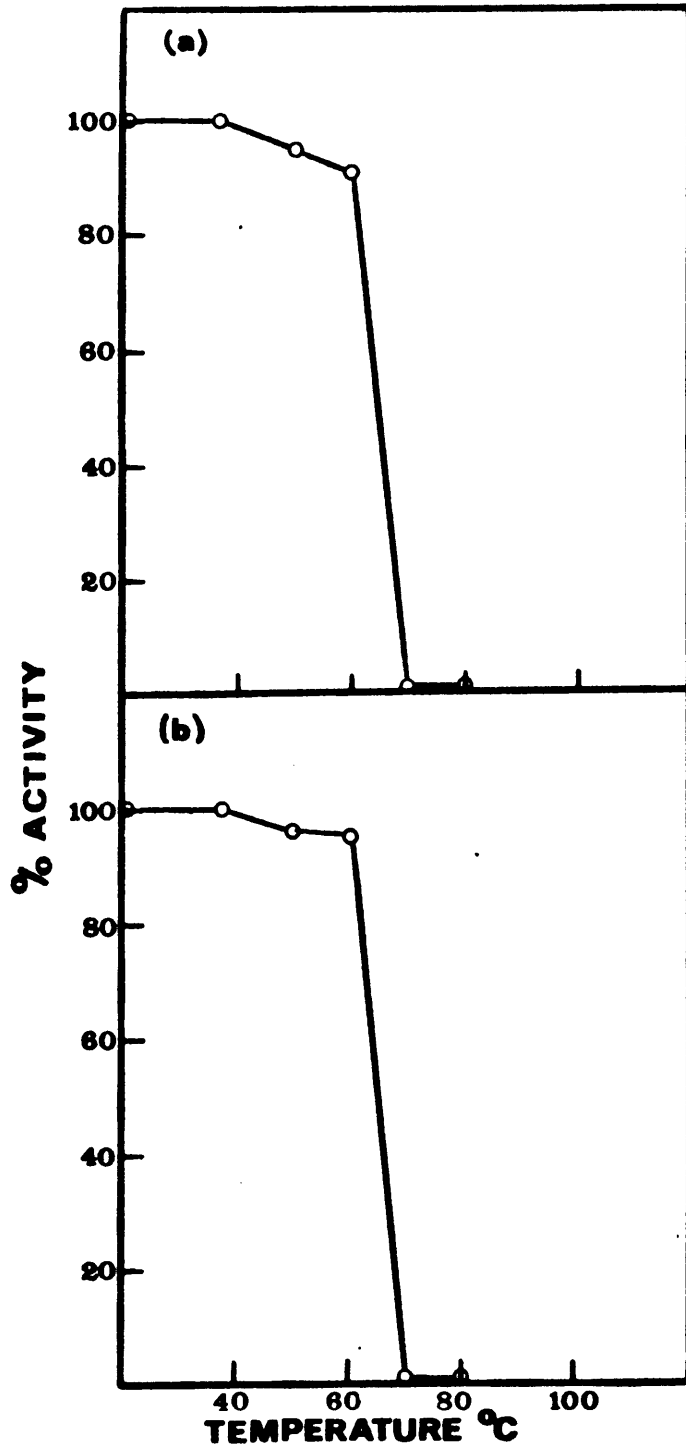
FIG. 5. Heat stability of the low molecular weight form of rabbit intestinal adenosine deaminase (a) using adenosine and (b) using deoxyadenosine as substrates. The suitably diluted enzyme (in 0.1 M phosphate pH 7.0) was heated for 15 min. at various temperatures and assays performed spectrophotometrically at 265 nm (pH 6.5).
