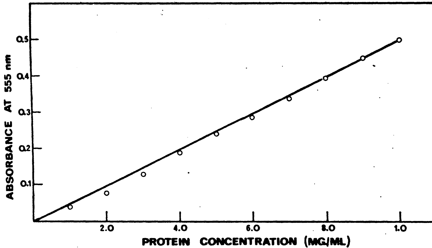
FIG. 1. Standard graph for measurement of protein concentration using the Biuret Method. Solutions of egg albumen (0 - 10 mg./ml.) were incubated with 4 ml. of Biuret reagent, and the absorbance at 555 nm measured after 30 min.
