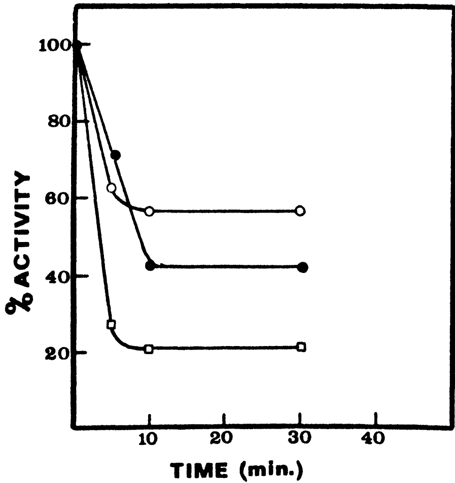
FIG. 36. The effect of anti-serum (rabbit) on the activity of bovine intestinal adenosine deaminase (□—□) and the low molecular weight (○—○) and the high molecular weight (●—●) forms of rabbit intestinal adenosine deaminase.
