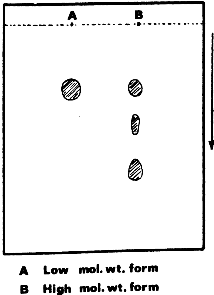
FIG. A. Thin-layer gel filtration pattern of the low and high molecular weight forms of rabbit intestinal adenosine deaminase after treatment with 6M guanidine hydrochloride. The enzymes were incubated with the reagent (in 0.5 M Tris pH 7.0) for 24 h. at 37°C and applied to a Sephadex G-75 coated thin-layer plate equilibrated with 0.5 M Tris pH 7.0 containing 6 M guanidine hydrochloride. After chromatography the plate was stained for protein using the Ponceau S-Nigrosine stain.
