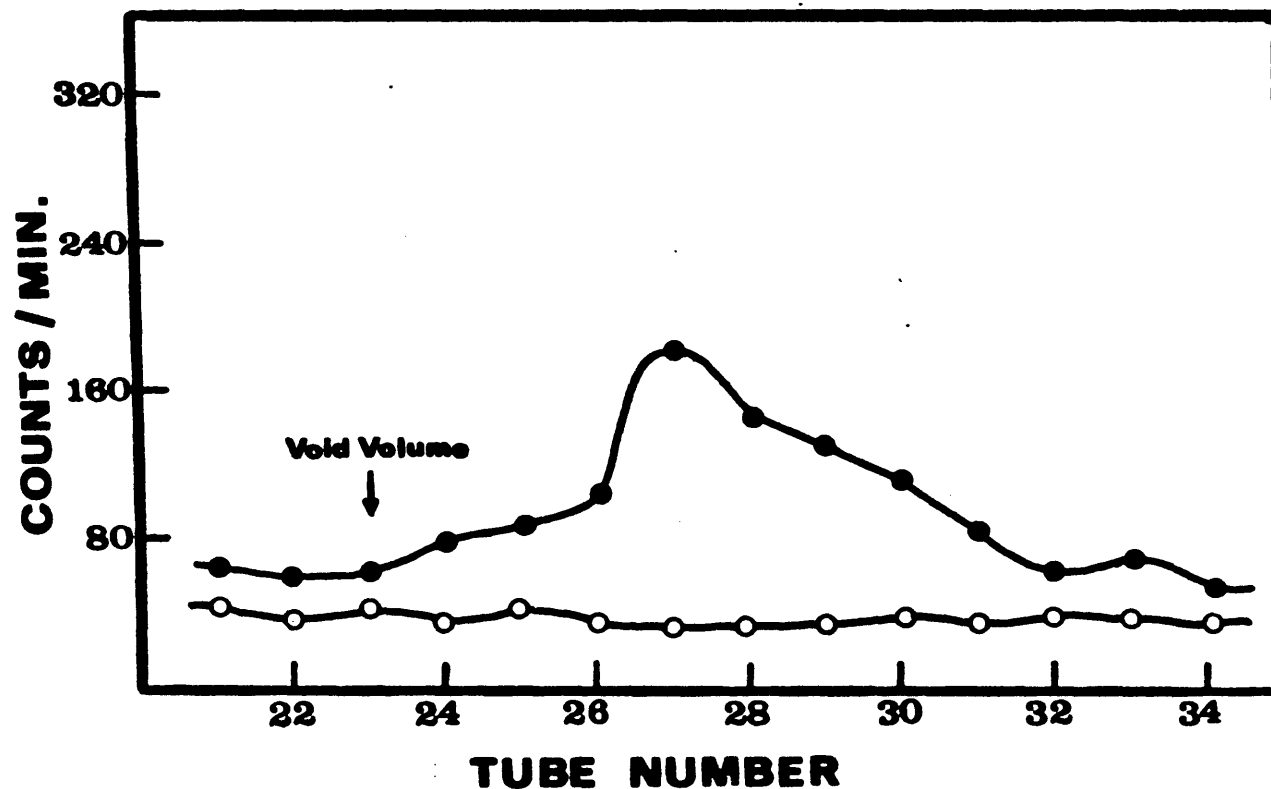
FIG. 40. Gel filtration of adenosine deaminase (treated with C^{14} -maleic anhydride) on Sephadex G-75 (Superfine). Bovine intestinal deaminase (●—●) and the high molecular weight form of rabbit intestinal adenosine deaminase (○—○) were treated with C^{14} -maleic anhydride and applied to the Sephadex column equilibrated with 10 mM phosphate pH 7.0 containing 10 mM \beta -mercaptoethanol. 3 ml. fractions were collected and radioactivity measured using a nuclear Chigago Gas Flow Detector.
