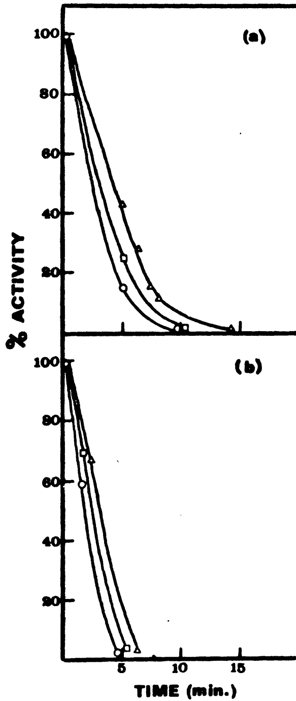
FIG. 24. The effect of photooxidation (using 0.01% rose bengal as sensitizer) on the activity of (a) the low molecular weight form and (b) the high molecular weight form of rabbit intestinal adenosine deaminase. \circ — \circ , pH 6.5; \square — \square , pH 5.0; \triangle — \triangle pH 8.6.
