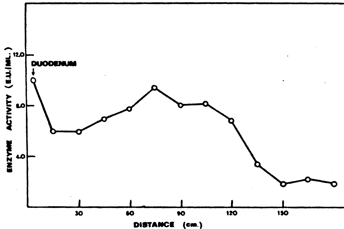
FIG. 4. Distribution of adenosine deaminase activity along the small intestine of the rabbit. Portions of tissue (0.5 g.) taken at 15 cm. intervals were extracted (dil. 1:10) and the activity of the supernatant fluid obtained after centrifugation estimated using the Microdiffusion Method of assay (pH 7.0).
