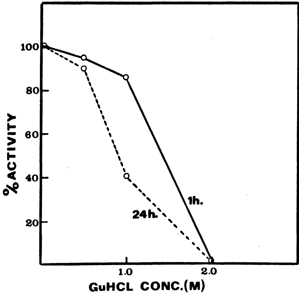
FIG. 14. Effect of guanidine hydrochloride on the activity of the low molecular weight form of rabbit intestinal adenosine deaminase. The diluted enzyme (in 0.1 M phosphate pH 7.0) was incubated at 37°C for 1 h. and 24 h. with the GuHCl solutions (1-2 M) and assays performed spectrophotometrically at 265 nm (pH 7.0).
