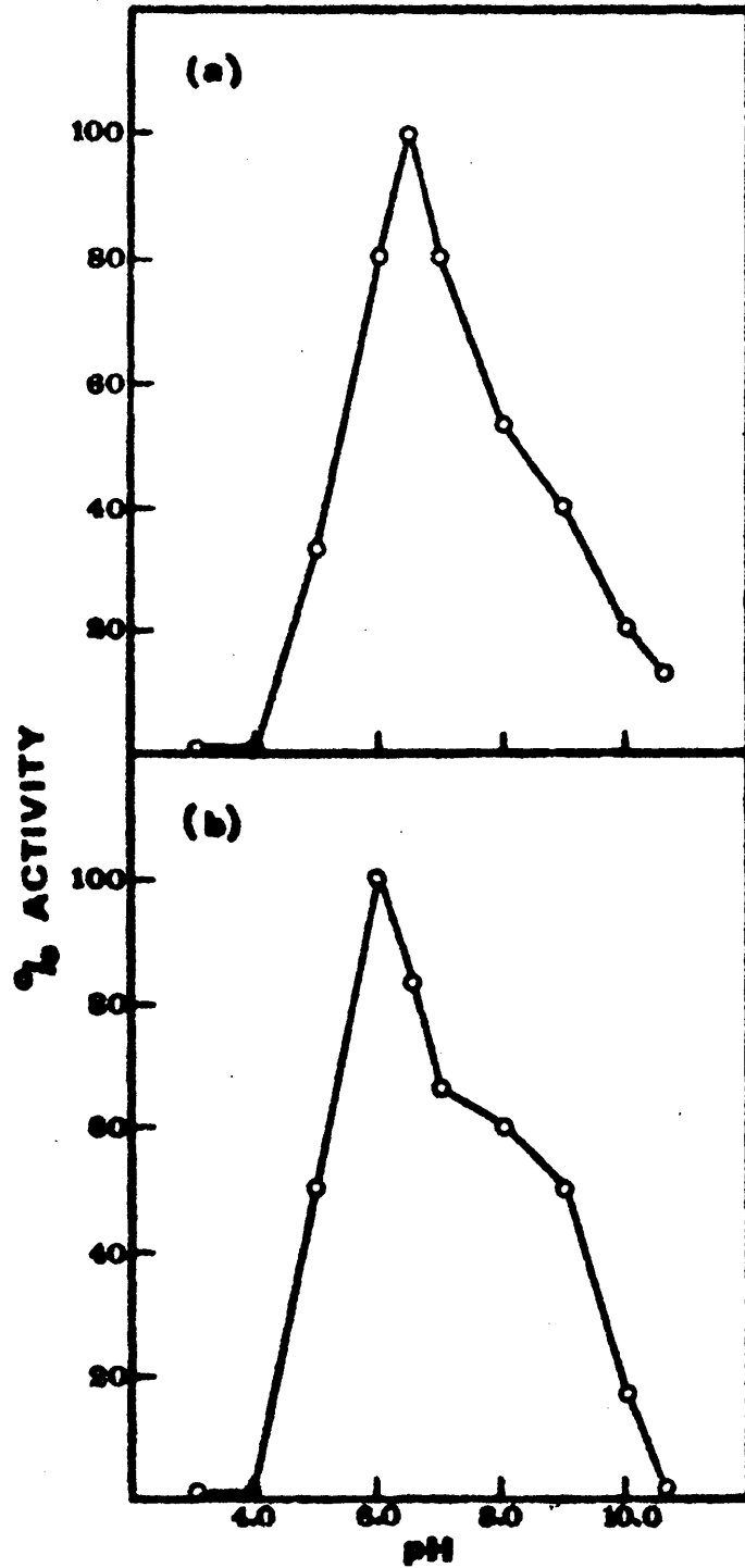
FIG. 2. pH activity profiles of the high molecular weight form of rabbit intestinal adenosine deaminase, (a) using adenosine and (b) using deoxyadenosine as substrates. Phosphate buffer (pH 3.0-8.0) and glycine buffer (pH 9.0-10.6) were used, and assays performed spectrophotometrically at 265 nm.
