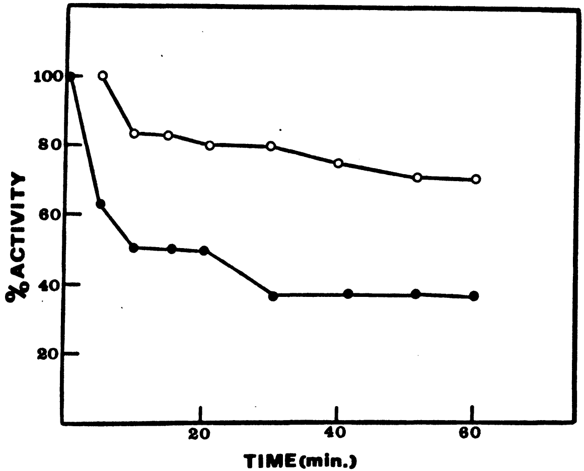
FIG. 16. The effect of 1.5 M guanidine hydrochloride on the activity of the low molecular weight form (○—○) and the high molecular weight form (●—●) of rabbit intestinal adenosine deaminase. The enzymes were incubated for 60 min. at 27°C in 1.5 M GuHCl (in 0.1M phosphate pH 7.0) and assays performed spectrophotometrically at 265 nm (pH 7.0).
