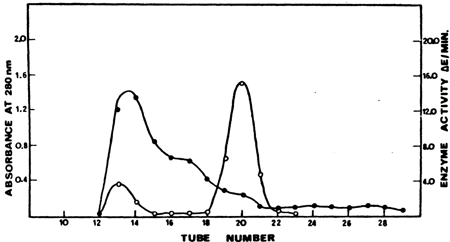
FIG. 17. Gel filtration of adenosine deaminase on Sephadex G-75 (Superfine). 1 ml. of concentrated enzyme solution after the DEAE chromatography step (sp. act. 16.8 e.u.) was applied to the column which was equilibrated with 0.002 M sodium citrate buffer pH 5.8. 5 ml. fractions were collected. Protein concentration was determined by absorption at 280 nm and enzyme activity estimated spectrophotometrically at 265 nm (pH 7.0). ●—● protein; ○—○, adenosine deaminase activity.
