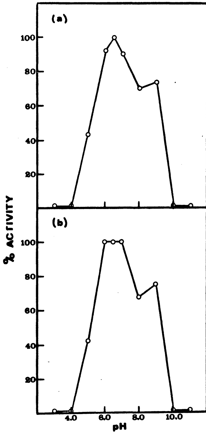
FIG. 3. pH stability profiles of the low molecular weight form of rabbit intestinal adenosine deaminase (a) using adenosine and (b) using deoxyadenosine as substrates. Phosphate buffer (pH 3.0-8.0) and glycine buffer (pH 9.0-10.6) were used, and assays performed spectrophotometrically at 265 nm.
