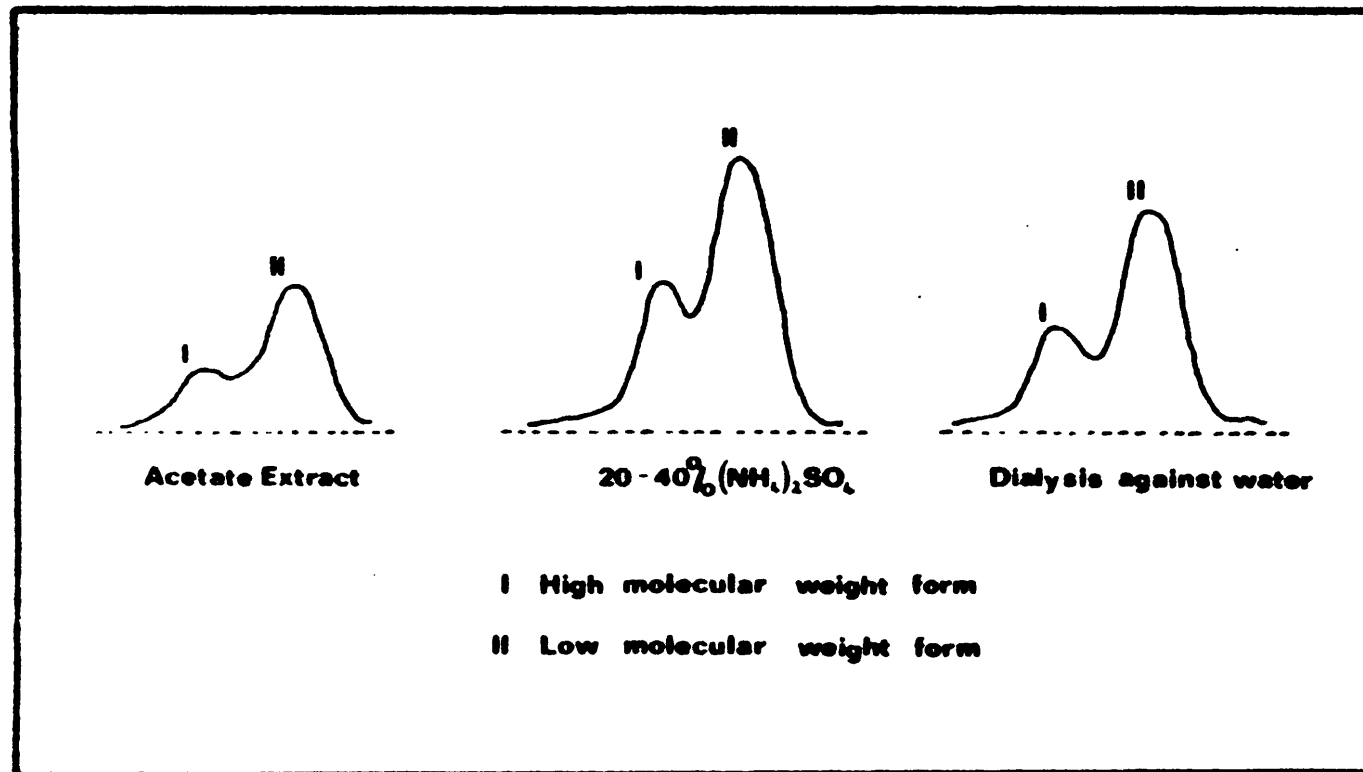
FIG.15. Densitometer tracings of thin-layer gel filtration patterns. Samples from the first three steps in the purification were applied to a Sephadex G-75 coated thin-layer plate and after development (using 0.05 M KCl as solvent) sites of enzyme activity were detected using the zymogram stain for adenosine deaminase.
