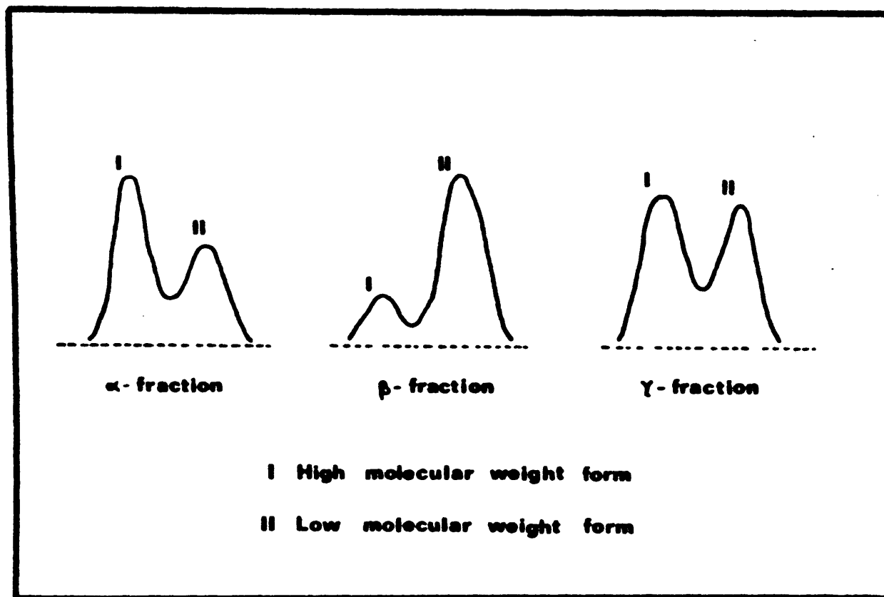
FIG. 28. Densitometer tracings of thin-layer gel filtration patterns. Samples of the \alpha -, \beta - and \gamma -fractions from the DEAE chromatography step were applied to a Sephadex G-75 coated thin-layer plate and after development (using 0.05 M KCl as solvent) sites of enzyme activity were detected using the zymogram stain for adenosine deaminase.
