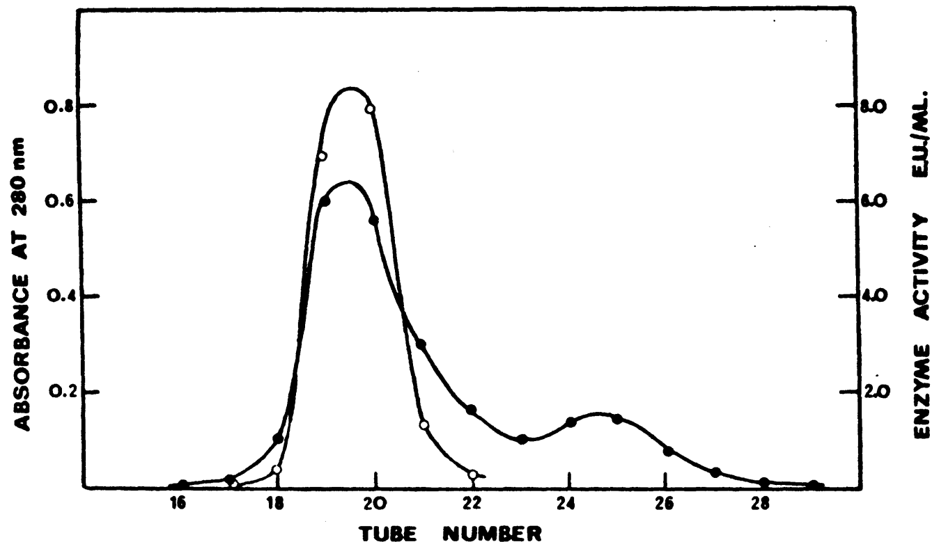
FIG. 26. Gel filtration of adenosine deaminase on Sephadex G-200 (Superfine). Tubes 12 and 13 from Sephadex G-75 1 (FIG. 23) were pooled, concentrated and applied to the column which was equilibrated with 0.002M sodium citrate buffer pH 5.8. 5 ml. fractions were collected. Protein concentration was determined by absorption at 280 nm and enzyme activity was estimated spectrophotometrically at 265 nm (pH 7.0). ●—●, protein; ○—○, adenosine deaminase activity.
