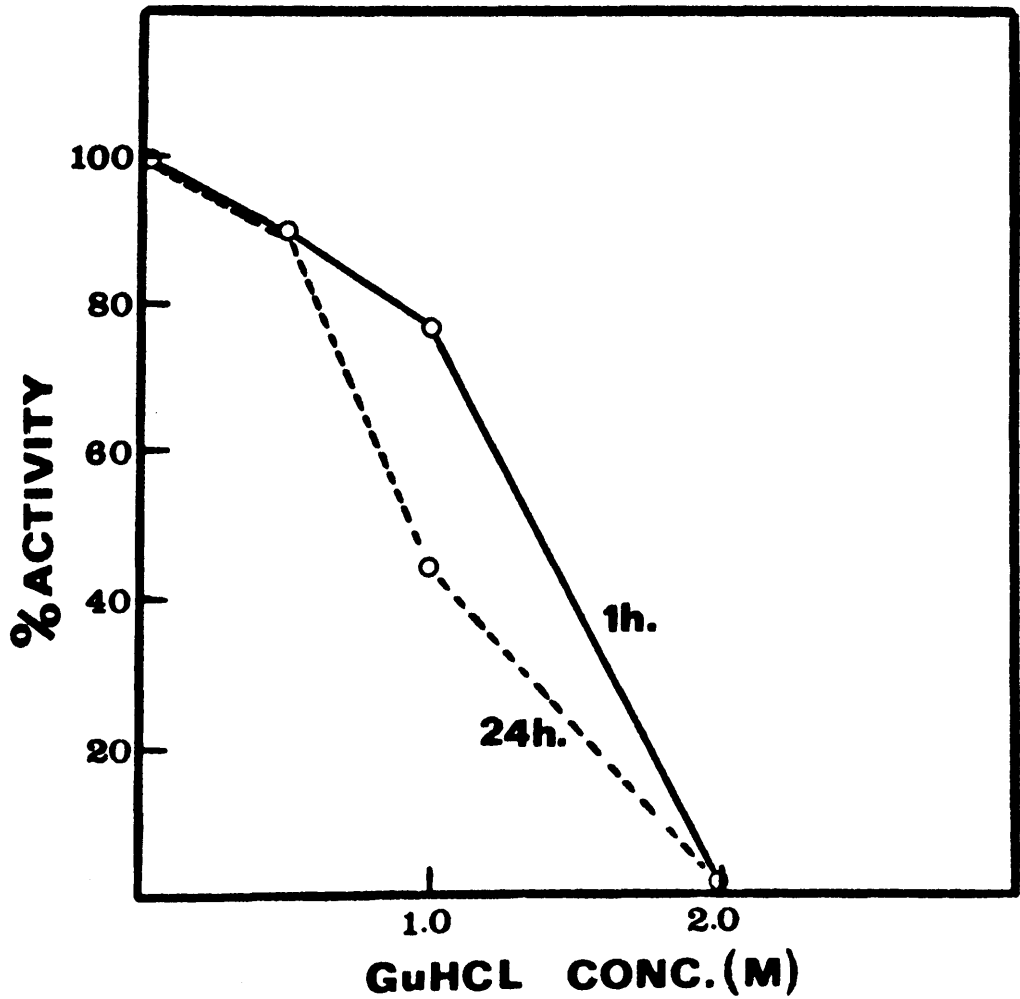
FIG. 15. Effect of guanidine hydrochloride on the activity of the high molecular weight form of rabbit intestinal adenosine deaminase. The diluted enzyme (in 0.1 M phosphate pH 7.0) was incubated at 37°C for 1 h. and 24 h. with the GuHCl solutions (1-2 M) and assays performed spectrophotometrically at 265 nm (pH 7.0).
