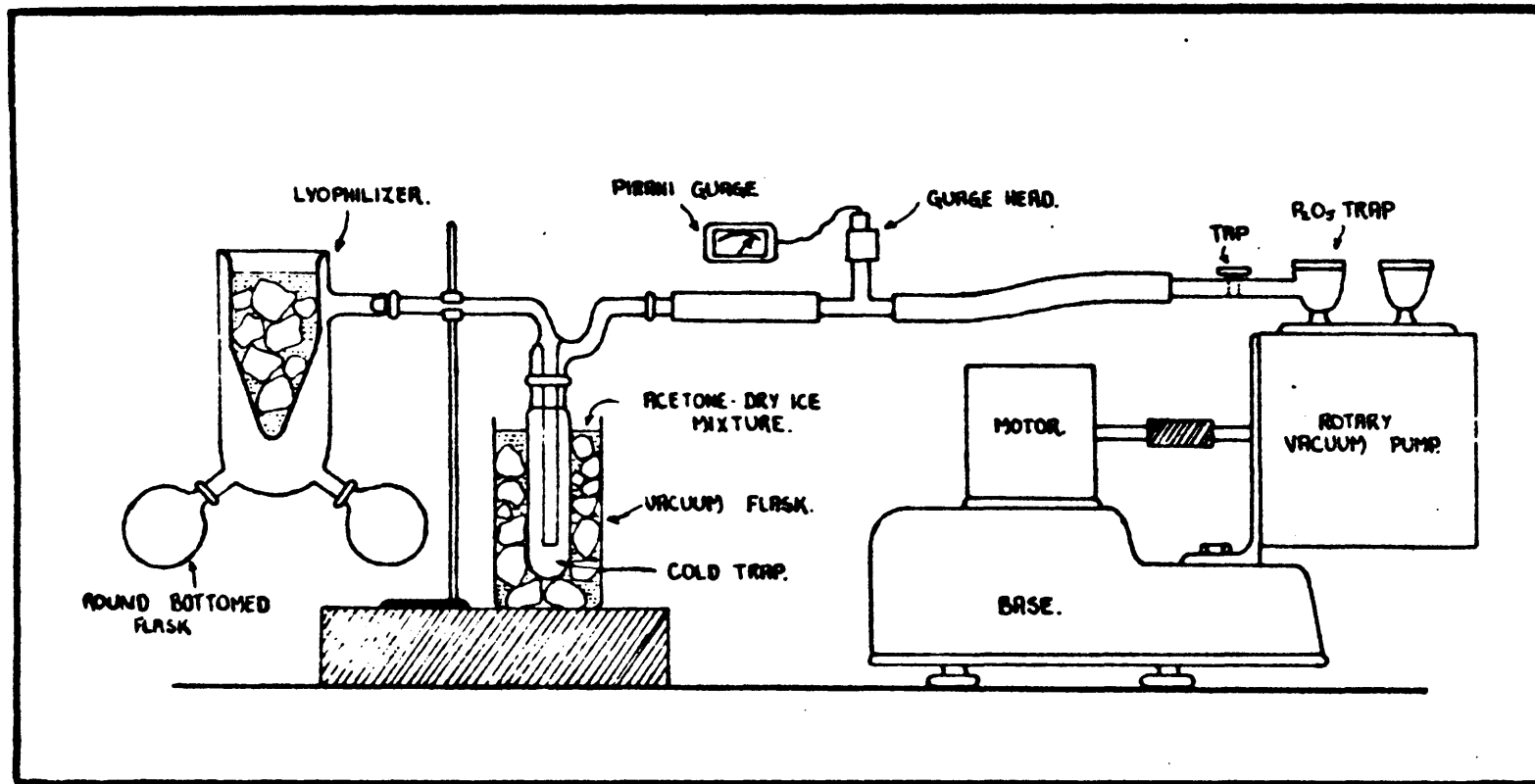
FIG. 2. Schematic representation of apparatus used for freeze drying adenosine deaminase solutions.
