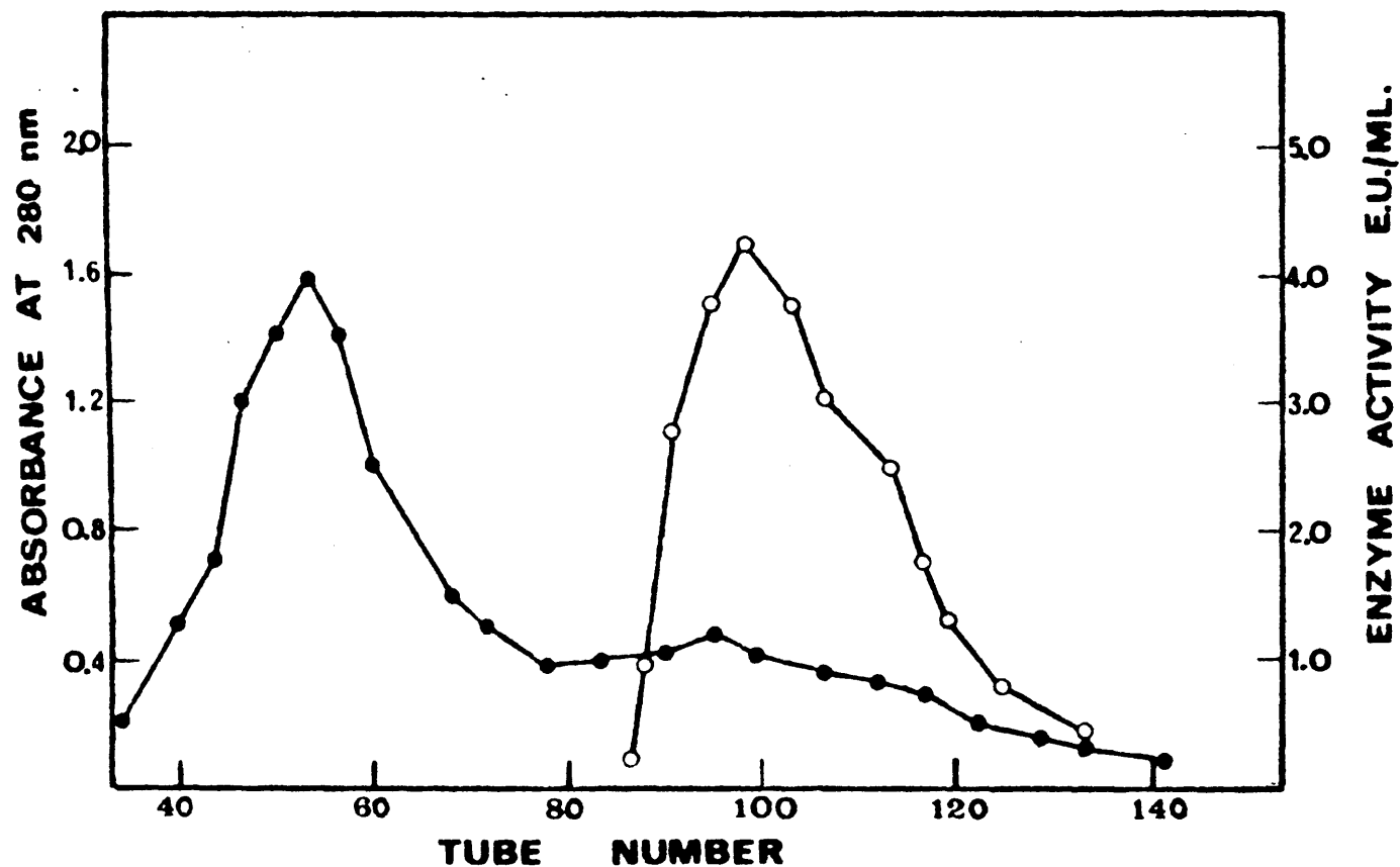
FIG. 9. Chromatography of adenosine deaminase on DEAE cellulose. 242 ml. of enzyme (after Sephadex G-75 chromatography : sp. act. 3.15 e.u.) was applied to the column and eluted using a sodium citrate gradient (pH 5.8) from 0.002 - 0.03 M. 3 ml. fractions were collected. Protein concentration was measured by absorption at 280 nm and enzyme activity estimated using the Microdiffusion Method of assay (pH 7.0). ●—● , protein; ○—○ , adenosine deaminase activity.
