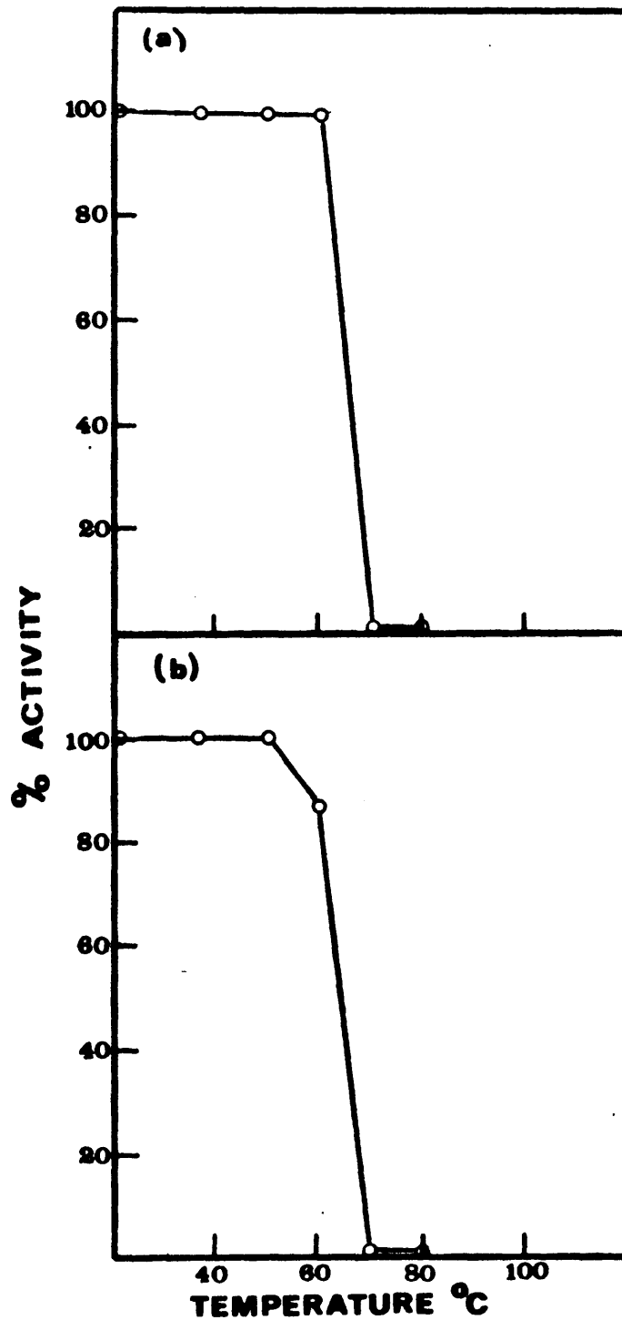
FIG. 6. Heat stability of the high molecular weight form of rabbit intestinal adenosine deaminase (a) using adenosine and (b) using deoxyadenosine as substrates. The suitably diluted enzyme (in 0.1 M phosphate pH 7.0) was heated for 15 min. at various temperatures, and assays performed spectrophotometrically at 265 nm.
