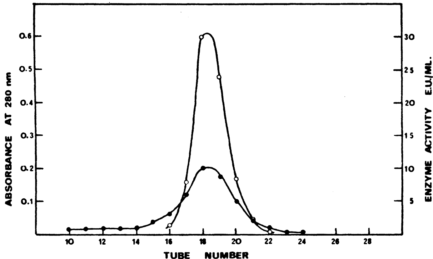
FIG. 25. Sephadex G-75 111. Gel filtration of adenosine deaminase on Sephadex G-75 (Superfine). Tube 20 from Sephadex G-75 1 (FIG. 23) and tubes 19 and 20 from Sephadex G-75 11 (FIG. 24) were pooled, concentrated and applied to the column equilibrated with 0.002 M sodium citrate buffer pH 5.8. 5 ml. fractions were collected. Protein concentration was determined by absorption at 280 nm and enzyme activity was estimated spectrophotometrically at 265 nm (pH 7.0). ●—●, protein; ○—○, adenosine deaminase activity.
