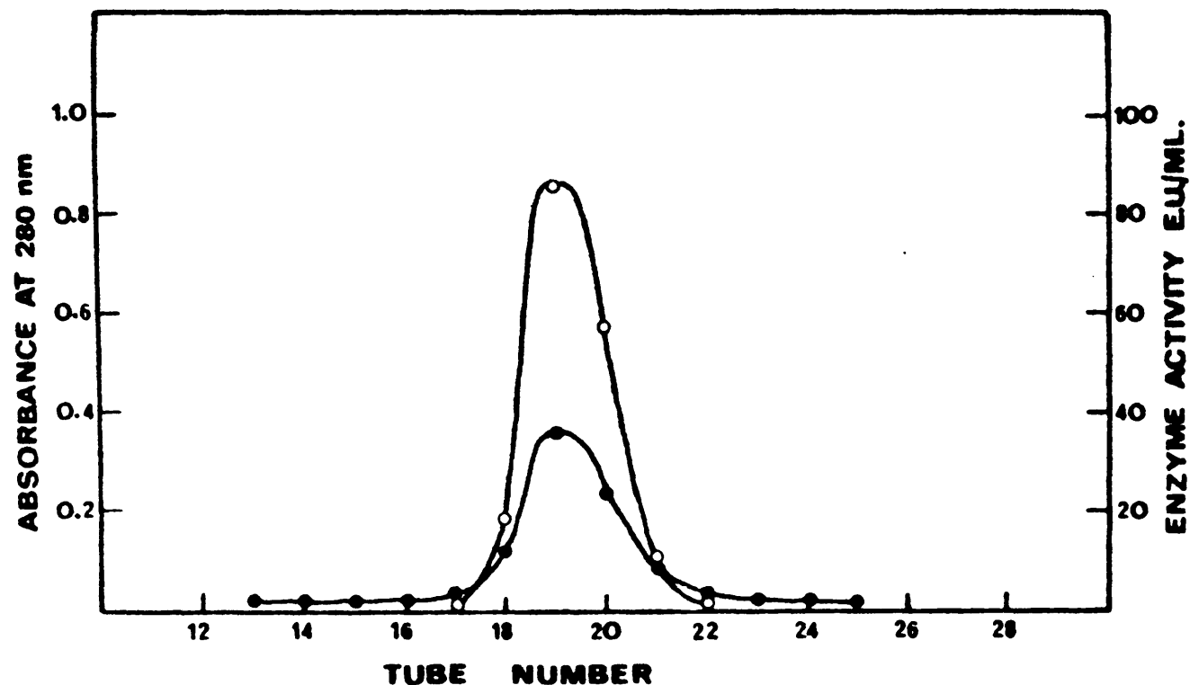
FIG. 18. Gel filtration of adenosine deaminase on Sephadex G-75 (Superfine). A number of low molecular weight enzyme preparations (prepared as described in Purification IV) were pooled, concentrated and applied to the column which was equilibrated with 0.002M sodium citrate buffer pH 5.8. 5 ml. fractions were collected. Protein concentration was determined by absorption at 280 nm and enzyme activity estimated spectrophotometrically at 265 nm (pH 7.0). ●—●, protein; ○—○, adenosine deaminase activity.
