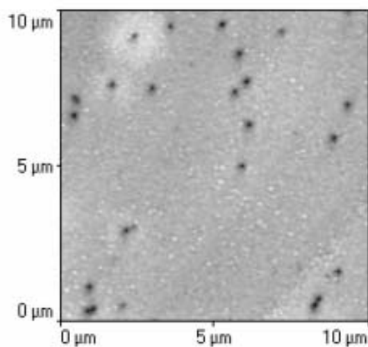
Fig. 8 AFM image of the surface of an InP electrode subjected to a potential sweep from 0.0 V to 0.48 V at 2.5 \text{ mV s}^{-1} in 5 \text{ mol dm}^{-3} \text{ KOH} .
