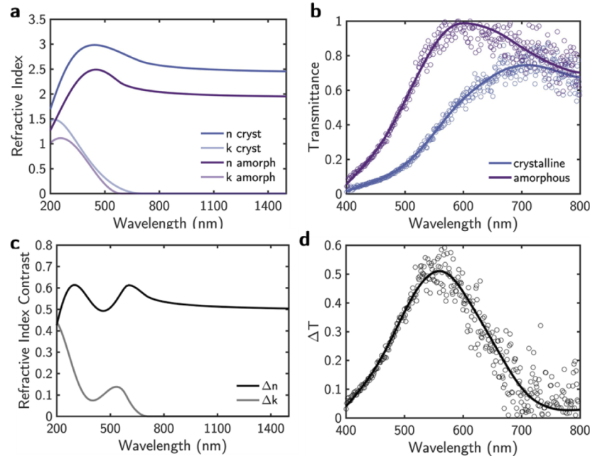
Fig. 2. (a) Refractive index ( n + ik ) of as-grown amorphous and thermally crystallized Sb 2 S 3 . (b) Transmittance of the as-grown amorphous and thermally crystallized Sb 2 S 3 . (c) Refractive index contrast \Delta n and \Delta k between amorphous and thermally crystallized Sb 2 S 3 . (d) Difference in the transmittance spectra \Delta T measured on the as-grown amorphous and thermally crystallized Sb 2 S 3 film.
