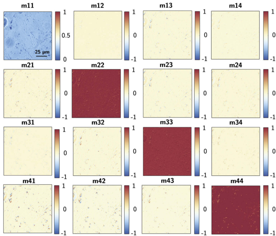
Fig. 3. Experimental Mueller matrix of amorphous \text{Sb}_2\text{S}_3 films measured at \lambda = 634 \text{ nm} with a 5\times microscope objective.
