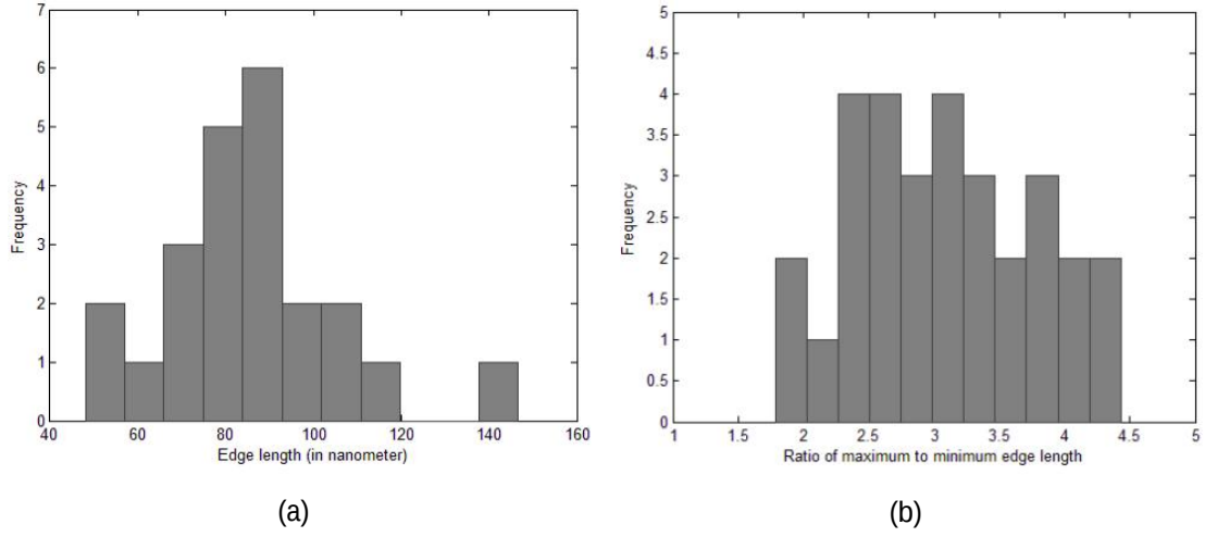
Figure 4.11: Checking deformation through edge length. (a) Distribution of edge lengths from a single metabolosome. (b) Distribution of edge length ratio from 30 metabolosomes.
