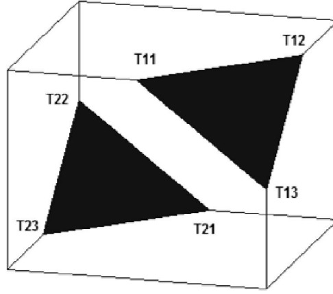
Figure 6.3: A cube truncated by two parallel planes ( T11, T12, T13 ) and ( T21, T22, T23 ).
