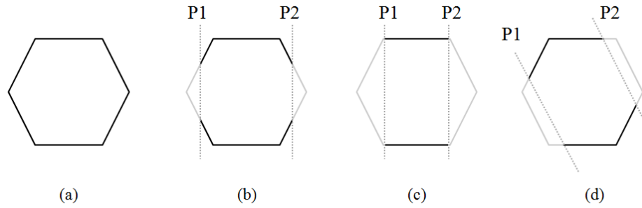
Figure 6.2: Effects of truncation parameters. (a) A complete hexagon. (b) Two parallel planes P_1 and P_2 truncate the shape. The truncated shape has 4 vertices and 6 edges. (c) Increased truncation proportion keeping the truncation angle fixed as (b) - the truncated shape has only 2 edges, no vertex. (d) Changed truncation angle, keeping truncation proportion fixed as (b) - the truncated shape has 2 vertices and 4 edges.
