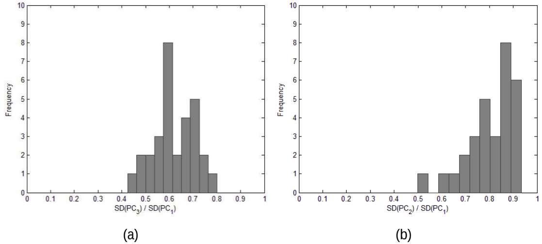
Figure 4.14: The distribution of the aspect ratios. (a) The distribution of R_1 and (b) the distribution of R_2 , calculated from 30 metabosomes.
