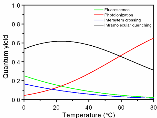
Figure S.6. Calculated quantum yields of fluorescence, intersystem crossing, photoionization and intramolecular quenching for tryptophan at pH 7, as a function of temperature.
