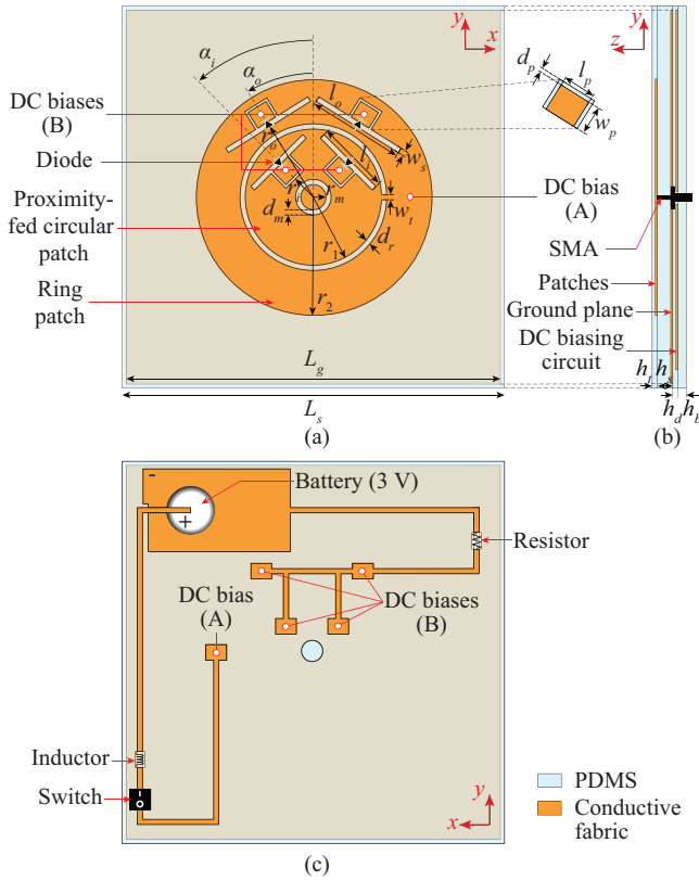
Fig. 1. Proposed antenna geometry: (a) front view, (b) side view, and (c) back view. The final dimensions (in millimeters) are: r_m = 2.4 , d_m = 1 , r_1 = 13 , r_2 = 22.5 , d_r = 1 , L_i = 14 , L_o = 18.5 , w_s = 1 , r_i = 4.9 , r_o = 15.8 , \alpha_i = 45^\circ , \alpha_o = 32^\circ , L_p = 4 , w_p = 3.5 , d_p = 0.5 , w_t = 1 , L_s = 70 , L_g = 68 , h_t = 0.3 , h_s = 5.5 , h_d = 0.3 , and h_b = 0.5
