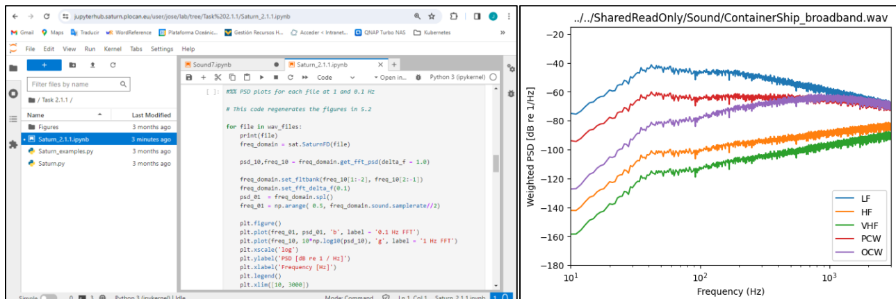
Figure 2: Left: Notebook with "standardisation code." Right: PSD output of Notebook.
