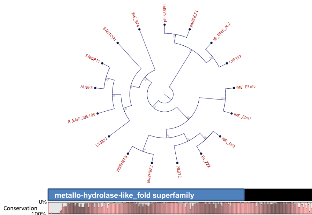
Figure 2. Maximum likelihood phylogenetic analysis sequence relatedness of the Enterococcus faecalis phage putative metallo-beta-lactamase gene (orthologous group 32); tree node labels represent bootstrap values.
