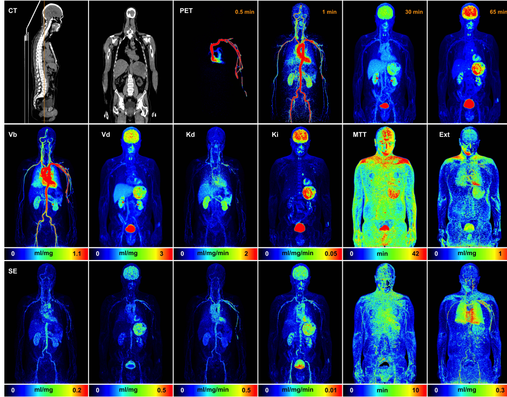
Figure 4.2: MIP maps of NPRM kinetic parameters including associated SEs. SEs are based on the standard deviation of MIP results for each of 25 bootstrap replications. Top-row: CT images for a selected cross-sections through the volume and PET MIP maps at indicated times.
