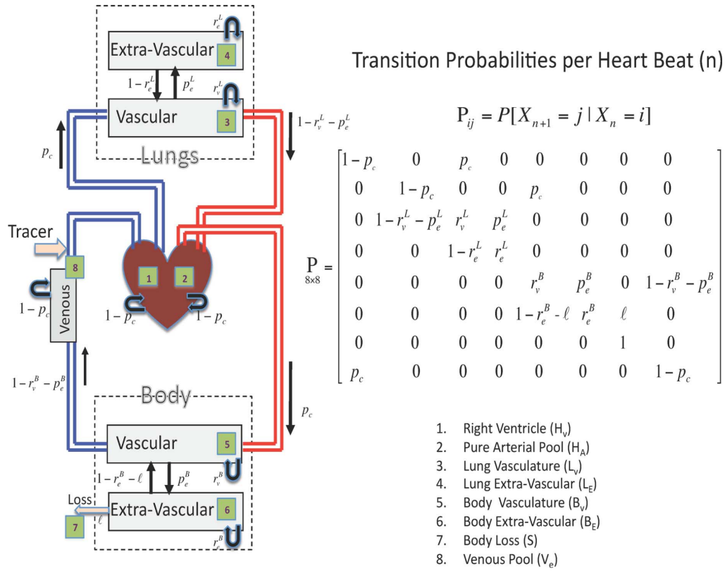
Figure 2.7: Markov chain model for tracer atom dynamics within the body. Graph representation (left). Transition matrix (right). (Huang & O'Sullivan 2014)
