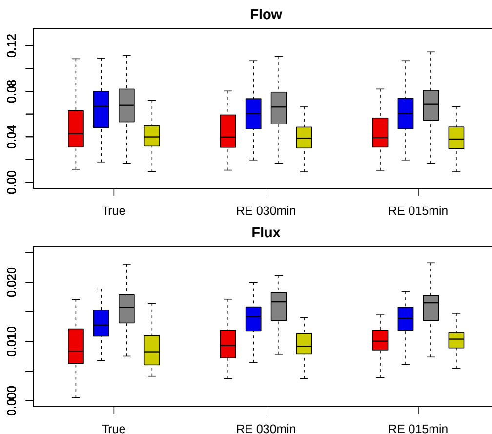
Figure 5.9: The boxplot shows the distribution of Flow and Flux recovered from a full scan using NPRM, and the use of residue extension with short acquisition times of 15 and 30 minutes. The colors refer to different regions: red for tumors, blue for the whole brain, grey for grey matter, and yellow for white matter.
