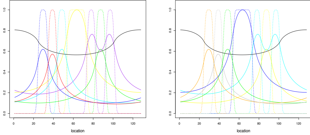
Figure 3.8: Scaled spatial patterns ( \alpha_j ) for source distribution in 1-D experiments (dotted lines); projection domain patterns ( K_\beta \alpha_j ) are also shown (solid lines). Left - FDG studies; Right - FLT studies. Source sub-TACs ( \mu_j ) are in Figure 3.4 A(ii) (FDG) and Figure 3.4 B(ii) (FLT). Colors of \alpha_j 's here match the colors of corresponding sub-TACs in Figure 3.8. The solid black line is the attenuation pattern.
