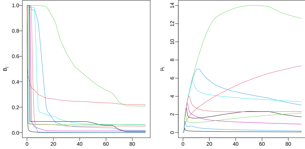
Figure 5.5: Population residue basis B_j(t) and a sample basis elements \mu_j(t) in a brain tumor study.
