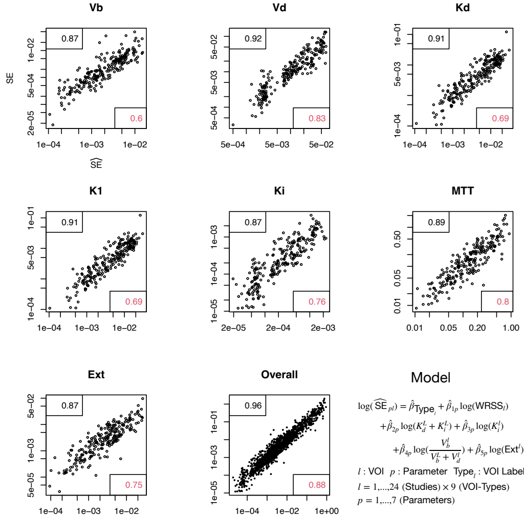
Figure 4.6: Prediction of VOI kinetic standard errors (SE - vertical axes) via a log-linear model prediction ( \hat{SE} - horizontal axes) - formula indicated. Correlations in black are for logarithmic SE values; red for the raw scale.
