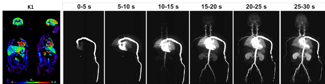
Figure 2.6: Voxel level quantitative parametric perfusion image with radio-tracer delay. (left). ^{15}\text{O}\text{-H}_2\text{O} dynamic images with 5s duration in each time frame after tracer injection. (right series) (Knuuti et al. 2023)
