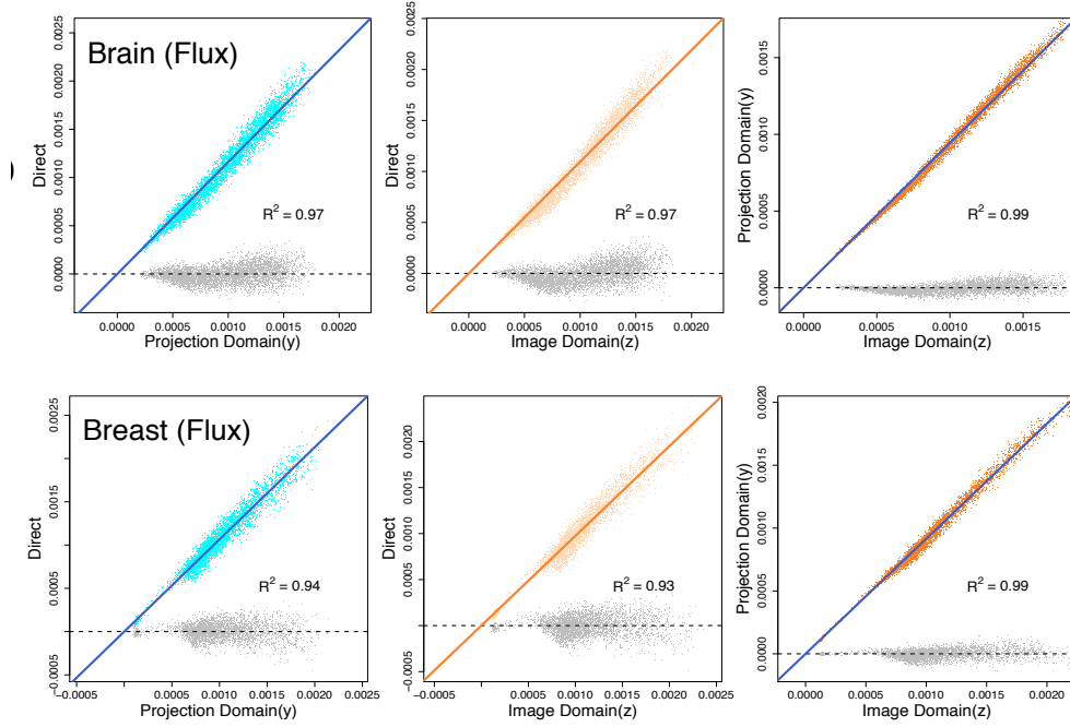
Figure 3.6: Voxel estimates of average standard deviations of flux. The true values are estimated by direct replication, these values are compared to image and projection domain bootstraps for a single replicate.
