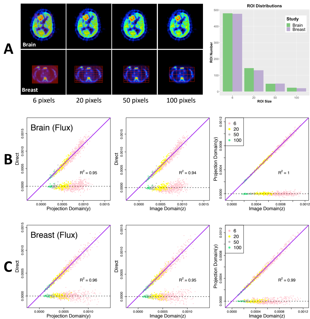
Figure 3.7: Schematic for 2-D investigation of Bootstrapping ROI averages. A total of 696 and 676 ROIs are defined for Brain and Breast, respectively. (A) Grids of rectangular ROIs and their size distributions. Estimates of average ROI standard deviations of flux are shown on rows B and C - colors correspond to different ROI sizes.
