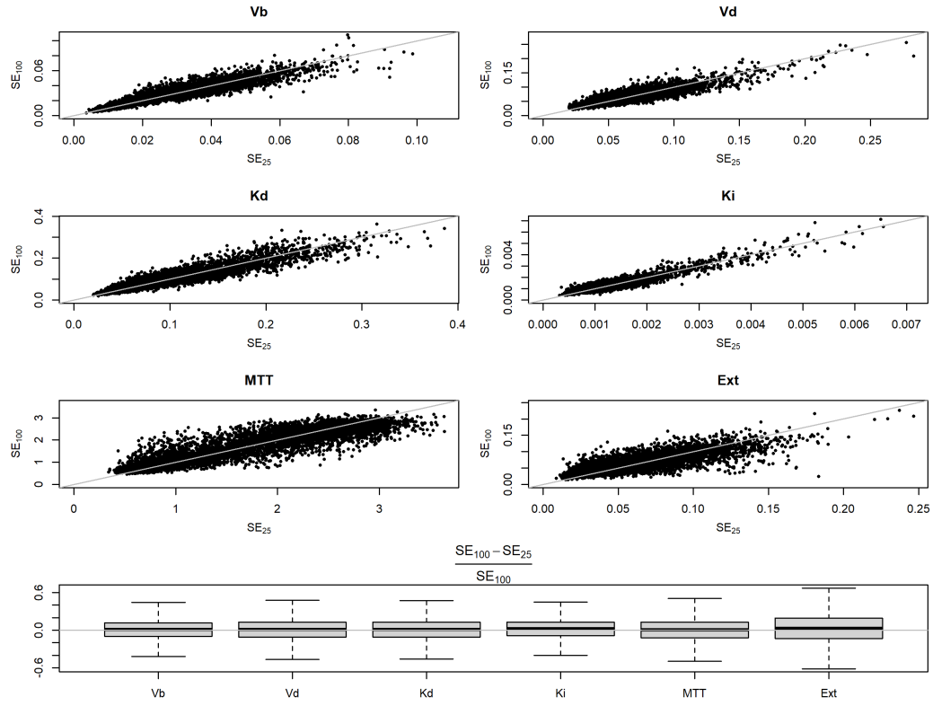
Figure 4.8: Comparison of bootstrap generated voxel-level SEs based on 25 and 100 bootstrap samples - SE_{25} and SE_{100} . Points correspond to 5000 voxels randomly sampled from each VOI. The boxplot shows the relative deviations between SE_{25} and SE_{100} . The mean absolute deviation is on the order of 10% for all parameters.
