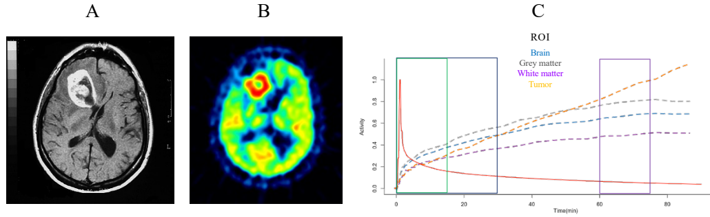
Figure 5.2: Diagram of resampled PET-FDG scan data in brain tumour series. First 15 minutes(green), 0-30 minutes(navy) and clinical setting 60-75 minutes(purple). A similar resampling approach was used for the breast series.
