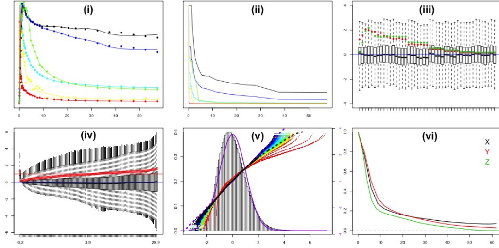
Figure 3.3: Diagnostics associated with the Image-Domain Bootstrapping Model (3.2) using the FLT-Breast data. Six plots, labeled (i) to (vi), are shown for each dataset: (i) raw sub-TACs (dots) and fitted models (lines) for the selected basis set - columns of X . (ii) Non-parametric residues corresponding to the fitted model - c.f. (3.10). (iii) Boxplots by time-frame of standardized residuals from the unconstrained least squares fit, r_{ij}/\hat{\sigma}_i\hat{\phi}_j\hat{h}_{ij} . The simple, \hat{\phi}_j^0 in (3.5), and optimized, \hat{\phi}_j , standard deviations are shown as green and red dots. (iv) Boxplots of scaled residuals, \hat{\epsilon}_{ij} = r_{ij}/\hat{\sigma}_i\hat{\phi}_j , for each \kappa -bin (each containing roughly 10000 data points). \hat{h}_l -values are shown as red points; the red line is for comparison with unity (zero skewness of bin data). (v) Histogram of the overall distribution of the standardized residuals and its relation to a Gaussian fit (purple curve). Super-imposed are points showing quantiles of standardized residuals from different \kappa -bins (colored from red to dark blue according to bin order) versus corresponding quantiles of the Gaussian (right y-axis). The quantile pattern for the overall histogram and the Gaussian fit are shown with dashed black and purple lines. (vi) Directional auto-correlation patterns of the normalized residuals, \hat{\eta} , as a function of distance in millimeters. X-Y are transverse with Y perpendicular to the scanning bed; Z is the axial direction.
