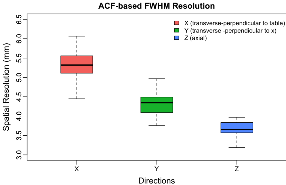
Figure 4.5: ACF-based measure of Scanner FWHM Resolution. Note this measure takes account of patient specific factors - activity distribution, positioning and movements associated with breathing etc - which may impact the 3-D resolution of data.
