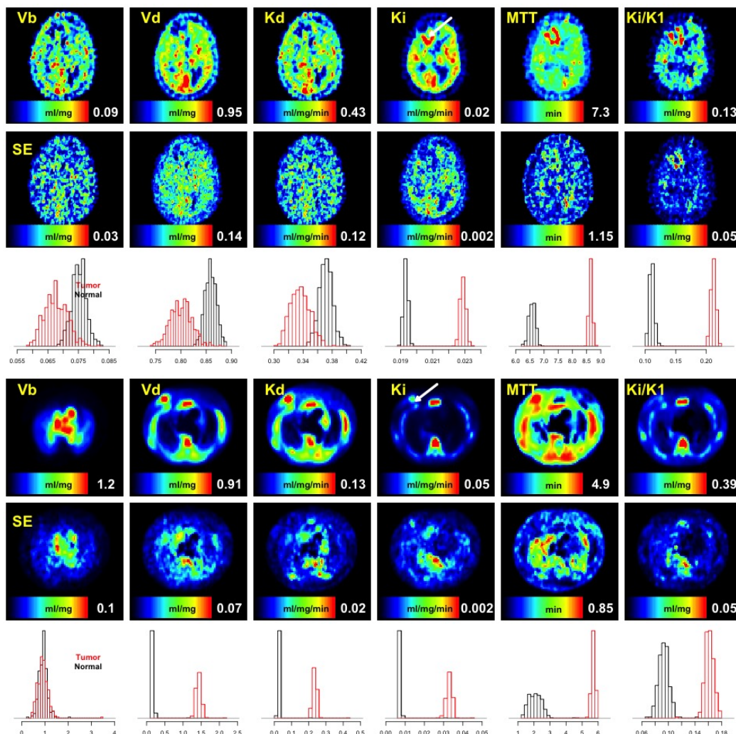
Figure 3.1: Metabolic Images with image-domain bootstrap assessment of standard errors: Rows 1-3 show the Brain tumor FDG data; 4-6 for the Breast tumor FLT data. The mapped parameters are shown on rows 1&4 – the location of tumor volume of interest (VOI) on the slice is indicated with an arrow. Columns correspond to different metabolic parameters (labeled in yellow) with color bars indicating units - see section 3.3.1 for definitions. Computed standard errors (SE) are on rows 2&5. Rows 3&6 show histograms of the bootstrap sampling distributions of the 95th percentile of the metabolic parameter in the normal [black] and tumor [red] VOIs.
