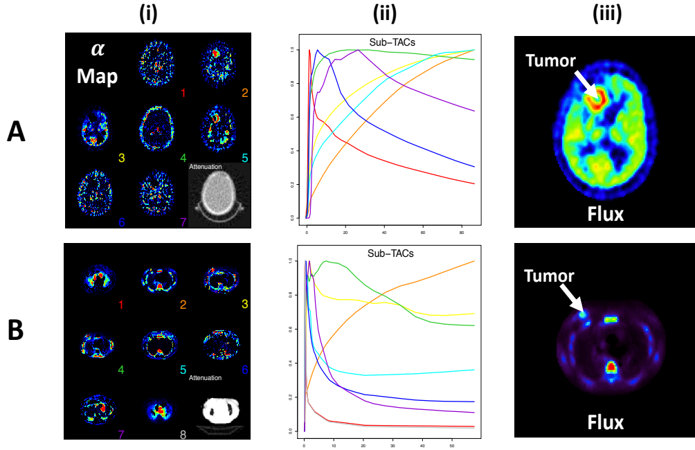
Figure 3.4: Source distribution, \lambda_{xt} = \sum_{k=1} \alpha_k(x)\mu_k(t) , for the 2-D simulation experiments. Rows correspond to the FDG-Brain data (A) and FLT-Breast data (B). \alpha_k(x) patterns and attenuation in (i), time-courses for each component, \mu_k(t) (normalized), are in (ii). Flux parameters are in (iii).
