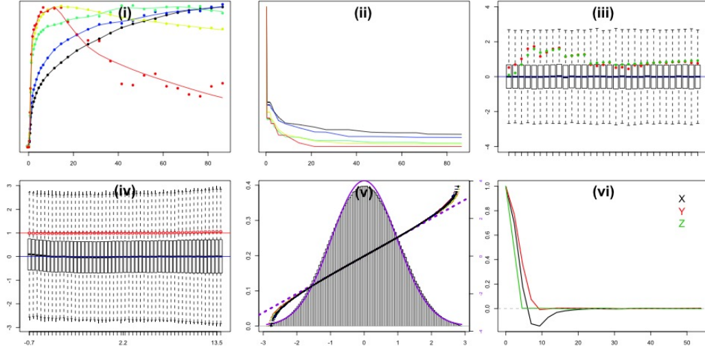
Figure 3.2: Diagnostics associated with the Image-Domain Bootstrapping Model (3.2) using the FDG-Brain data. Six plots, labeled (i) to (vi), are shown for each dataset: (i) raw sub-TACs (dots) and fitted models (lines) for the selected basis set - columns of X . (ii) Non-parametric residues corresponding to the fitted model - c.f. (3.10). (iii) Boxplots by time-frame of standardized residuals from the unconstrained least squares fit, r_{ij}/\hat{\sigma}_i\hat{\phi}_j\hat{h}_{ij} . The simple, \hat{\phi}_j^0 in (3.5), and optimized, \hat{\phi}_j , standard deviations are shown as green and red dots. (iv) Boxplots of scaled residuals, \hat{\epsilon}_{ij} = r_{ij}/\hat{\sigma}_i\hat{\phi}_j , for each \kappa -bin (each containing roughly 10000 data points). \hat{h}_l -values are shown as red points; the red line is for comparison with unity (zero skewness of bin data). (v) Histogram of the overall distribution of the standardized residuals and its relation to a Gaussian fit (purple curve). Super-imposed are points showing quantiles of standardized residuals from different \kappa -bins (colored from red to dark blue according to bin order) versus corresponding quantiles of the Gaussian (right y-axis). The quantile pattern for the overall histogram and the Gaussian fit are shown with dashed black and purple lines. (vi) Directional auto-correlation patterns of the normalized residuals, \hat{\eta} , as a function of distance in millimeters. X-Y are transverse with Y perpendicular to the scanning bed; Z is the axial direction.
