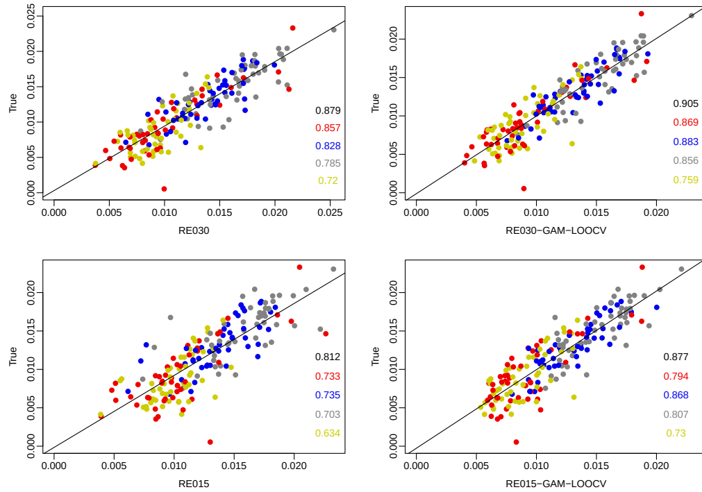
Figure 5.10: The comparison of flux values at the regional level. Left column: direct comparison of flux recovered from different methods. Right column: prediction of Flux as described in Section 5.2.5, using GAM and LOOCV. The colors refer to different regions: red for the tumor, blue for the whole brain, grey for grey matter, and yellow for white matter. The correlations shown in black represent overall correlations, the others correspond to their respective colors.
