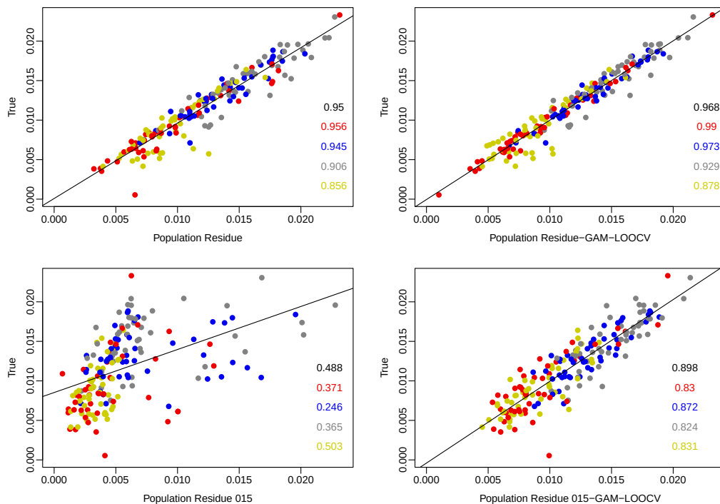
Figure 5.8: The comparison of flux values at the regional level. Left column: direct comparison of flux recovered from different methods. Right column: prediction of Flux as described in Section 5.2.4, using GAM and LOOCV. The colors refer to different regions: red for the tumor, blue for the whole brain, grey for grey matter, and yellow for white matter. The correlations shown in black represent overall correlations, the others correspond to their respective colors.
