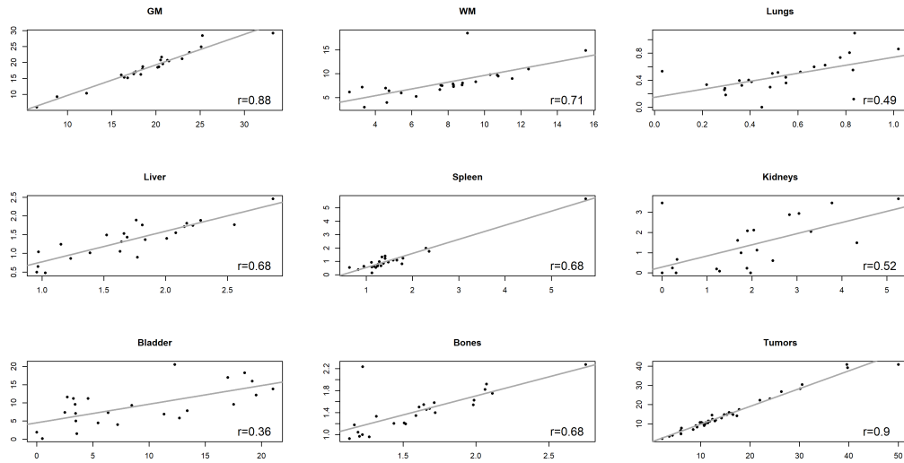
Figure 4.9: Pairwise plots for each VOI type of the relation between ^{18}\text{F} -FDG flux values ( \text{MR}_{\text{FDG}} ) computed using the NP-voxel (vertical-axis) and 2C (horizontal) analysis. Correlation (indicated by: r = ** ) values and best fitting linear regression (solid line) are shown.
