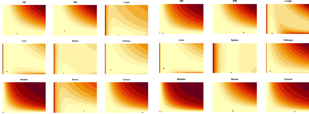
Figure 4.7: Contoured images of the reduced objective function in 2C-VOI analysis, g(\phi_2, \phi_1|\Delta) in equation(4.5) with \Delta fixed at the optimal value, over a fine grid of values for (\phi_2, \phi_1) . Darker colors correspond to large values for the objective function. The minimum value of the objective function over the grid is the red point; the value determined by the Broyden-Fletcher-Goldfarb-Shanno algorithm is in blue. Two panels of results for 9 VOIs are shown. The left set is for the VOI data in Figure 4.3; the right set is for a time-course corresponding to a randomly selected voxel in each VOI. Note the colors in each image ranges from the minimum (bright yellow) to a maximum (dark red). In all cases the value of the objective function at the blue point is no bigger than its value at the red point, demonstrating the reliability of the algorithm.
