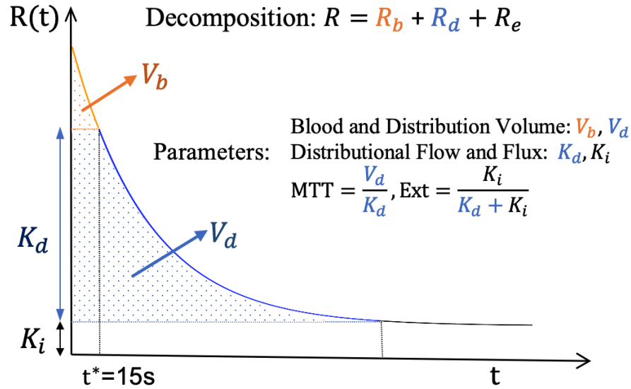
Figure 4.1: Meier-Zierler tissue residue ( R ) and a decomposition into vascular ( R_b ), based on consideration of atoms with travel-times less than 15 seconds in the tissue), in-distribution ( R_d ) and extracted ( R_e ) components. These are used to define associated metabolic parameters indicated.
