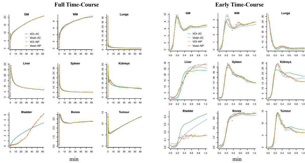
Figure 4.3: Results of four fitting procedures to the VOI time-course data in Figure 4.2. Data are points, line-colors correspond to methods used [top-left]. Full time course on the left; first minute on the right.
