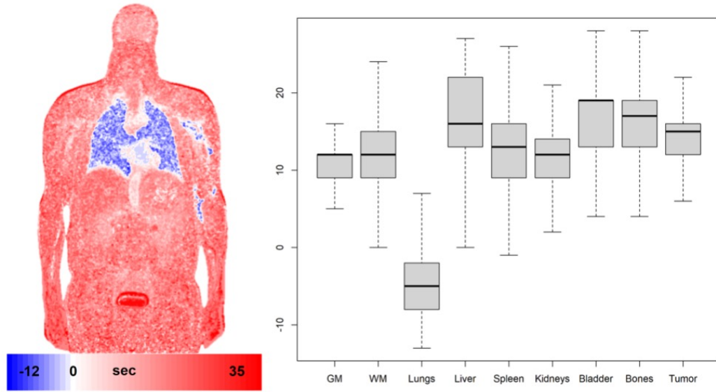
Figure 4.10: Voxel mapping of arrival of ^{18}\text{F} -FDG signal. Mapped values are the amplitude-weighted delay values, \{\delta + \Delta_k, k = 1, 2, \dots, K\} in equation 4.6. Data are centered so that the mean delay in the LV is zero. Left: Image of coronal scan corresponding to the CT slice in Figure 4.2. The boxplot on the right shows the distribution of mapped delay values by VOI.
