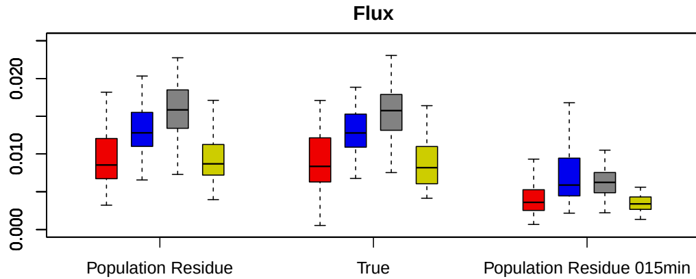
Figure 5.7: The boxplot shows the distribution of Flux recovered from a full scan using NPRM, the application of population residue, and the use of population residue with a short acquisition time of 15 minutes. The colors refer to different regions: red for tumor, blue for the whole brain, grey for grey matter, and yellow for white matter.
