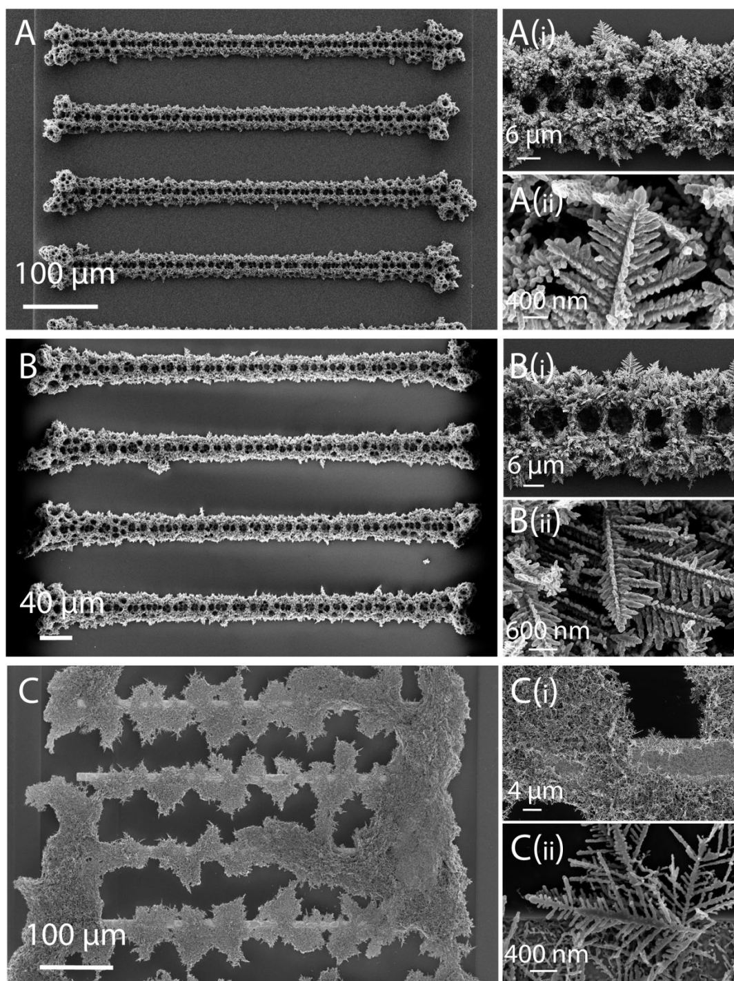
Figure 2. SEM images of BA10-CuFoam electrodes prepared at different \text{H}_2\text{SO}_4 concentrations; (A, A-i and A-ii; increased magnification), 1M \text{H}_2\text{SO}_4 , (B, B-i and B-ii; increased magnifications) 0.5M \text{H}_2\text{SO}_4 , (C, C-i and C-ii; increased magnifications) 0.05M \text{H}_2\text{SO}_4 at a applied voltage of -6 V vs. Ag/AgCl in the solution containing 0.87 \text{ mg Cu}^{2+}
