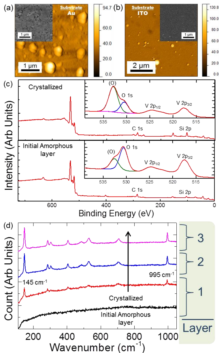
Figure 4. Post-crystallization AFM and SEM (insets) images of V_2O_5 thin films on (a) Au and (b) ITO substrates. The images show the formation of dispersed crystallites on the surface. (c) XPS spectra of amorphous and crystalline V_2O_5 thin films on ITO showing the contribution of photoelectron emission from the underlying substrate due to the thinness of the film. (d) Raman scattering spectra of the as-deposited and crystallized films for successive films in the multilayer.
