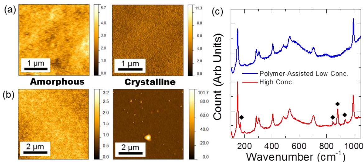
Figure 5. AFM images pre- and post-crystallization for (a) polymer-assisted low concentration and (b) high concentration \text{V}_2\text{O}_5 thin films formed on ITO. (c) Raman scattering spectra showing the formation of crystalline orthorhombic \text{V}_2\text{O}_5 from both films. The peaks marked with diamonds are due to the layered structure of the films and the presence of small amounts of \text{VO}_2 . The broad background seen in the polymer-assisted spectra between 400\text{ cm}^{-1} - 700\text{ cm}^{-1} is due to the thinness of the film and the interaction with the ITO and glass substrate.
